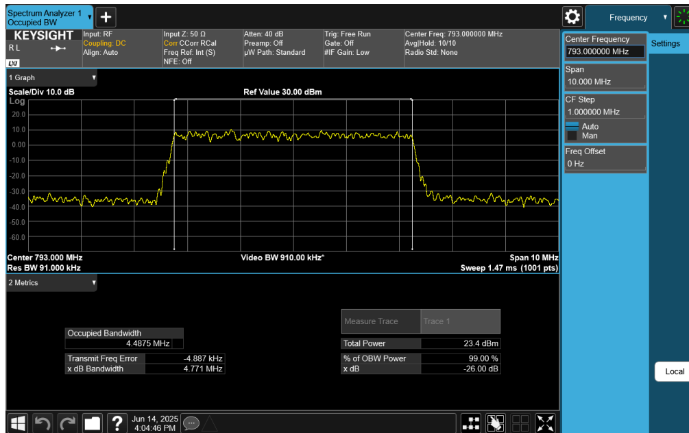
Plot 7-23. Occupied Bandwidth Plot (NR Band 14 - 5MHz CP-OFDM 16-QAM - Full RB Configuration)
