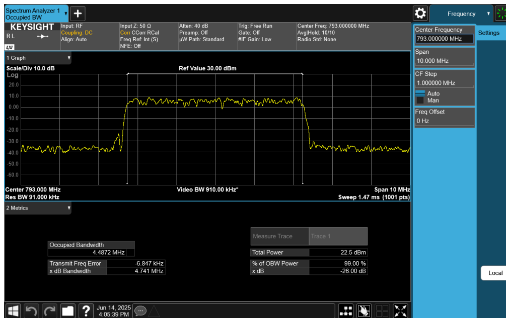
Plot 7-24. Occupied Bandwidth Plot (NR Band 14 - 5MHz CP-OFDM 64-QAM - Full RB Configuration)
