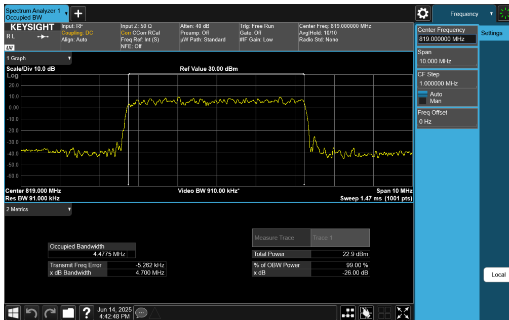
Plot 7-16. Occupied Bandwidth Plot (NR Band 26 - 5MHz CP-OFDM 64-QAM - Full RB Configuration)
