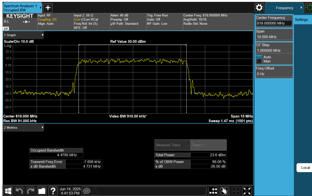
Plot 7-15. Occupied Bandwidth Plot (NR Band 26 - 5MHz CP-OFDM 16-QAM - Full RB Configuration)
