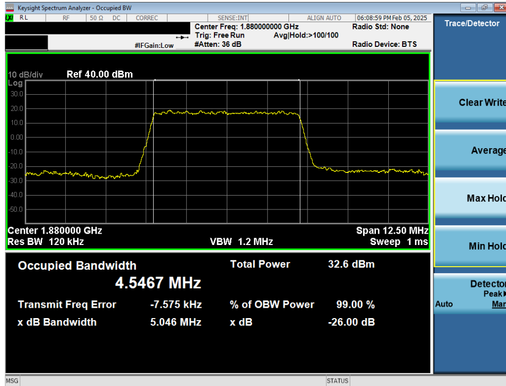
Plot 7-5. Occupied Bandwidth Plot (LTE Band 25/2 - 5MHz QPSK - Full RB Configuration)
