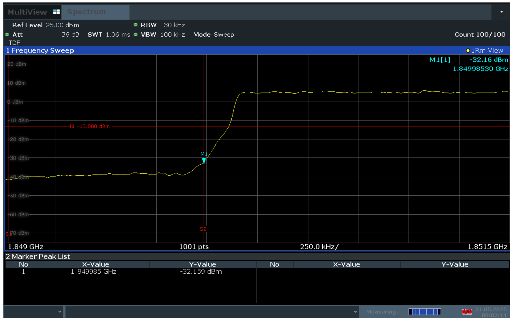
Plot 7-51. Lower Band Edge Plot (LTE Band 25 – 3MHz QPSK – Full RB Configuration)
