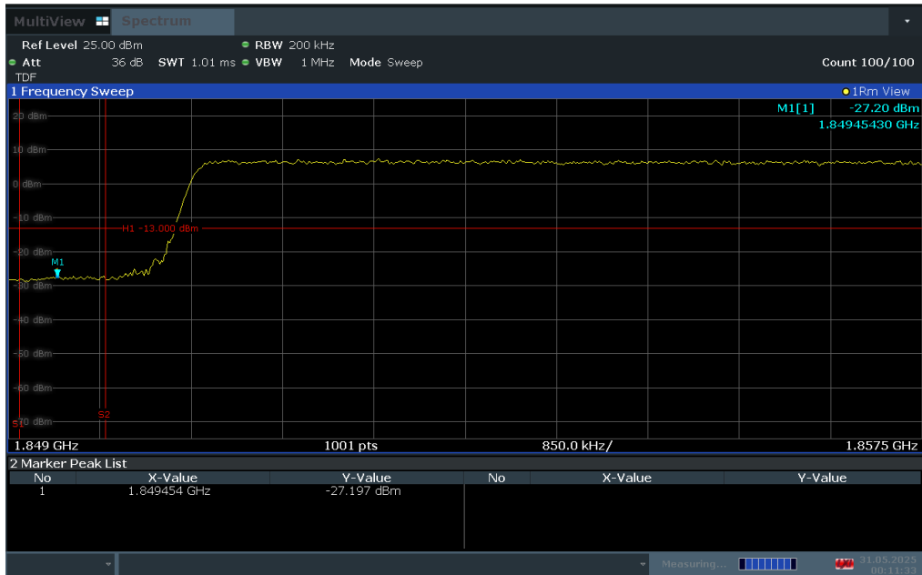
Plot 7-63. Lower Band Edge Plot (LTE Band 25 – 15MHz QPSK – Full RB Configuration)
