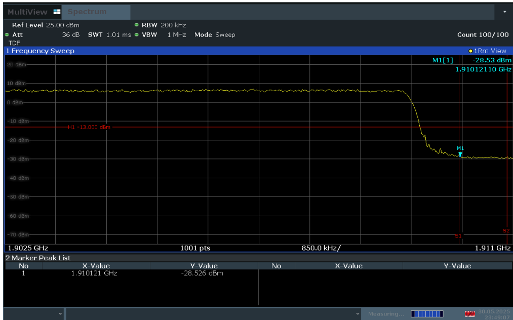
Plot 7-89. Upper Band Edge Plot (LTE Band 2 – 15MHz QPSK – Full RB Configuration)
