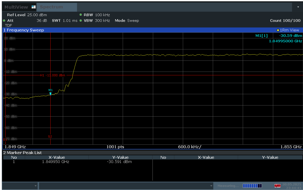
Plot 7-83. Lower Band Edge Plot (LTE Band 2 – 10MHz QPSK – Full RB Configuration)
