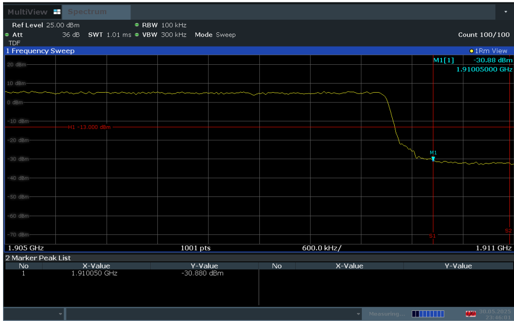
Plot 7-85. Upper Band Edge Plot (LTE Band 2 – 10MHz QPSK – Full RB Configuration)
