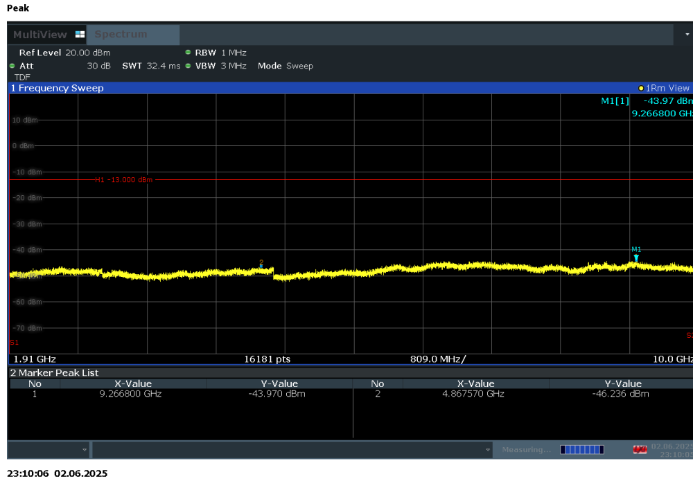
Plot 7-33. Conducted Spurious Plot (LTE Band 25/2 - 20MHz QPSK - RB Size 1, RB Offset 50 - Mid Channel)
