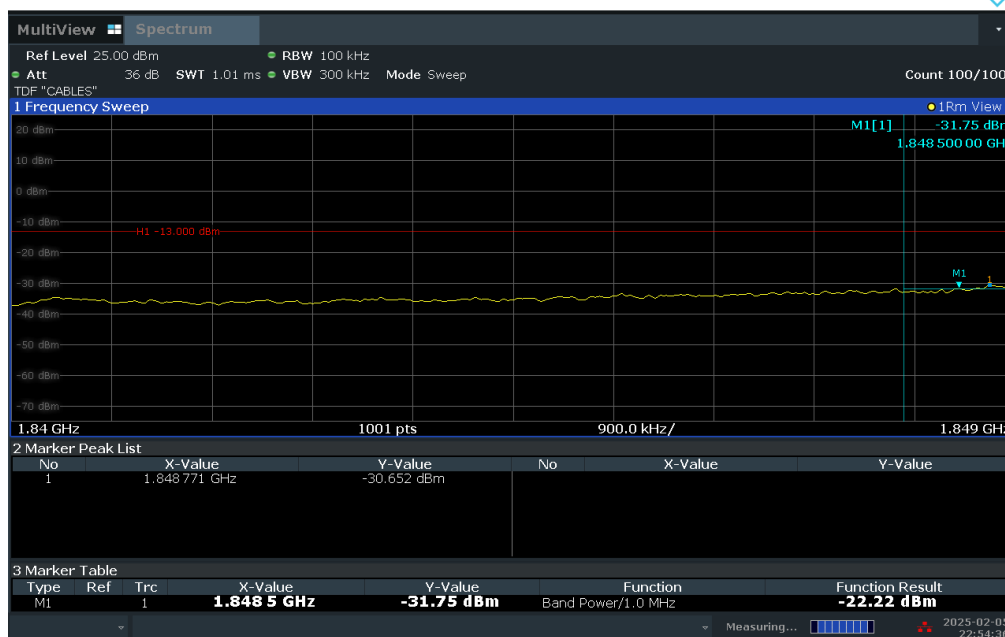
Plot 7-68. Extended Lower Band Edge Plot (LTE Band 25 – 20MHz QPSK – Full RB Configuration)
