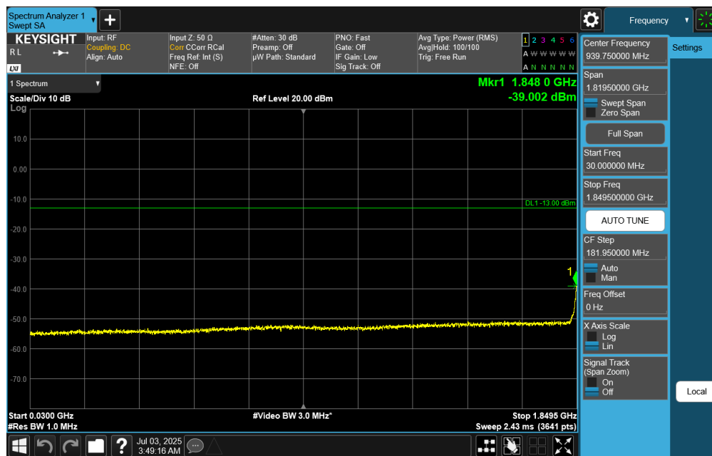
Plot 7-38. Conducted Spurious Plot (NR Band n25/n2 - 20.0MHz - RB Size 1, RB Offset 50 - Low Channel)
