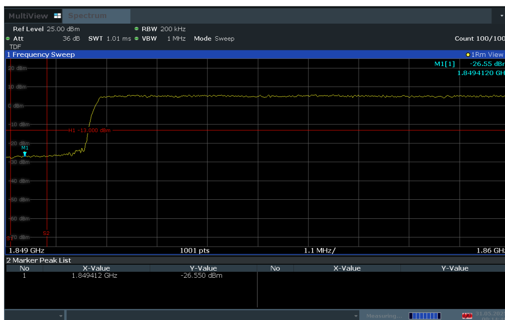
Plot 7-67. Lower Band Edge Plot (LTE Band 25 – 20MHz QPSK – Full RB Configuration)
