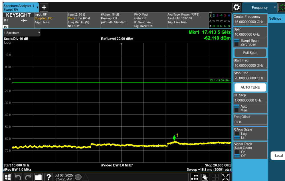
Plot 7-43. Conducted Spurious Plot (NR Band n25/n2 - 20.0MHz - RB Size 1, RB Offset 50 - Mid Channel)
