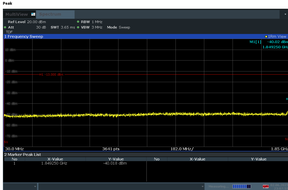
Plot 7-29. Conducted Spurious Plot (LTE Band 25/2 - 20MHz QPSK - RB Size 1, RB Offset 50 - Low Channel)
