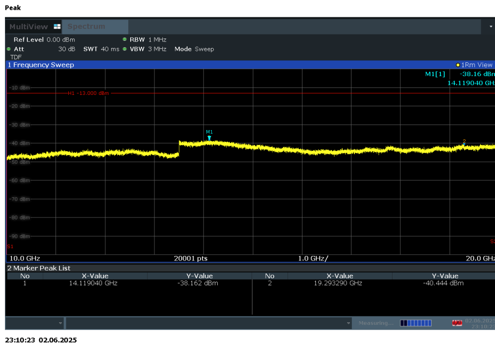
Plot 7-34. Conducted Spurious Plot (LTE Band 25/2 - 20MHz QPSK - RB Size 1, RB Offset 50 - Mid Channel)
