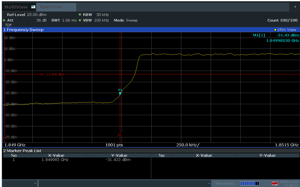
Plot 7-75. Lower Band Edge Plot (LTE Band 2 – 3MHz QPSK – Full RB Configuration)
