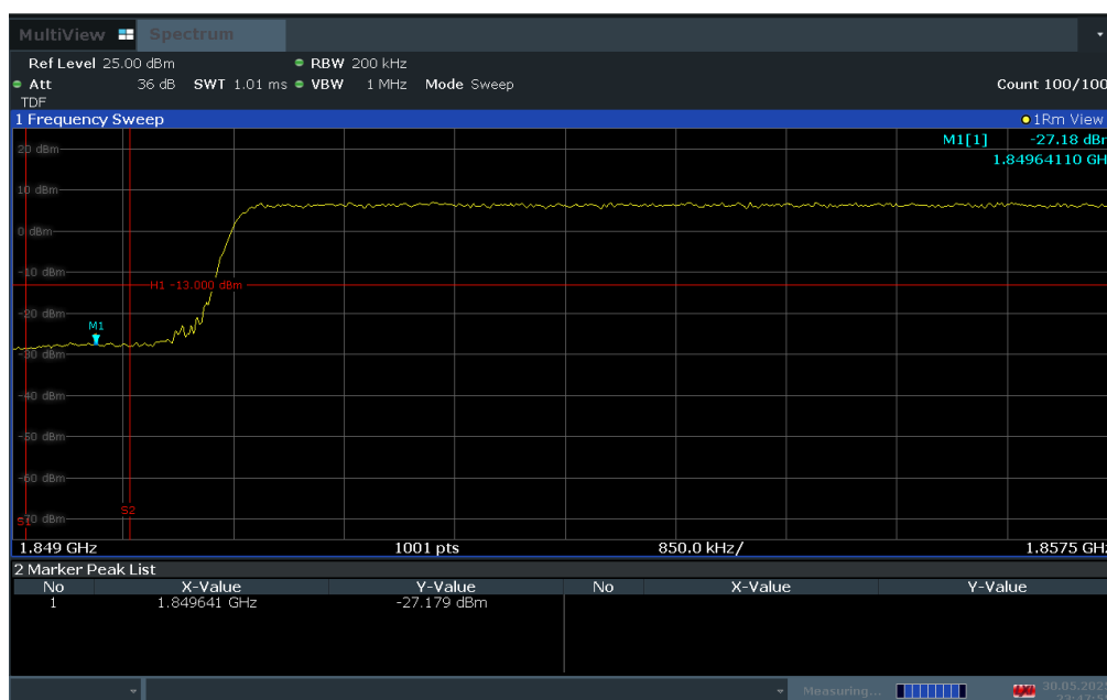
Plot 7-87. Lower Band Edge Plot (LTE Band 2 – 15MHz QPSK – Full RB Configuration)
