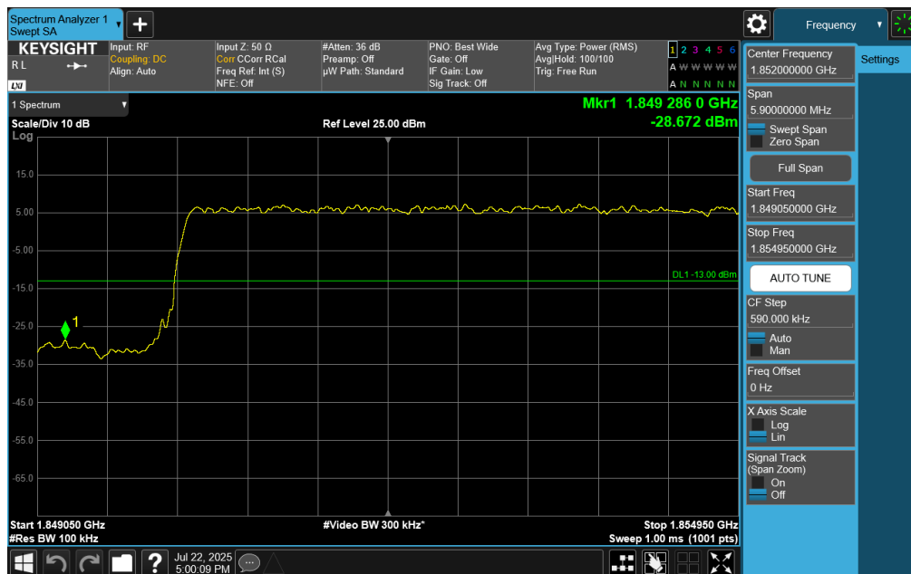
Plot 7-99. Lower Band Edge Plot (NR Band n25 – 10MHz DF-OFDM BPSK – Full RB Configuration)
