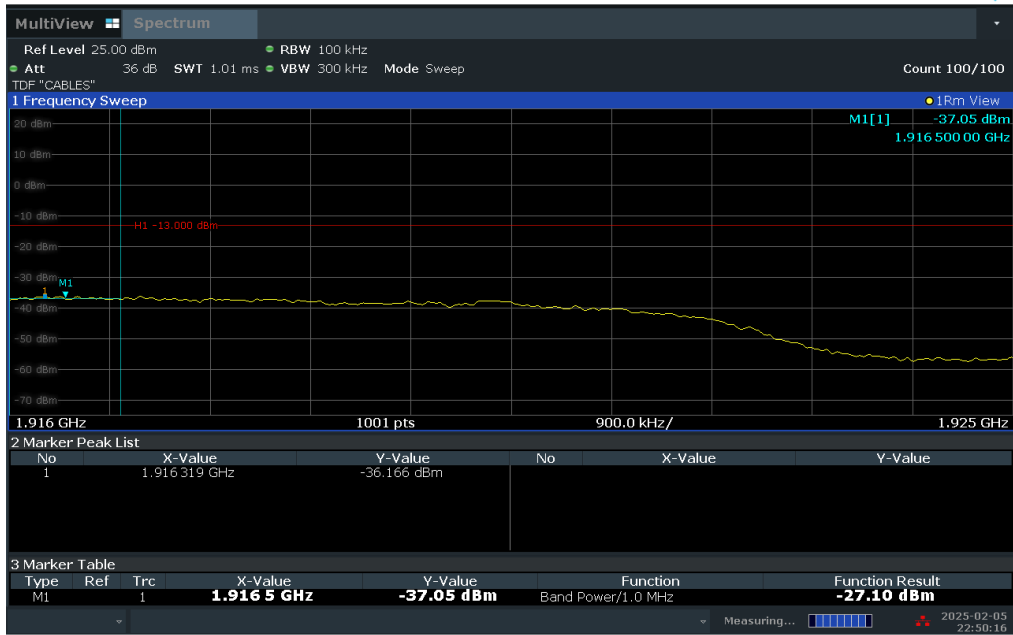
Plot 7-62. Extended Upper Band Edge Plot (LTE Band 25 – 10MHz QPSK – Full RB Configuration)
