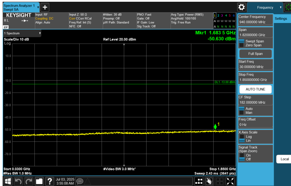
Plot 7-44. Conducted Spurious Plot (NR Band n25/n2 - 20.0MHz - RB Size 1, RB Offset 50 - High Channel)
