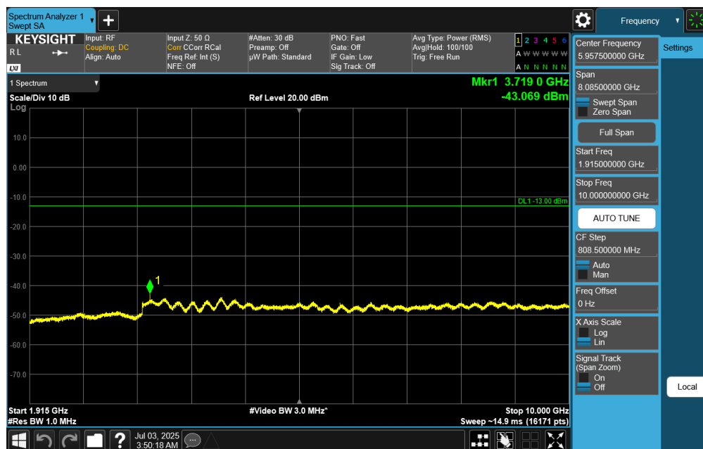
Plot 7-39. Conducted Spurious Plot (NR Band n25/n2 - 20.0MHz - RB Size 1, RB Offset 50 - Low Channel)
