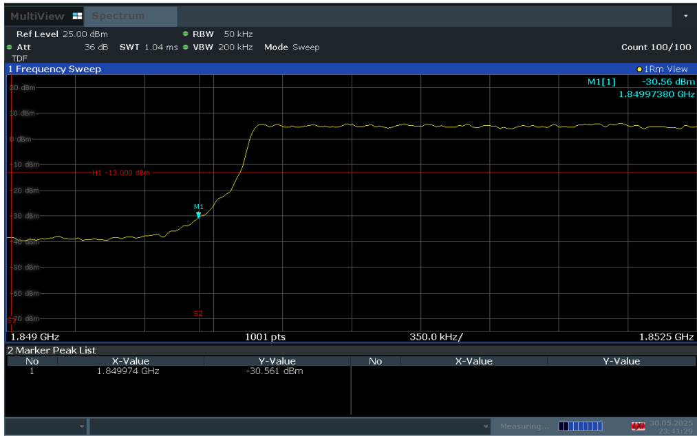
Plot 7-79. Lower Band Edge Plot (LTE Band 2 – 5MHz QPSK – Full RB Configuration)
