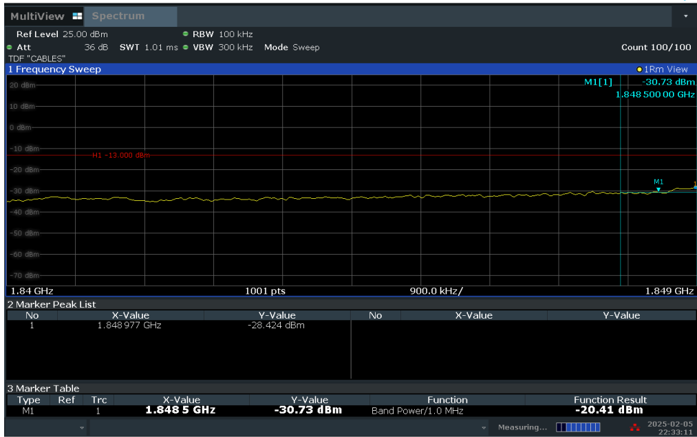
Plot 7-92. Extended Lower Band Edge Plot (LTE Band 2 – 20MHz QPSK – Full RB Configuration)
