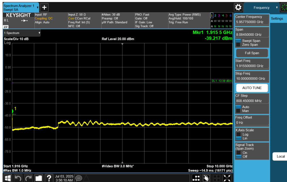
Plot 7-45. Conducted Spurious Plot (NR Band n25/n2 - 20.0MHz - RB Size 1, RB Offset 50 - High Channel)
