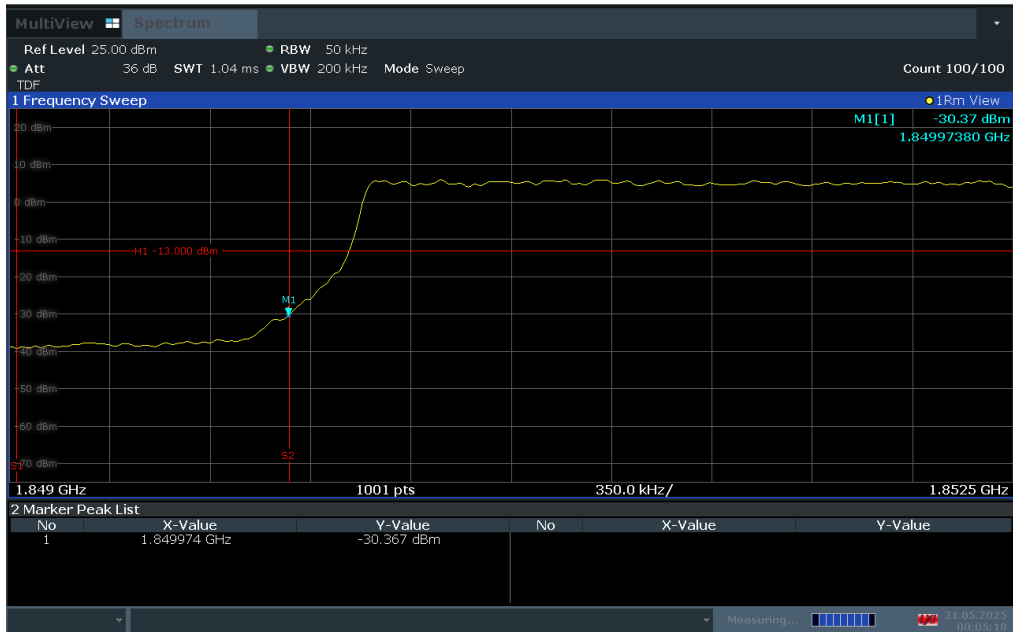
Plot 7-55. Lower Band Edge Plot (LTE Band 25 – 5MHz QPSK – Full RB Configuration)
