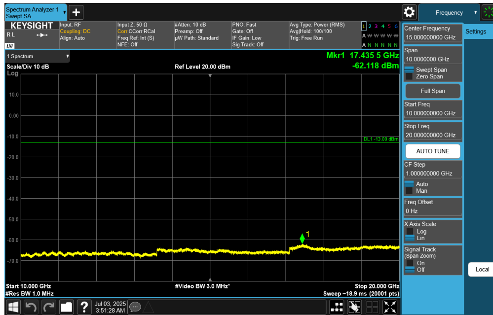
Plot 7-40. Conducted Spurious Plot (NR Band n25/n2 - 20.0MHz - RB Size 1, RB Offset 50 - Low Channel)
