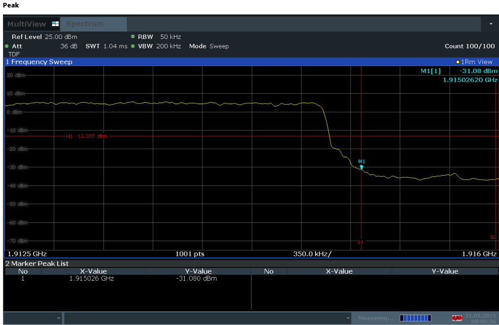
Plot 7-57. Upper Band Edge Plot (LTE Band 25 – 5MHz QPSK – Full RB Configuration)
