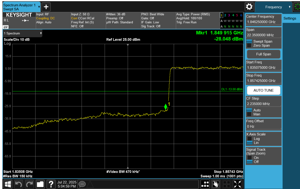
Plot 7-103. Lower Band Edge Plot (NR Band n25 – 15MHz DF-OFDM BPSK – Full RB Configuration)
