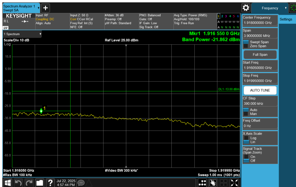
Plot 7-98. Extended Upper Band Edge Plot (NR Band n25 – 5MHz DF-OFDM BPSK – Full RB Configuration)
