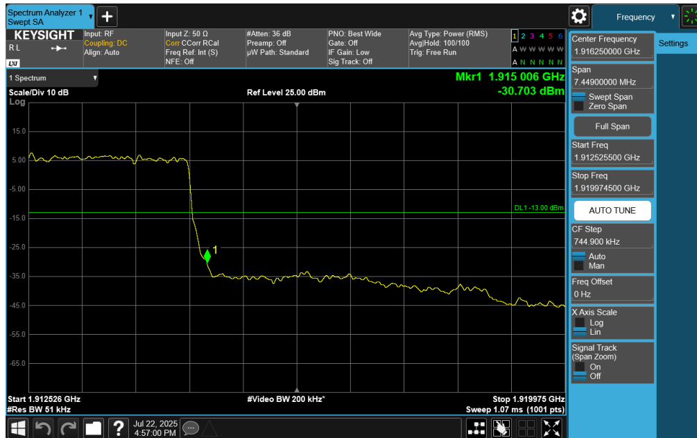
Plot 7-97. Upper Band Edge Plot (NR Band n25 – 5MHz DF-OFDM BPSK – Full RB Configuration)
