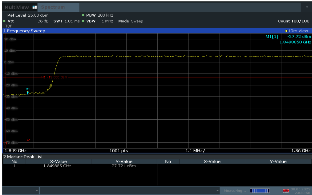
Plot 7-91. Lower Band Edge Plot (LTE Band 2 – 20MHz QPSK – Full RB Configuration)
