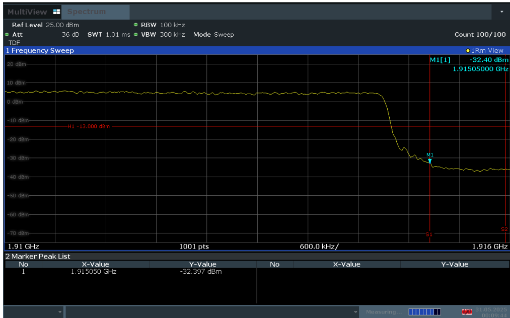
Plot 7-61. Upper Band Edge Plot (LTE Band 25 – 10MHz QPSK – Full RB Configuration)
