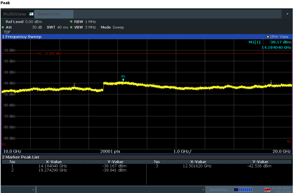
Plot 7-37. Conducted Spurious Plot (LTE Band 25/2 - 20MHz QPSK - RB Size 1, RB Offset 50 - High Channel)
