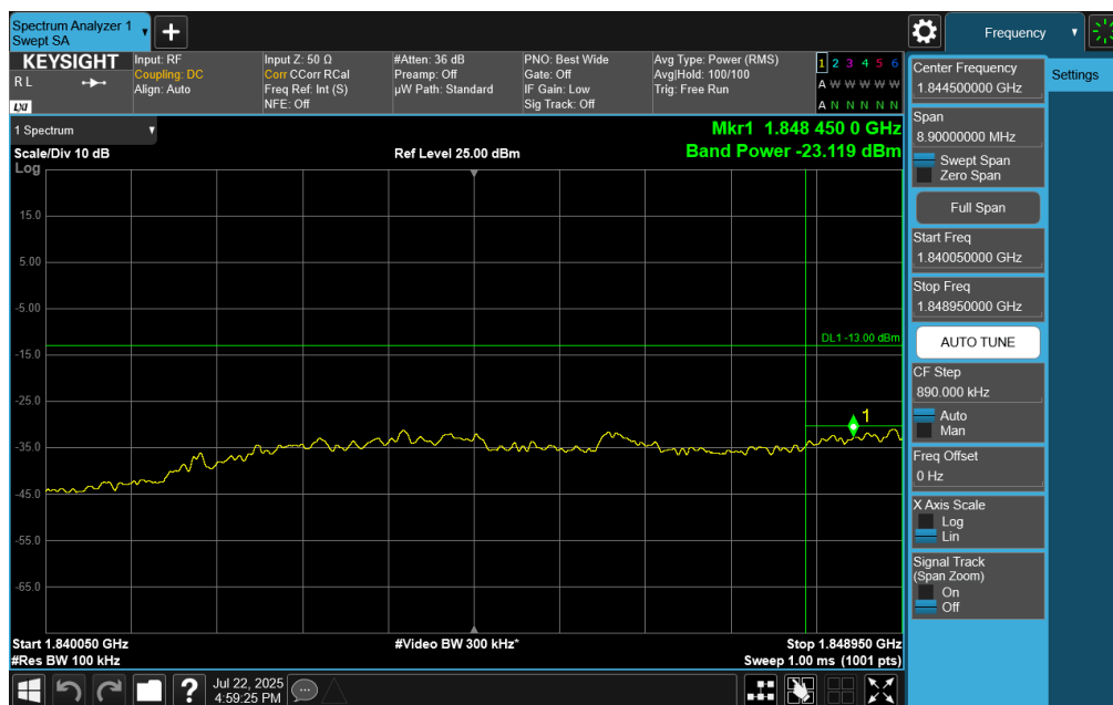
Plot 7-100. Extended Lower Band Edge Plot (NR Band n25 – 10MHz DF-OFDM BPSK – Full RB Configuration)
