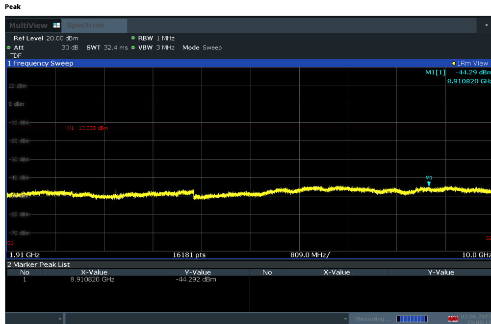
Plot 7-30. Conducted Spurious Plot (LTE Band 25/2 - 20MHz QPSK - RB Size 1, RB Offset 50 - Low Channel)
