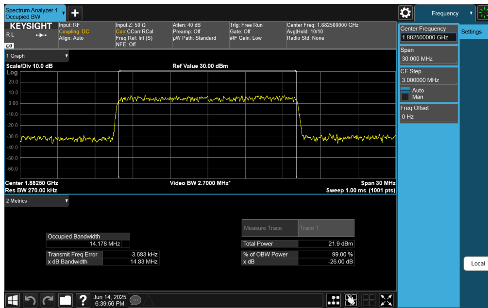
Plot 7-22. Occupied Bandwidth Plot (NR Band n25/n2 - 15.0MHz CP-OFDM QPSK - Full RB)
