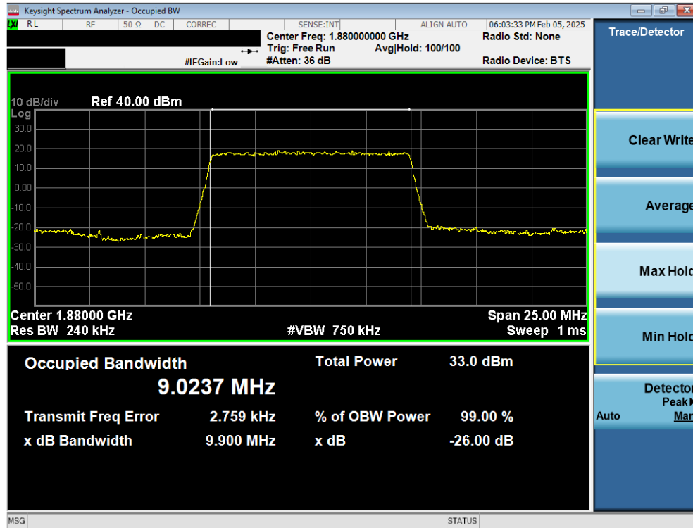
Plot 7-7. Occupied Bandwidth Plot (LTE Band 25/2 - 10MHz QPSK - Full RB Configuration)
