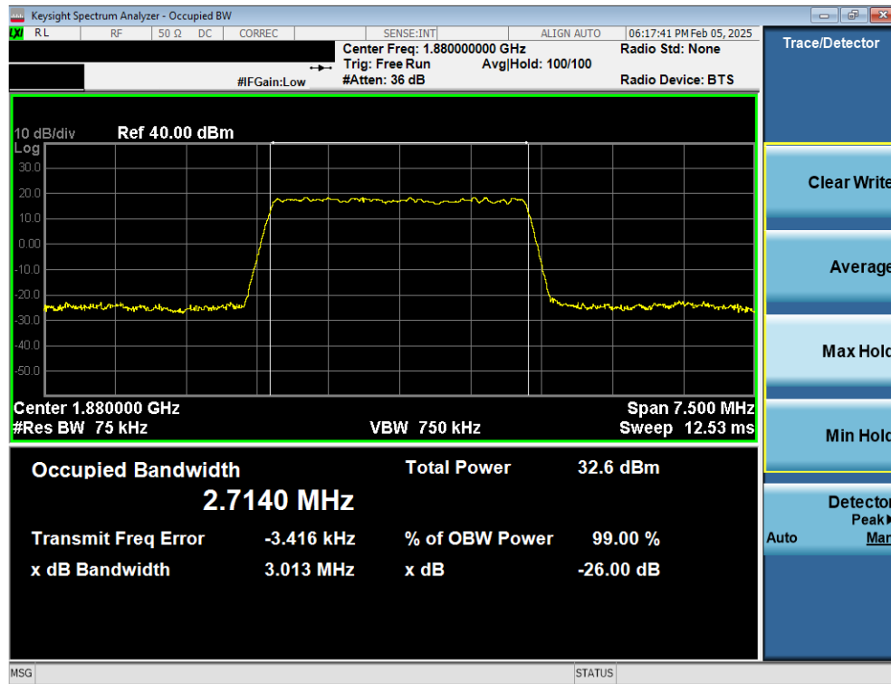
Plot 7-3. Occupied Bandwidth Plot (LTE Band 25/2 - 3MHz QPSK - Full RB Configuration)
