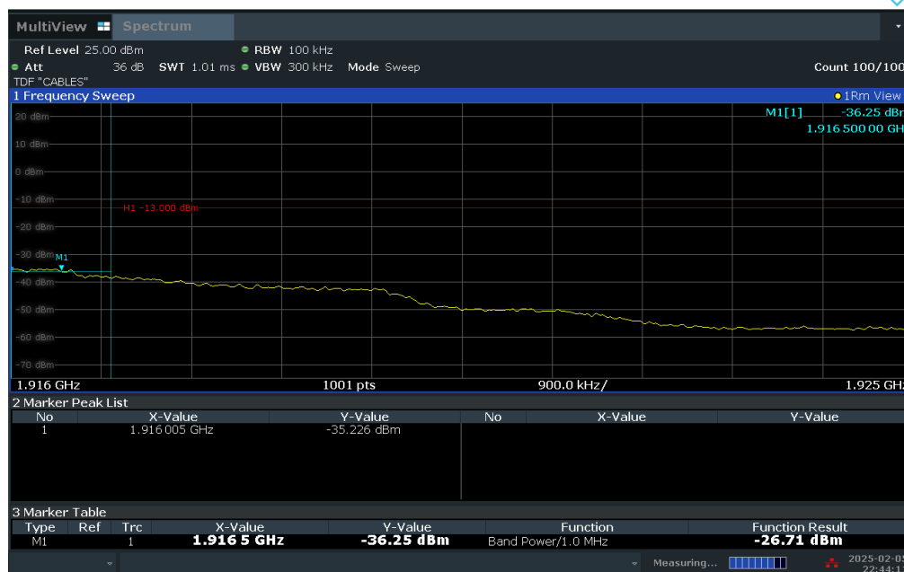
Plot 7-54. Extended Upper Power Edge Plot (LTE Band 25 – 3MHz QPSK – Full RB Configuration)
