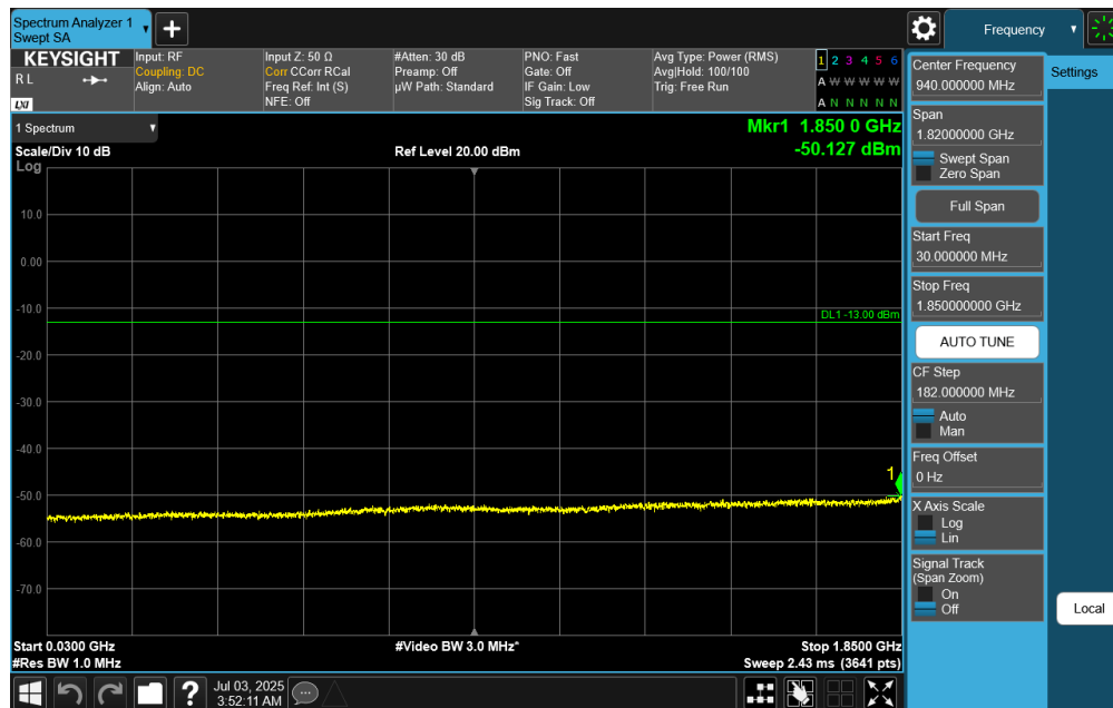
Plot 7-41. Conducted Spurious Plot (NR Band n25/n2 - 20.0MHz - RB Size 1, RB Offset 50 - Mid Channel)
