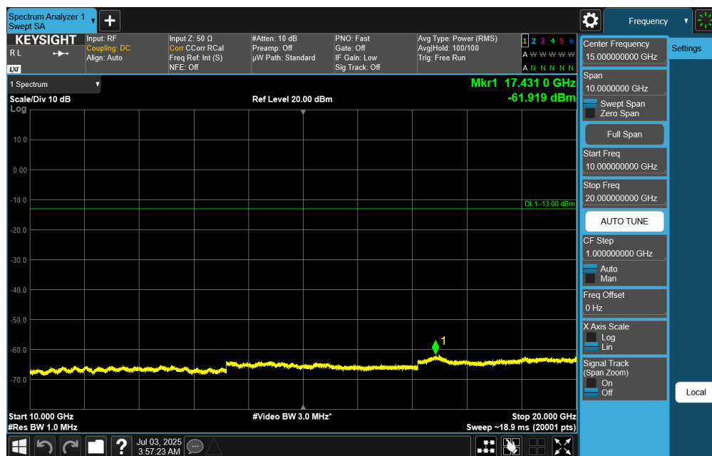
Plot 7-46. Conducted Spurious Plot (NR Band n25/n2 - 20.0MHz - RB Size 1, RB Offset 50 - High Channel)
