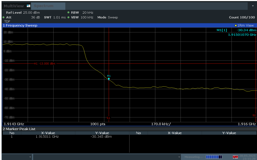
Plot 7-49. Upper Band Edge Plot (LTE Band 25 – 1.4MHz QPSK – Full RB Configuration)
