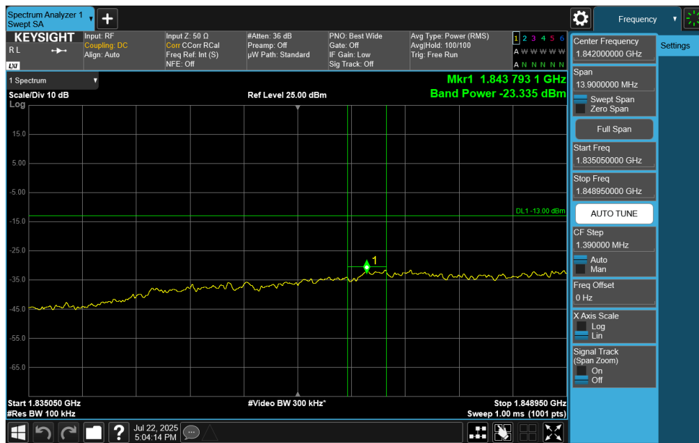
Plot 7-104. Extended Lower Band Edge Plot (NR Band n25 – 15MHz DF-OFDM BPSK – Full RB Configuration)
