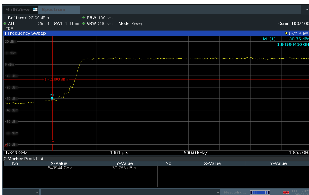
Plot 7-59. Lower Band Edge Plot (LTE Band 25 – 10MHz QPSK – Full RB Configuration)
