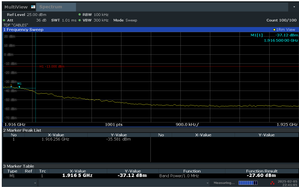
Plot 7-50. Extended Upper Band Edge Plot (LTE Band 25 – 1.4MHz QPSK – Full RB Configuration)
