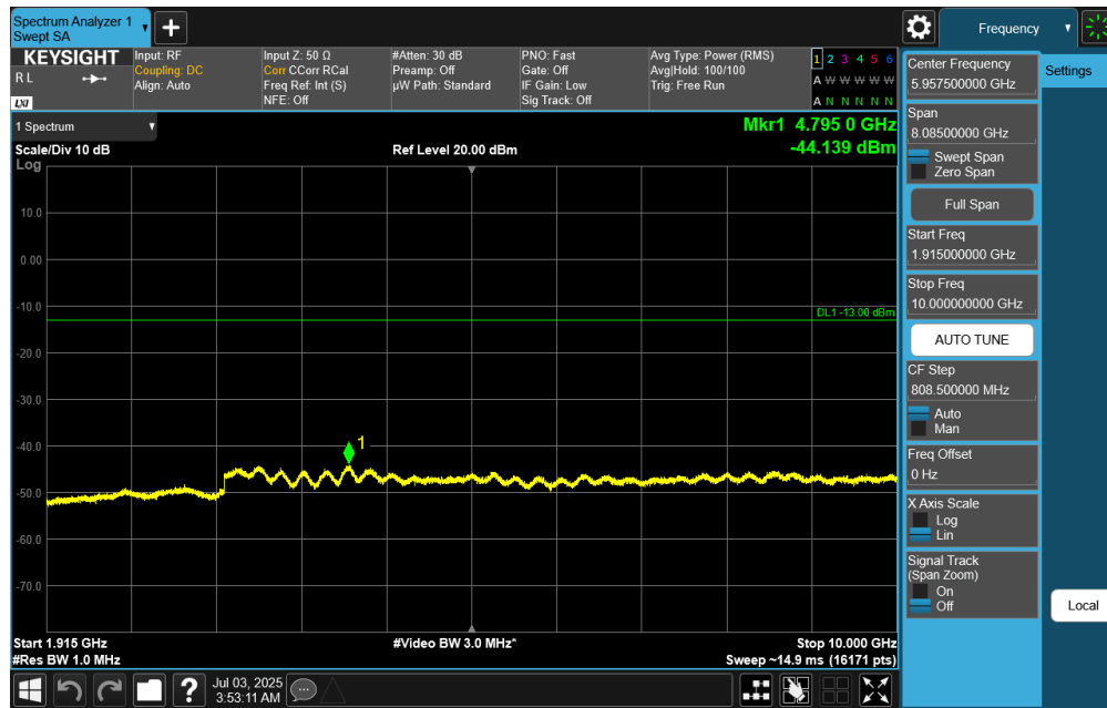
Plot 7-42. Conducted Spurious Plot (NR Band n25/n2 - 20.0MHz - RB Size 1, RB Offset 50 - Mid Channel)
