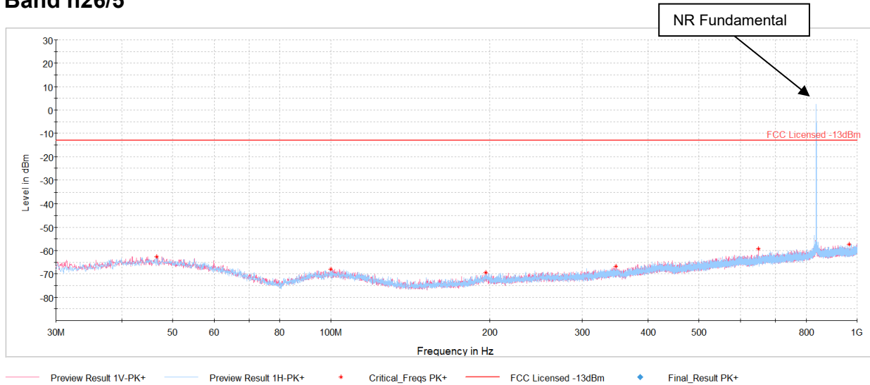
Plot 7-77. Antenna BCM Radiated Spurious Plot below 1GHz (NR Band n26/5)
