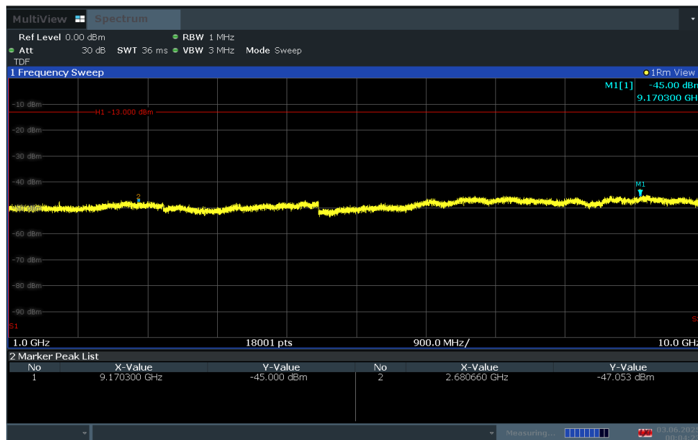
Plot 7-27. Conducted Spurious Plot (LTE Band 26/5 - 10MHz QPSK - RB Size 1, RB Offset 14 - Low Channel)
