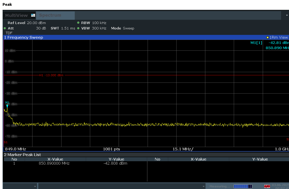
Plot 7-32. Conducted Spurious Plot (LTE Band 26/5 - 10MHz QPSK - RB Size 1, RB Offset 14 - High Channel)
