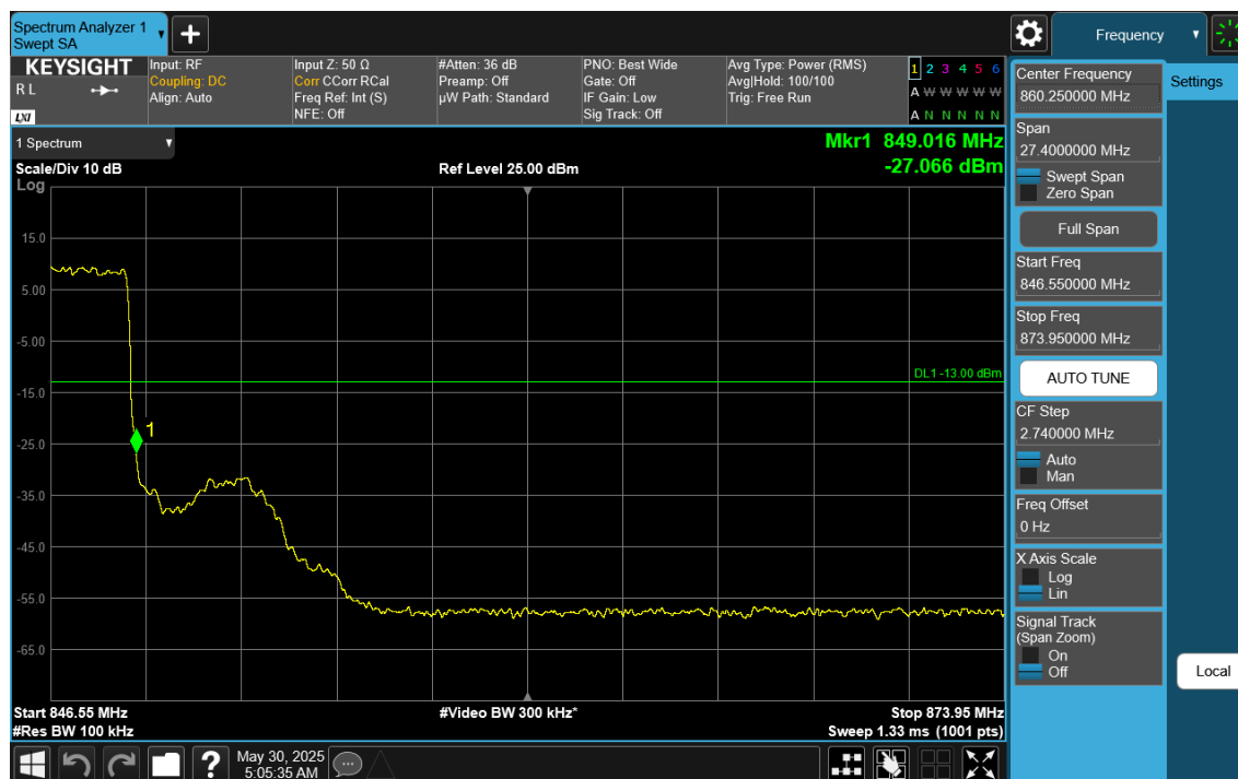
Plot 7-60. Upper BE Plot (NR Band n26 CP-OFDM \pi/2 BPSK – 5.0MHz - Full RB)
