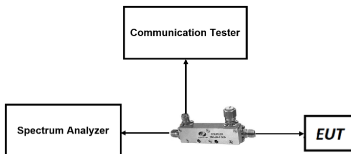
Figure 7-5. LTE Test Instrument & Measurement Setup
