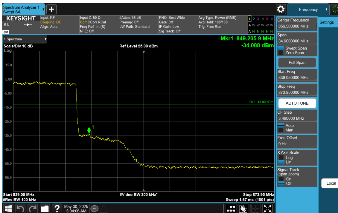
Plot 7-66. Upper BE Plot (NR Band n26 DFT-s-OFDM QPSK – 20.0MHz - Full RB)
