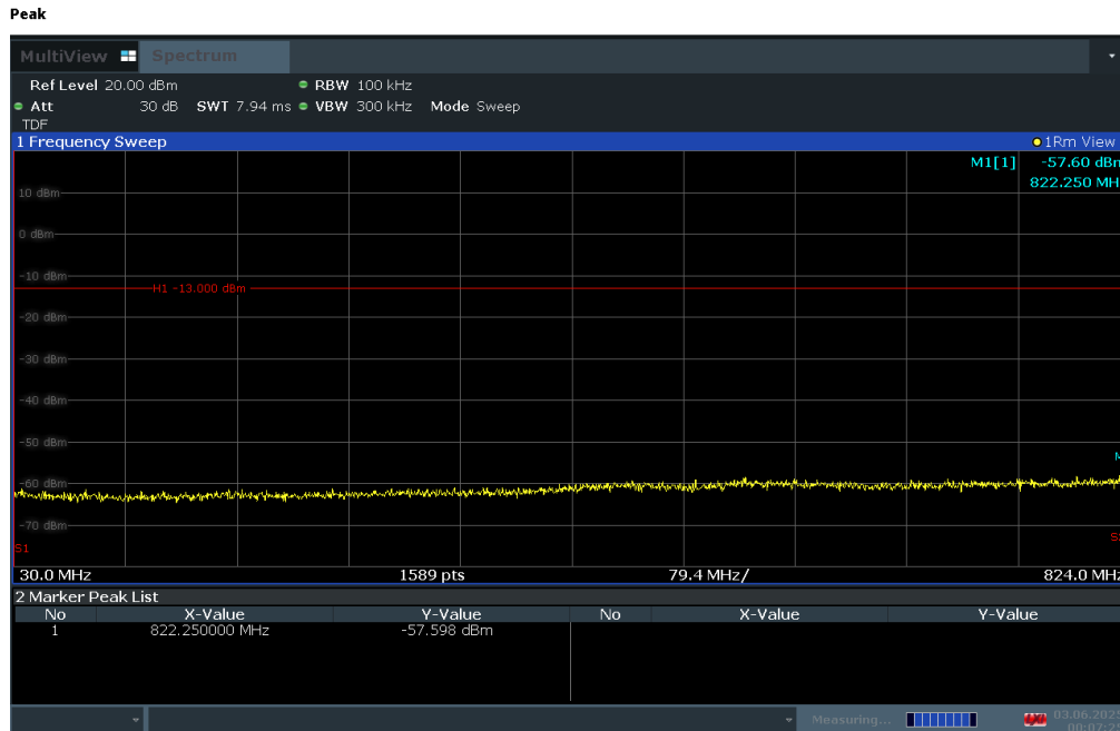
Plot 7-31. Conducted Spurious Plot (LTE Band 26/5 - 10MHz QPSK - RB Size 1, RB Offset 14 - High Channel)
