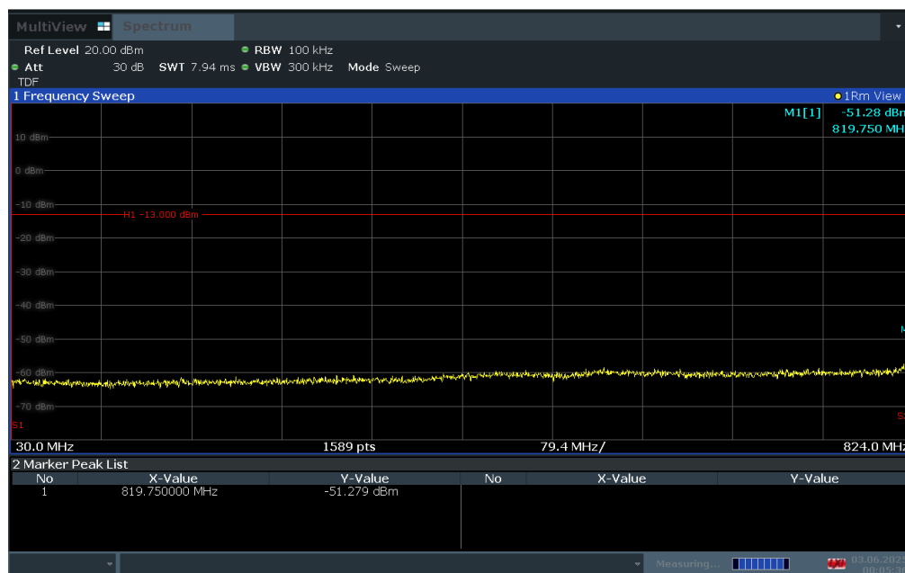
Plot 7-28. Conducted Spurious Plot (LTE Band 26/5 - 10MHz QPSK - RB Size 1, RB Offset 14 - Mid Channel)
