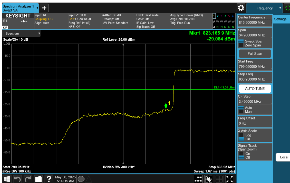
Plot 7-65. Lower BE Plot (NR Band n26 DFT-s-OFDM \pi/2 BPSK – 20.0MHz - Full RB)
