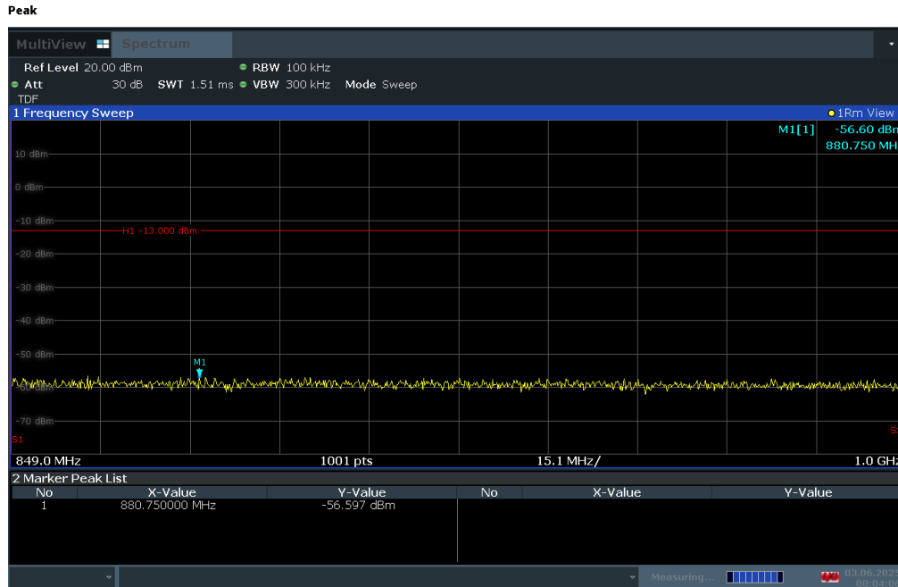
Plot 7-26. Conducted Spurious Plot (LTE Band 26/5 - 10MHz QPSK - RB Size 1, RB Offset 14 - Low Channel)
