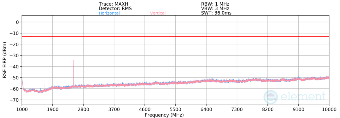
Plot 7-78. Antenna BCM Radiated Spurious Plot above 1GHz (NR Band n26/5)
