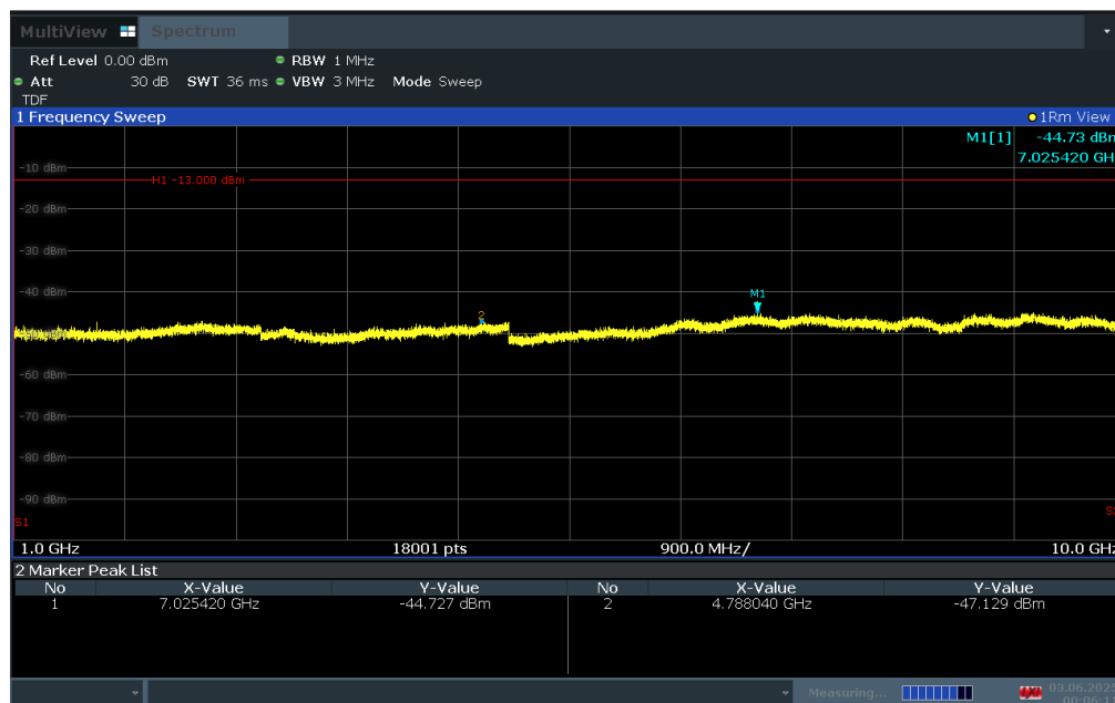
Plot 7-30. Conducted Spurious Plot (LTE Band 26/5 - 10MHz QPSK - RB Size 1, RB Offset 14 - Mid Channel)
