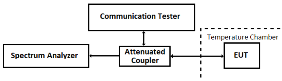
Figure 7-11. LTE Test Instrument & Measurement Setup
