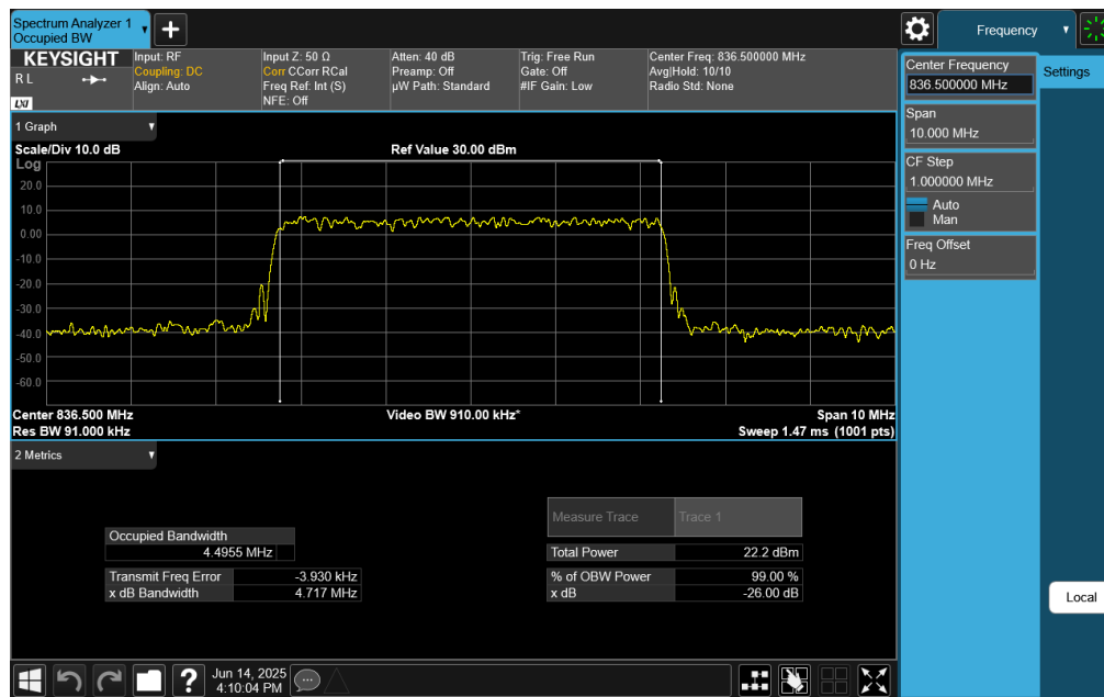
Plot 7-10. Occupied Bandwidth Plot (NR Band n26/n5 - 5MHz CP-OFDM QPSK - Full RB Configuration)
