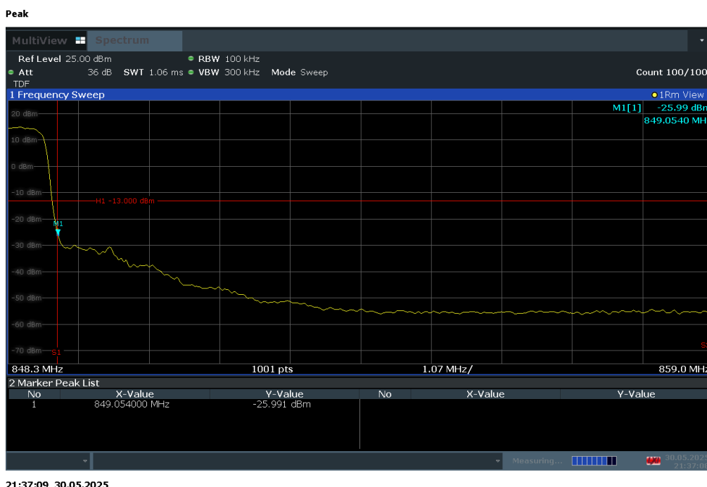
Plot 7-44. Upper BE Plot (LTE Band 26 – 1.4MHz QPSK – Full RB Configuration)
