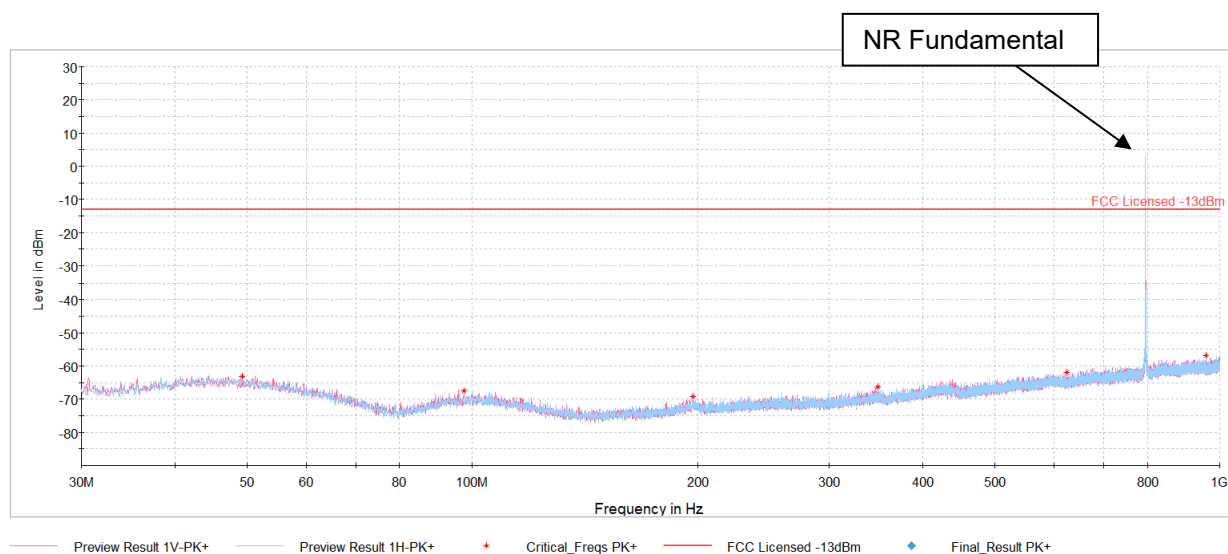
Plot 7-111. Antenna BCM Radiated Spurious Plot Below 1GHz (NR Band n14)
