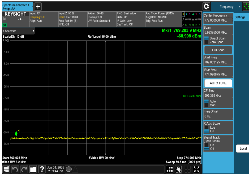
Plot 7-101. Lower Emission Mask Plot (NR Band n14, 10MHz DFT-s-OFDM \pi/2 BPSK – RB Size 50)
