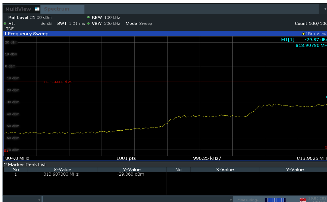
Plot 7-69. Channel Edge Plot (LTE Band 26 - 3MHz QPSK - Lower Channel)
