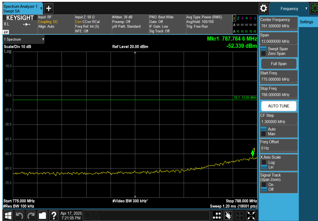
Plot 7-64. Conducted Spurious Plot (NR Band n14 - 5MHz DFT-s-OFDM QPSK - RB Size 1, RB Offset 12 - High Channel)
