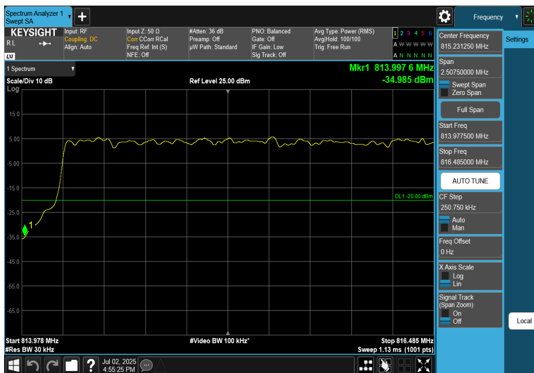
Plot 7-90. Channel Edge Plot (NR Band n26, 5MHz DFT-s-OFDM \pi/2 BPSK – Lower Channel)
