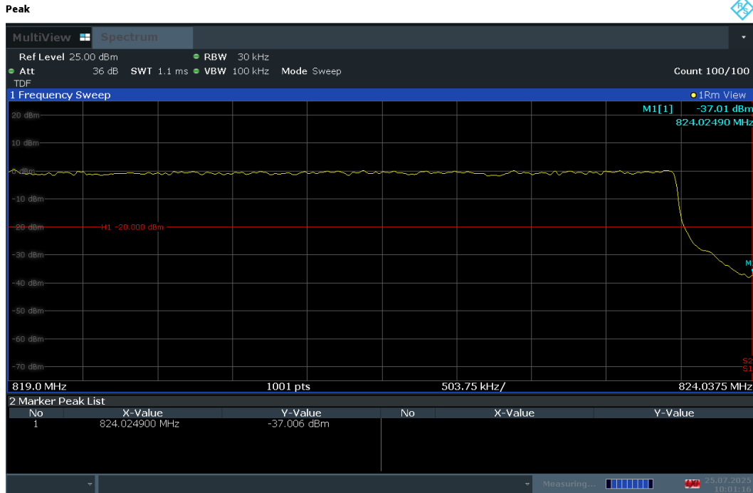
Plot 7-79. Channel Edge Plot (LTE Band 26 - 10MHz QPSK - Upper Channel)
