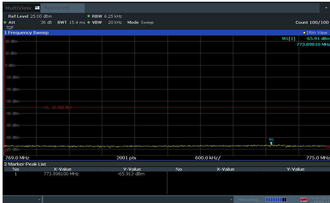
Plot 7-85. Lower Emission Mask Plot (LTE Band 14 - 10MHz QPSK – RB Size 50)
