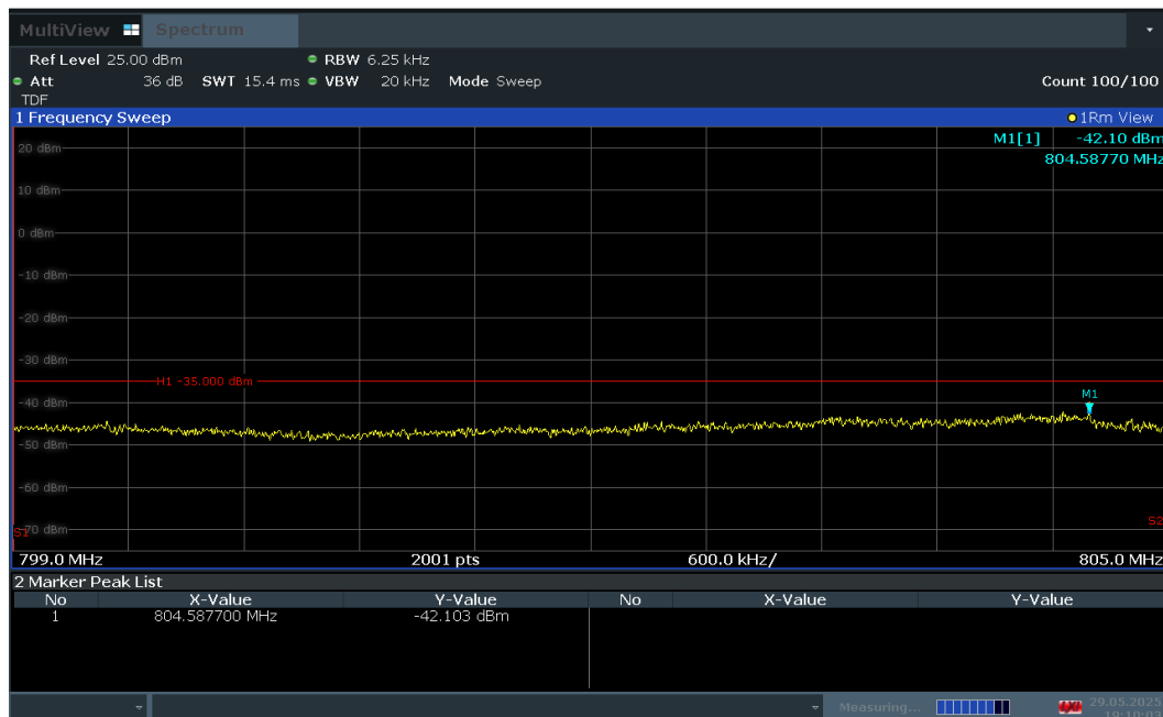
Plot 7-88. Upper Emission Mask Plot (LTE Band 14 - 10MHz QPSK – RB Size 50)
