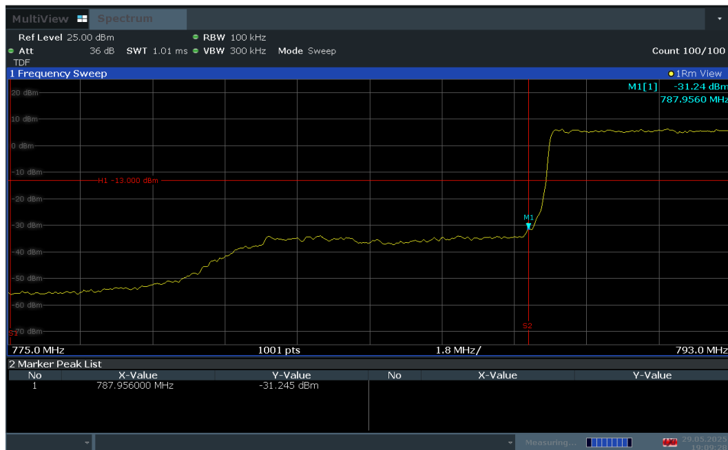
Plot 7-86. Lower Band Edge Plot (LTE Band 14 - 10MHz QPSK – RB Size 50)
