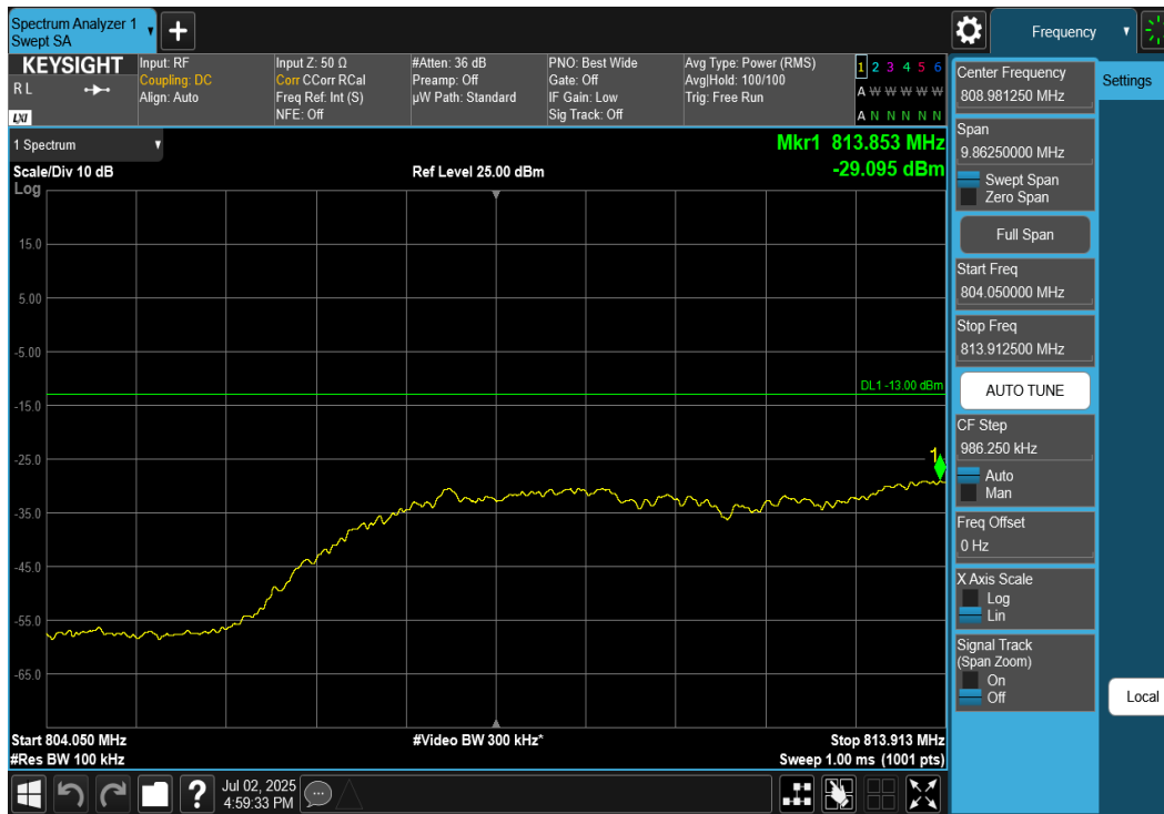
Plot 7-93. Channel Edge Plot (NR Band n26, 10MHz DFT-s-OFDM \pi/2 BPSK – Lower Channel)
