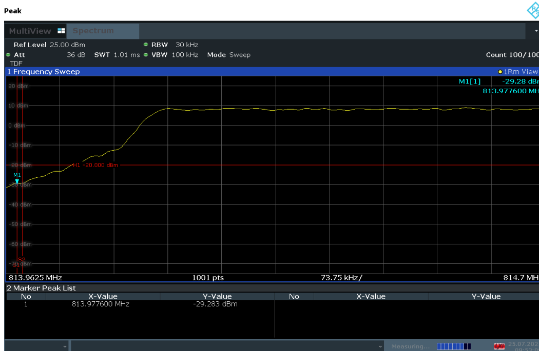
Plot 7-66. Channel Edge Plot (LTE Band 26 - 1.4MHz QPSK - Lower Channel)
