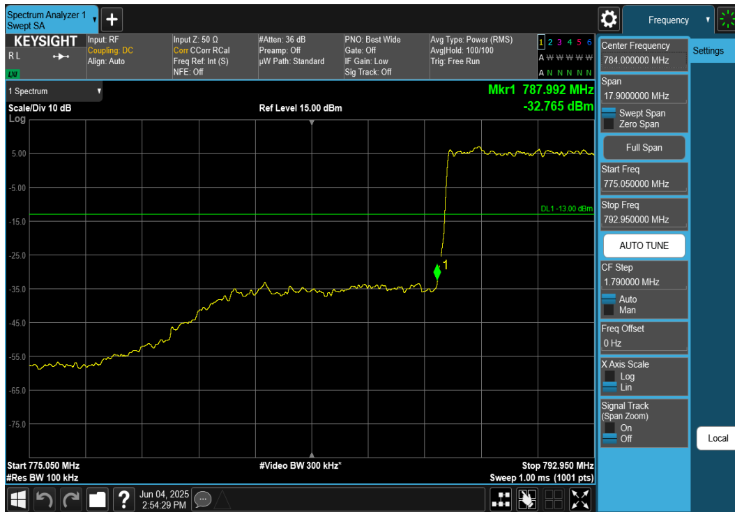
Plot 7-102. Lower Band Edge Plot (NR Band n14, 10MHz DFT-s-OFDM \pi/2 BPSK – RB Size 50)
