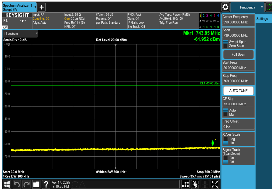
Plot 7-62. Conducted Spurious Plot (NR Band n14 - 5MHz DFT-s-OFDM QPSK - RB Size 1, RB Offset 12 - High Channel)
