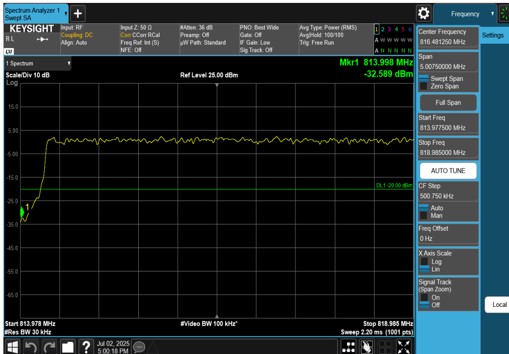
Plot 7-94. Channel Edge Plot (NR Band n26, 10MHz DFT-s-OFDM \pi/2 BPSK – Lower Channel)
