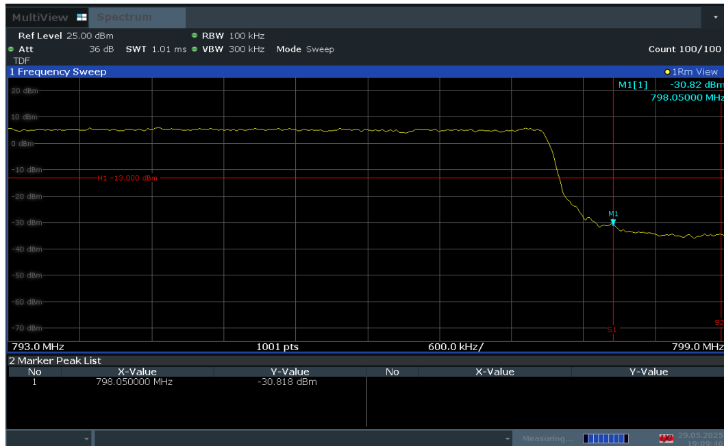
Plot 7-87. Upper Band Edge Plot (LTE Band 14 - 10MHz QPSK – RB Size 50)
