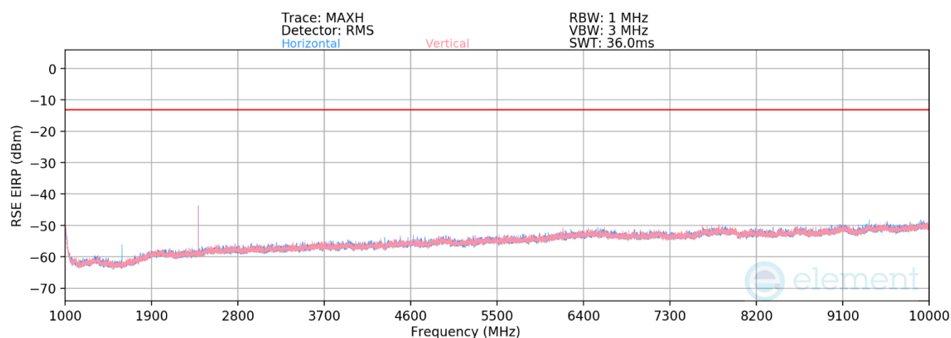
Plot 7-112. Antenna BCM Radiated Spurious Plot Above 1GHz (NR Band n14)
