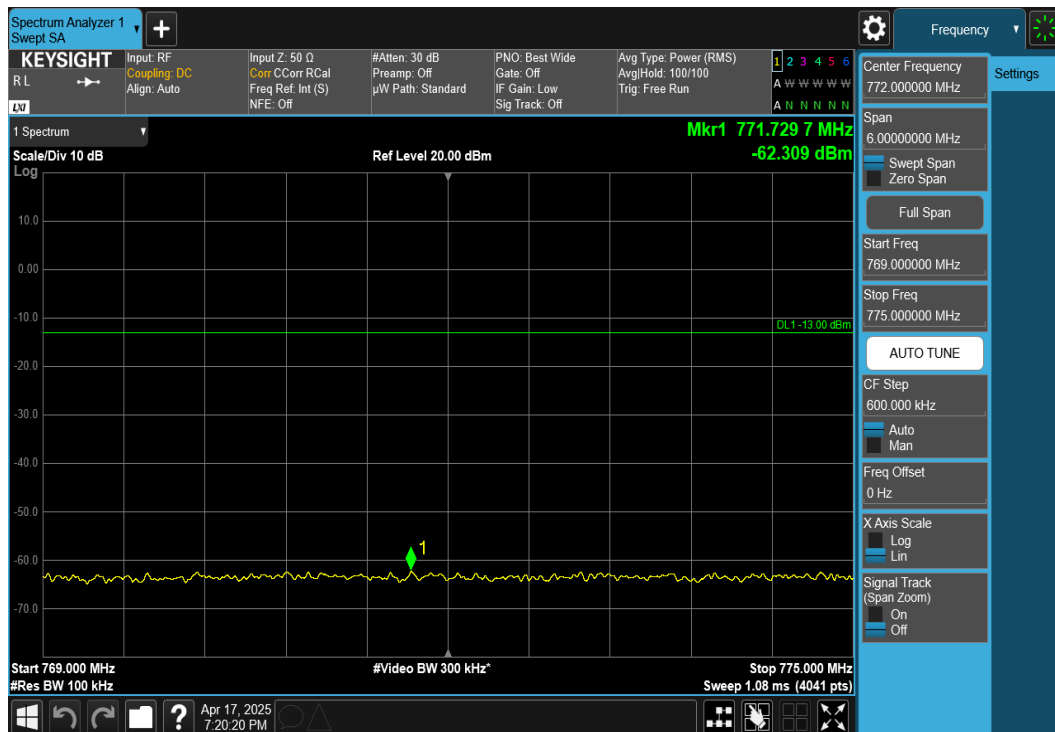
Plot 7-63. Conducted Spurious Plot (NR Band n14 - 5MHz DFT-s-OFDM QPSK - RB Size 1, RB Offset 12 - High Channel)
