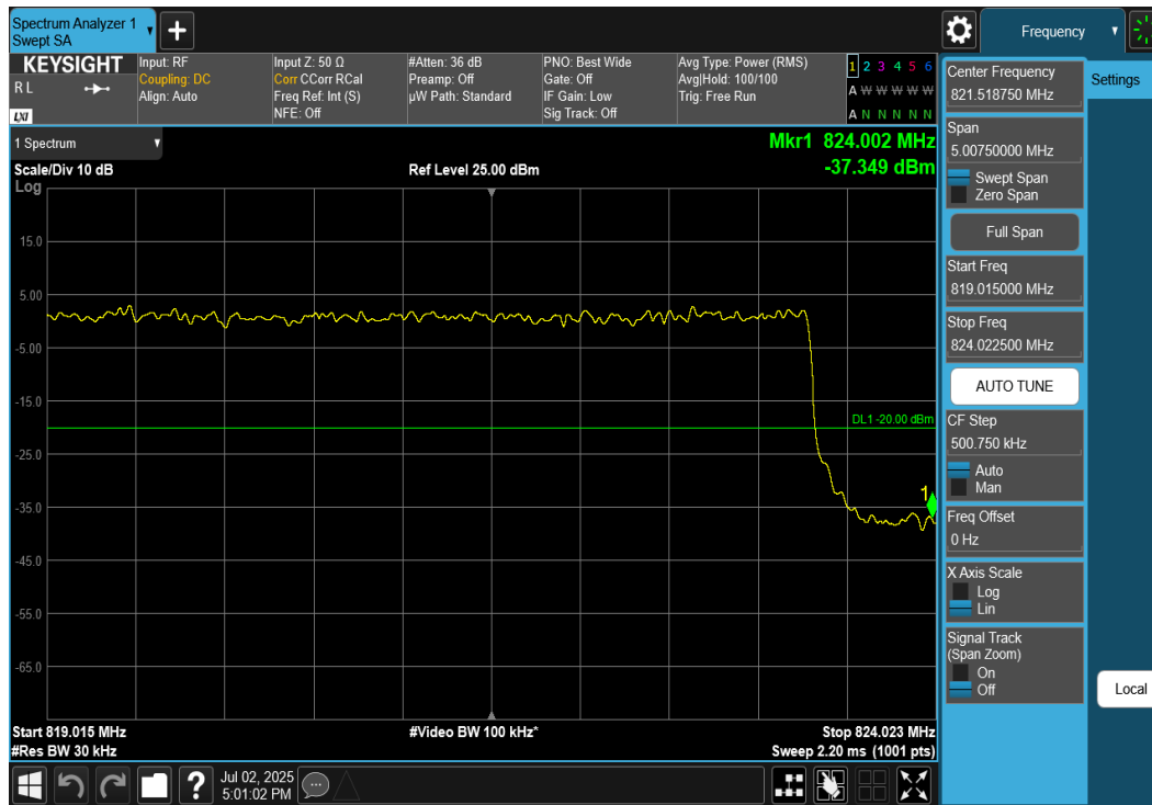
Plot 7-95. Channel Edge Plot (NR Band n26, 10MHz DFT-s-OFDM \pi/2 BPSK – Upper Channel)
