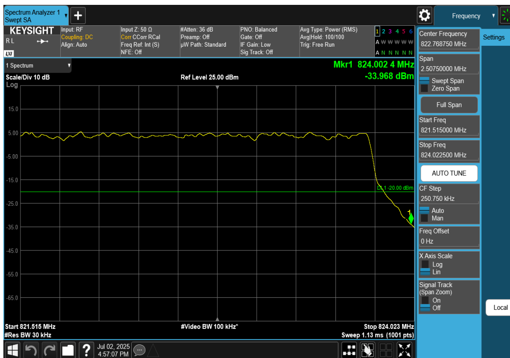
Plot 7-91. Channel Edge Plot (NR Band n26, 5MHz DFT-s-OFDM \pi/2 BPSK – Upper Channel)
