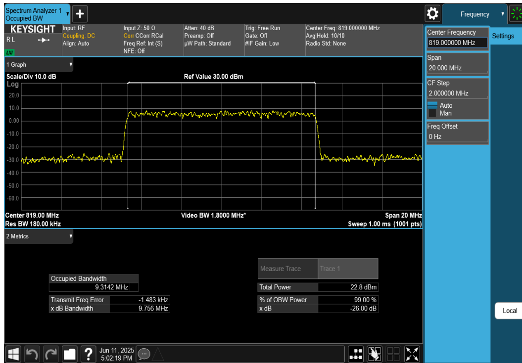
Plot 7-19. Occupied Bandwidth Plot (NR Band 26 - 10MHz CP-OFDM 16-QAM - Full RB Configuration)
