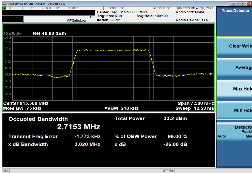
Plot 7-3. Occupied Bandwidth Plot (LTE Band 26 - 3MHz QPSK - Full RB Configuration)
