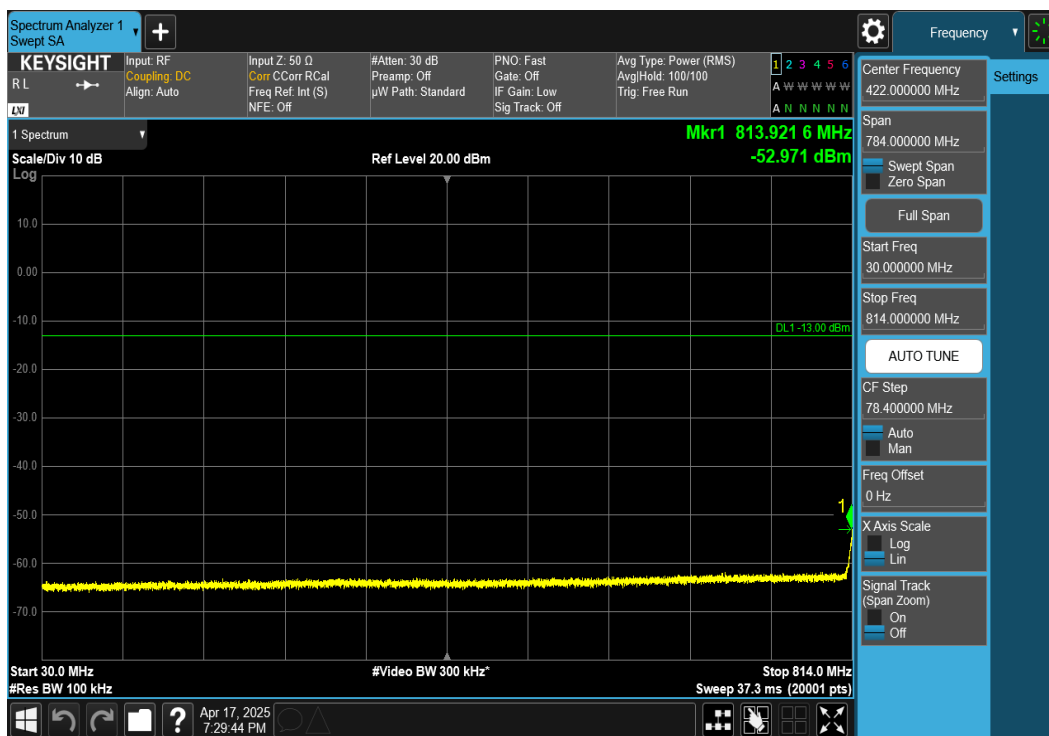
Plot 7-53. Conducted Spurious Plot (NR Band n26 - 5MHz DFT-s-OFDM QPSK - RB Size 1, RB Offset 12 - High Channel)
