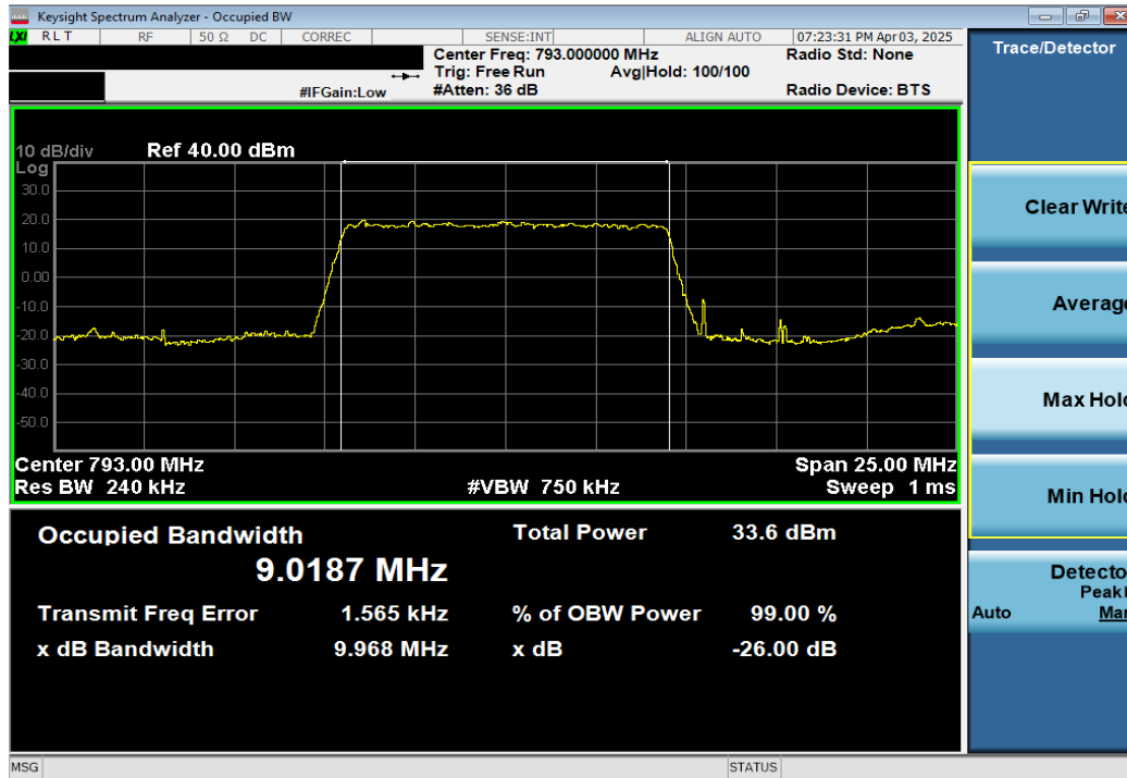
Plot 7-11. Occupied Bandwidth Plot (LTE Band 14 - 10MHz QPSK - Full RB Configuration)
