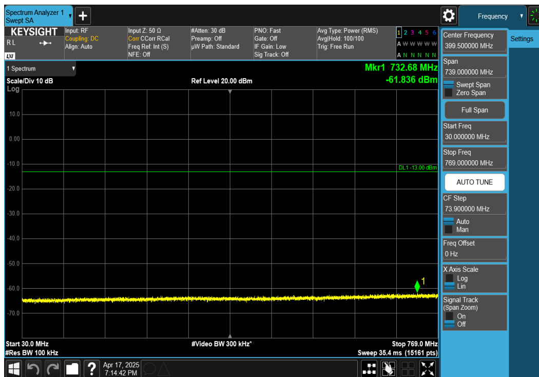
Plot 7-59. Conducted Spurious Plot (NR Band n14 - 10MHz DFT-s-OFDM QPSK - RB Size 1, RB Offset 25 - Mid Channel)
