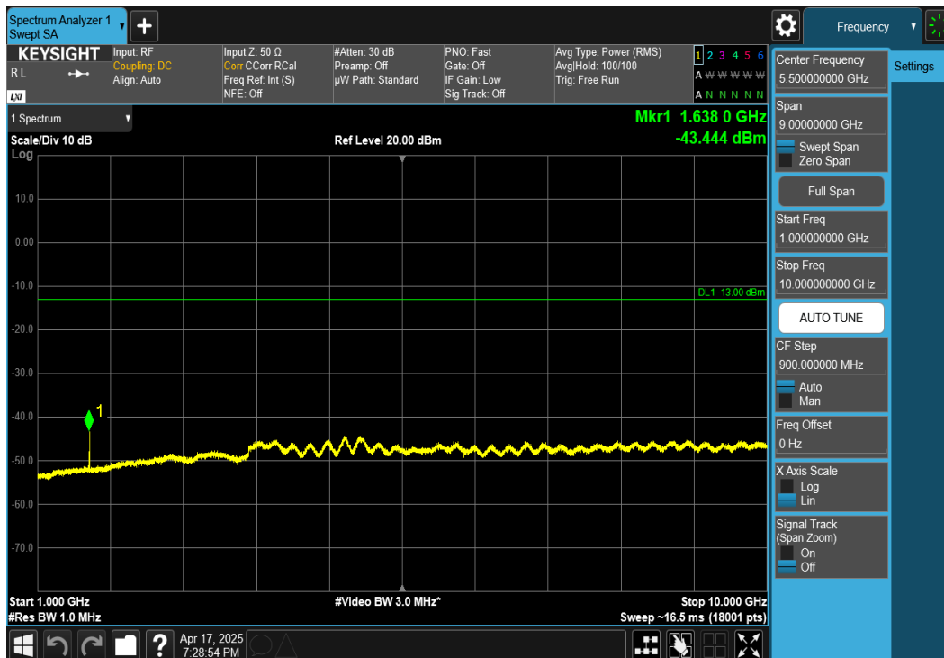
Plot 7-52. Conducted Spurious Plot (NR Band n26 - 10MHz DFT-s-OFDM QPSK - RB Size 1, RB Offset 25 – Mid Channel)
