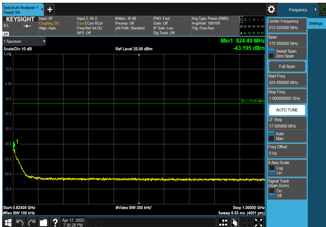
Plot 7-54. Conducted Spurious Plot (NR Band n26 - 5MHz DFT-s-OFDM QPSK - RB Size 1, RB Offset 12 - High Channel)
