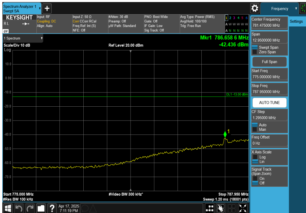
Plot 7-58. Conducted Spurious Plot (NR Band n14 - 5MHz DFT-s-OFDM QPSK - RB Size 1, RB Offset 12 - Low Channel)
