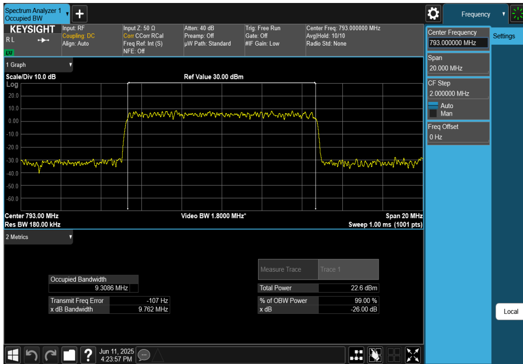
Plot 7-26. Occupied Bandwidth Plot (NR Band 14 - 10MHz CP-OFDM QPSK - Full RB Configuration)
