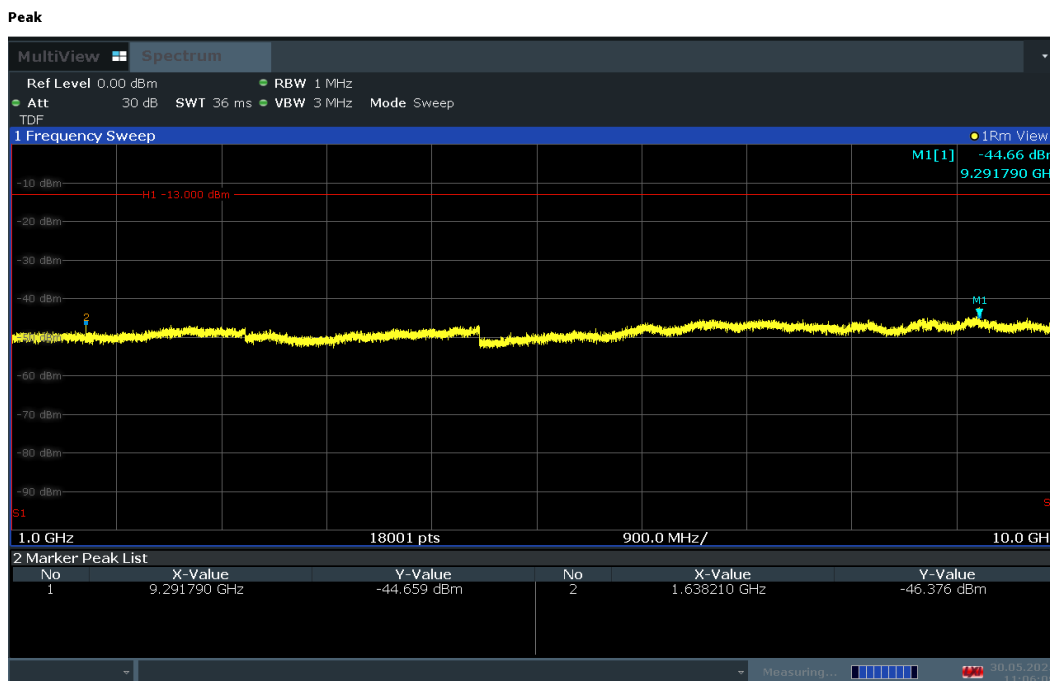
Plot 7-34. Conducted Spurious Plot (LTE Band 26 - 10MHz QPSK - RB Size 1, RB Offset 25 – Mid Channel)
