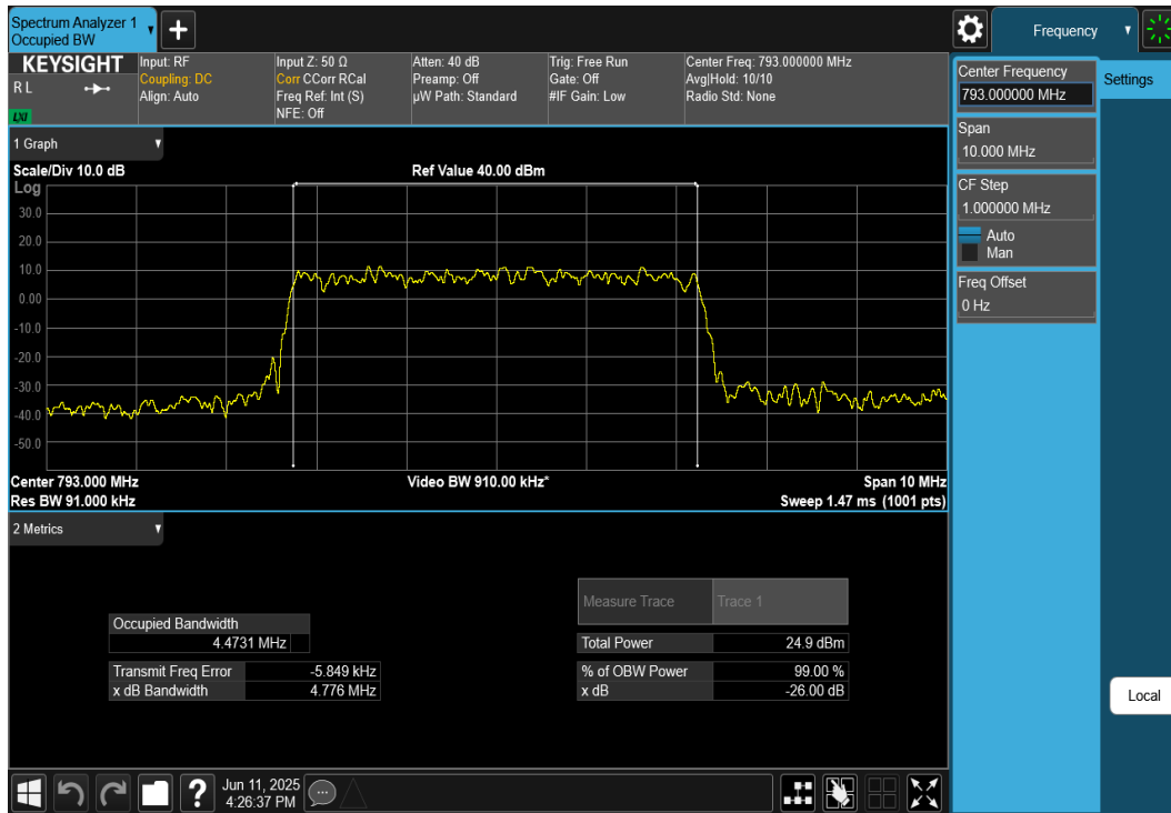
Plot 7-21. Occupied Bandwidth Plot (NR Band 14 - 5MHz DFT-s-OFDM \pi/2 BPSK - Full RB Configuration)
