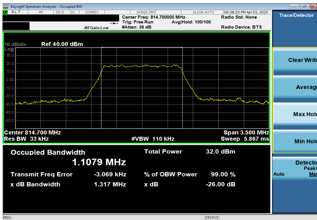
Plot 7-2. Occupied Bandwidth Plot (LTE Band 26 - 1.4MHz 16-QAM - Full RB Configuration)
