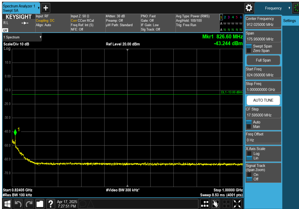
Plot 7-51. Conducted Spurious Plot (NR Band n26 - 10MHz DFT-s-OFDM QPSK - RB Size 1, RB Offset 25 – Mid Channel)
