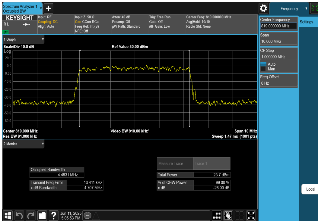
Plot 7-15. Occupied Bandwidth Plot (NR Band 26 - 5MHz DFT-s-OFDM 16-QAM - Full RB Configuration)
