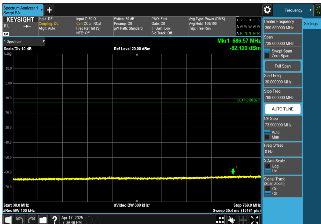
Plot 7-56. Conducted Spurious Plot (NR Band n14 - 5MHz DFT-s-OFDM QPSK - RB Size 1, RB Offset 12 - Low Channel)
