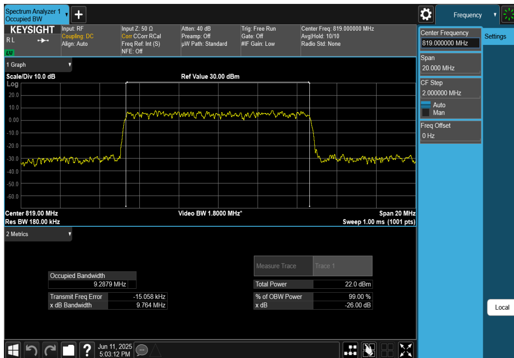
Plot 7-20. Occupied Bandwidth Plot (NR Band 26 - 10MHz CP-OFDM 64-QAM - Full RB Configuration)
