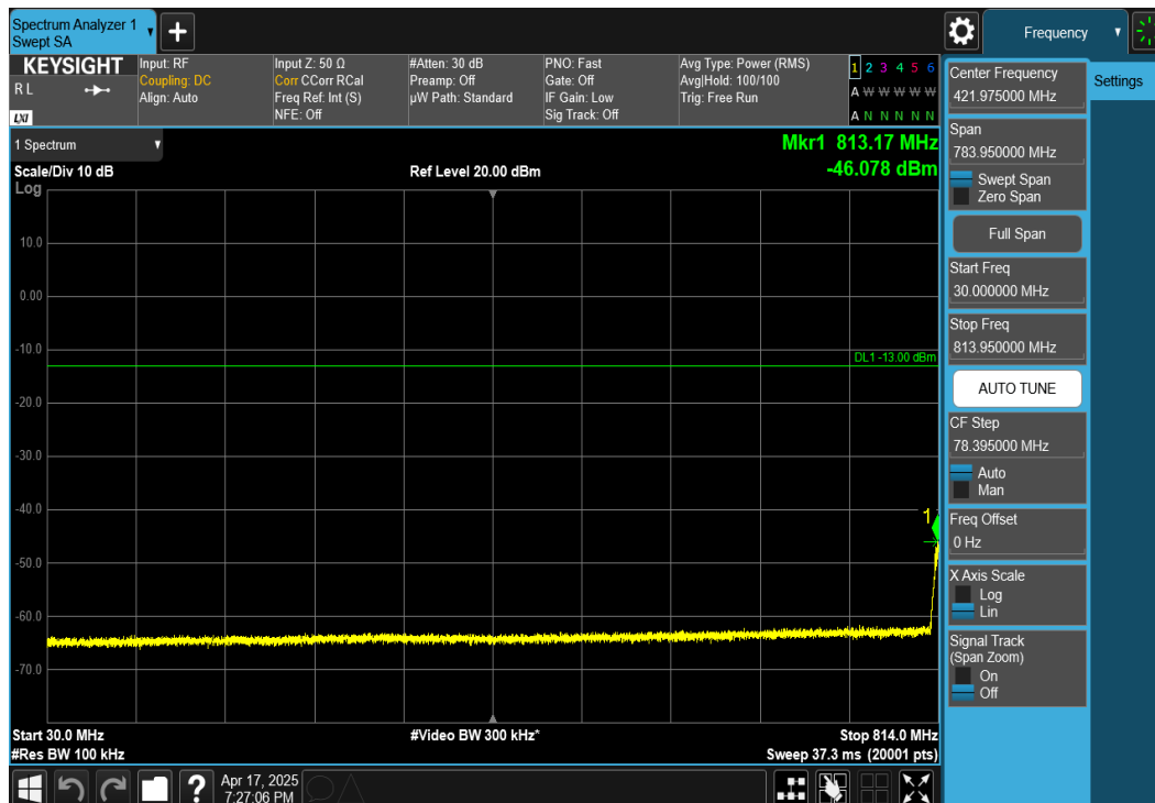
Plot 7-50. Conducted Spurious Plot (NR Band n26 - 10MHz DFT-s-OFDM QPSK - RB Size 1, RB Offset 25 - Mid Channel)
