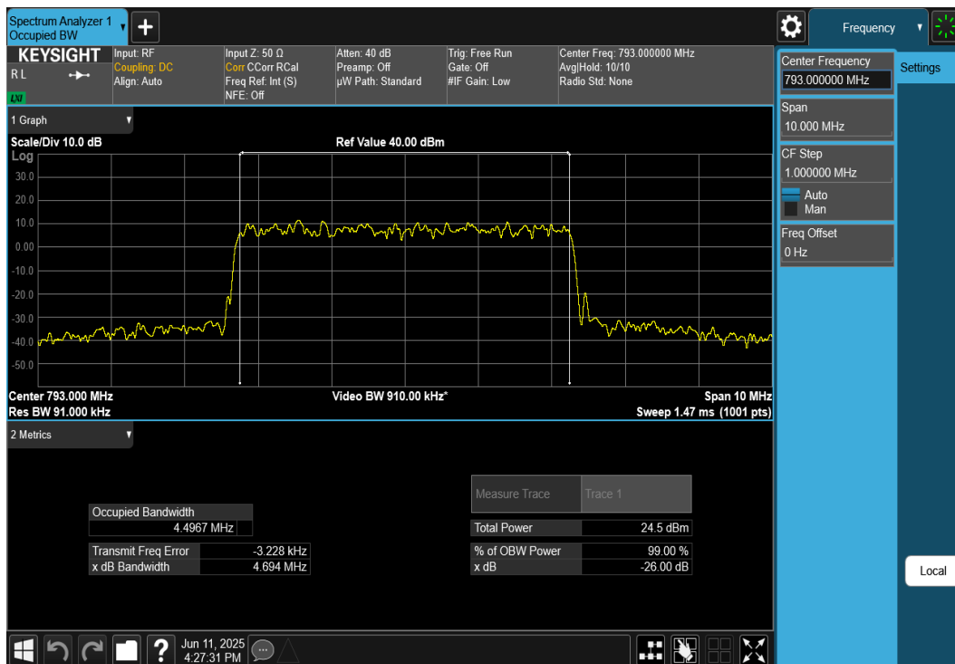
Plot 7-22. Occupied Bandwidth Plot (NR Band 14 - 5MHz DFT-s-OFDM QPSK - Full RB Configuration)
