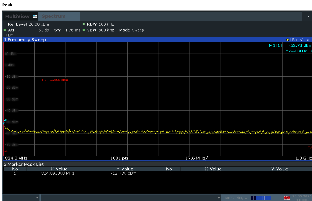
Plot 7-30. Conducted Spurious Plot (LTE Band 26 - 5MHz QPSK - RB Size 1, RB Offset 12 – Low Channel)
