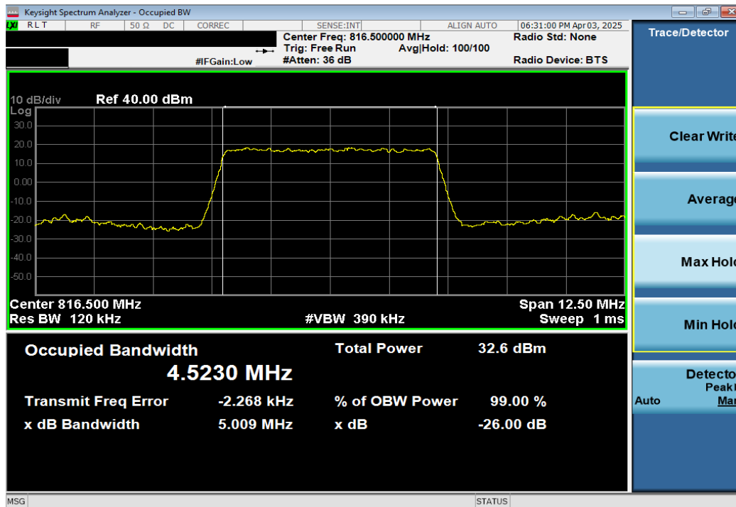
Plot 7-6. Occupied Bandwidth Plot (LTE Band 26 - 5MHz 16-QAM - Full RB Configuration)
