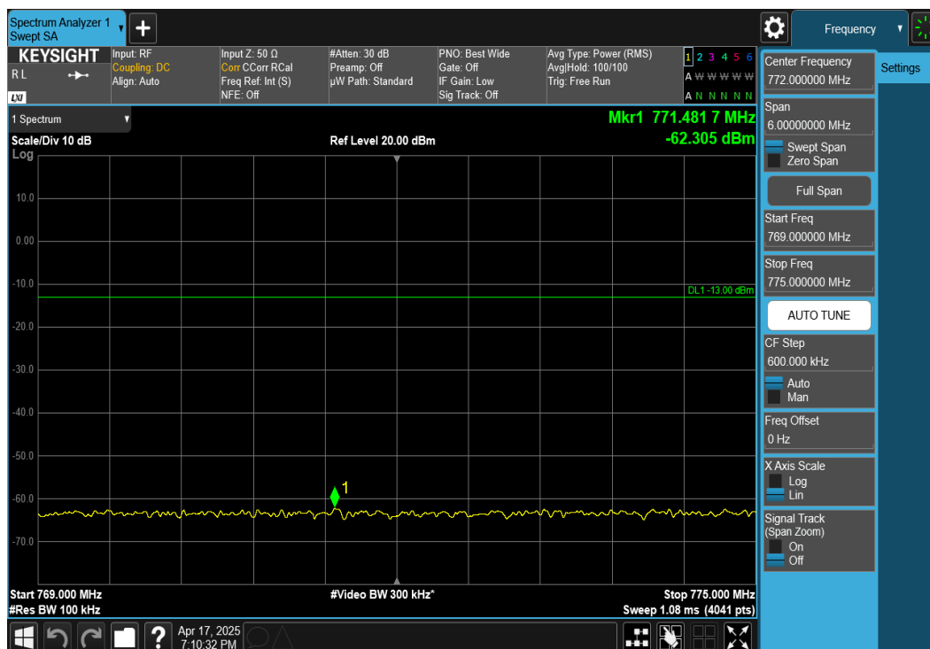
Plot 7-57. Conducted Spurious Plot (NR Band n14 - 5MHz DFT-s-OFDM QPSK - RB Size 1, RB Offset 12 - Low Channel)
