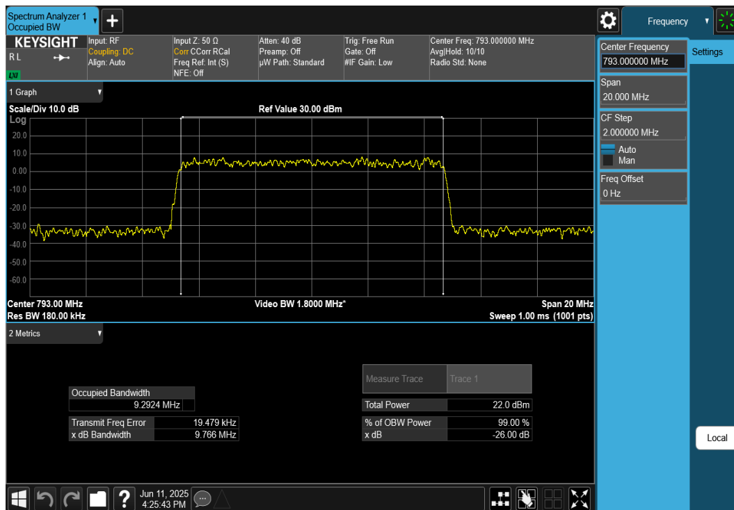
Plot 7-28. Occupied Bandwidth Plot (NR Band 14 - 10MHz CP-OFDM 64-QAM - Full RB Configuration)
