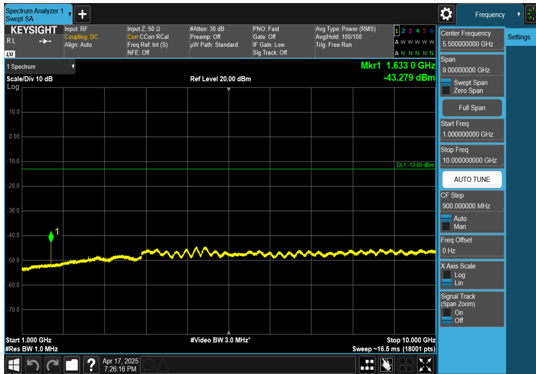
Plot 7-49. Conducted Spurious Plot (NR Band n26 - 5MHz DFT-s-OFDM QPSK - RB Size 1, RB Offset 12 - Low Channel)
