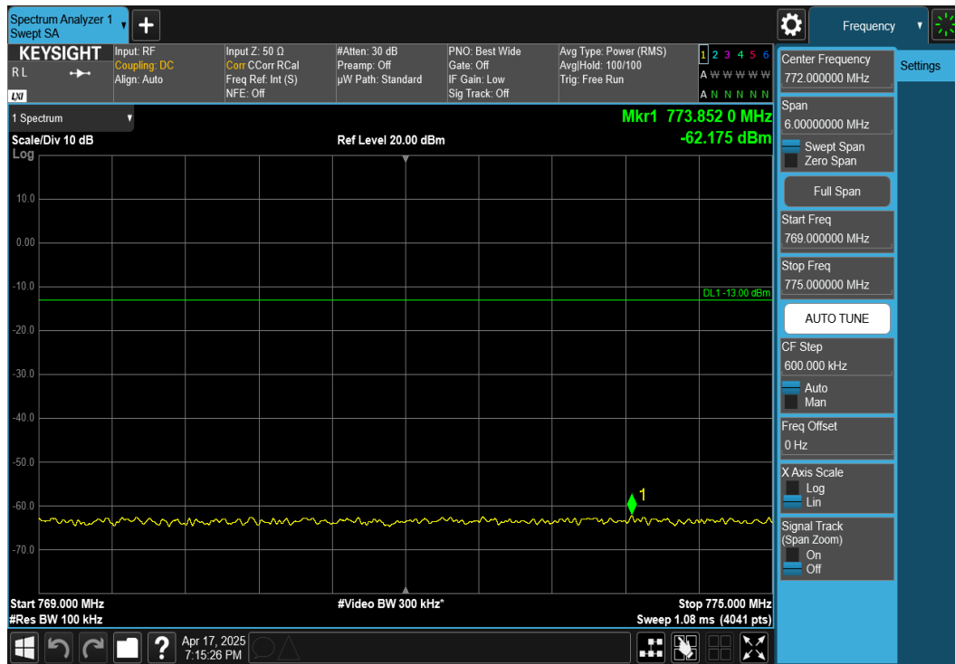
Plot 7-60. Conducted Spurious Plot (NR Band n14 - 10MHz DFT-s-OFDM QPSK - RB Size 1, RB Offset 25 - Mid Channel)
