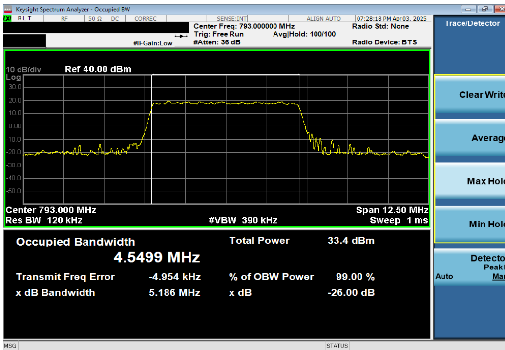
Plot 7-9. Occupied Bandwidth Plot (LTE Band 14 - 5MHz QPSK - Full RB Configuration)
