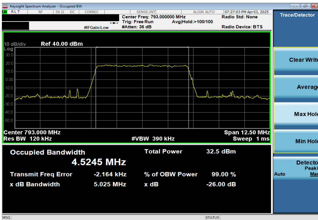
Plot 7-10. Occupied Bandwidth Plot (LTE Band 14 - 5MHz 16-QAM - Full RB Configuration)
