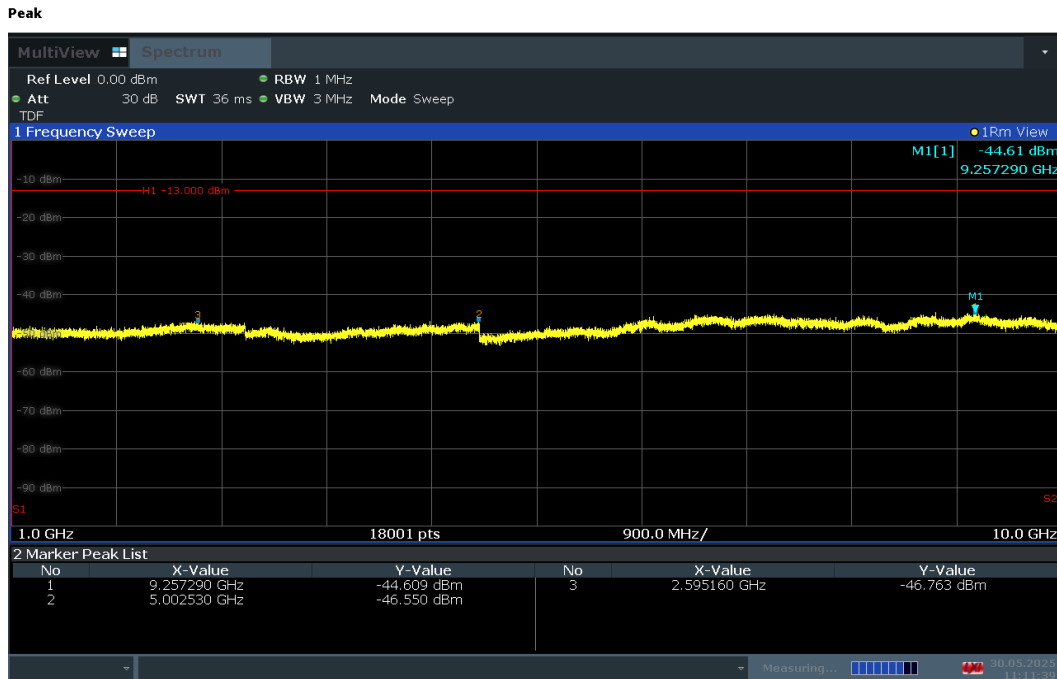
Plot 7-43. Conducted Spurious Plot (LTE Band 14 - 10MHz QPSK - RB Size 1, RB Offset 25 – Mid Channel)
