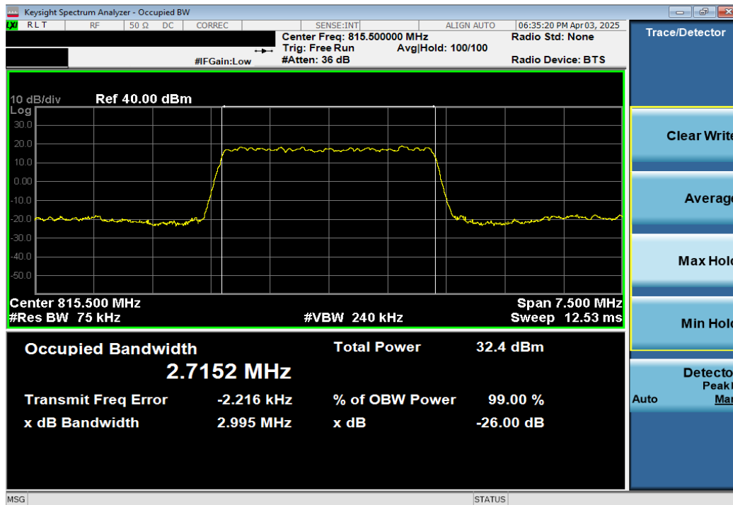
Plot 7-4. Occupied Bandwidth Plot (LTE Band 26 - 3MHz 16-QAM - Full RB Configuration)
