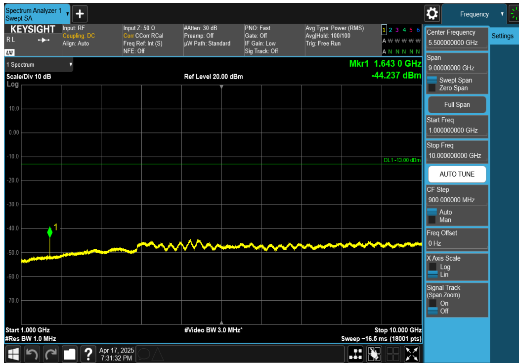
Plot 7-55. Conducted Spurious Plot (NR Band n26 - 5MHz DFT-s-OFDM QPSK - RB Size 1, RB Offset 12 - High Channel)
