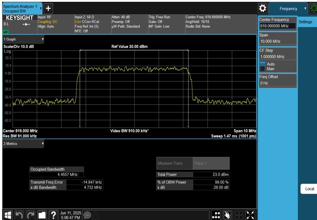
Plot 7-16. Occupied Bandwidth Plot (NR Band 26 - 5MHz DFT-s-OFDM 64-QAM - Full RB Configuration)
