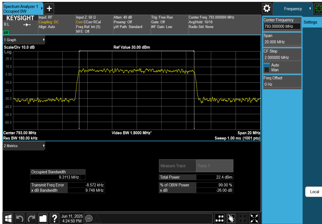
Plot 7-27. Occupied Bandwidth Plot (NR Band 14 - 10MHz CP-OFDM 16-QAM - Full RB Configuration)
