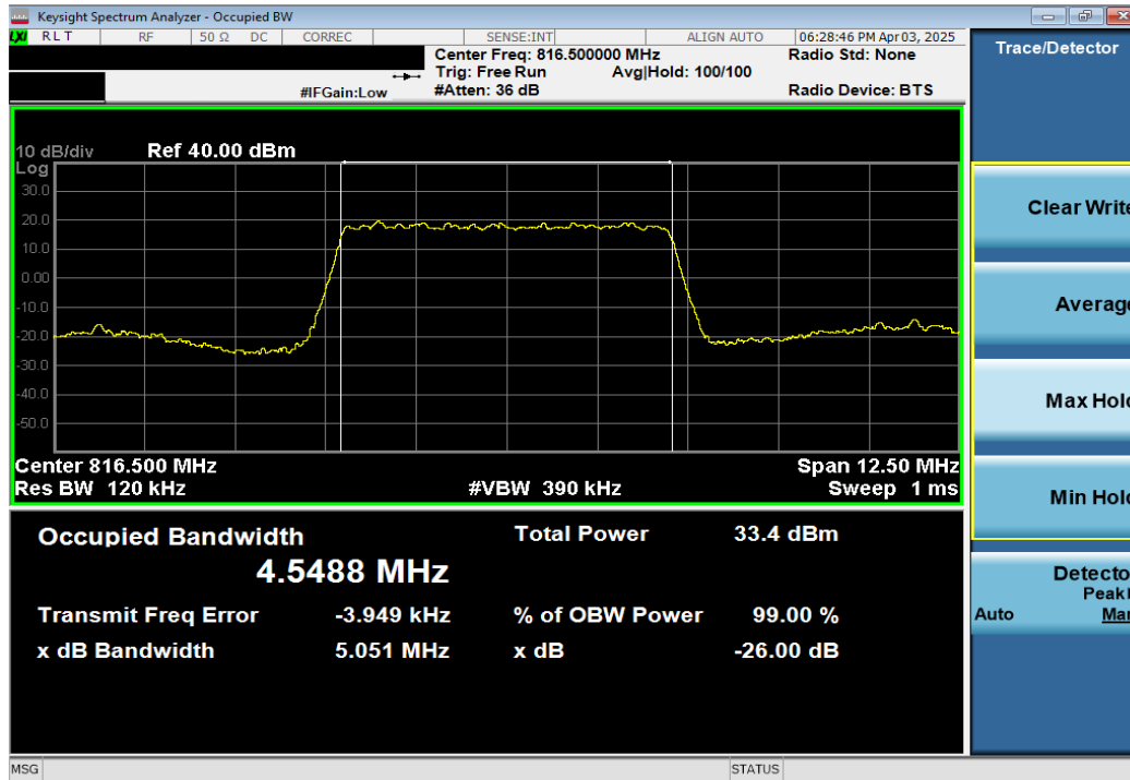
Plot 7-5. Occupied Bandwidth Plot (LTE Band 26 - 5MHz QPSK - Full RB Configuration)
