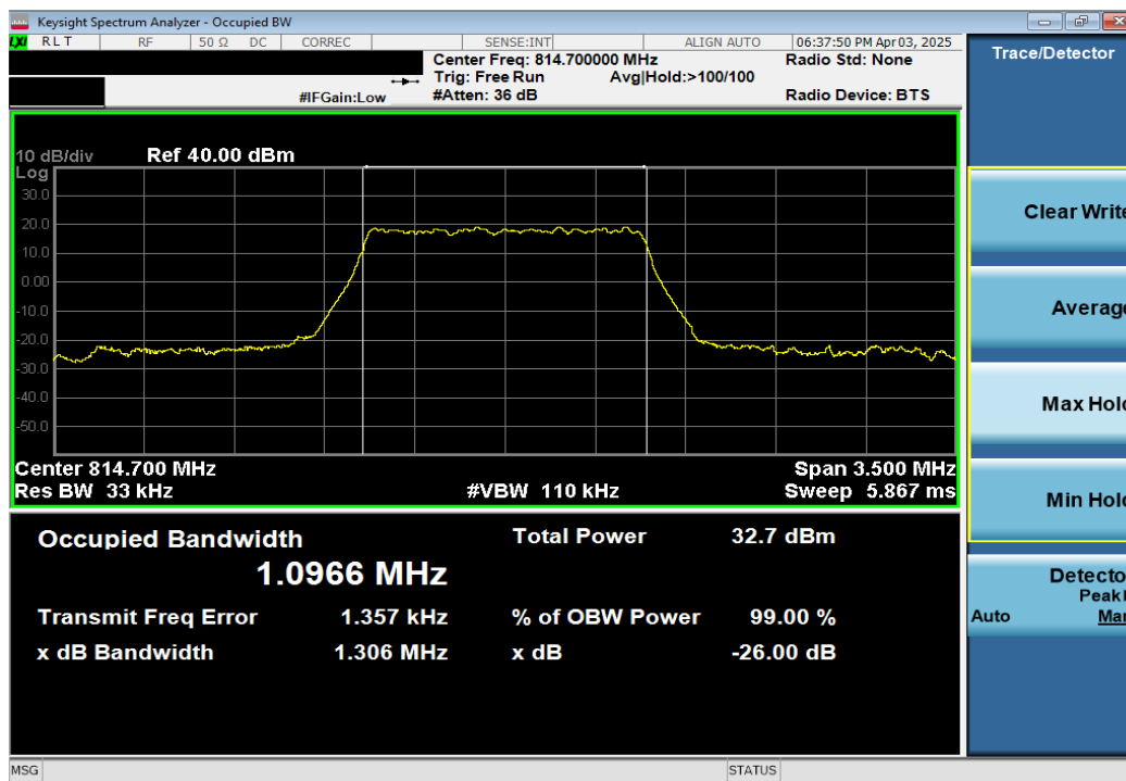
Plot 7-1. Occupied Bandwidth Plot (LTE Band 26 - 1.4MHz QPSK - Full RB Configuration)
