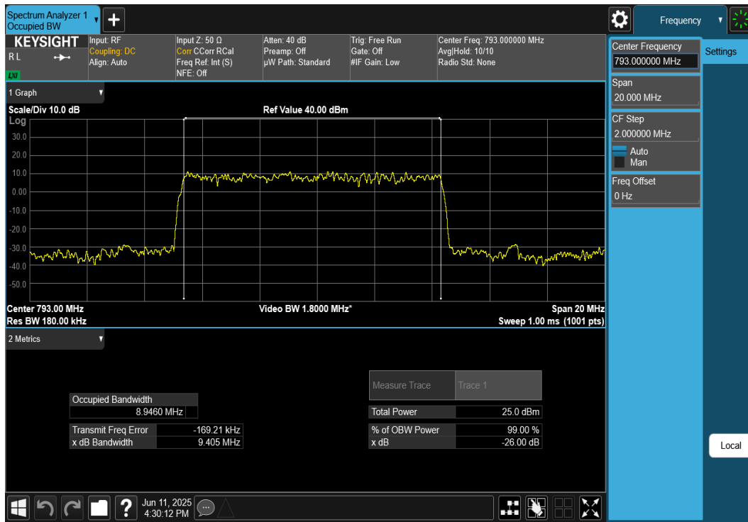
Plot 7-25. Occupied Bandwidth Plot (NR Band 14 - 10MHz DFT-s-OFDM \pi/2 BPSK - Full RB Configuration)
