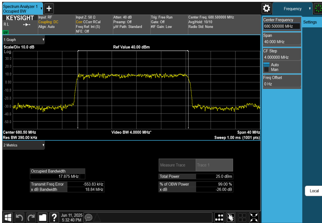
Plot 7-61. Occupied Bandwidth Plot (NR Band n71 - 20MHz DFT-s-OFDM \pi/2 BPSK - Full RB)
