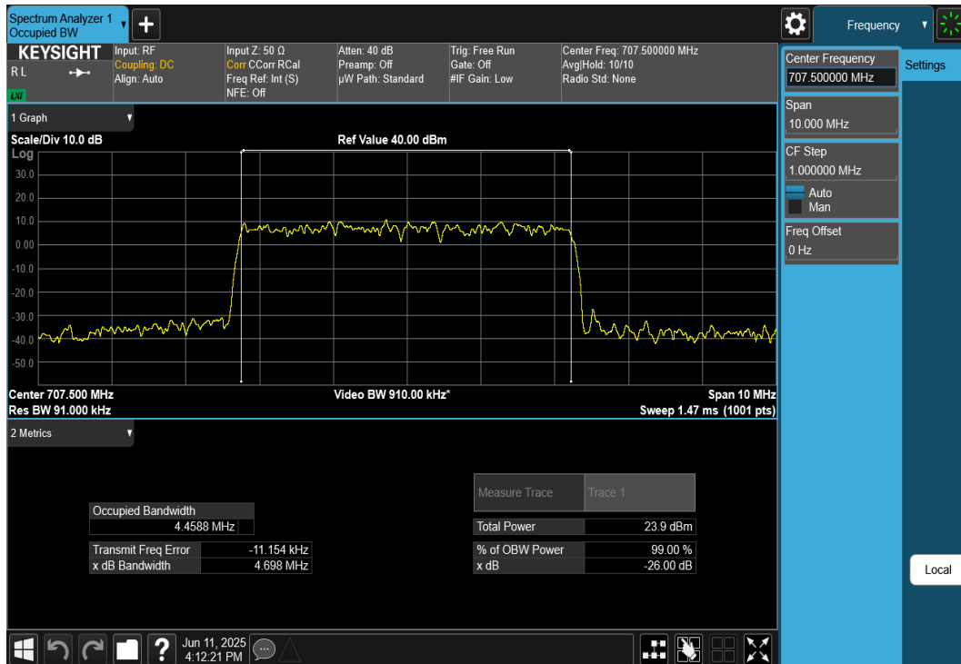
Plot 7-67. Occupied Bandwidth Plot (NR Band n12 - 5MHz DFT-s-OFDM 16-QAM - Full RB)
