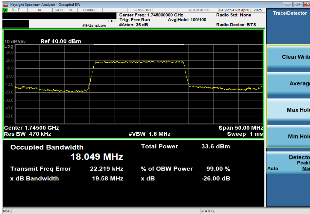
Plot 7-11. Occupied Bandwidth Plot (LTE Band 66/4 - 20MHz QPSK - Full RB)
