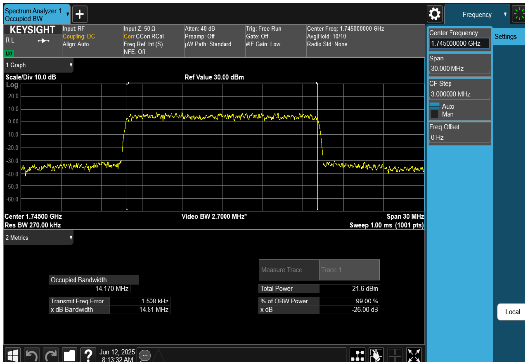
Plot 7-44. Occupied Bandwidth Plot (NR Band n66 - 15MHz CP-OFDM 64QAM - Full RB)
