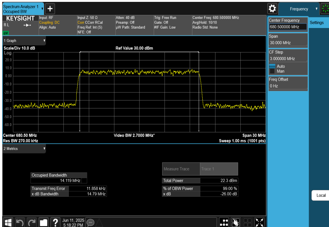
Plot 7-60. Occupied Bandwidth Plot (NR Band n71 - 15MHz CP-OFDM 64-QAM - Full RB)
