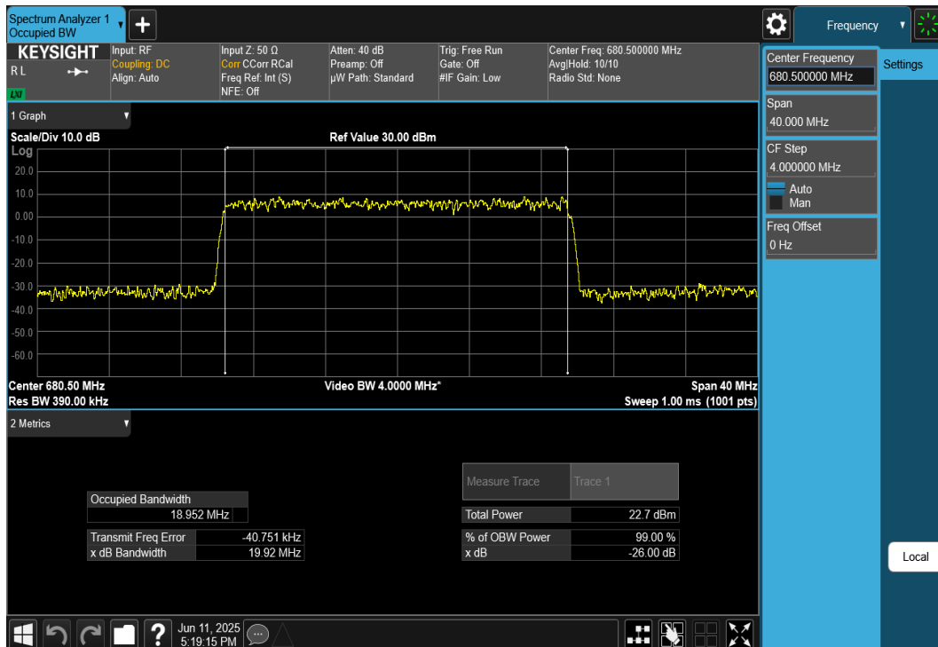
Plot 7-62. Occupied Bandwidth Plot (NR Band n71 - 20MHz CP-OFDM QPSK - Full RB)
