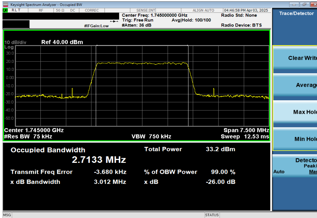
Plot 7-3. Occupied Bandwidth Plot (LTE Band 66/4 - 3MHz QPSK - Full RB)
