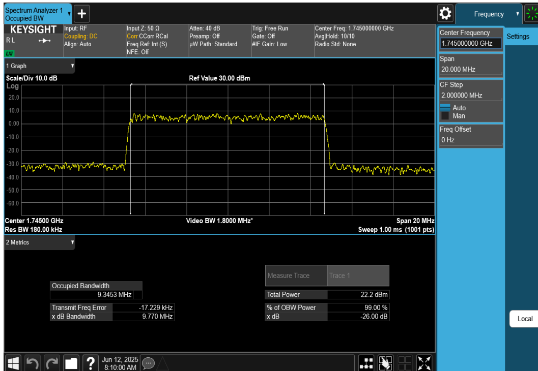
Plot 7-39. Occupied Bandwidth Plot (NR Band n66 - 10MHz CP-OFDM 16QAM - Full RB)
