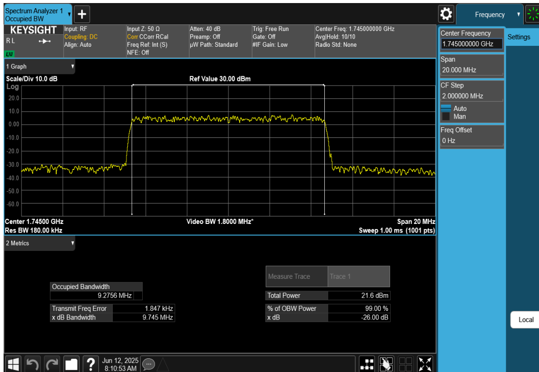
Plot 7-40. Occupied Bandwidth Plot (NR Band n66 - 10MHz CP-OFDM 64QAM - Full RB)
