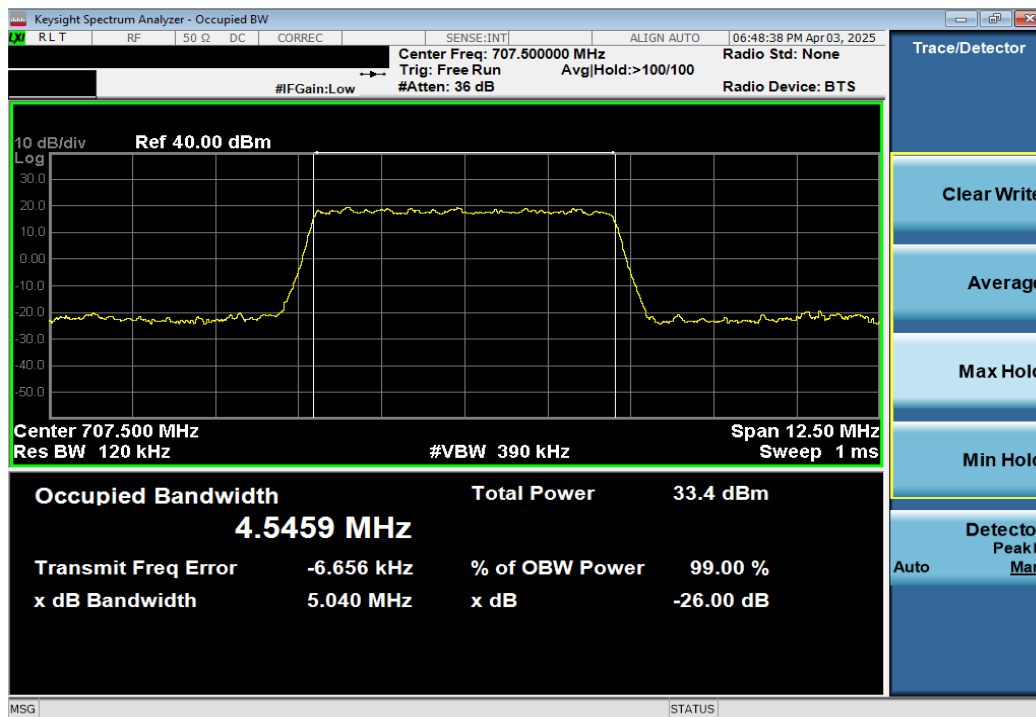
Plot 7-25. Occupied Bandwidth Plot (LTE Band 12/17 - 5MHz QPSK - Full RB)
