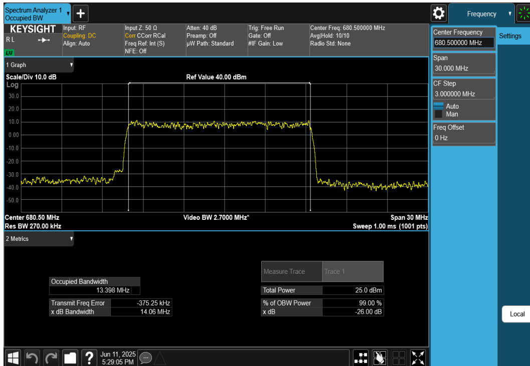
Plot 7-57. Occupied Bandwidth Plot (NR Band n71 - 15MHz DFT-s-OFDM \pi/2 BPSK - Full RB)
