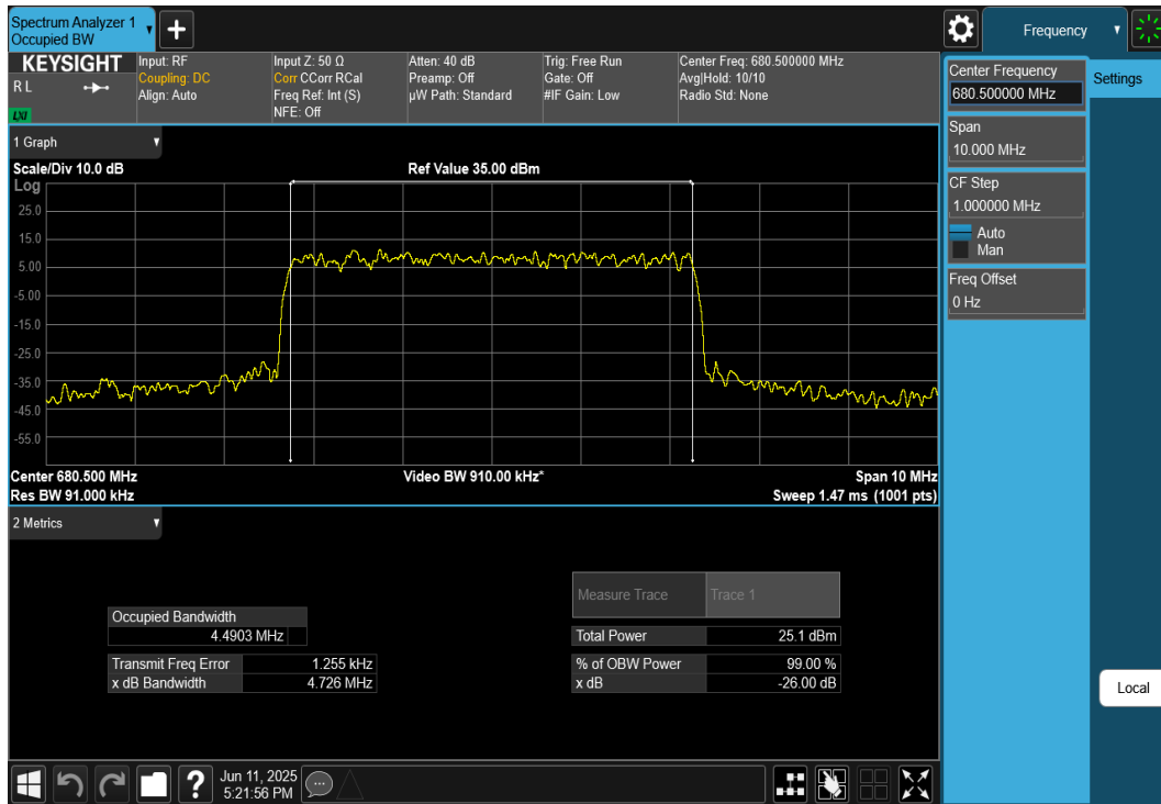
Plot 7-49. Occupied Bandwidth Plot (NR Band n71 - 5MHz DFT-s-OFDM \pi/2 BPSK - Full RB)
