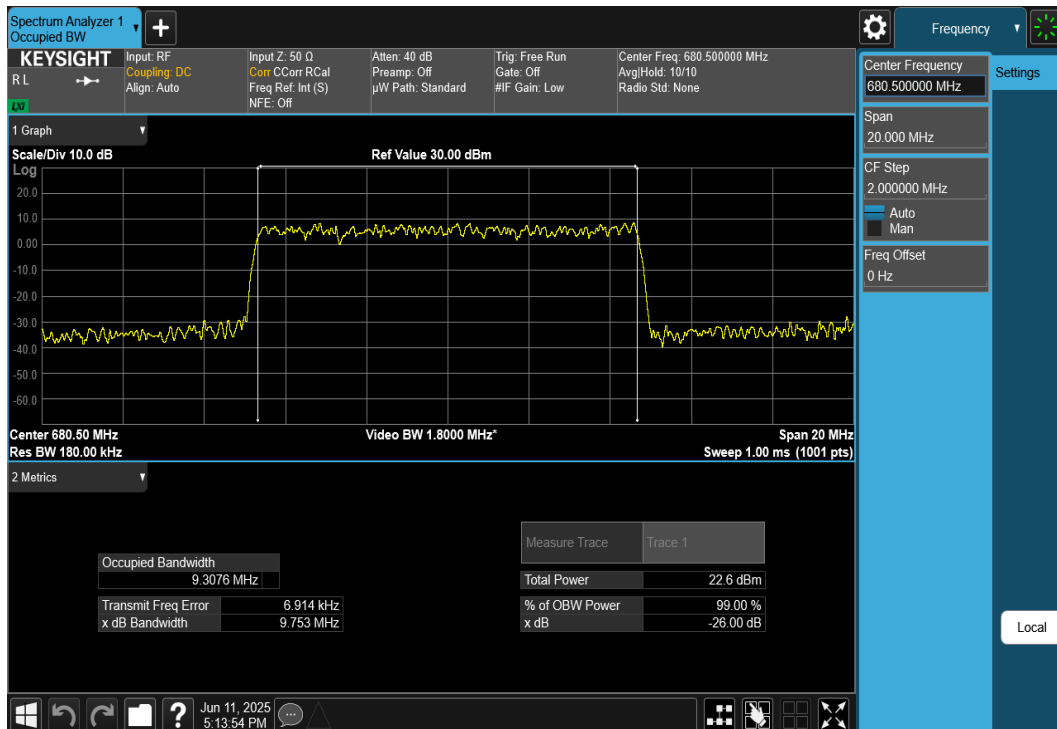
Plot 7-54. Occupied Bandwidth Plot (NR Band n71 - 10MHz CP-OFDM QPSK - Full RB)
