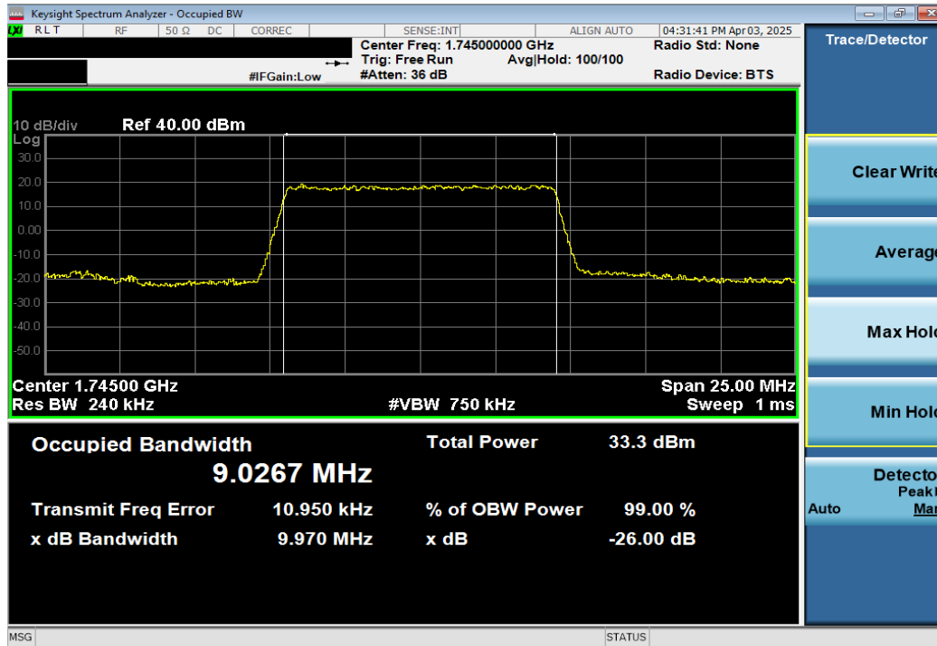
Plot 7-7. Occupied Bandwidth Plot (LTE Band 66/4 - 10MHz QPSK - Full RB)
