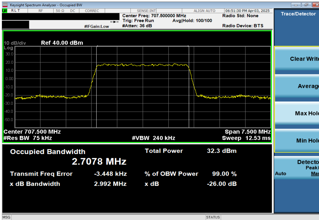
Plot 7-24. Occupied Bandwidth Plot (LTE Band 12 - 3MHz 16-QAM - Full RB)
