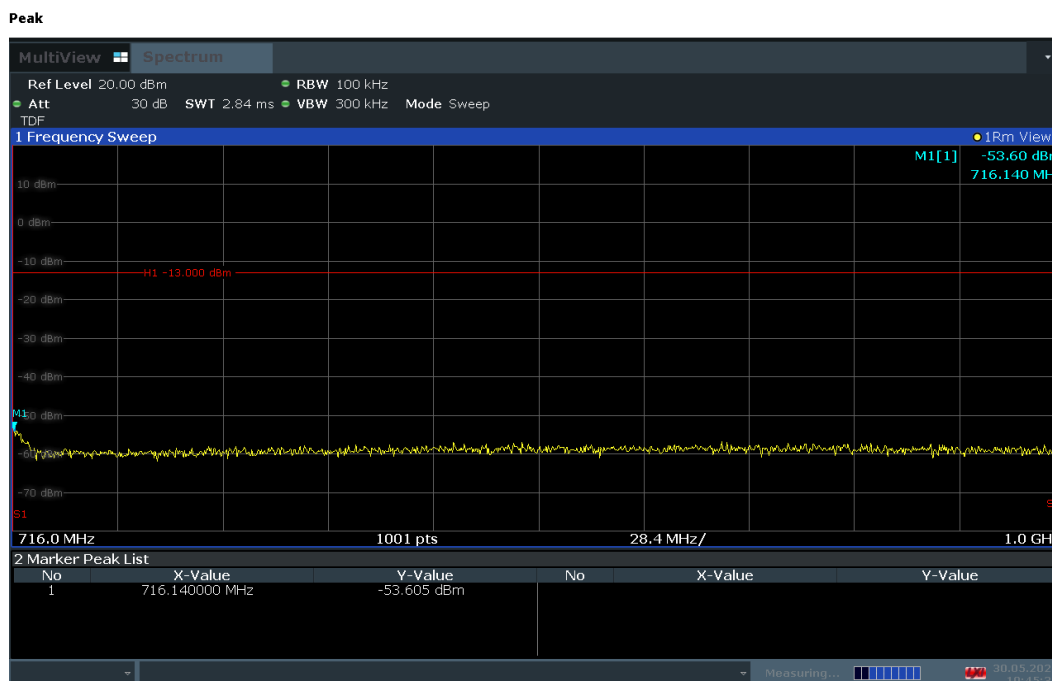
Plot 7-96. Conducted Spurious Plot (LTE Band 12/17 - 10MHz QPSK - RB Size 1, RB Offset 25 - Low Channel)
