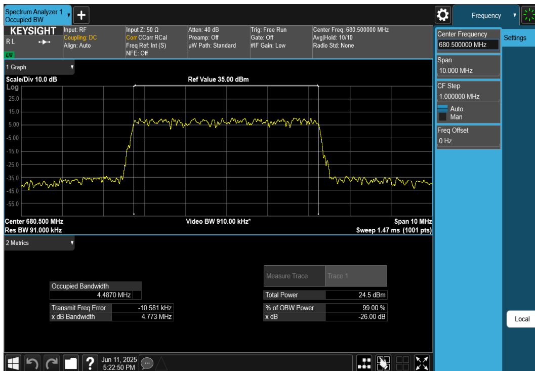
Plot 7-50. Occupied Bandwidth Plot (NR Band n71 - 5MHz DFT-s-OFDM QPSK - Full RB)
