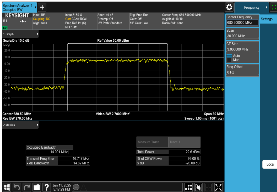
Plot 7-59. Occupied Bandwidth Plot (NR Band n71 - 15MHz CP-OFDM 16-QAM - Full RB)
