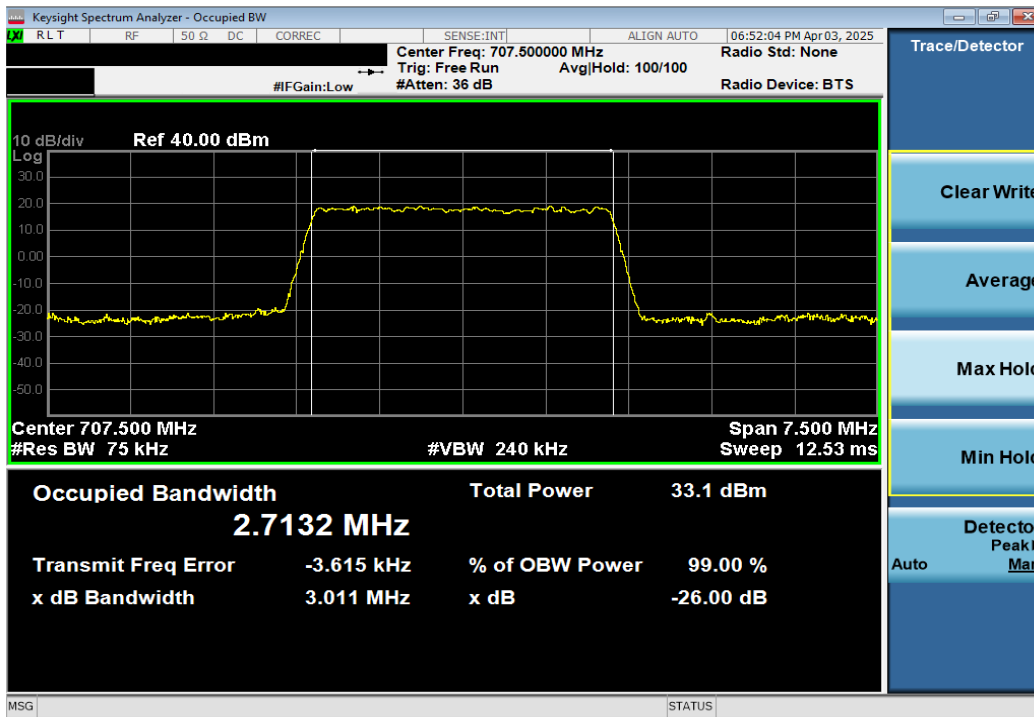
Plot 7-23. Occupied Bandwidth Plot (LTE Band 12 - 3MHz QPSK - Full RB)
