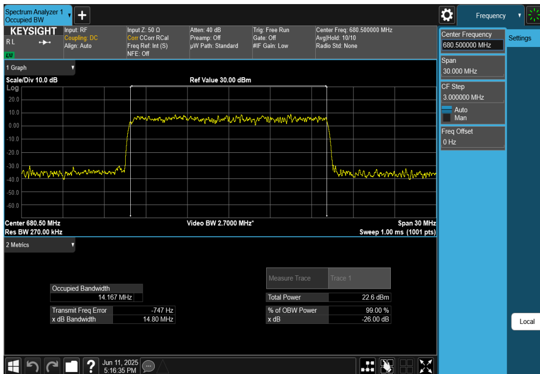
Plot 7-58. Occupied Bandwidth Plot (NR Band n71 - 15MHz CP-OFDM QPSK - Full RB)
