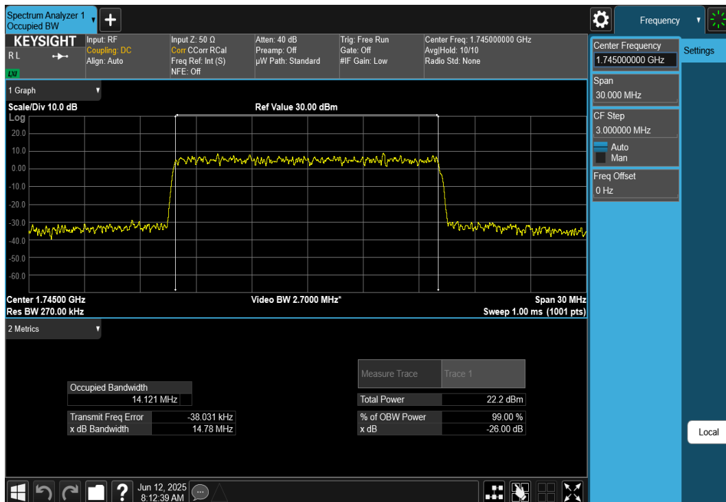
Plot 7-43. Occupied Bandwidth Plot (NR Band n66 - 15MHz CP-OFDM 16QAM - Full RB)
