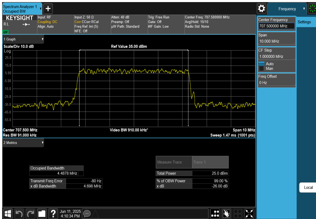
Plot 7-65. Occupied Bandwidth Plot (NR Band n12 - 5MHz DFT-s-OFDM \pi/2 BPSK - Full RB)
