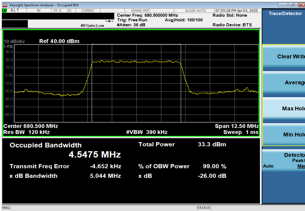
Plot 7-13. Occupied Bandwidth Plot (LTE Band 71 - 5MHz QPSK - Full RB)
