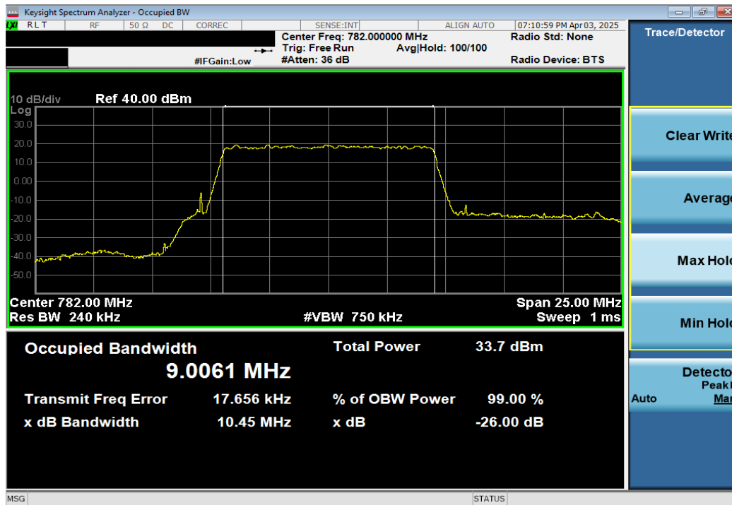
Plot 7-31. Occupied Bandwidth Plot (LTE Band 13 - 10MHz QPSK - Full RB)
