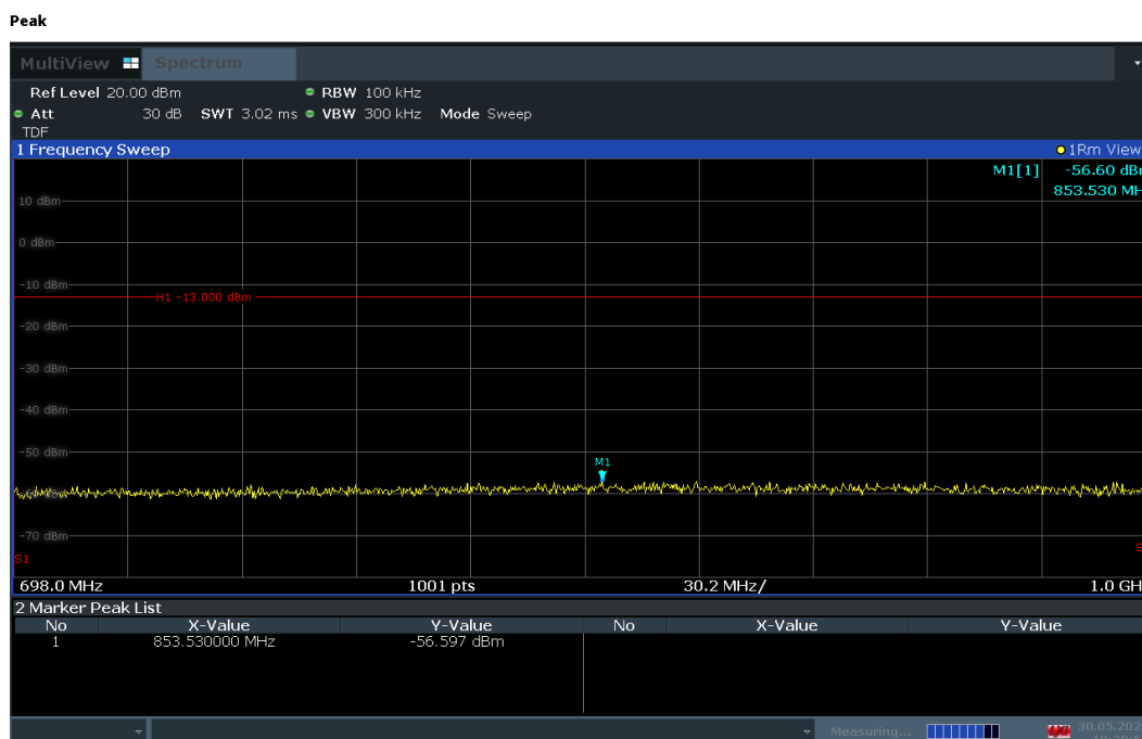
Plot 7-87. Conducted Spurious Plot (LTE Band 71 - 20MHz QPSK - RB Size 1, RB Offset 50 - Low Channel)
