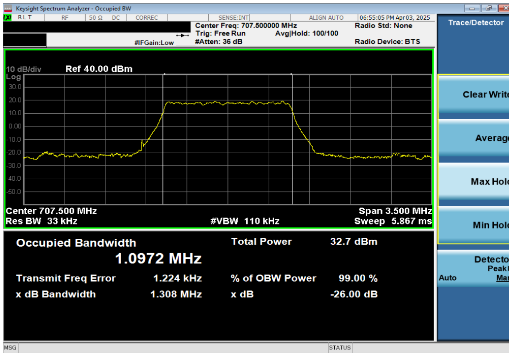
Plot 7-21. Occupied Bandwidth Plot (LTE Band 12 – 1.4MHz QPSK - Full RB)
