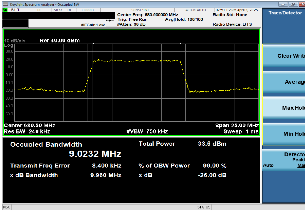
Plot 7-15. Occupied Bandwidth Plot (LTE Band 71 - 10MHz QPSK - Full RB)
