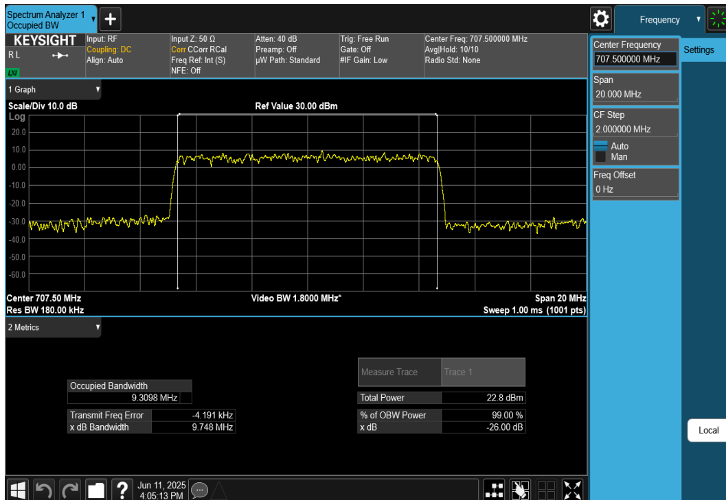
Plot 7-70. Occupied Bandwidth Plot (NR Band n12 - 10MHz CP-OFDM QPSK - Full RB)
