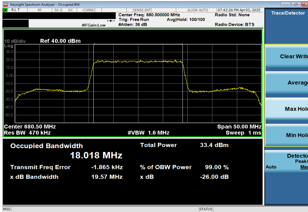
Plot 7-19. Occupied Bandwidth Plot (LTE Band 71 - 20MHz QPSK - Full RB)
