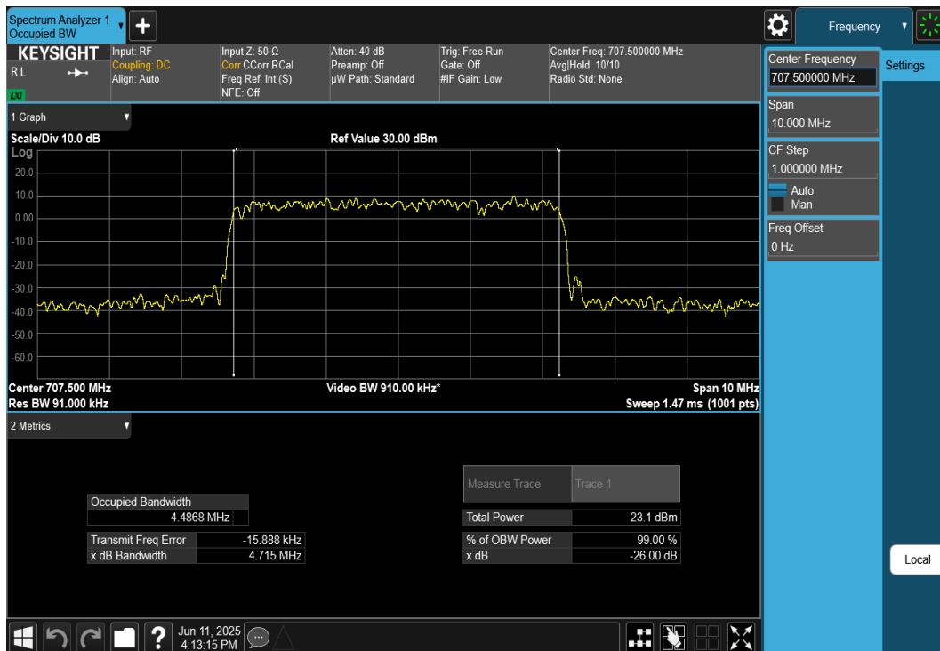
Plot 7-68. Occupied Bandwidth Plot (NR Band n12 - 5MHz DFT-s-OFDM 64-QAM - Full RB)
