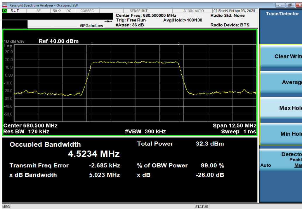
Plot 7-14. Occupied Bandwidth Plot (LTE Band 71 - 5MHz 16-QAM - Full RB)
