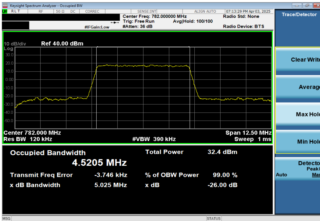
Plot 7-30. Occupied Bandwidth Plot (LTE Band 13 - 5MHz 16-QAM - Full RB)
