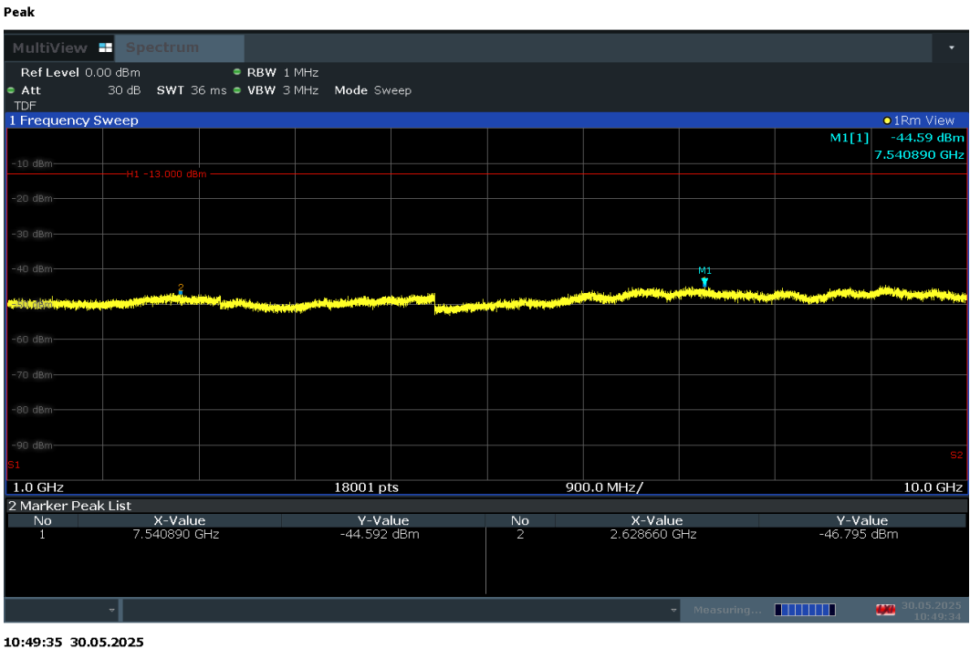
Plot 7-103. Conducted Spurious Plot (LTE Band 12/17 - 10MHz QPSK - RB Size 1, RB Offset 25 - High Channel)
