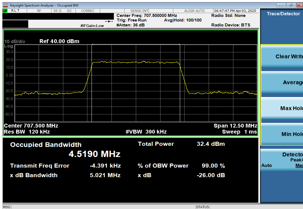
Plot 7-26. Occupied Bandwidth Plot (LTE Band 12/17 - 5MHz 16-QAM - Full RB)
