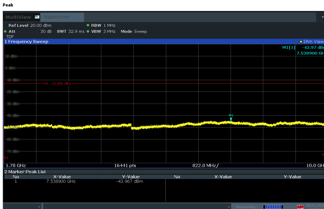
Plot 7-78. Conducted Spurious Plot (LTE Band 66/4 - 20MHz QPSK - RB Size 1, RB Offset 50 - Low Channel)
