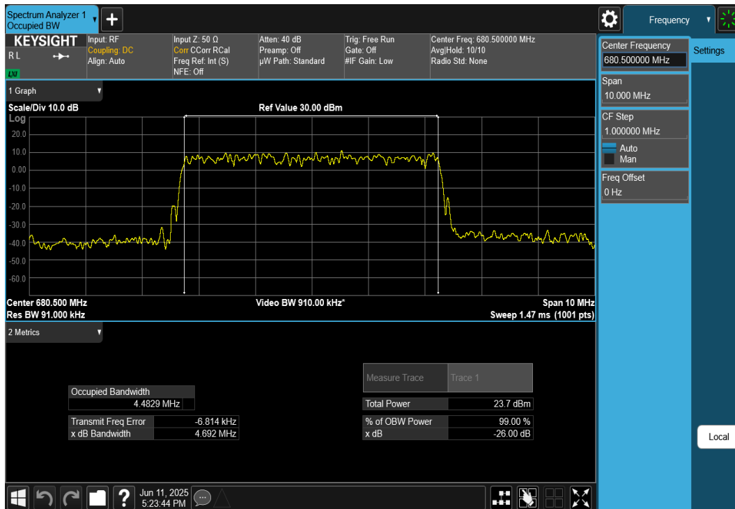
Plot 7-51. Occupied Bandwidth Plot (NR Band n71 - 5MHz DFT-s-OFDM 16-QAM - Full RB)
