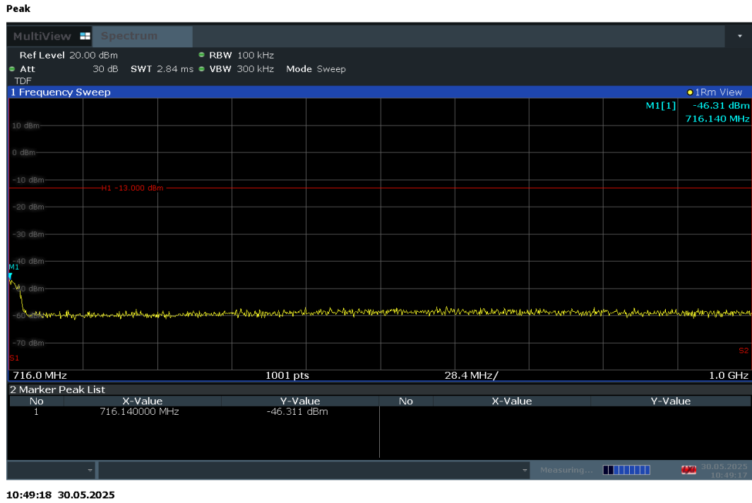
Plot 7-102. Conducted Spurious Plot (LTE Band 12/17 - 10MHz QPSK - RB Size 1, RB Offset 25 - High Channel)
