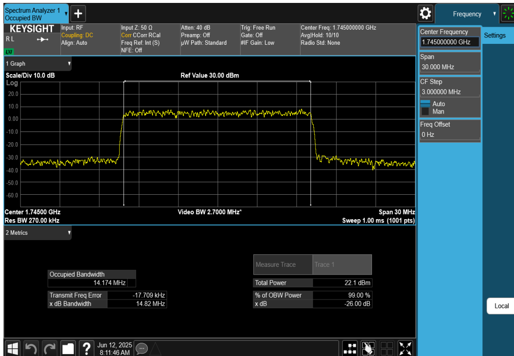
Plot 7-42. Occupied Bandwidth Plot (NR Band n66 - 15MHz CP-OFDM QPSK - Full RB)
