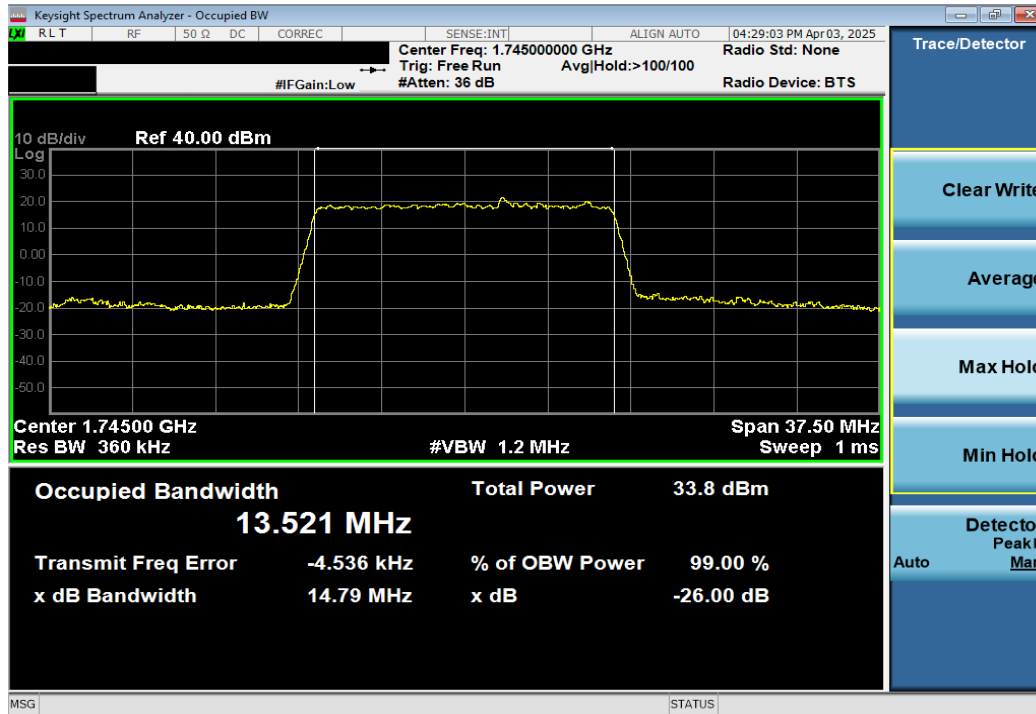
Plot 7-9. Occupied Bandwidth Plot (LTE Band 66/4 - 15MHz QPSK - Full RB)
