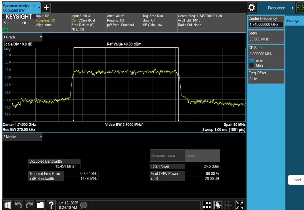
Plot 7-41. Occupied Bandwidth Plot (NR Band n66 - 15MHz DFT-s-OFDM \pi/2 BPSK - Full RB)
