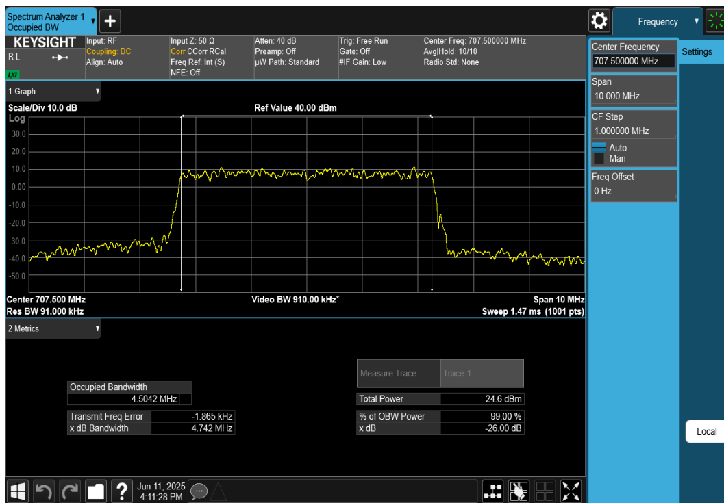
Plot 7-66. Occupied Bandwidth Plot (NR Band n12 - 5MHz DFT-s-OFDM QPSK - Full RB)
