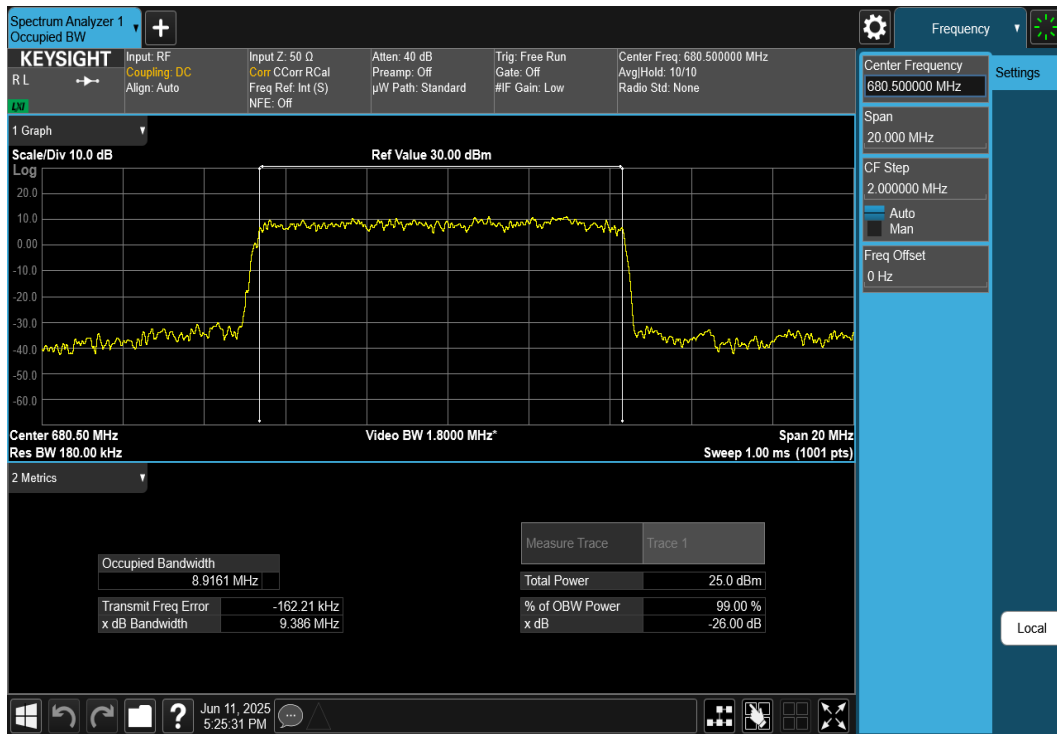
Plot 7-53. Occupied Bandwidth Plot (NR Band n71 - 10MHz DFT-s-OFDM \pi/2 BPSK - Full RB)
