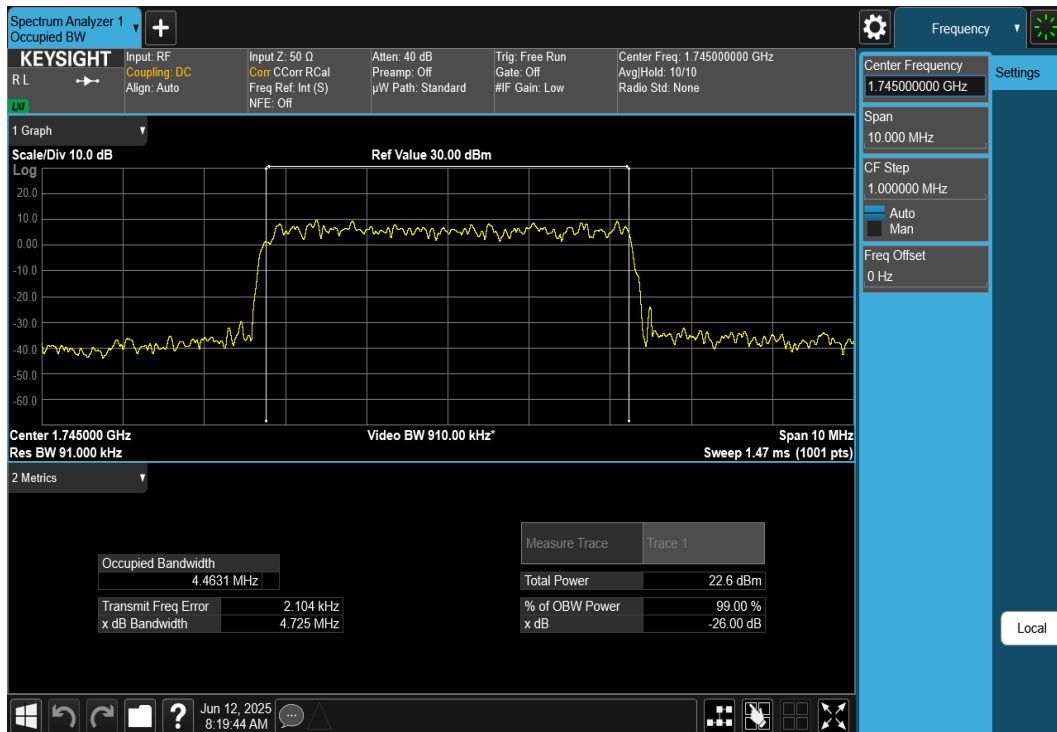
Plot 7-36. Occupied Bandwidth Plot (NR Band n66 - 5MHz DFT-s-OFDM 64QAM - Full RB)
