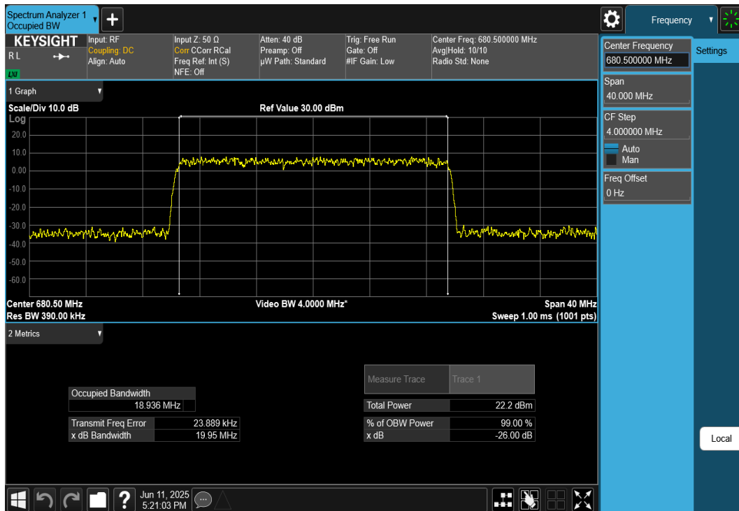
Plot 7-64. Occupied Bandwidth Plot (NR Band n71 - 20MHz CP-OFDM 64-QAM - Full RB)
