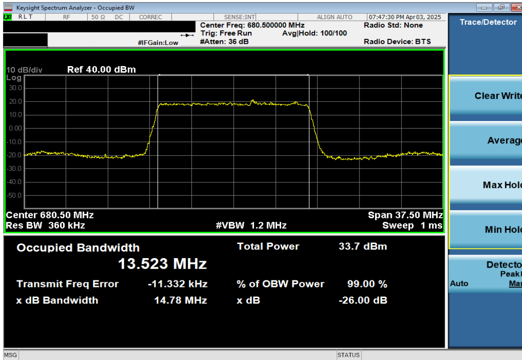
Plot 7-17. Occupied Bandwidth Plot (LTE Band 71 - 15MHz QPSK - Full RB)
