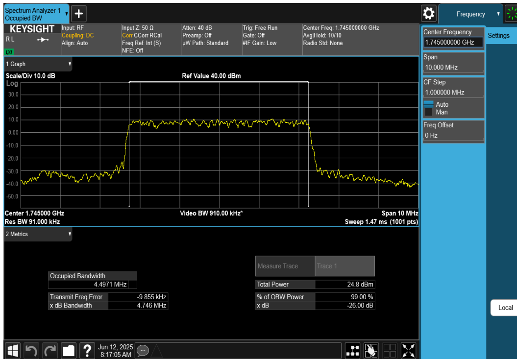
Plot 7-33. Occupied Bandwidth Plot (NR Band n66 - 5MHz DFT-s-OFDM \pi/2 BPSK - Full RB)
