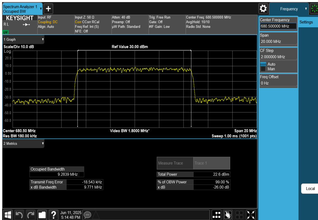
Plot 7-55. Occupied Bandwidth Plot (NR Band n71 - 10MHz CP-OFDM 16-QAM - Full RB)
