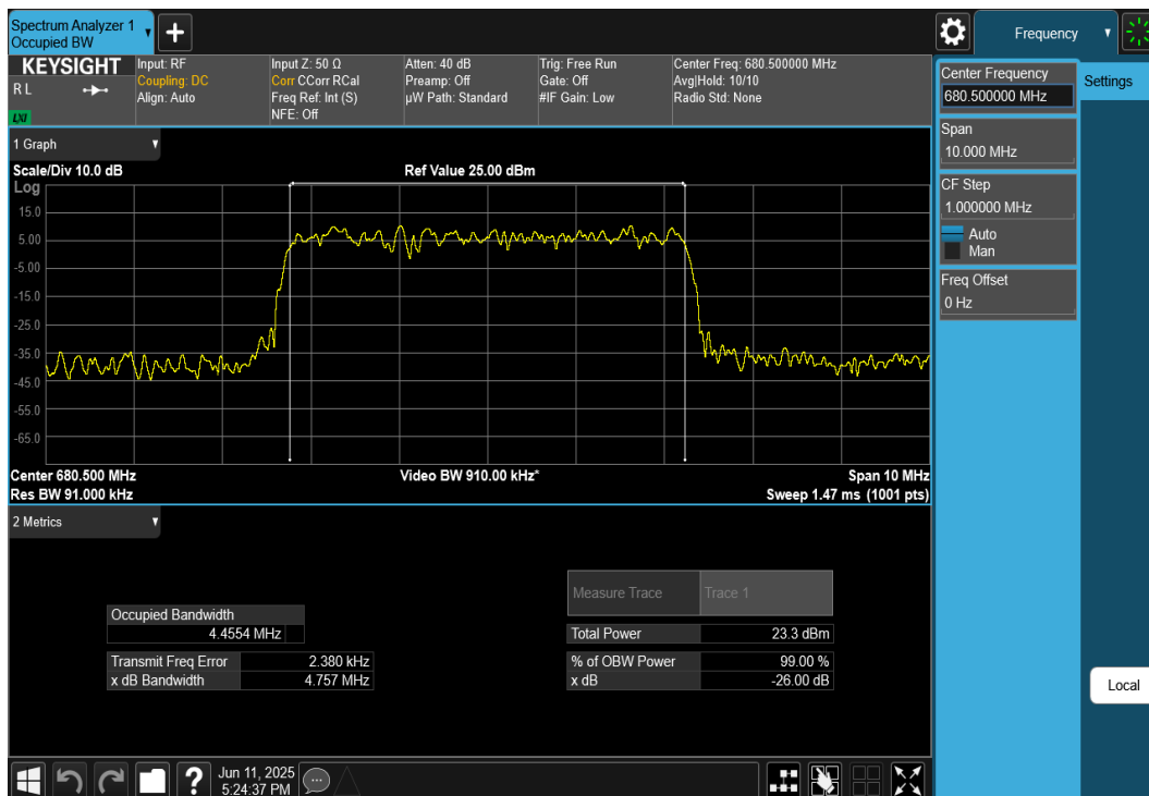
Plot 7-52. Occupied Bandwidth Plot (NR Band n71 - 5MHz DFT-s-OFDM 64-QAM - Full RB)
