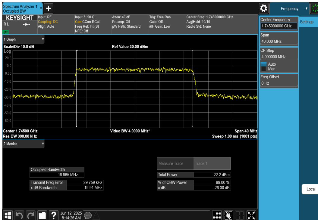
Plot 7-46. Occupied Bandwidth Plot (NR Band n66 - 20MHz CP-OFDM QPSK - Full RB)
