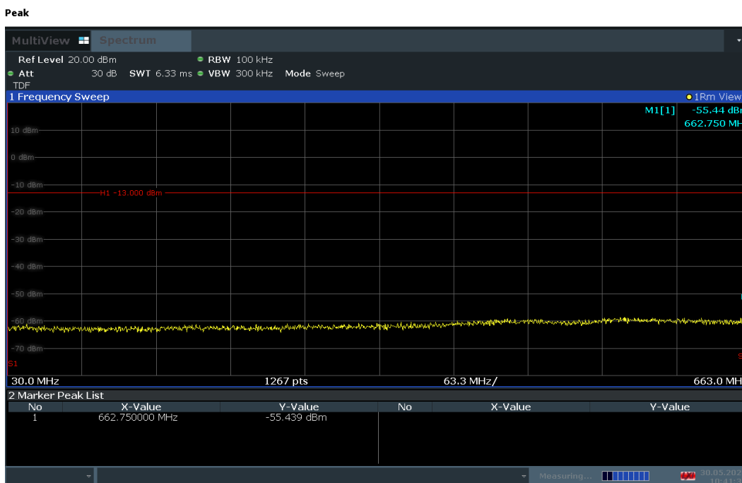
Plot 7-89. Conducted Spurious Plot (LTE Band 71 - 20MHz QPSK - RB Size 1, RB Offset 50 - Mid Channel)
