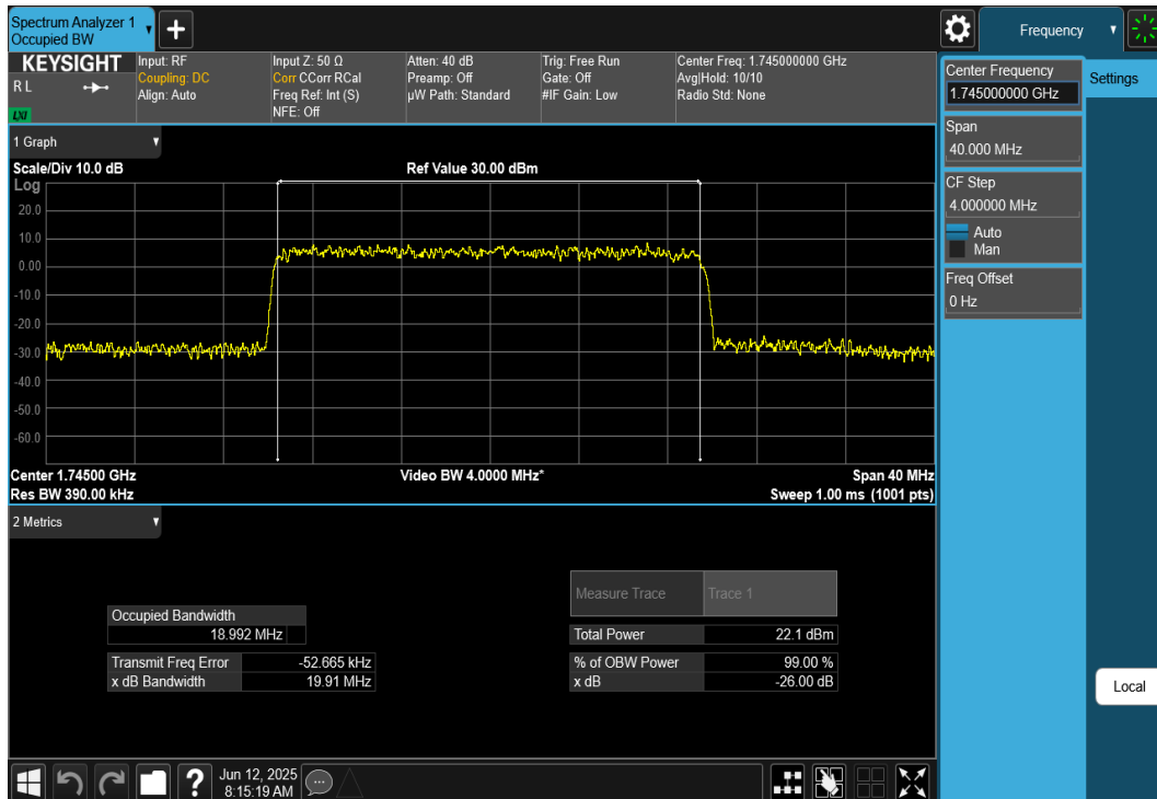
Plot 7-47. Occupied Bandwidth Plot (NR Band n66 - 20MHz CP-OFDM 16QAM - Full RB)
