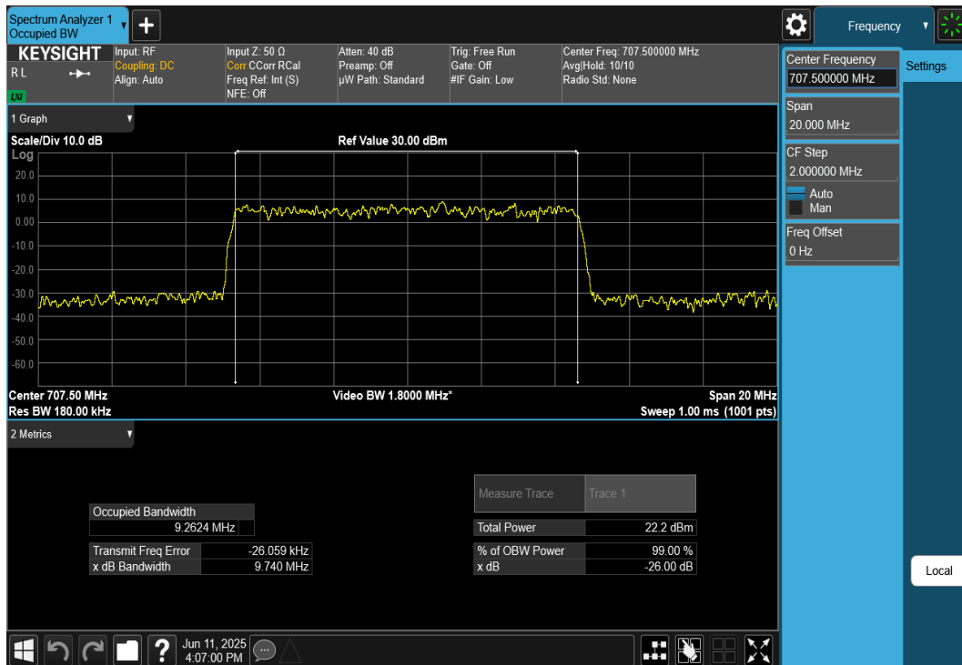
Plot 7-72. Occupied Bandwidth Plot (NR Band n12 - 10MHz CP-OFDM 64-QAM - Full RB)
