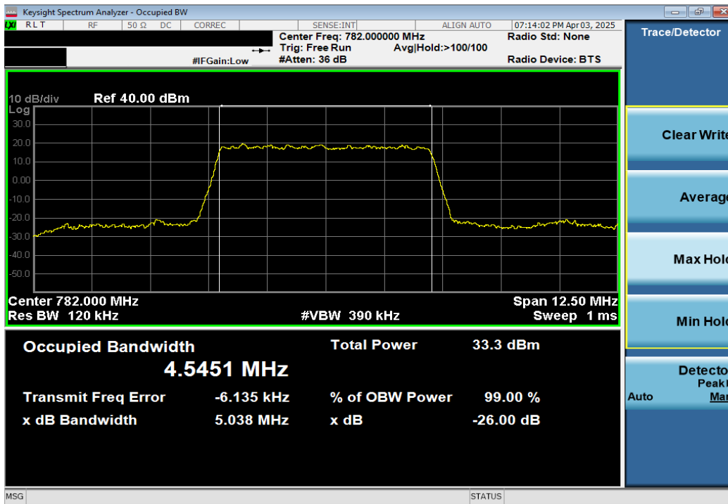
Plot 7-29. Occupied Bandwidth Plot (LTE Band 13 - 5MHz QPSK - Full RB)
