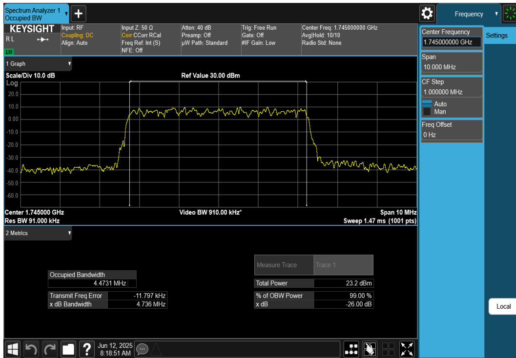
Plot 7-35. Occupied Bandwidth Plot (NR Band n66 - 5MHz DFT-s-OFDM 16QAM - Full RB)
