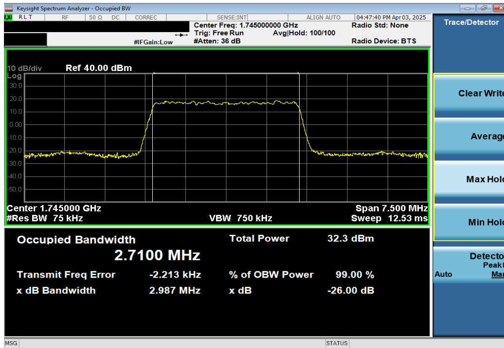
Plot 7-4. Occupied Bandwidth Plot (LTE Band 66/4 - 3MHz 16-QAM - Full RB)
