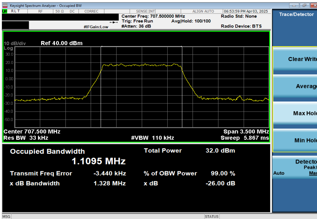
Plot 7-22. Occupied Bandwidth Plot (LTE Band 12 – 1.4MHz 16-QAM - Full RB)
