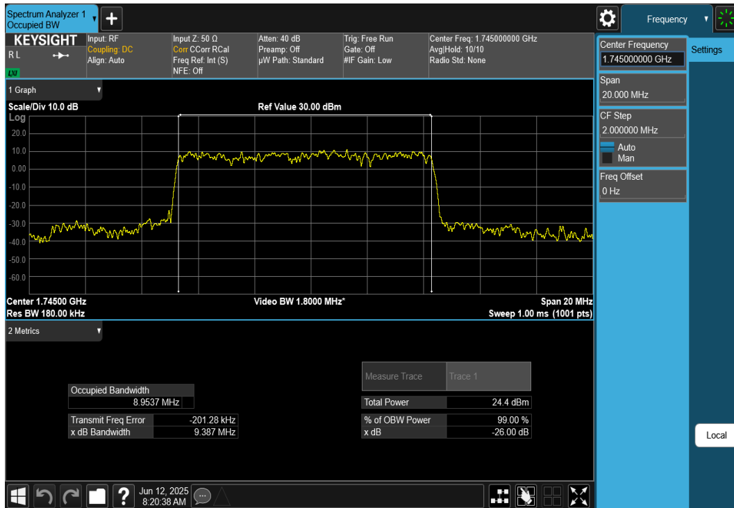
Plot 7-37. Occupied Bandwidth Plot (NR Band n66 - 10MHz DFT-s-OFDM \pi/2 BPSK - Full RB)
