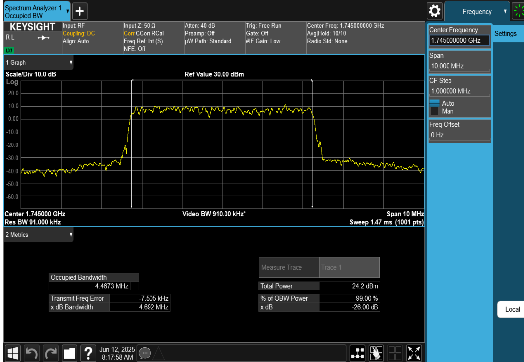
Plot 7-34. Occupied Bandwidth Plot (NR Band n66 - 5MHz DFT-s-OFDM QPSK - Full RB)
