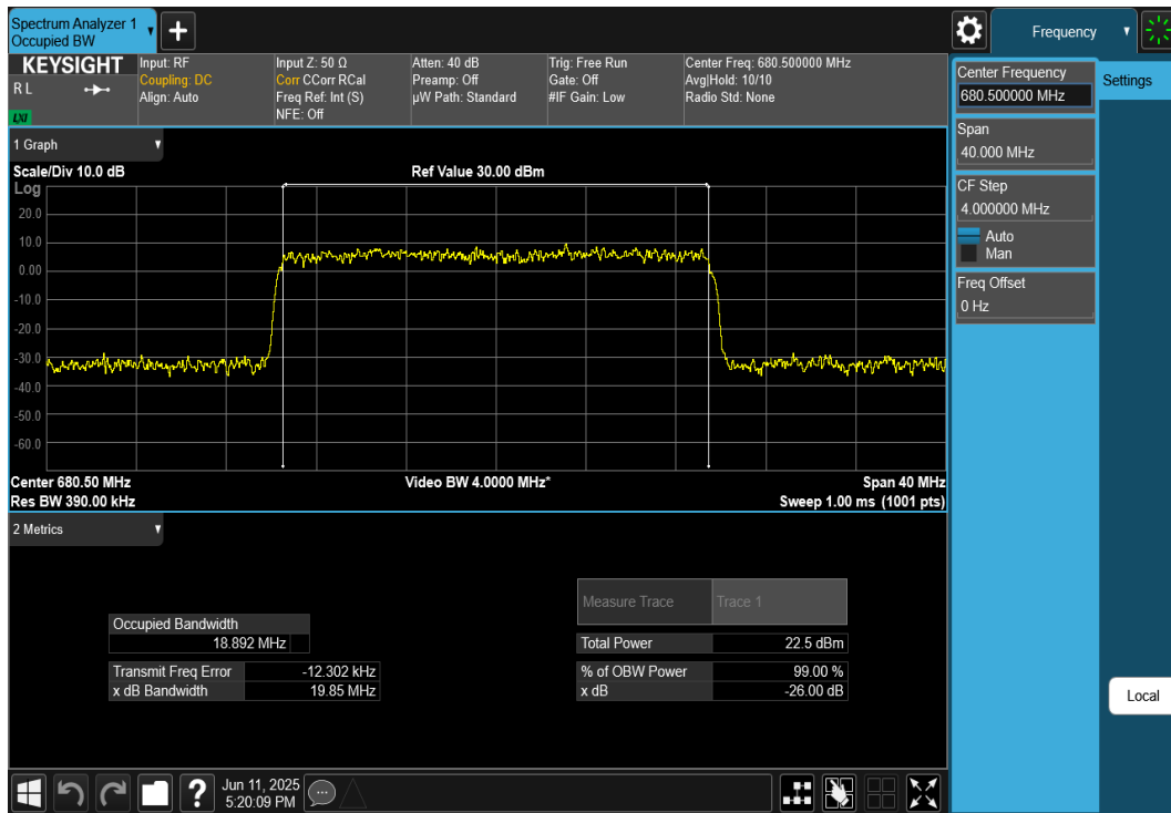
Plot 7-63. Occupied Bandwidth Plot (NR Band n71 - 20MHz CP-OFDM 16-QAM - Full RB)
