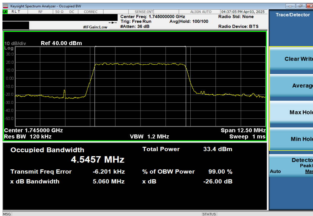
Plot 7-5. Occupied Bandwidth Plot (LTE Band 66/4 - 5MHz QPSK - Full RB)
