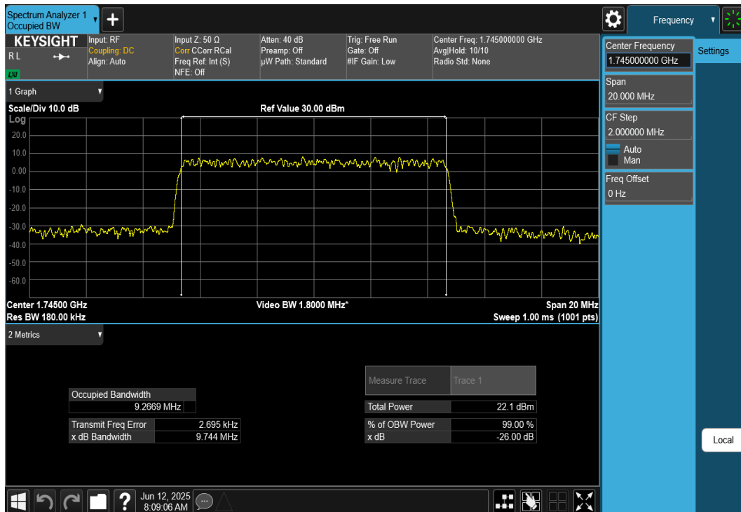
Plot 7-38. Occupied Bandwidth Plot (NR Band n66 - 10MHz CP-OFDM QPSK - Full RB)
