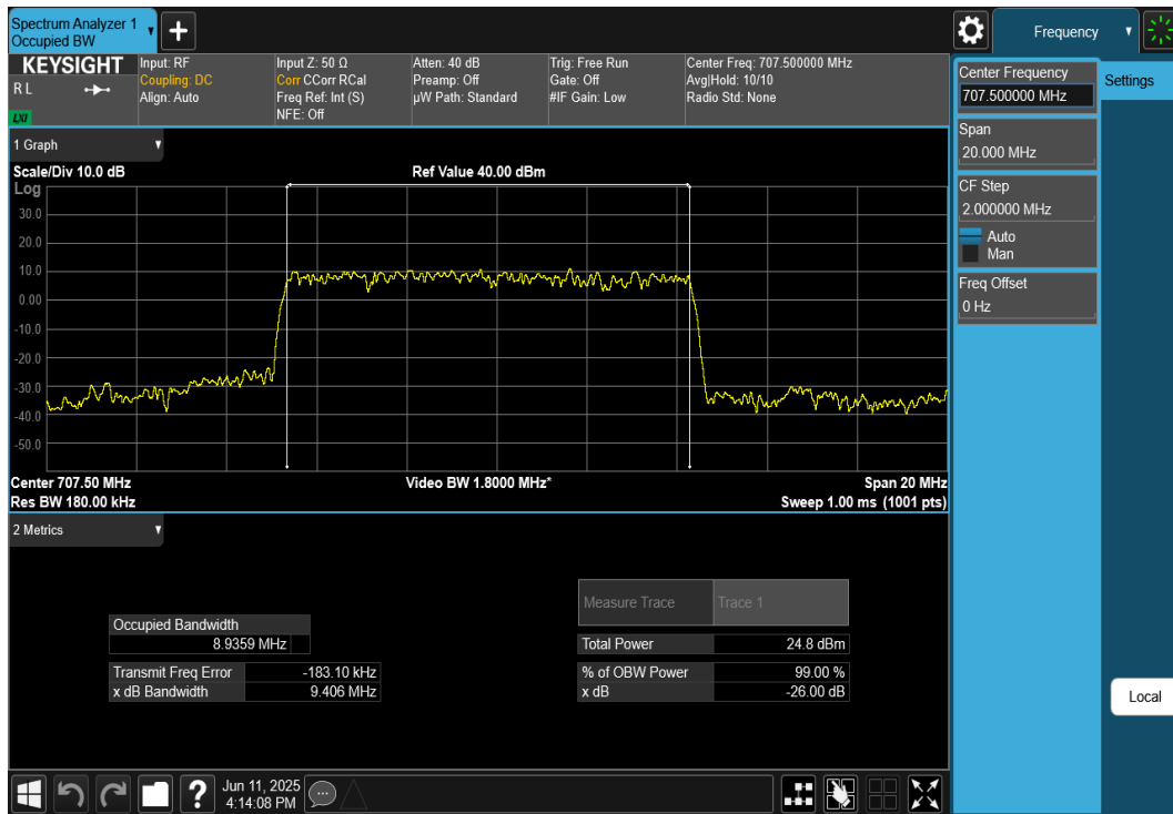
Plot 7-69. Occupied Bandwidth Plot (NR Band n12 - 10MHz DFT-s-OFDM \pi/2 BPSK - Full RB)
