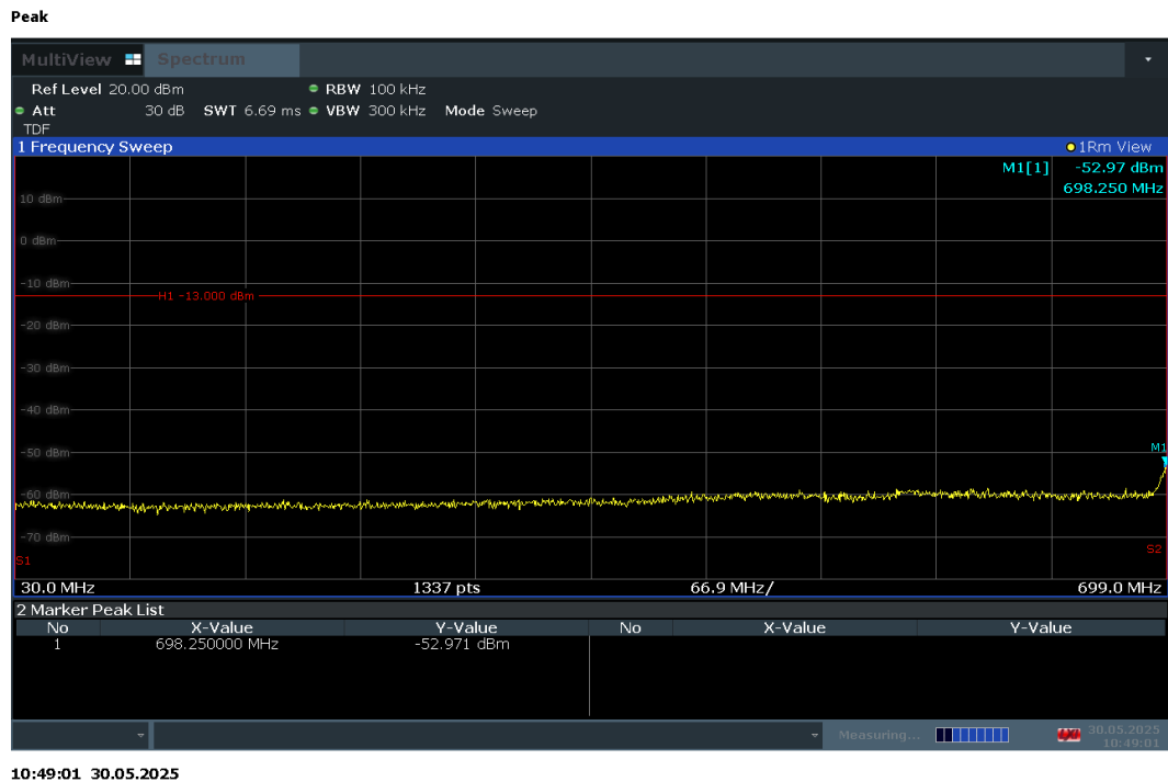
Plot 7-101. Conducted Spurious Plot (LTE Band 12/17 - 10MHz QPSK - RB Size 1, RB Offset 25 - High Channel)
