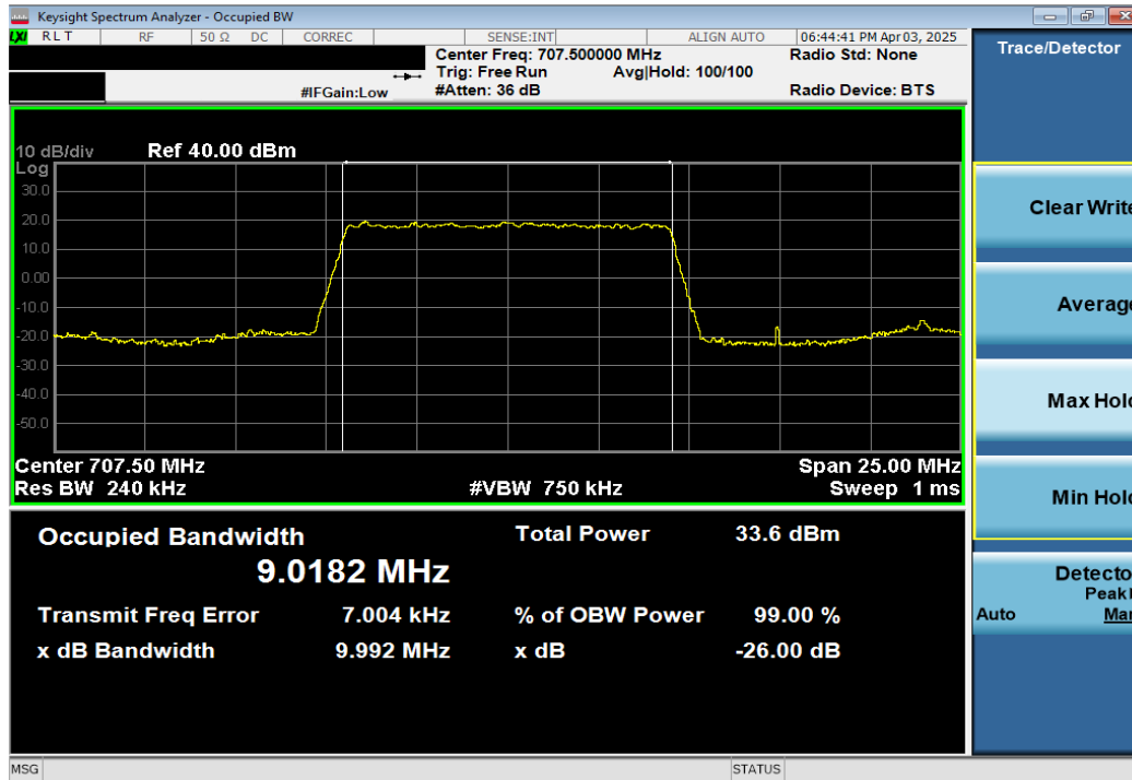
Plot 7-27. Occupied Bandwidth Plot (LTE Band 12/17 - 10MHz QPSK - Full RB)
