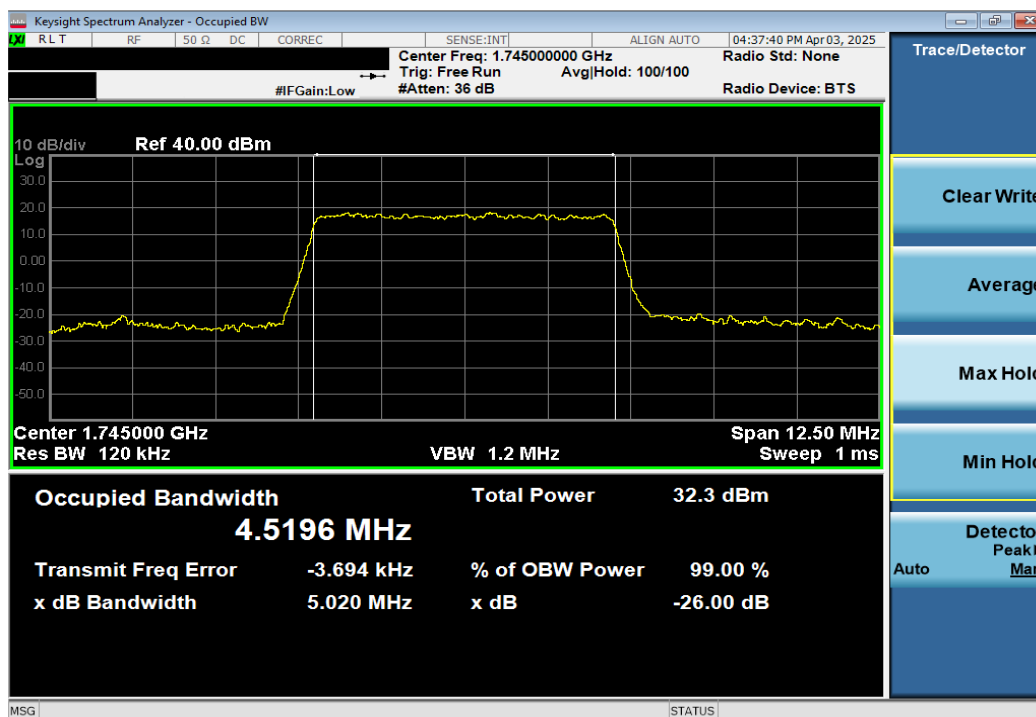
Plot 7-6. Occupied Bandwidth Plot (LTE Band 66/4 - 5MHz 16-QAM - Full RB)
