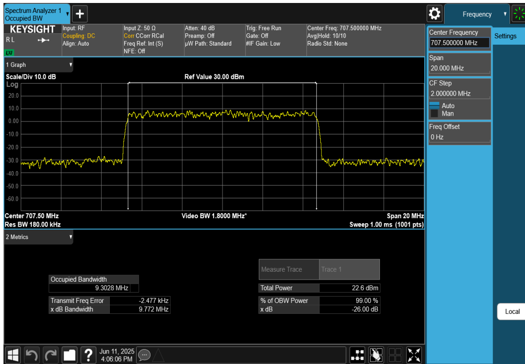
Plot 7-71. Occupied Bandwidth Plot (NR Band n12 - 10MHz CP-OFDM 16-QAM - Full RB)
