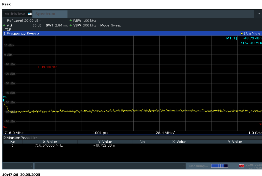
Plot 7-99. Conducted Spurious Plot (LTE Band 12/17 - 10MHz QPSK - RB Size 1, RB Offset 25 - Mid Channel)
