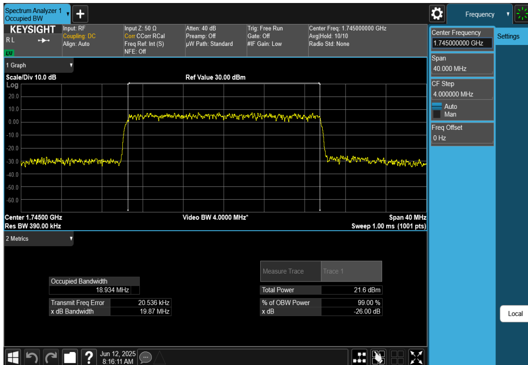
Plot 7-48. Occupied Bandwidth Plot (NR Band n66 - 20MHz CP-OFDM 64QAM - Full RB)
