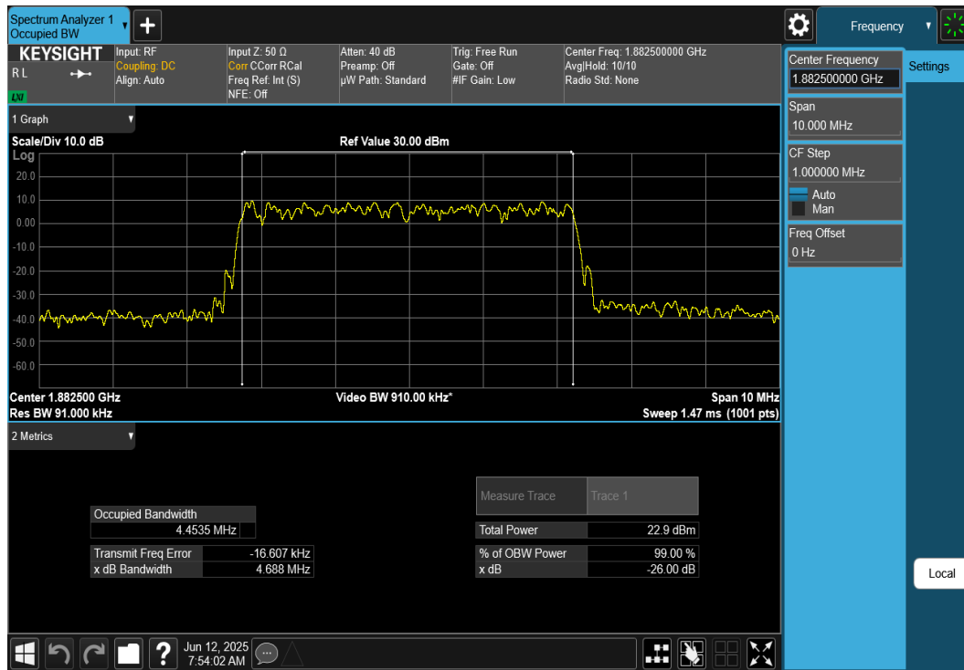
Plot 7-15. Occupied Bandwidth Plot (NR Band n25/n2 - 5MHz DFT-s-OFDM 16QAM - Full RB)
