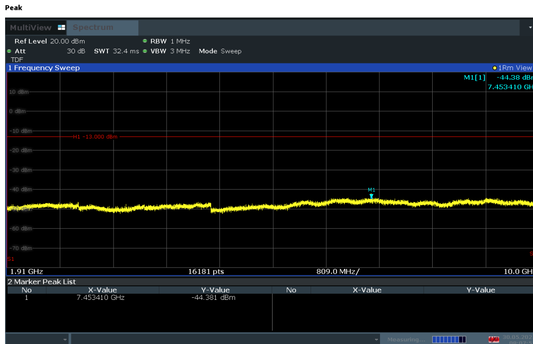
Plot 7-30. Conducted Spurious Plot (LTE Band 25/2 - 20MHz QPSK - RB Size 1, RB Offset 50 - Low Channel)
