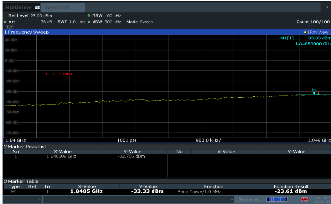
Plot 7-59. Extended Lower Band Edge Plot (LTE Band 25 – 10MHz QPSK – Full RB Configuration)
