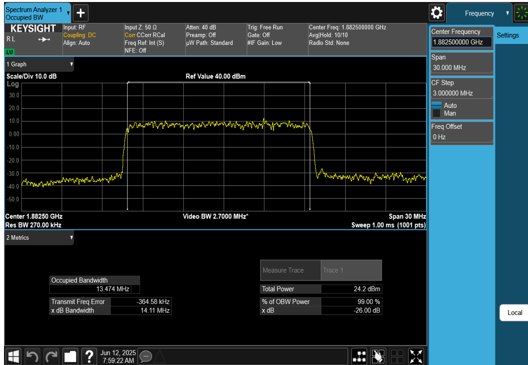
Plot 7-21. Occupied Bandwidth Plot (NR Band n25/n2 - 15MHz DFT-s-OFDM \pi/2 BPSK - Full RB)
