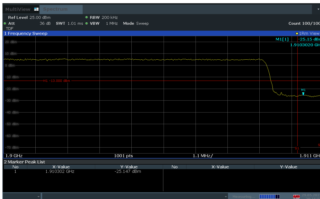
Plot 7-93. Upper Band Edge Plot (LTE Band 2 – 20MHz QPSK – Full RB Configuration)
