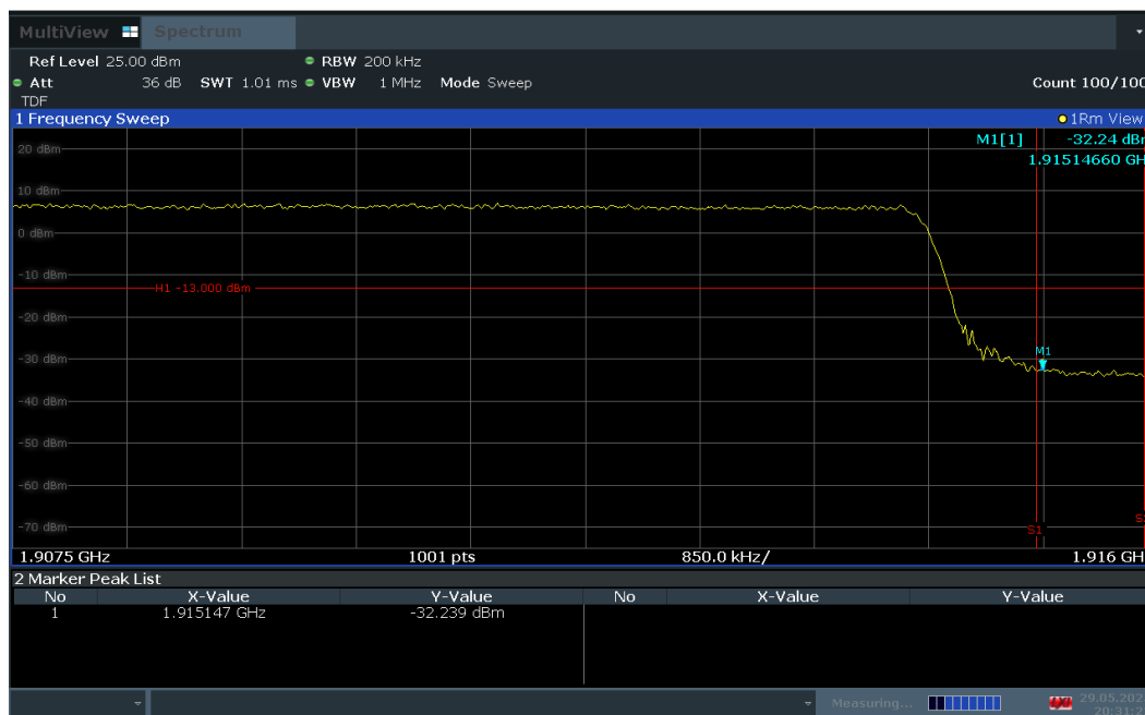
Plot 7-65. Upper Band Edge Plot (LTE Band 25 – 15MHz QPSK – Full RB Configuration)
