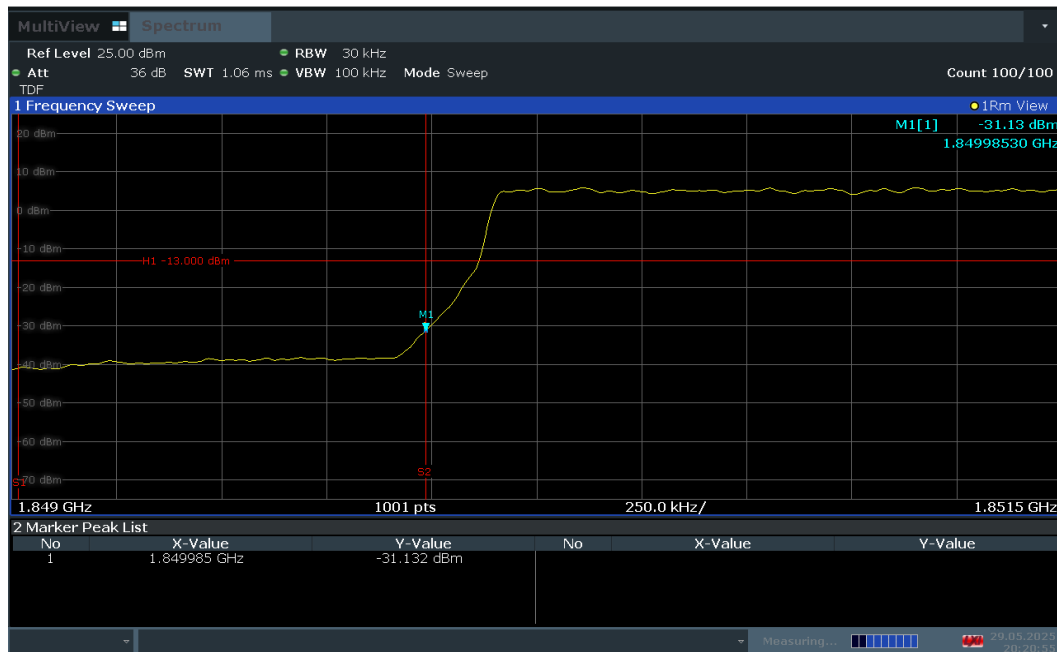
Plot 7-52. Lower Band Edge Plot (LTE Band 25 – 3MHz QPSK – Full RB Configuration)
