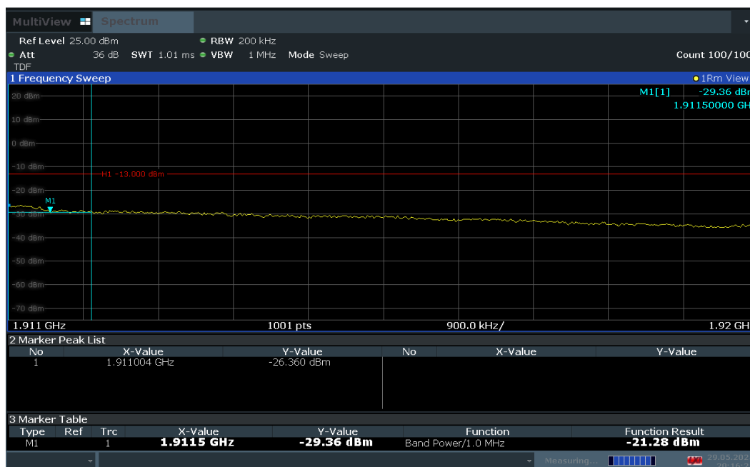
Plot 7-94. Extended Upper Band Edge Plot (LTE Band 2 – 20MHz QPSK – Full RB Configuration)
