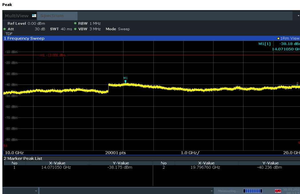
Plot 7-37. Conducted Spurious Plot (LTE Band 25/2 - 20MHz QPSK - RB Size 1, RB Offset 50 - High Channel)
