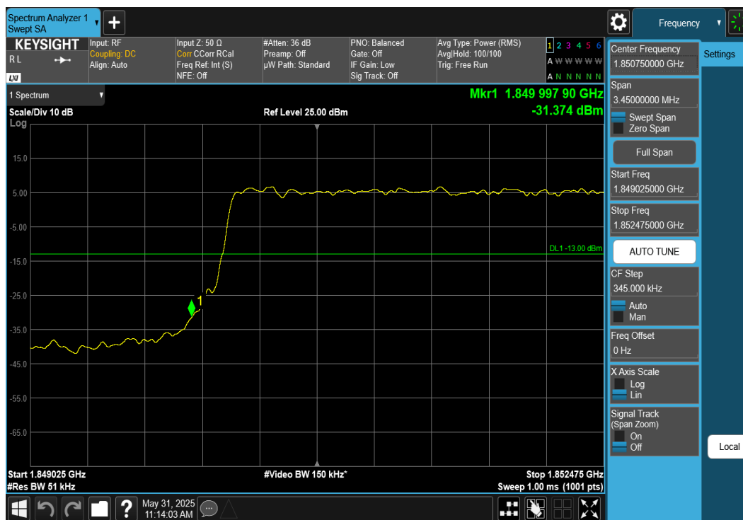
Plot 7-96. Lower Band Edge Plot (NR Band n25 – 5MHz DFT-S-OFDM \pi/2 BPSK – Full RB Configuration)
