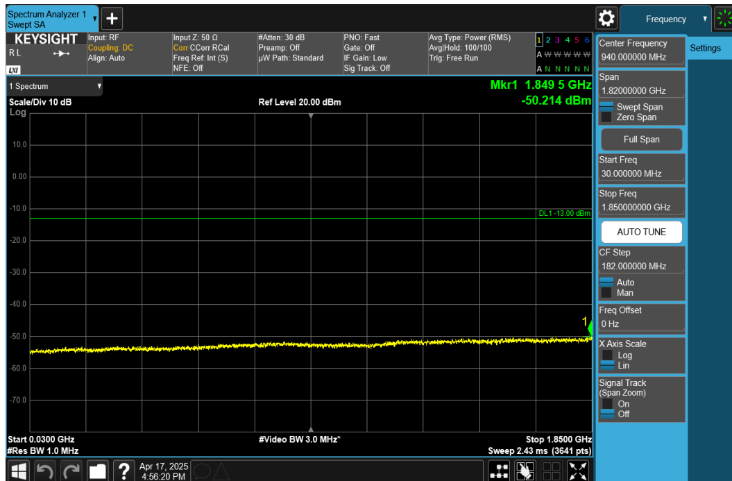
Plot 7-44. Conducted Spurious Plot (NR Band n25/n2 - 20MHz DFT-s-OFDM QPSK - RB Size 1, RB Offset 50 - High Channel)
