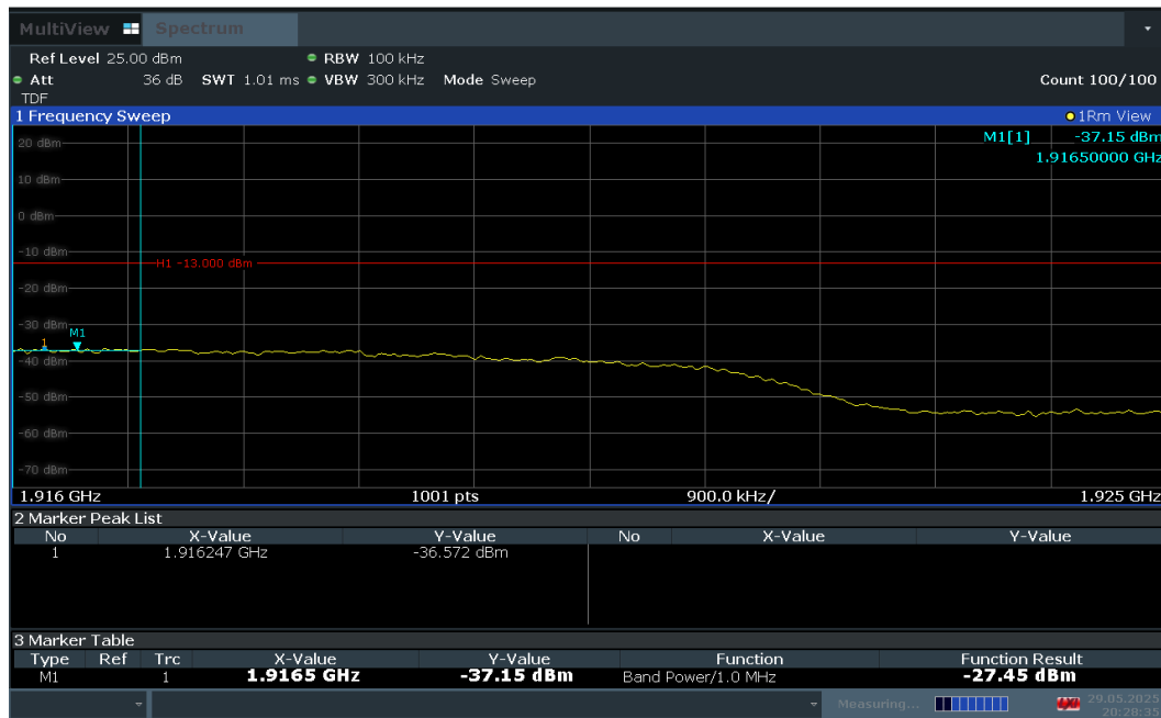
Plot 7-62. Extended Upper Band Edge Plot (LTE Band 25 – 10MHz QPSK – Full RB Configuration)
