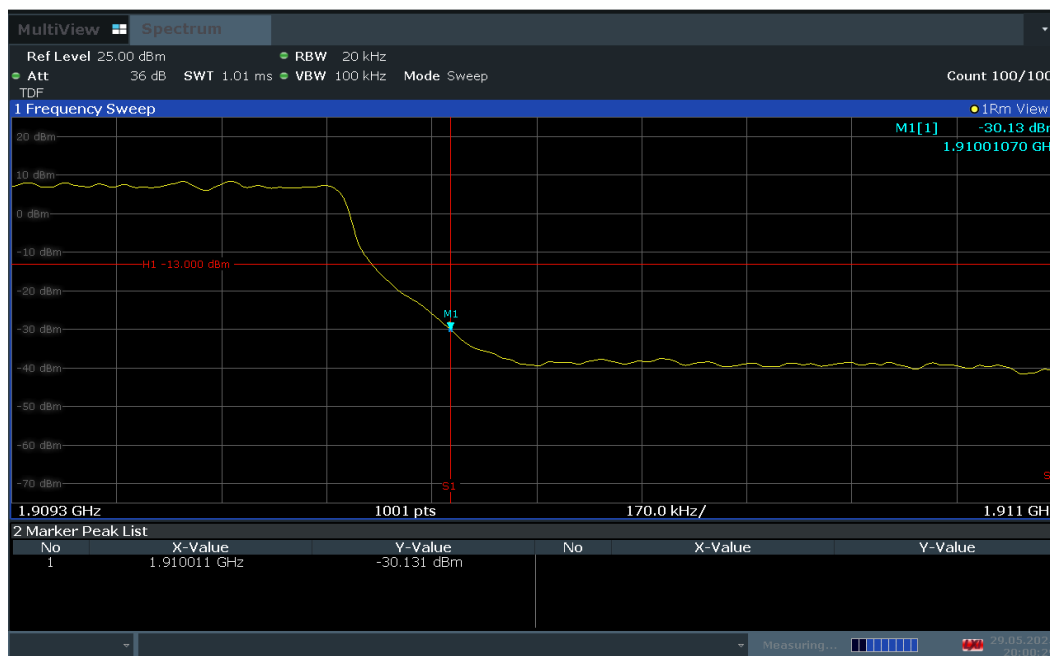
Plot 7-73. Upper Band Edge Plot (LTE Band 2 – 1.4MHz QPSK – Full RB Configuration)
