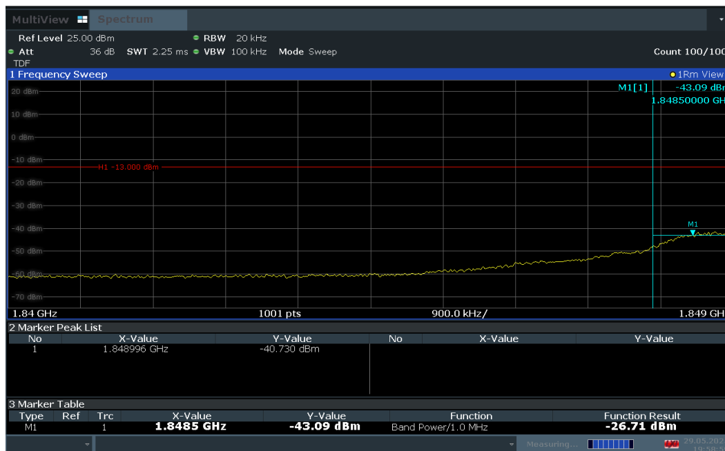
Plot 7-71. Extended Lower Band Edge Plot (LTE Band 2 – 1.4MHz QPSK – Full RB Configuration)
