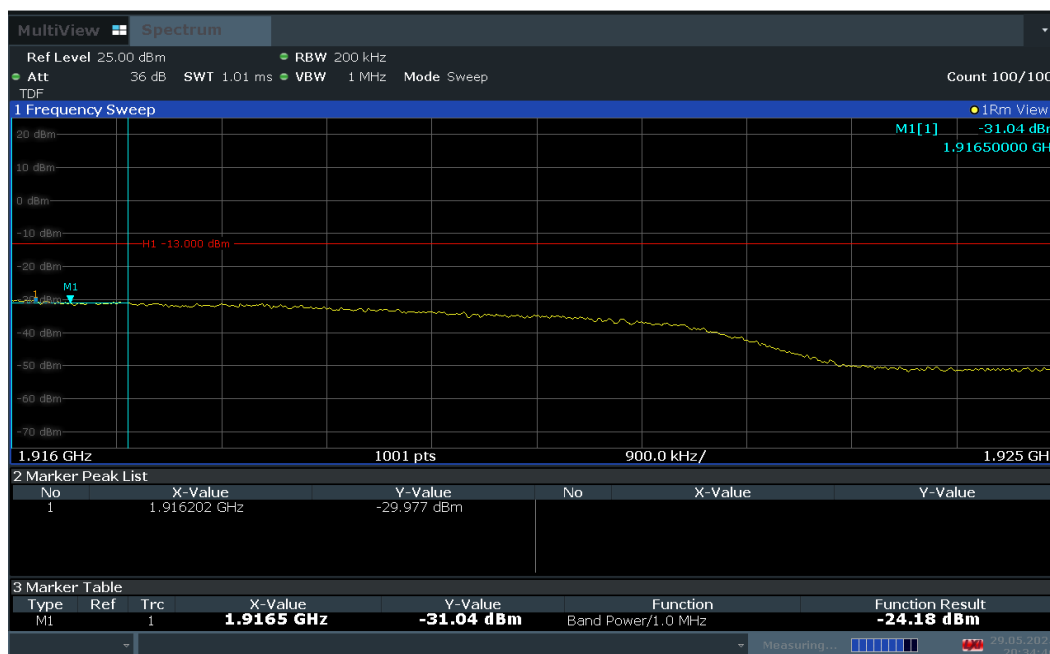
Plot 7-70. Extended Upper Band Edge Plot (LTE Band 25 – 20MHz QPSK – Full RB Configuration)
