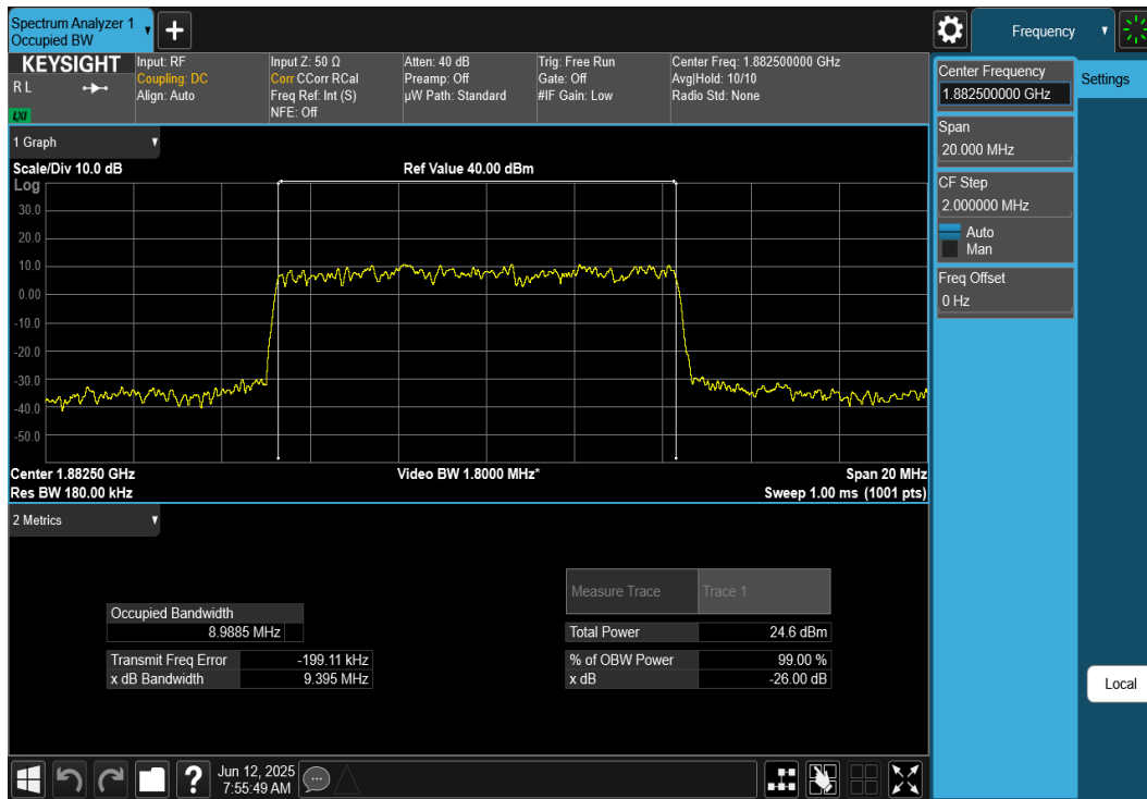
Plot 7-17. Occupied Bandwidth Plot (NR Band n25/n2 - 10MHz DFT-s-OFDM \pi/2 BPSK - Full RB)
