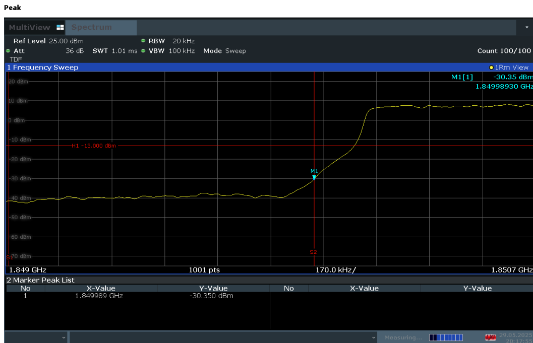
Plot 7-48. Lower Band Edge Plot (LTE Band 25 – 1.4MHz QPSK – Full RB Configuration)
