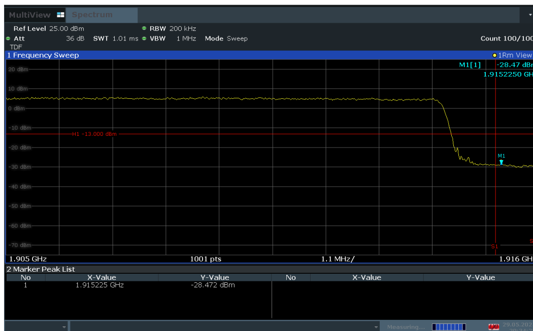
Plot 7-69. Upper Band Edge Plot (LTE Band 25 – 20MHz QPSK – Full RB Configuration)
