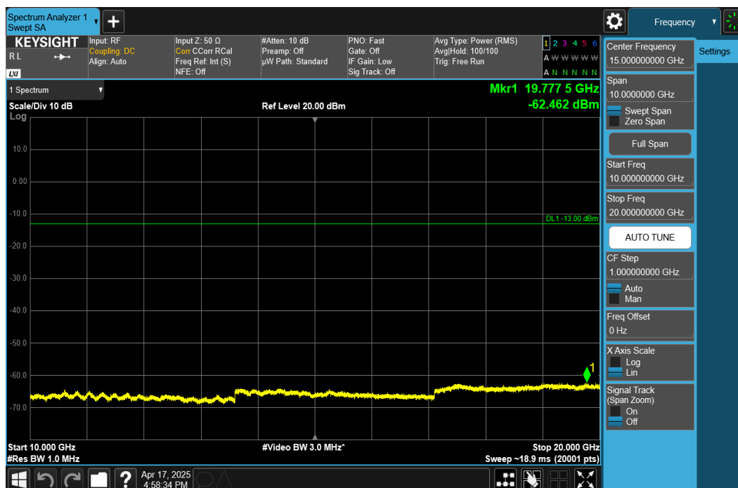
Plot 7-46. Conducted Spurious Plot (NR Band n25/n2 - 20MHz DFT-s-OFDM QPSK - RB Size 1, RB Offset 50 - High Channel)
