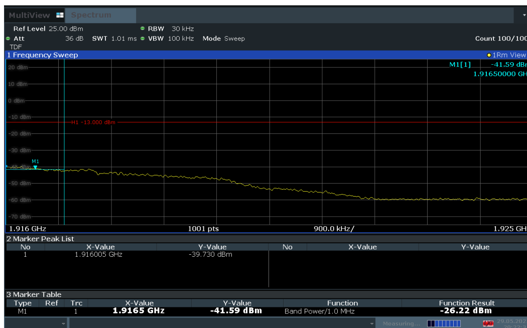
Plot 7-54. Extended Upper Band Edge Plot (LTE Band 25 – 3MHz QPSK – Full RB Configuration)
