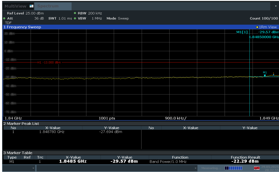
Plot 7-67. Extended Lower Band Edge Plot (LTE Band 25 – 20MHz QPSK – Full RB Configuration)
