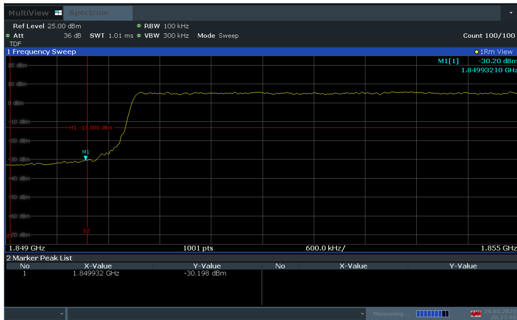
Plot 7-60. Lower Band Edge Plot (LTE Band 25 – 10MHz QPSK – Full RB Configuration)
