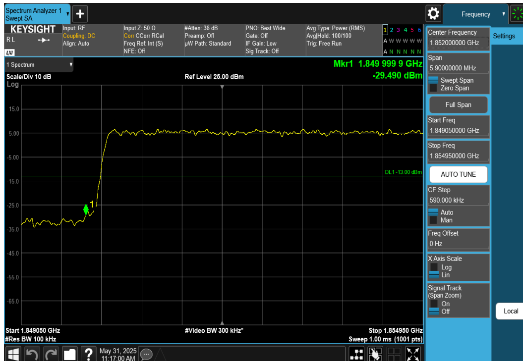
Plot 7-100. Lower Band Edge Plot (NR Band n25 – 10MHz DFT-S-OFDM \pi/2 BPSK – Full RB Configuration)
