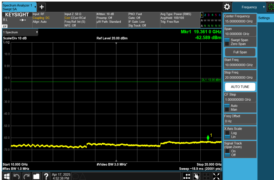
Plot 7-40. Conducted Spurious Plot (NR Band n25/n2 - 20MHz DFT-s-OFDM QPSK - RB Size 1, RB Offset 50 - Low Channel)
