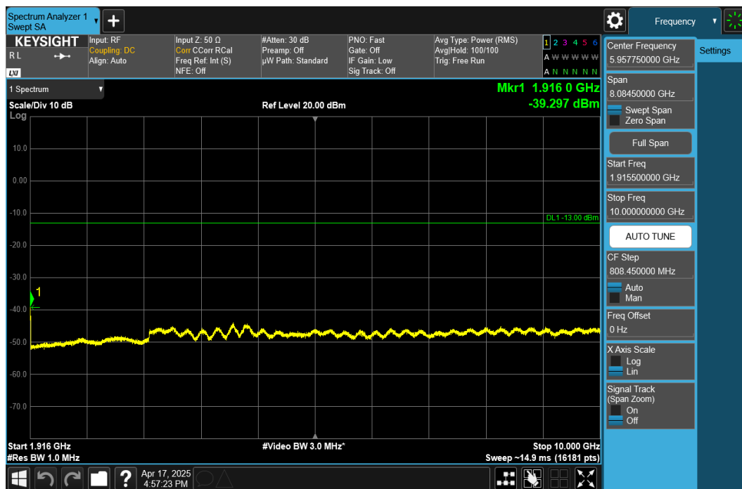
Plot 7-45. Conducted Spurious Plot (NR Band n25/n2 - 20MHz DFT-s-OFDM QPSK - RB Size 1, RB Offset 50 - High Channel)
