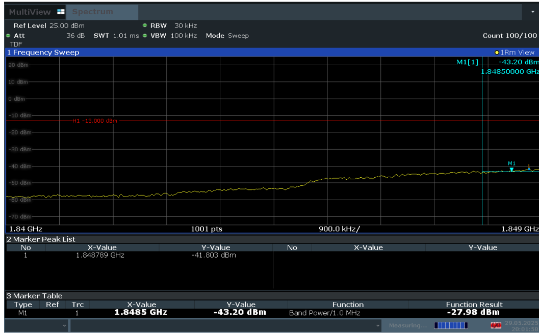
Plot 7-75. Extended Lower Band Edge Plot (LTE Band 2 – 3MHz QPSK – Full RB Configuration)
