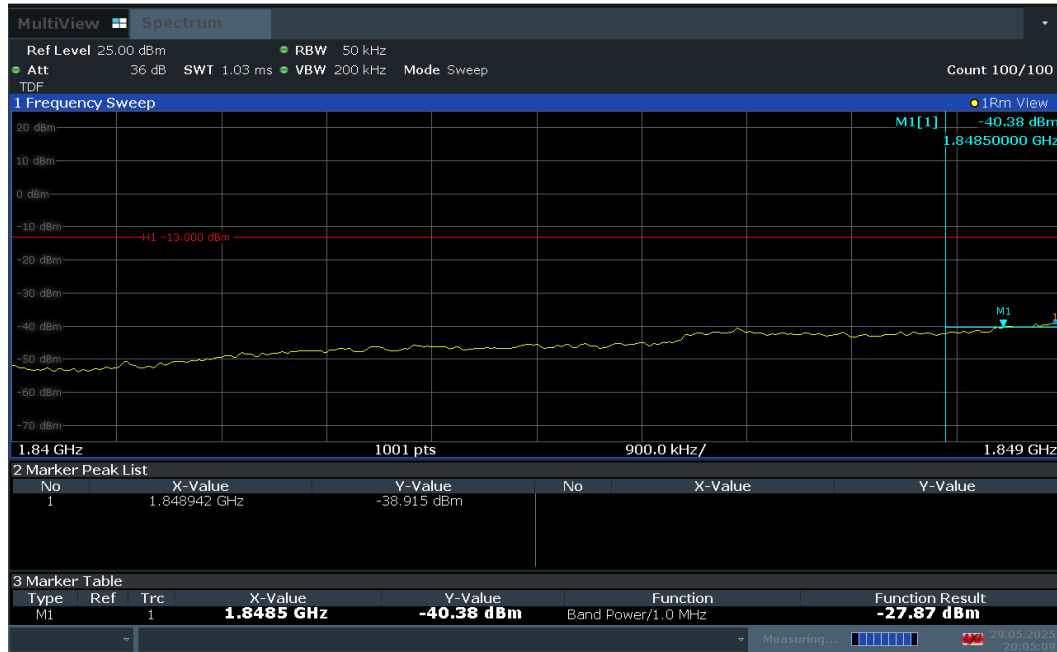
Plot 7-79. Extended Lower Band Edge Plot (LTE Band 2 – 5MHz QPSK – Full RB Configuration)
