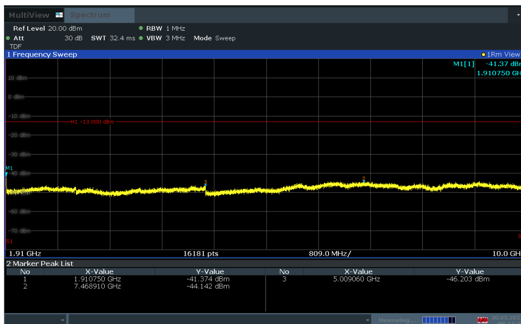
Plot 7-36. Conducted Spurious Plot (LTE Band 25/2 - 20MHz QPSK - RB Size 1, RB Offset 50 - High Channel)
