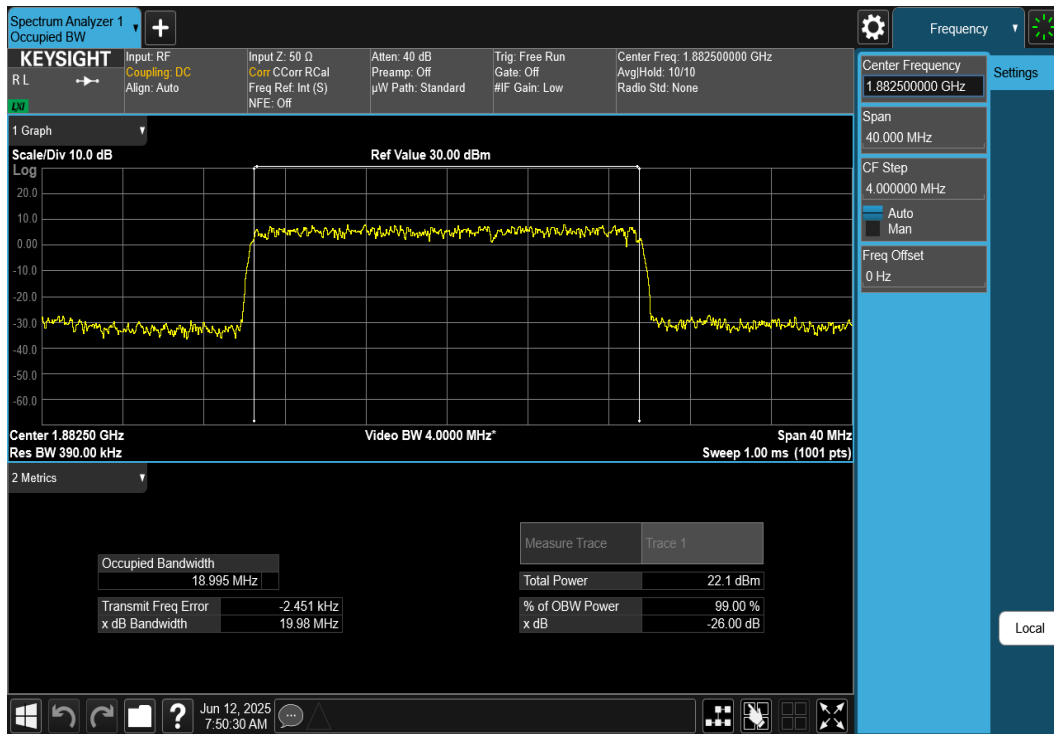
Plot 7-27. Occupied Bandwidth Plot (NR Band n25/n2 - 20MHz CP-OFDM 16QAM - Full RB)
