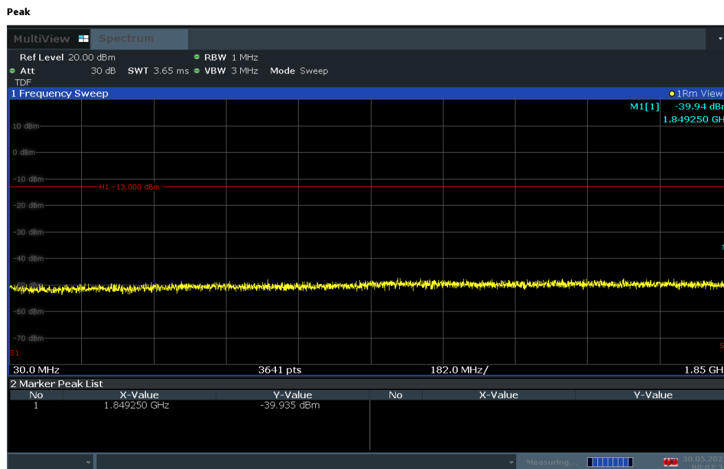
Plot 7-29. Conducted Spurious Plot (LTE Band 25/2 - 20MHz QPSK - RB Size 1, RB Offset 50 - Low Channel)
