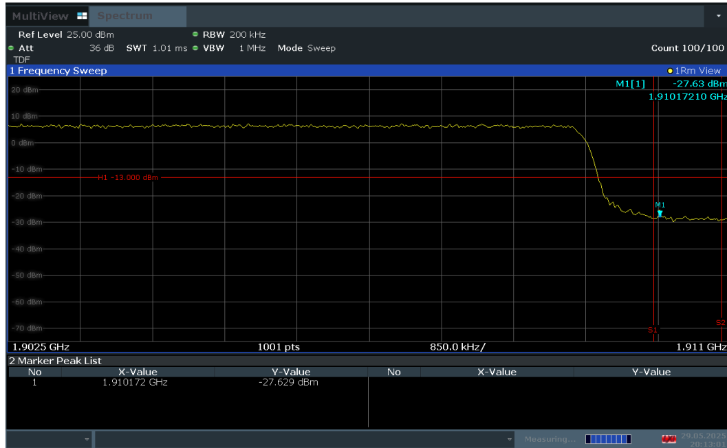
Plot 7-89. Upper Band Edge Plot (LTE Band 2 – 15MHz QPSK – Full RB Configuration)
