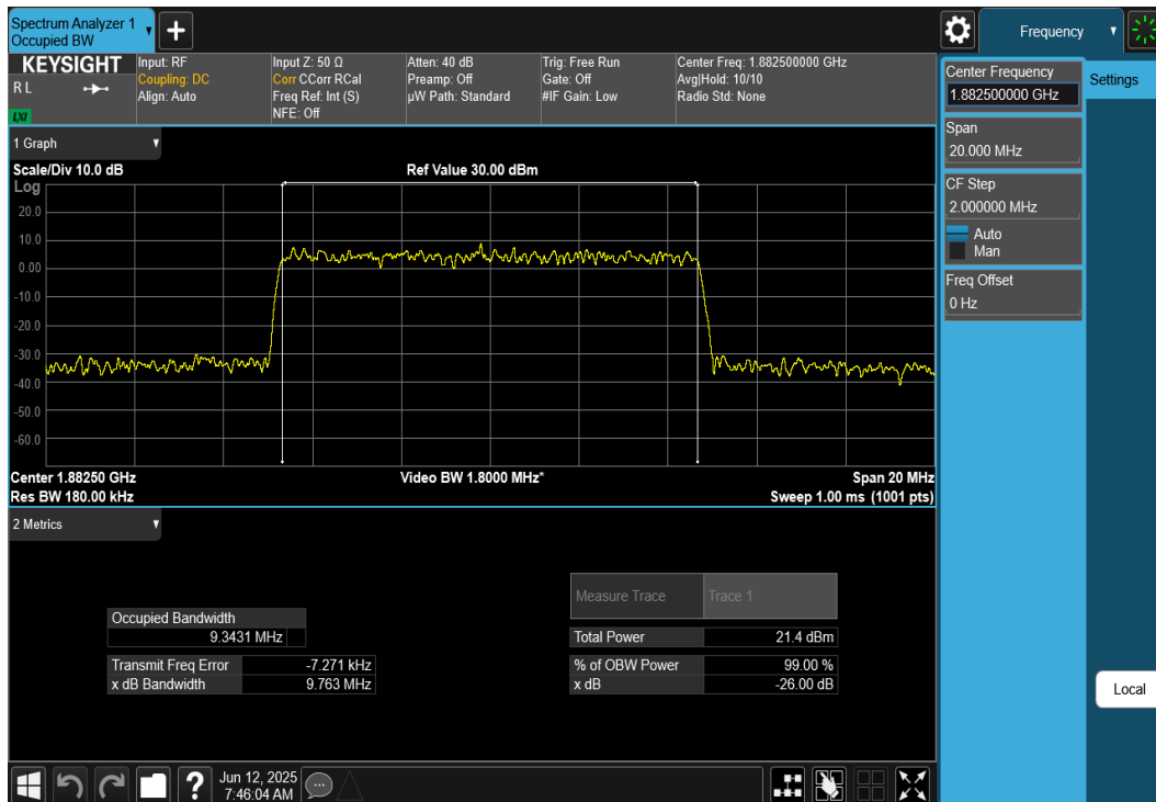
Plot 7-20. Occupied Bandwidth Plot (NR Band n25/n2 - 10MHz CP-OFDM 64QAM - Full RB)
