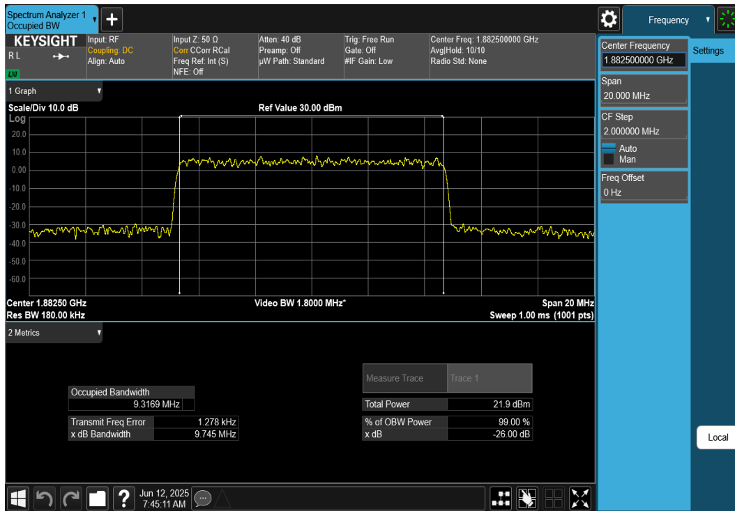
Plot 7-19. Occupied Bandwidth Plot (NR Band n25/n2 - 10MHz CP-OFDM 16QAM - Full RB)
