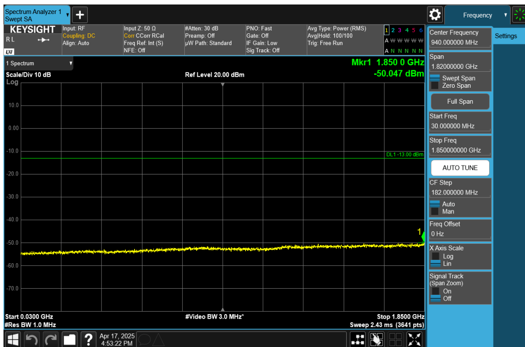
Plot 7-41. Conducted Spurious Plot (NR Band n25/n2 - 20MHz DFT-s-OFDM QPSK - RB Size 1, RB Offset 50 - Mid Channel)
