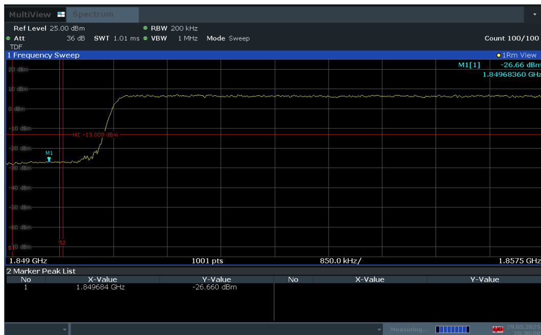
Plot 7-64. Lower Band Edge Plot (LTE Band 25 – 15MHz QPSK – Full RB Configuration)
