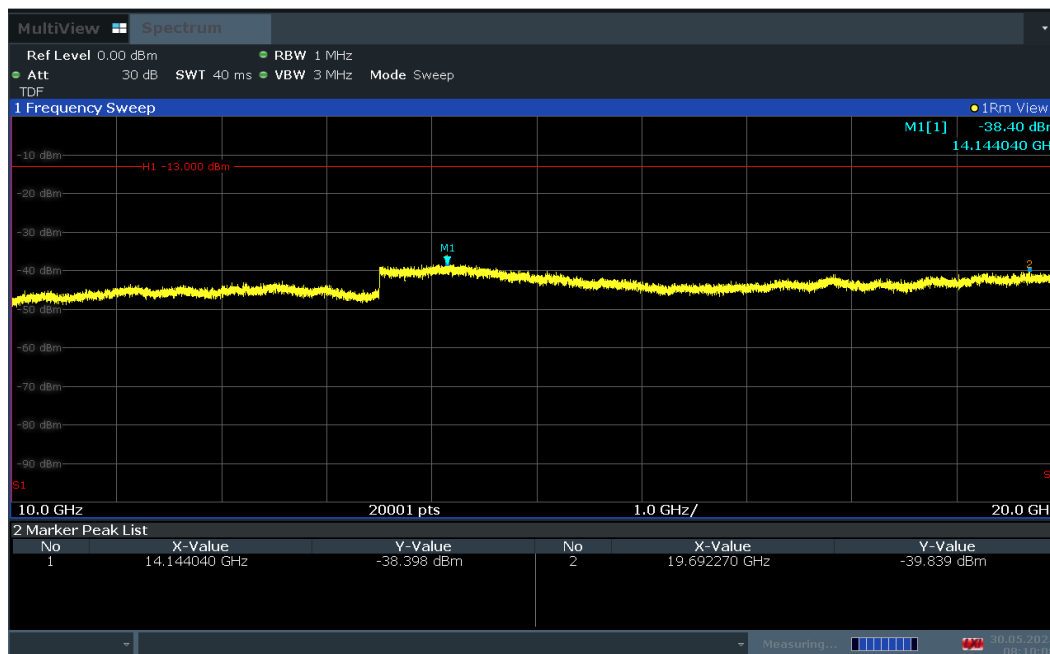
Plot 7-34. Conducted Spurious Plot (LTE Band 25/2 - 20MHz QPSK - RB Size 1, RB Offset 50 - Mid Channel)
