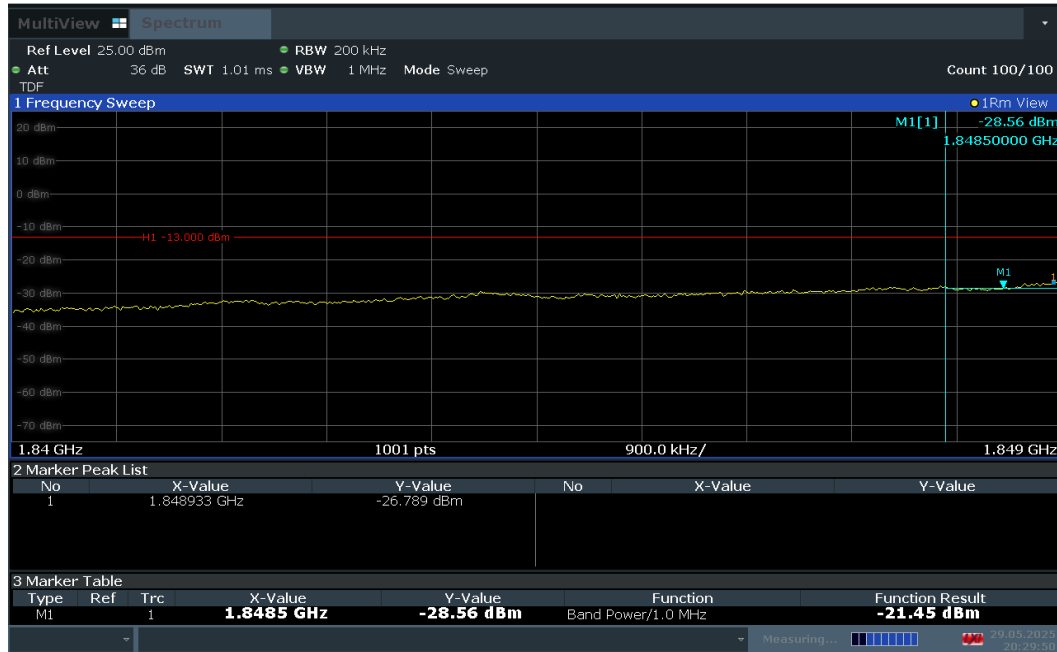
Plot 7-63. Extended Lower Band Edge Plot (LTE Band 25 – 15MHz QPSK – Full RB Configuration)
