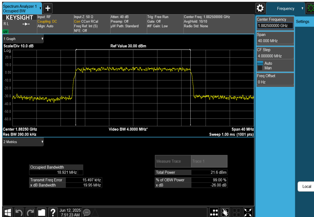
Plot 7-28. Occupied Bandwidth Plot (NR Band n25/n2 - 20MHz CP-OFDM 64QAM - Full RB)
