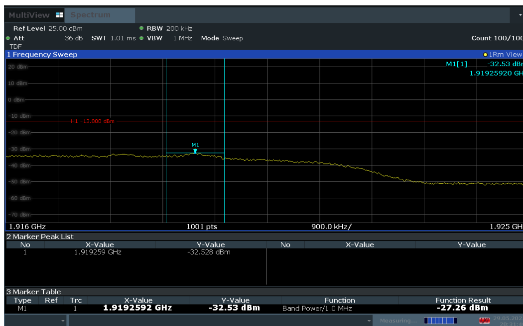
Plot 7-66. Extended Upper Band Edge Plot (LTE Band 25 – 15MHz QPSK – Full RB Configuration)
