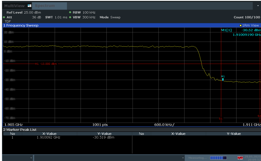
Plot 7-85. Upper Band Edge Plot (LTE Band 2 – 10MHz QPSK – Full RB Configuration)
