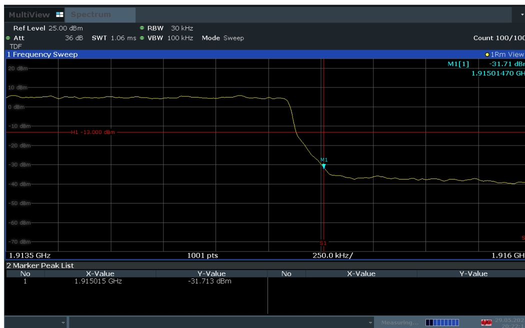
Plot 7-53. Upper Band Edge Plot (LTE Band 25 – 3MHz QPSK – Full RB Configuration)
