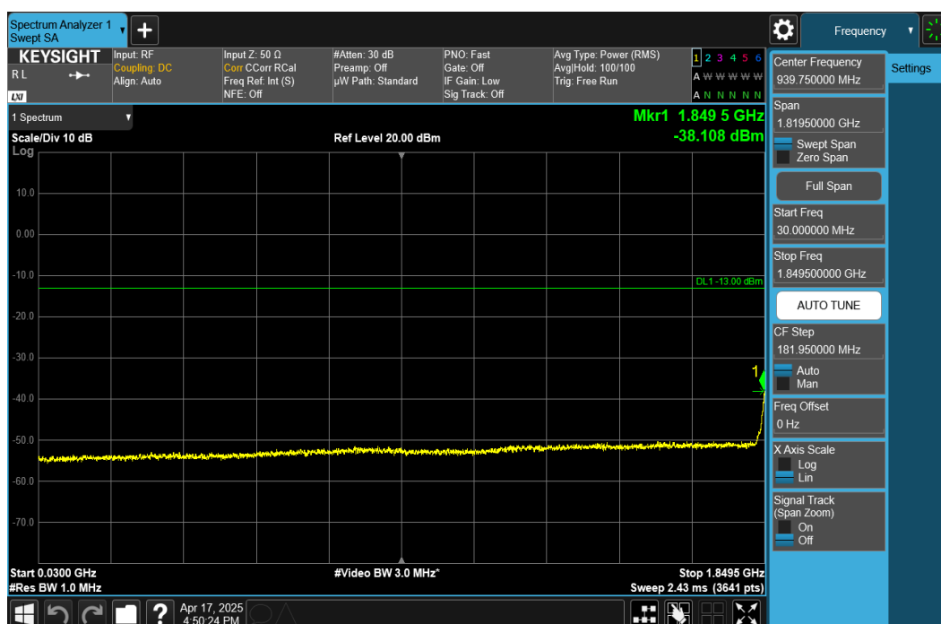
Plot 7-38. Conducted Spurious Plot (NR Band n25/n2 - 20MHz DFT-s-OFDM QPSK - RB Size 1, RB Offset 50 - Low Channel)
