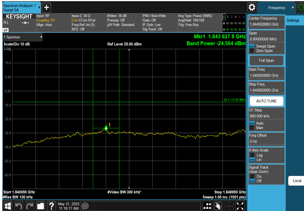
Plot 7-99. Extended Lower Band Edge Plot (NR Band n25 – 10MHz DFT-S-OFDM \pi/2 BPSK – Full RB Configuration)
