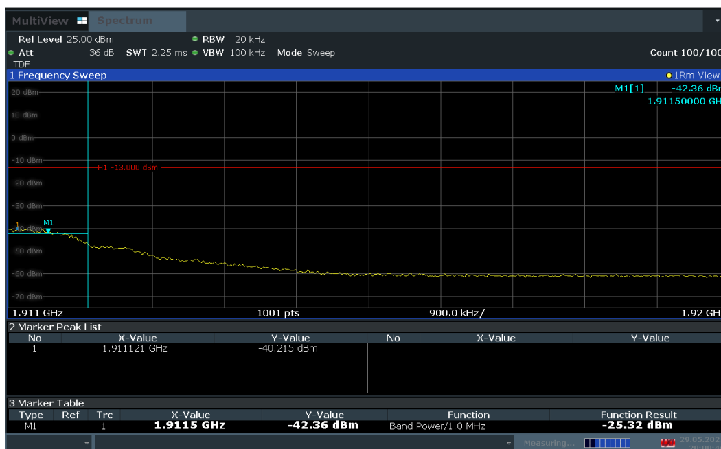
Plot 7-74. Extended Upper Band Edge Plot (LTE Band 2 – 1.4MHz QPSK – Full RB Configuration)
