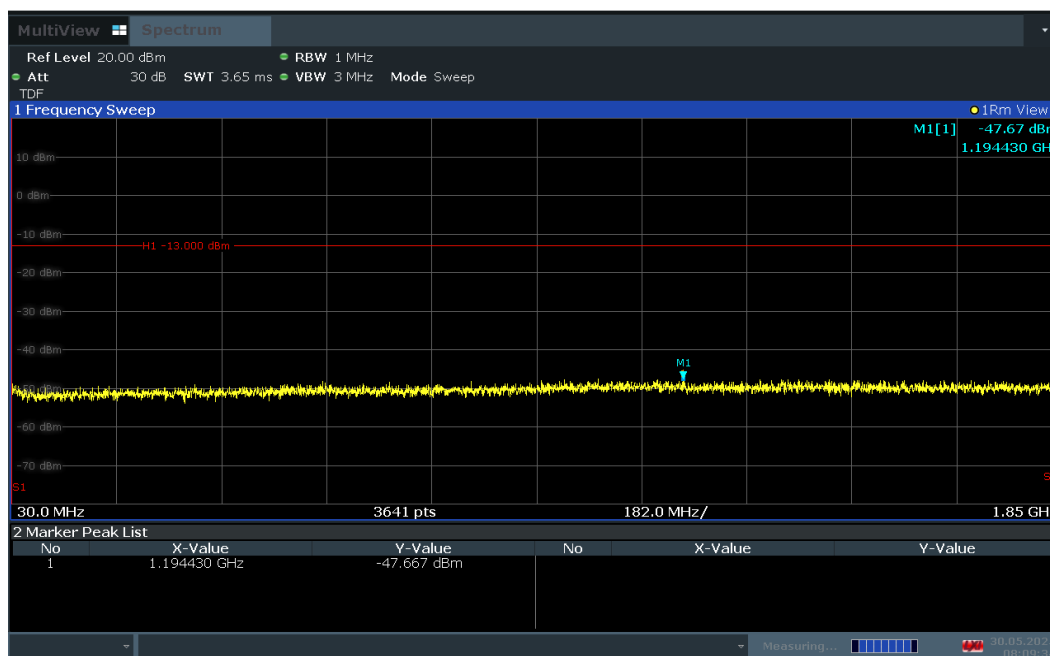
Plot 7-32. Conducted Spurious Plot (LTE Band 25/2 - 20MHz QPSK - RB Size 1, RB Offset 50 - Mid Channel)
