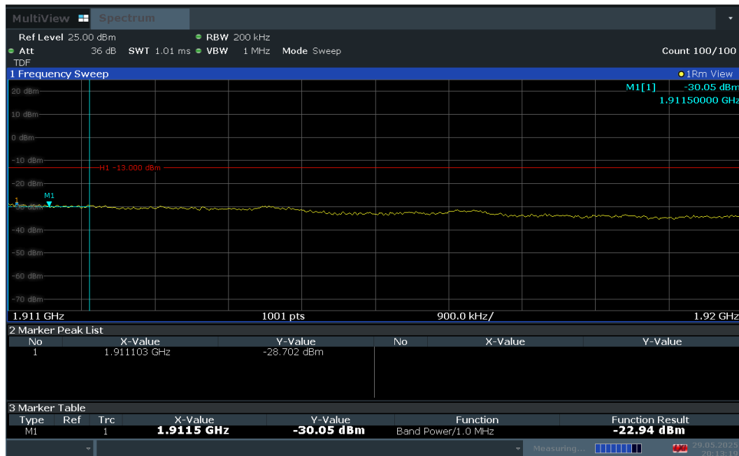
Plot 7-90. Extended Upper Band Edge Plot (LTE Band 2 – 15MHz QPSK – Full RB Configuration)
