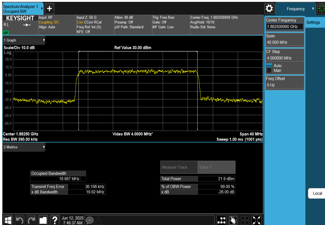
Plot 7-26. Occupied Bandwidth Plot (NR Band n25/n2 - 20MHz CP-OFDM QPSK - Full RB)
