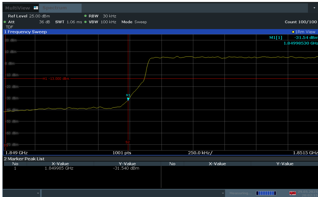
Plot 7-76. Lower Band Edge Plot (LTE Band 2 – 3MHz QPSK – Full RB Configuration)
