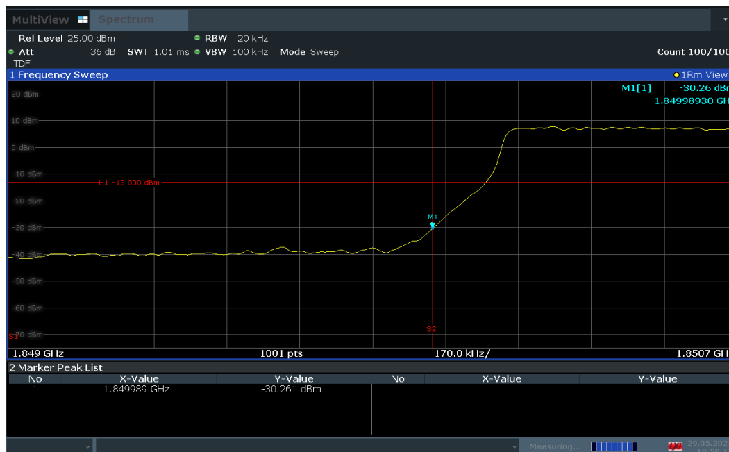
Plot 7-72. Lower Band Edge Plot (LTE Band 2 – 1.4MHz QPSK – Full RB Configuration)
