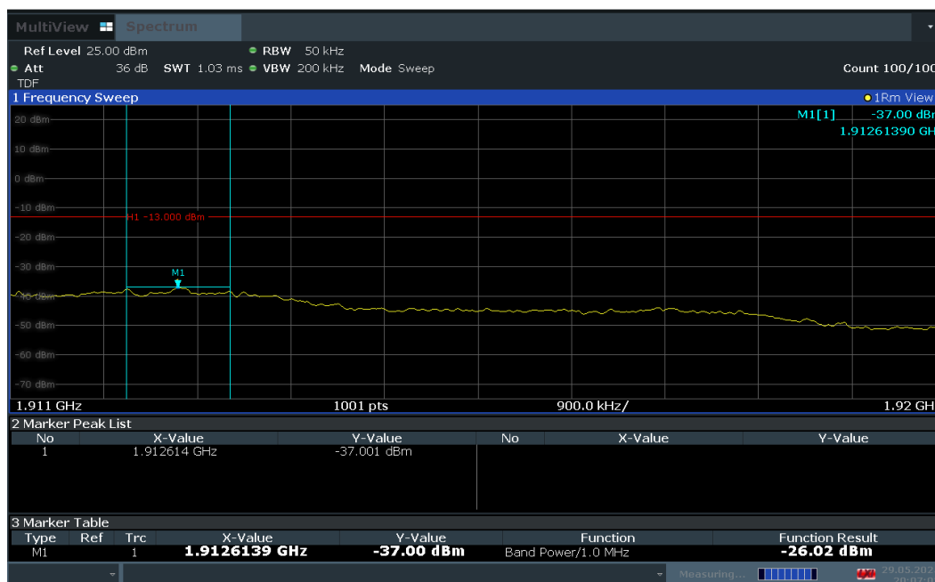
Plot 7-82. Extended Upper Band Edge Plot (LTE Band 2 – 5MHz QPSK – Full RB Configuration)
