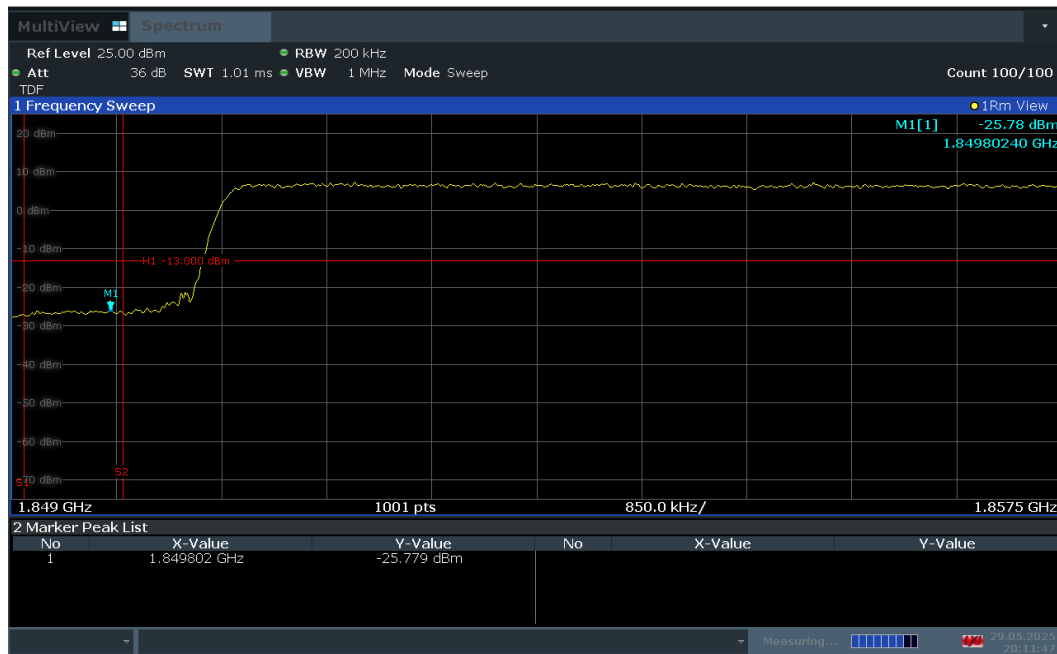
Plot 7-88. Lower Band Edge Plot (LTE Band 2 – 15MHz QPSK – Full RB Configuration)
