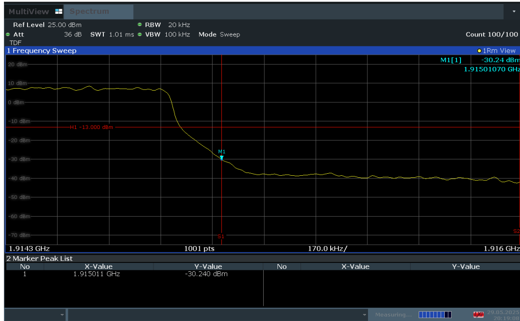
Plot 7-49. Upper Band Edge Plot (LTE Band 25 – 1.4MHz QPSK – Full RB Configuration)
