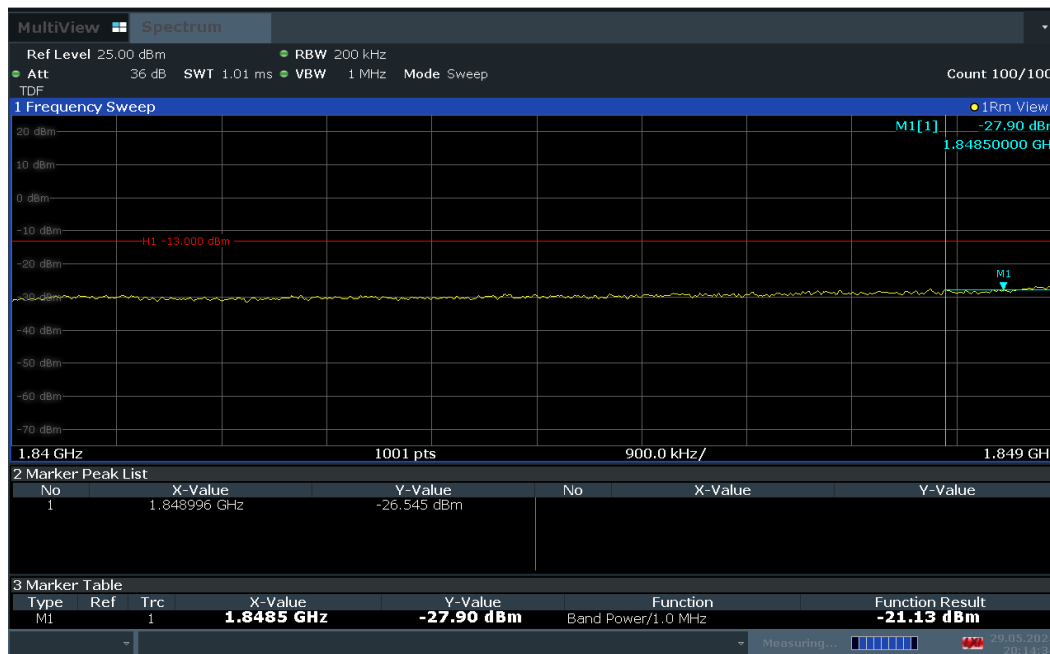
Plot 7-91. Extended Lower Band Edge Plot (LTE Band 2 – 20MHz QPSK – Full RB Configuration)
