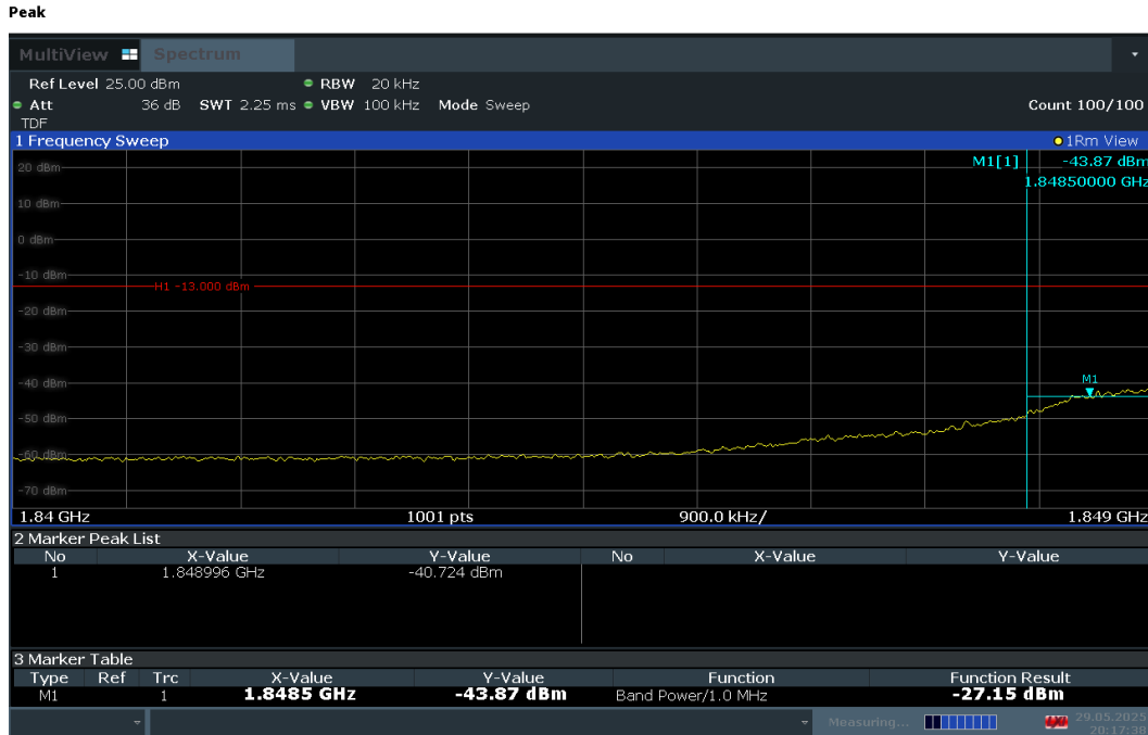
Plot 7-47. Extended Lower Band Edge Plot (LTE Band 25 – 1.4MHz QPSK – Full RB Configuration)
