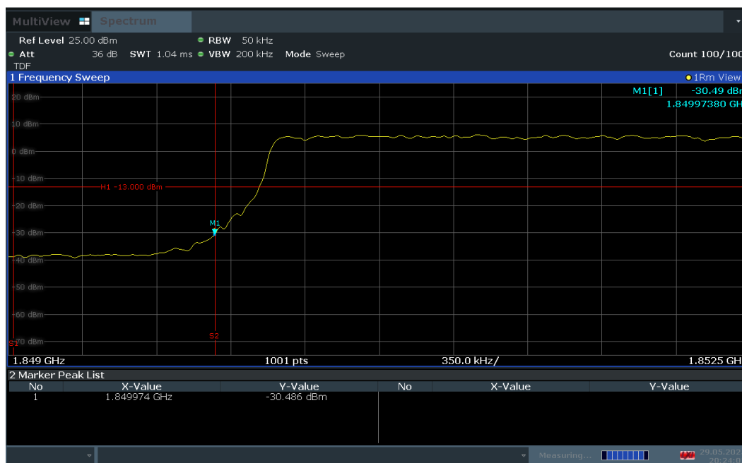
Plot 7-56. Lower Band Edge Plot (LTE Band 25 – 5MHz QPSK – Full RB Configuration)
