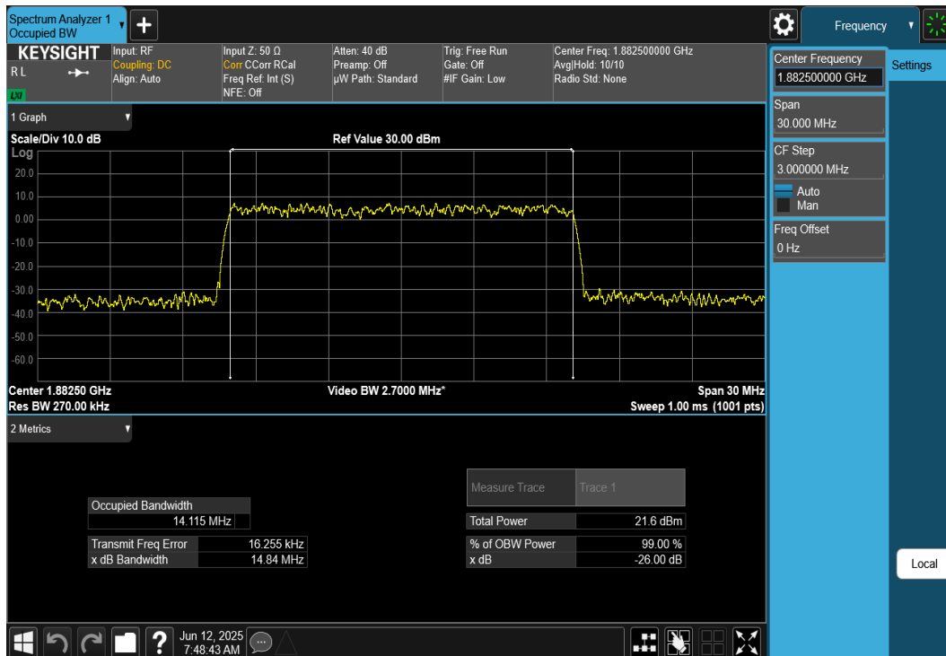
Plot 7-24. Occupied Bandwidth Plot (NR Band n25/n2 - 15MHz CP-OFDM 64QAM - Full RB)
