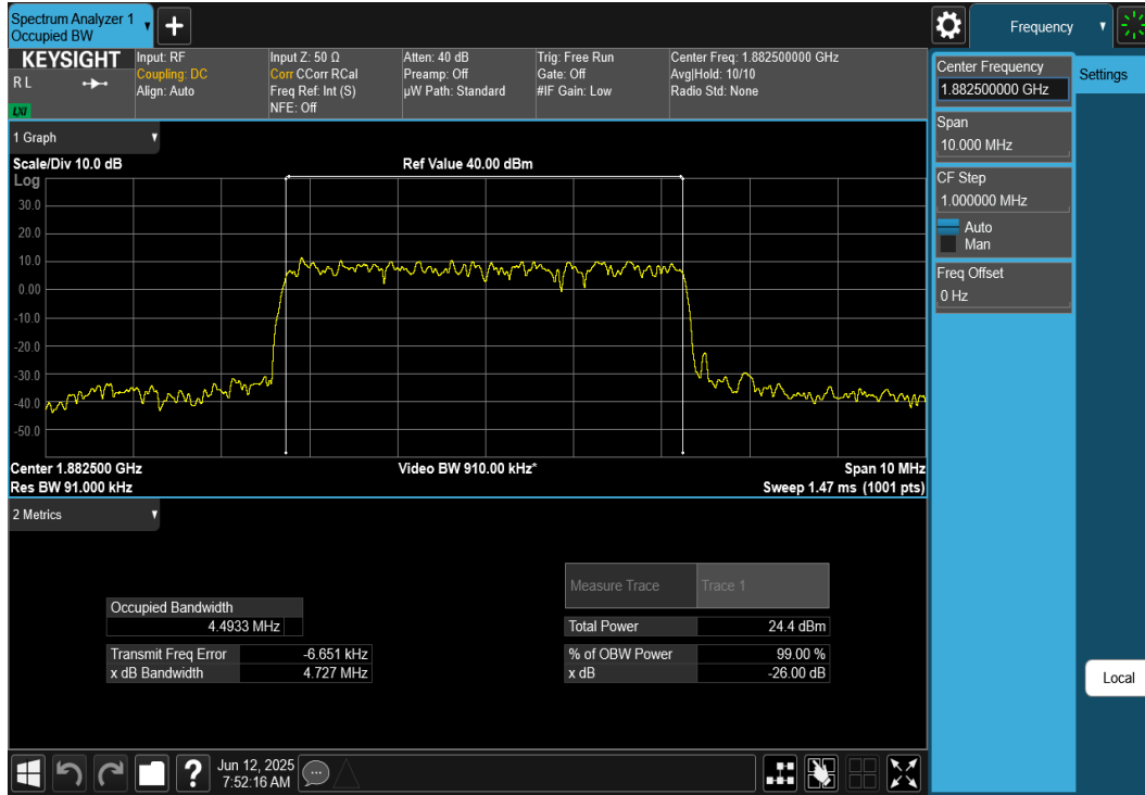
Plot 7-13. Occupied Bandwidth Plot (NR Band n25/n2 - 5MHz DFT-s-OFDM \pi/2 BPSK - Full RB)
