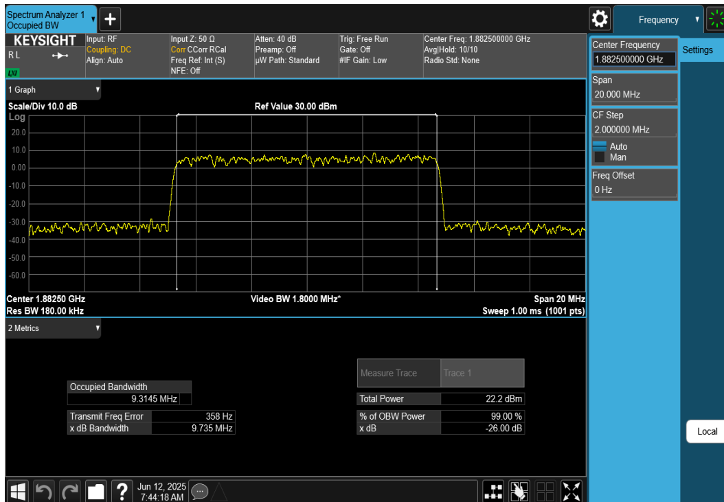
Plot 7-18. Occupied Bandwidth Plot (NR Band n25/n2 - 10MHz CP-OFDM QPSK - Full RB)
