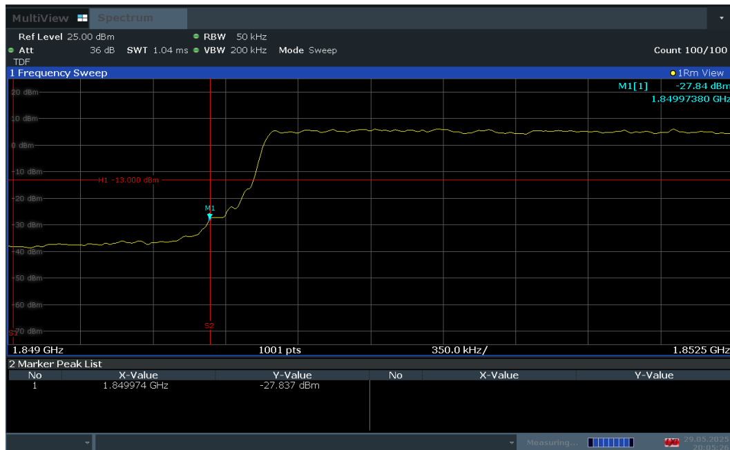
Plot 7-80. Lower Band Edge Plot (LTE Band 2 – 5MHz QPSK – Full RB Configuration)
