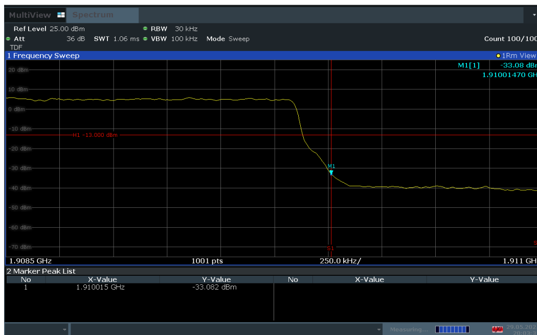
Plot 7-77. Upper Band Edge Plot (LTE Band 2 – 3MHz QPSK – Full RB Configuration)
