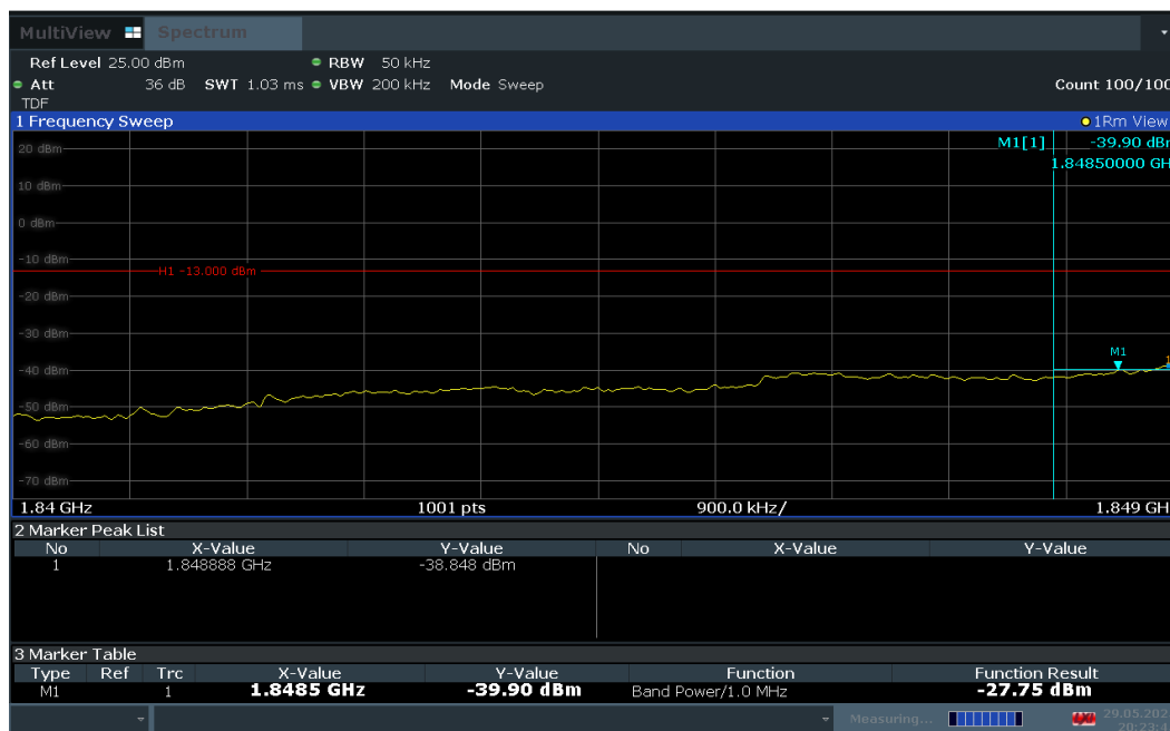
Plot 7-55. Extended Lower Band Edge Plot (LTE Band 25 – 5MHz QPSK – Full RB Configuration)
