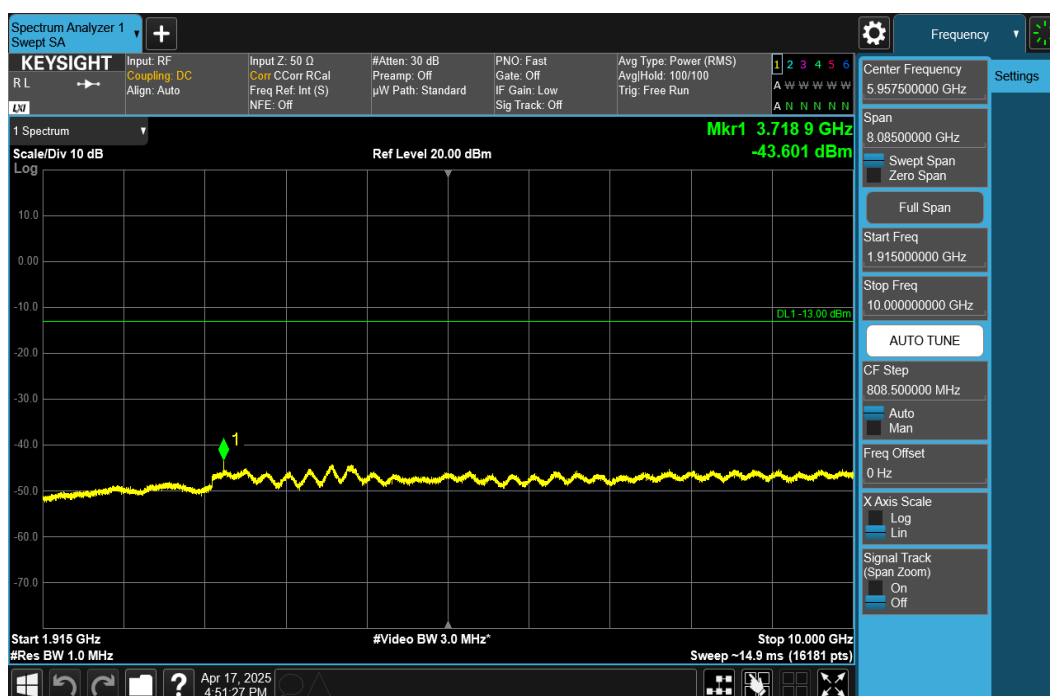
Plot 7-39. Conducted Spurious Plot (NR Band n25/n2 - 20MHz DFT-s-OFDM QPSK - RB Size 1, RB Offset 50 - Low Channel)
