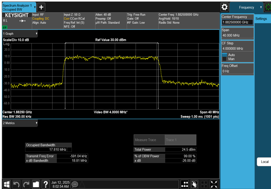
Plot 7-25. Occupied Bandwidth Plot (NR Band n25/n2 - 20MHz DFT-s-OFDM \pi/2 BPSK - Full RB)
