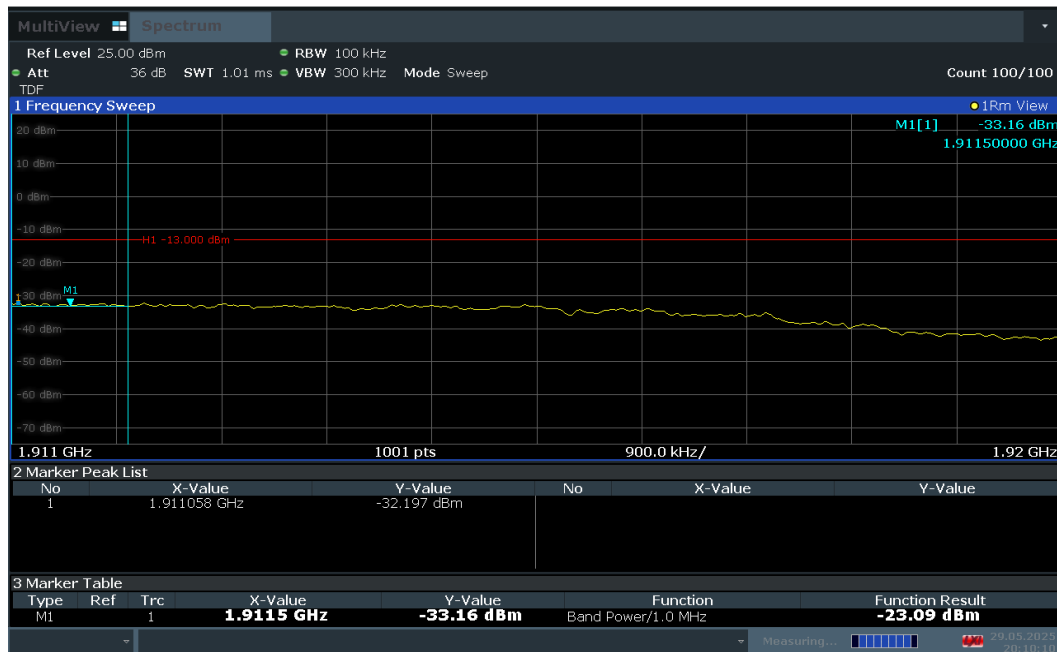
Plot 7-86. Extended Upper Band Edge Plot (LTE Band 2 – 10MHz QPSK – Full RB Configuration)
