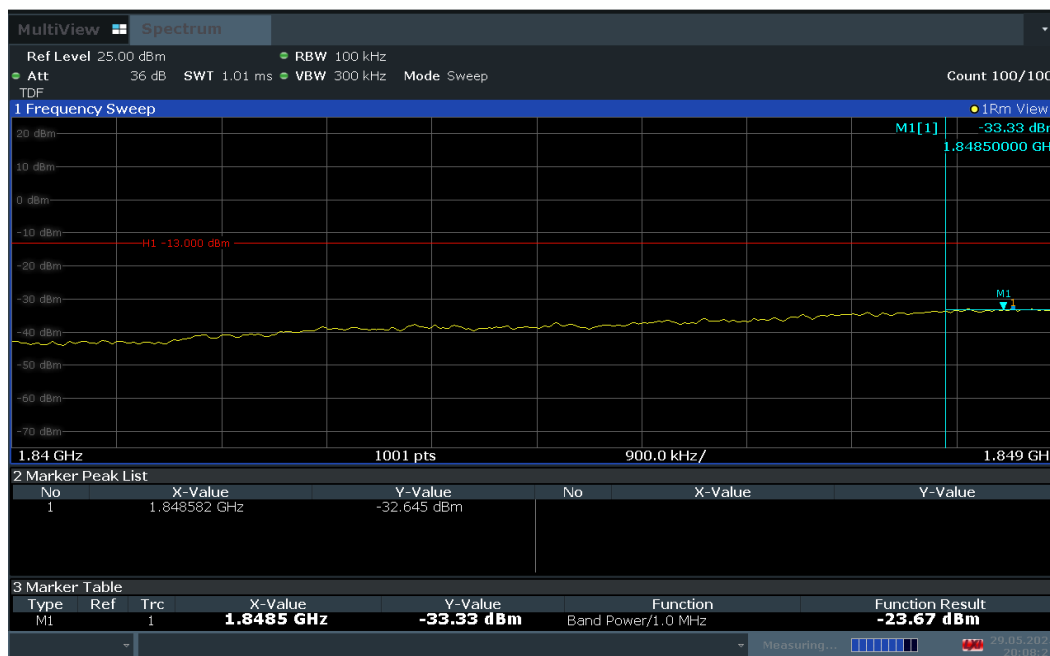
Plot 7-83. Extended Lower Band Edge Plot (LTE Band 2 – 10MHz QPSK – Full RB Configuration)
