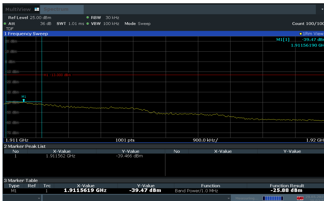
Plot 7-78. Extended Upper Band Edge Plot (LTE Band 2 – 3MHz QPSK – Full RB Configuration)
