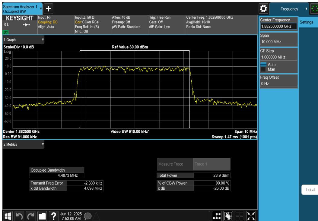
Plot 7-14. Occupied Bandwidth Plot (NR Band n25/n2 - 5MHz DFT-s-OFDM QPSK - Full RB)
