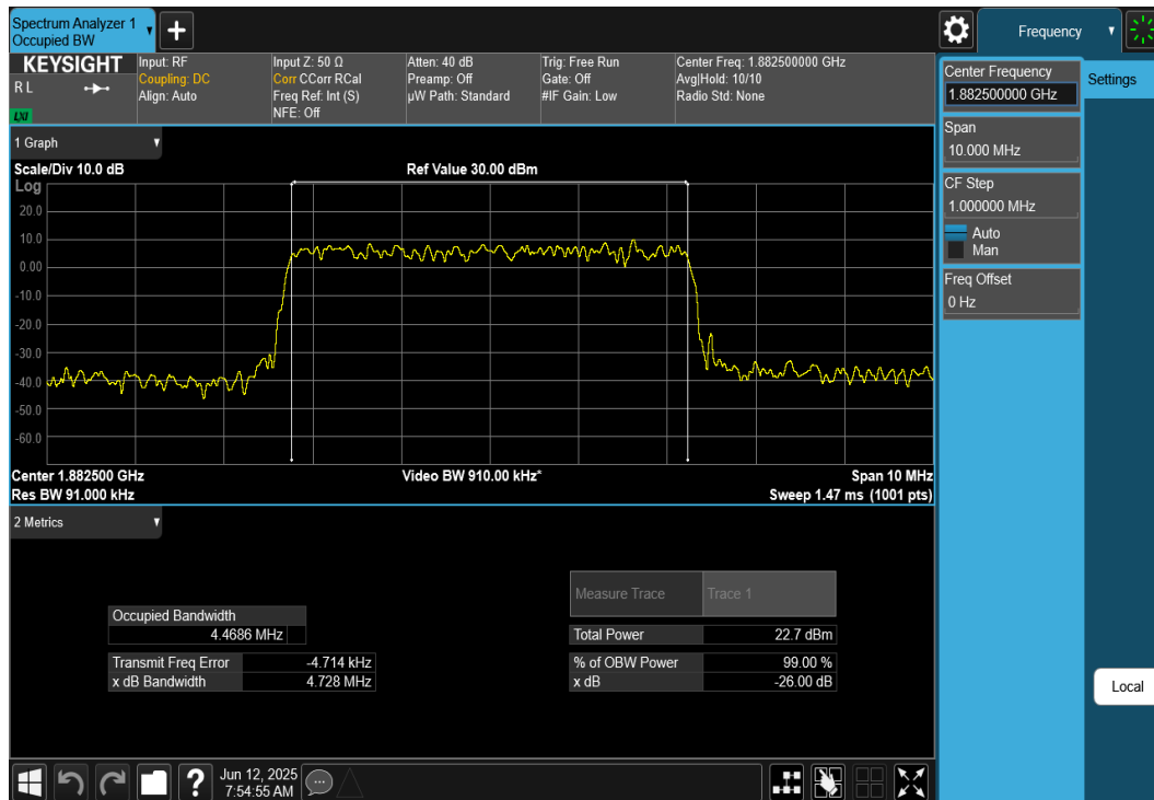
Plot 7-16. Occupied Bandwidth Plot (NR Band n25/n2 - 5MHz DFT-s-OFDM 64QAM - Full RB)
