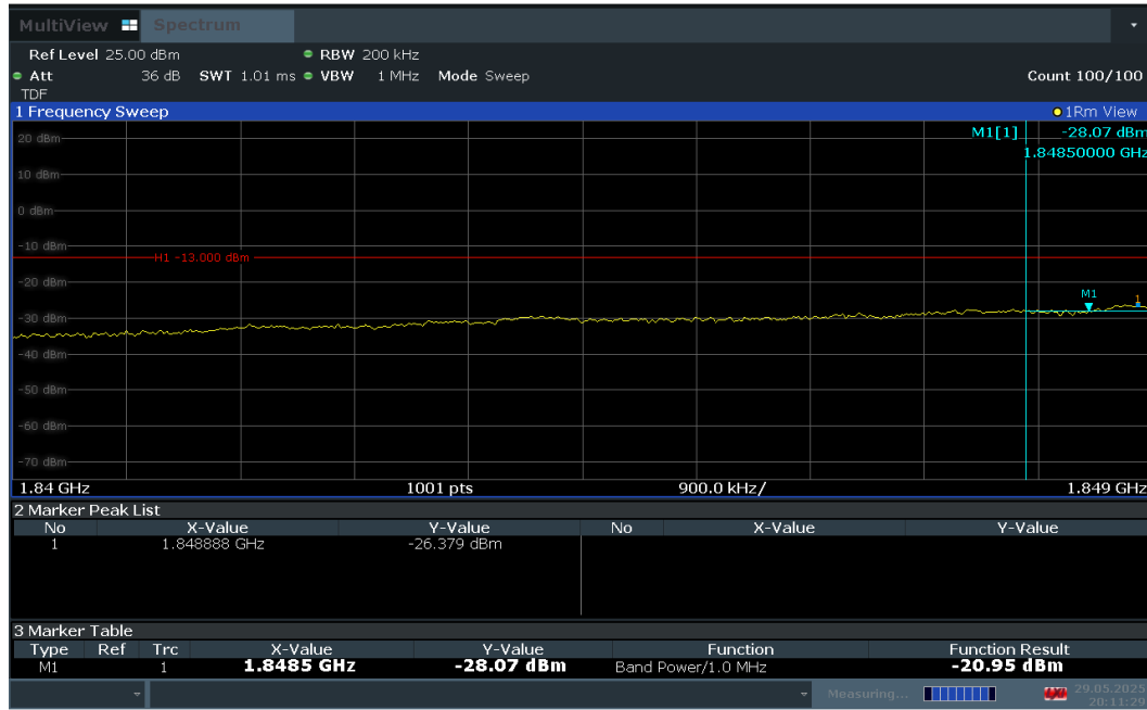
Plot 7-87. Extended Lower Band Edge Plot (LTE Band 2 – 15MHz QPSK – Full RB Configuration)
