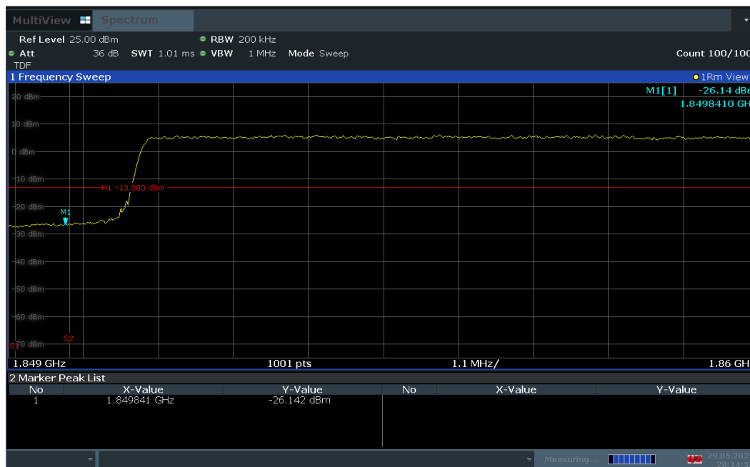
Plot 7-92. Lower Band Edge Plot (LTE Band 2 – 20MHz QPSK – Full RB Configuration)
