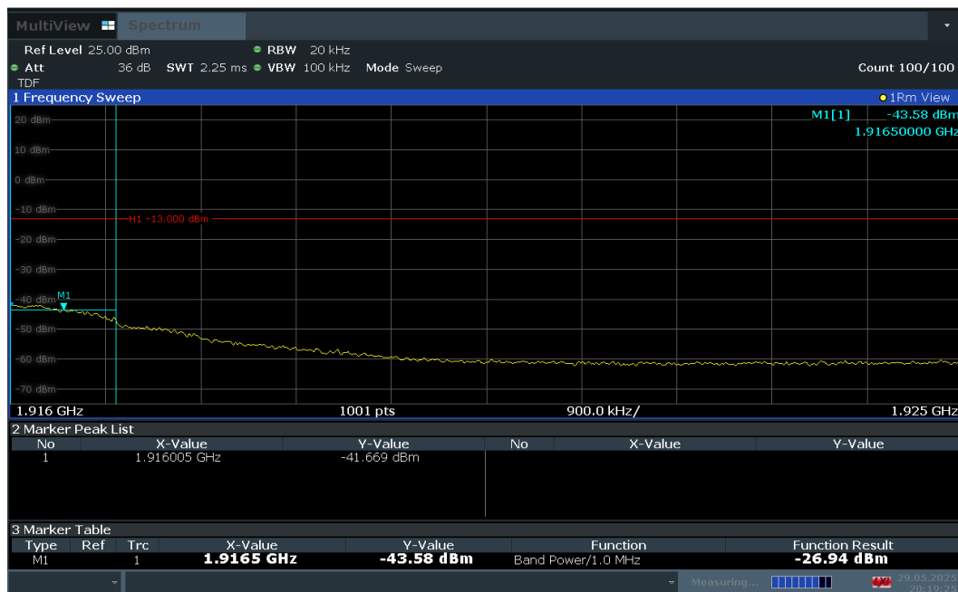
Plot 7-50. Extended Upper Band Edge Plot (LTE Band 25 – 1.4MHz QPSK – Full RB Configuration)
