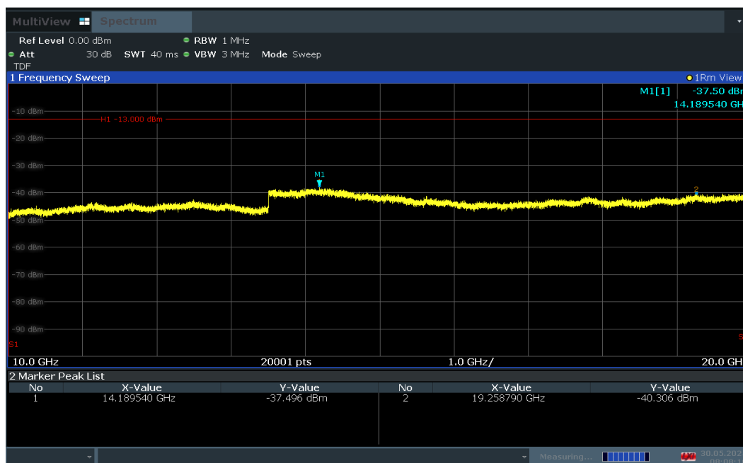
Plot 7-31. Conducted Spurious Plot (LTE Band 25/2 - 20MHz QPSK - RB Size 1, RB Offset 50 - Low Channel)
