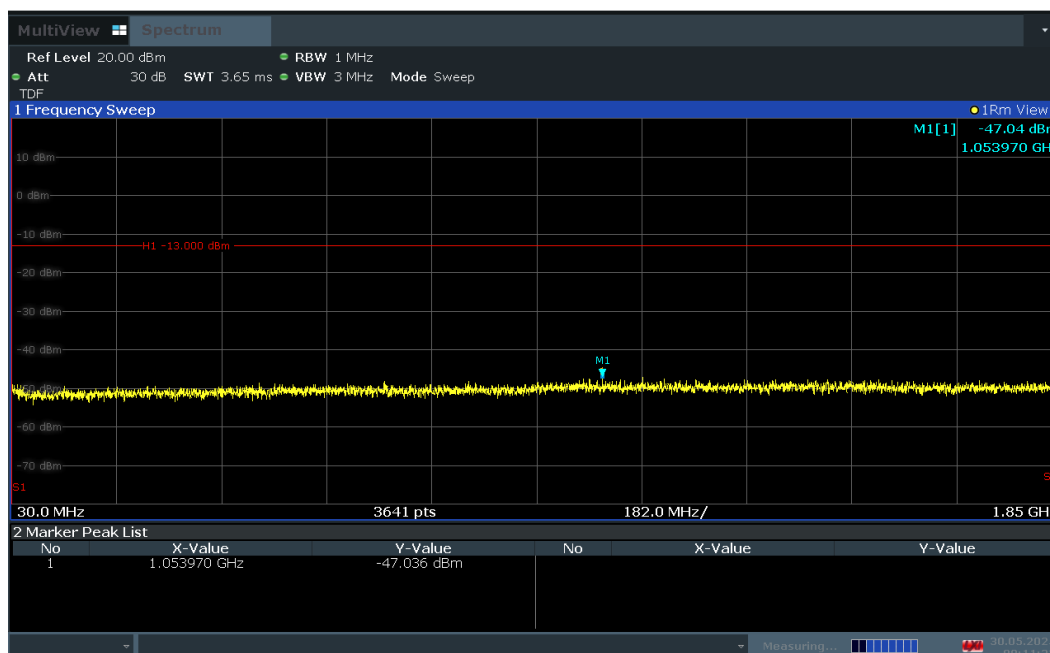
Plot 7-35. Conducted Spurious Plot (LTE Band 25/2 - 20MHz QPSK - RB Size 1, RB Offset 50 - High Channel)
