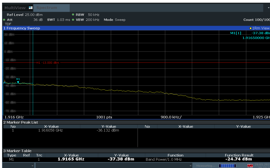
Plot 7-58. Extended Upper Band Edge Plot (LTE Band 25 – 5MHz QPSK – Full RB Configuration)
