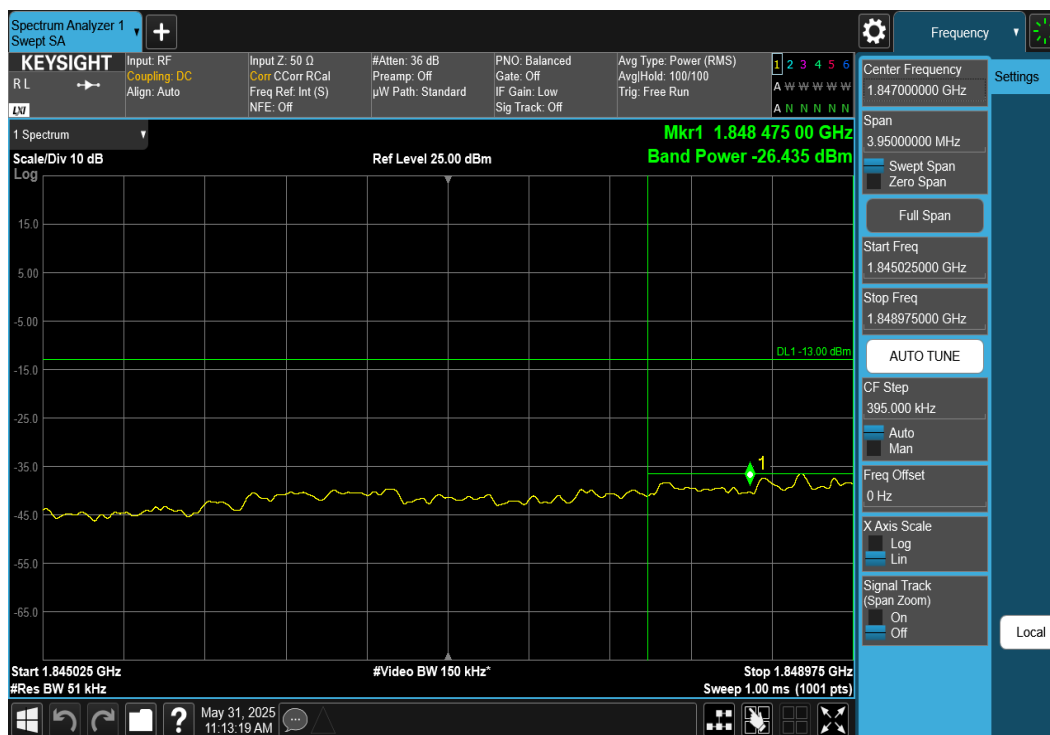
Plot 7-95. Extended Lower Band Edge Plot (NR Band n25 – 5MHz DFT-S-OFDM \pi/2 BPSK – Full RB Configuration)
