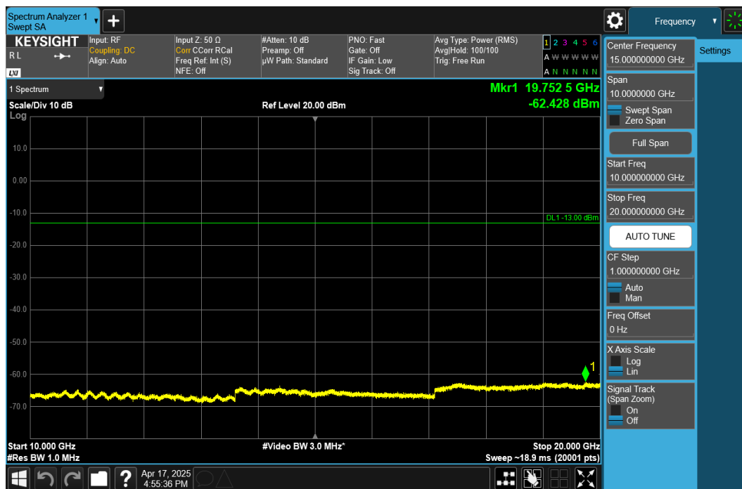
Plot 7-43. Conducted Spurious Plot (NR Band n25/n2 - 20MHz DFT-s-OFDM QPSK - RB Size 1, RB Offset 50 - Mid Channel)
