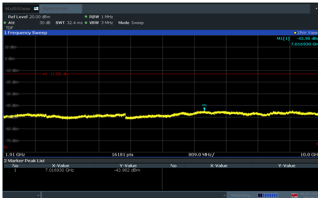
Plot 7-33. Conducted Spurious Plot (LTE Band 25/2 - 20MHz QPSK - RB Size 1, RB Offset 50 - Mid Channel)
