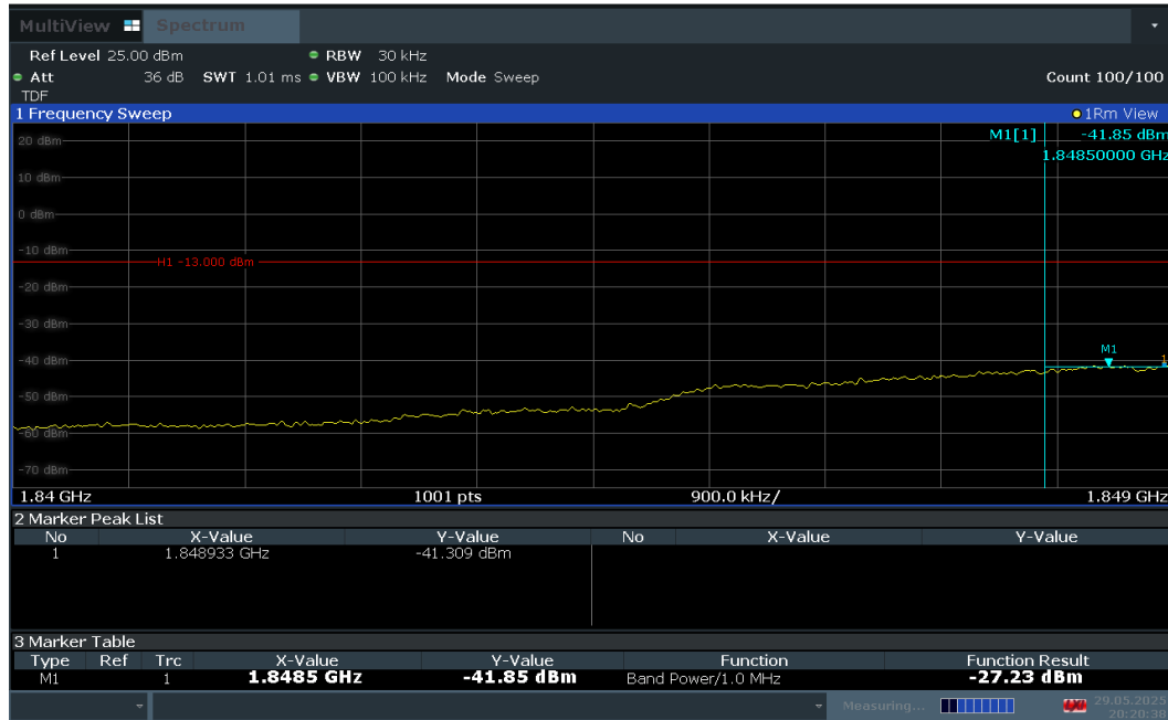
Plot 7-51. Extended Lower Band Edge Plot (LTE Band 25 – 3MHz QPSK – Full RB Configuration)
