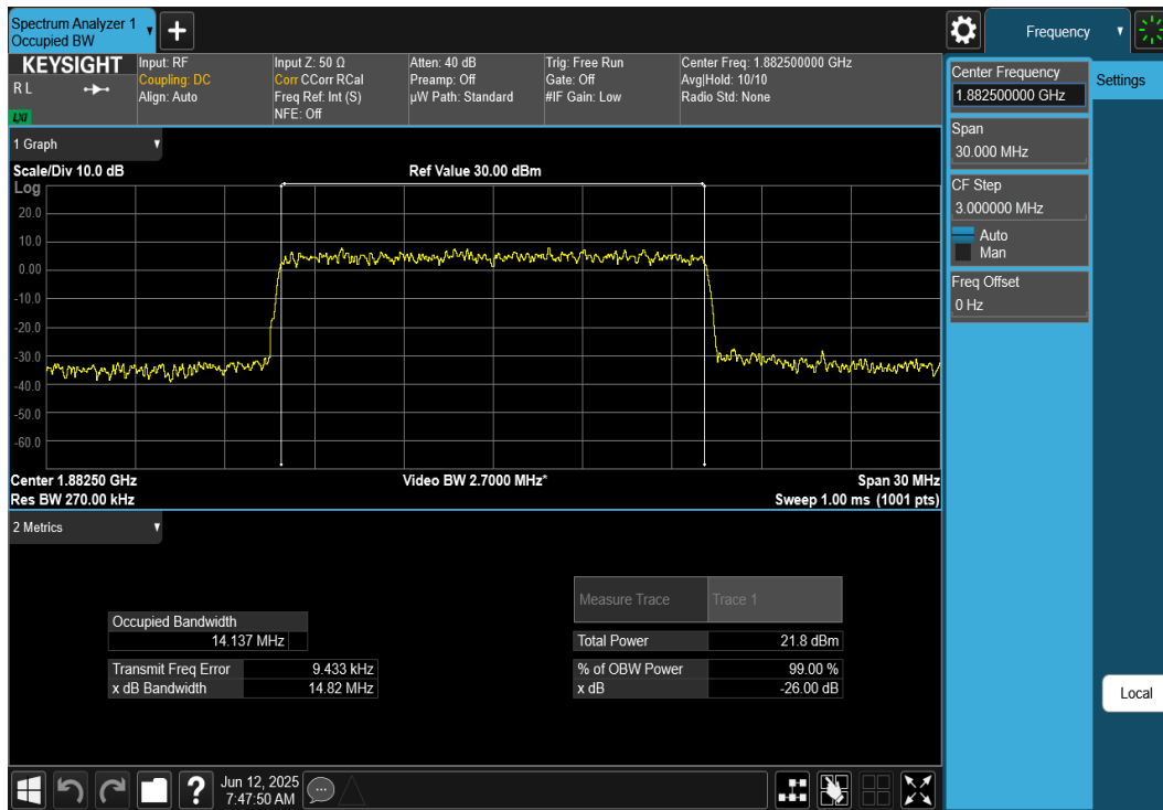
Plot 7-23. Occupied Bandwidth Plot (NR Band n25/n2 - 15MHz CP-OFDM 16QAM - Full RB)
