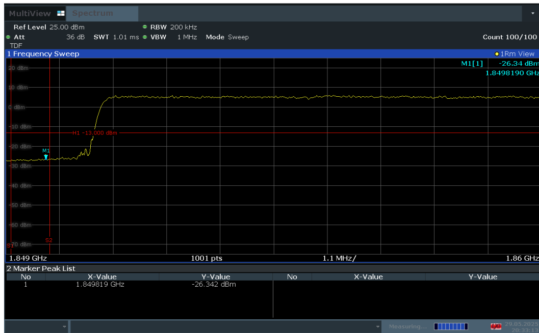
Plot 7-68. Lower Band Edge Plot (LTE Band 25 – 20MHz QPSK – Full RB Configuration)
