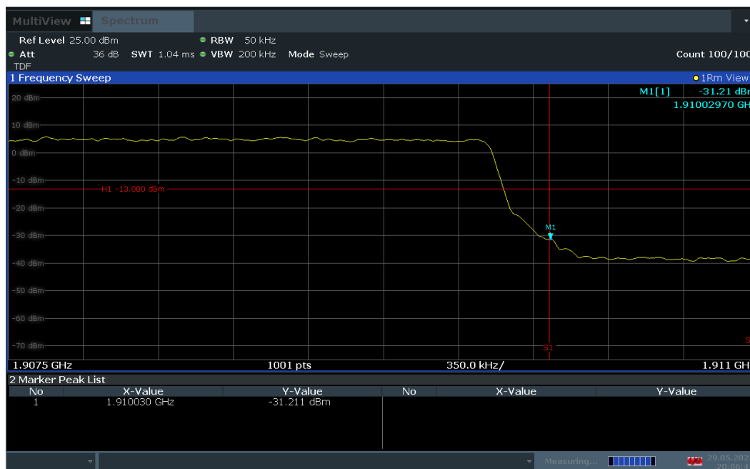
Plot 7-81. Upper Band Edge Plot (LTE Band 2 – 5MHz QPSK – Full RB Configuration)
