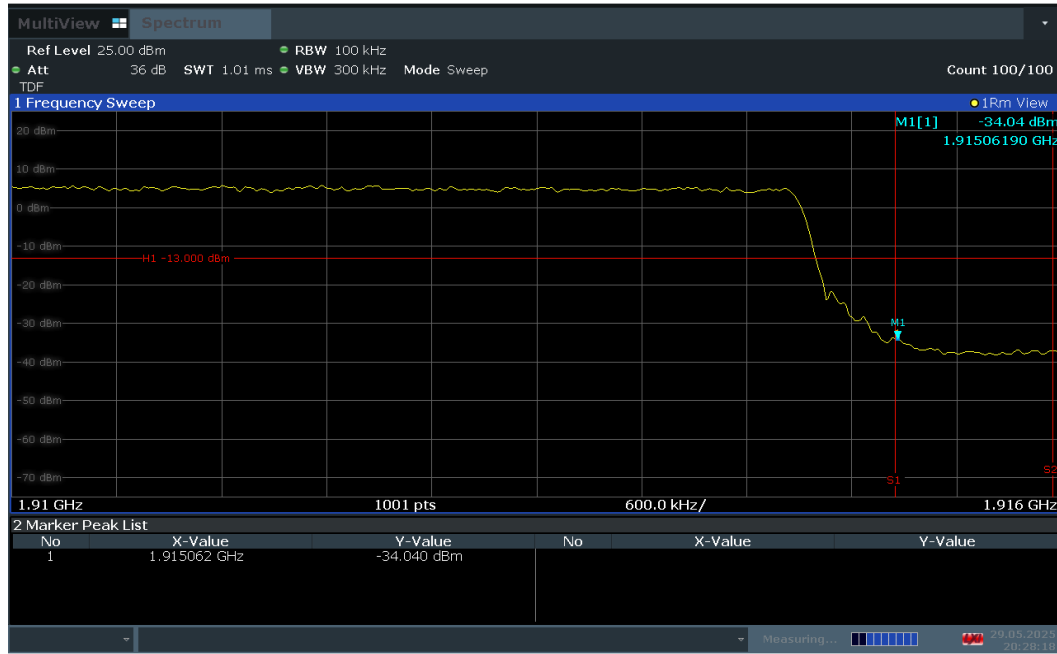
Plot 7-61. Upper Band Edge Plot (LTE Band 25 – 10MHz QPSK – Full RB Configuration)
