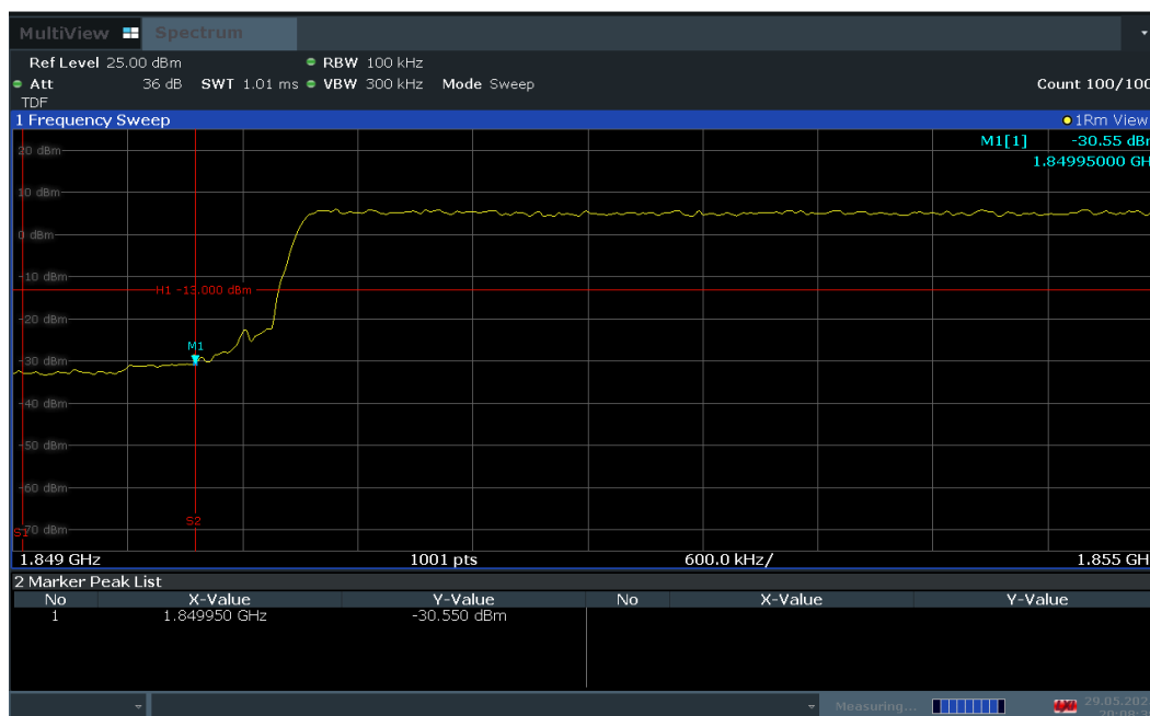
Plot 7-84. Lower Band Edge Plot (LTE Band 2 – 10MHz QPSK – Full RB Configuration)
