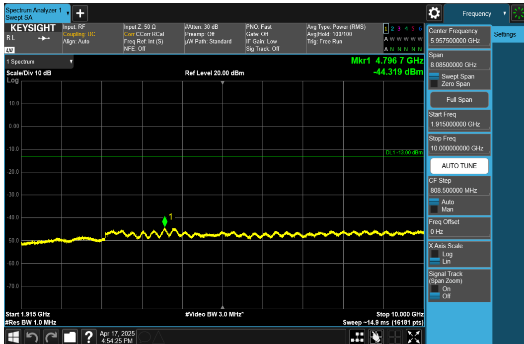
Plot 7-42. Conducted Spurious Plot (NR Band n25/n2 - 20MHz DFT-s-OFDM QPSK - RB Size 1, RB Offset 50 - Mid Channel)
