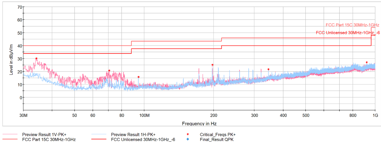
Plot 7-58. Radiated Spurious Emissions Below 1GHz – Simultaneous Transmission
