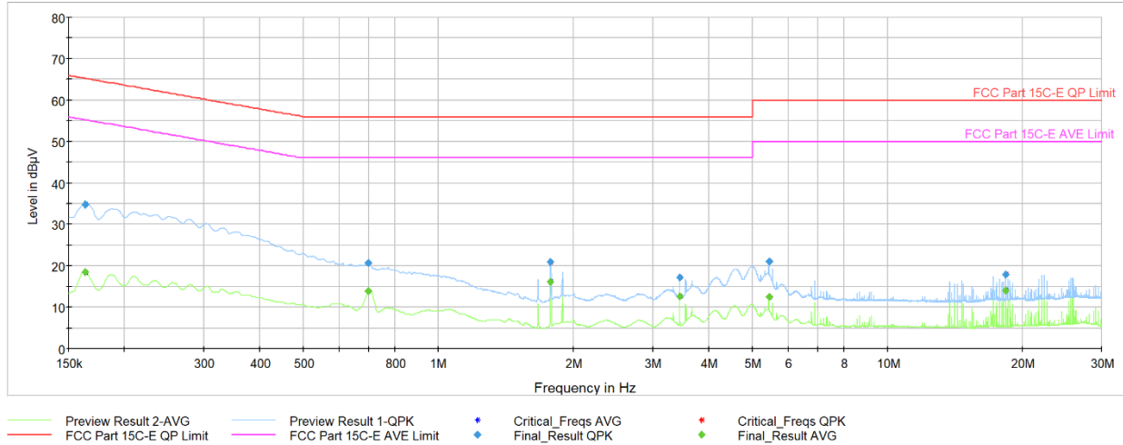
Plot 7-60. AC Line Conducted Plot with 802.11n Ch.64 (N), with AC/DC adapter & magnetic charger
