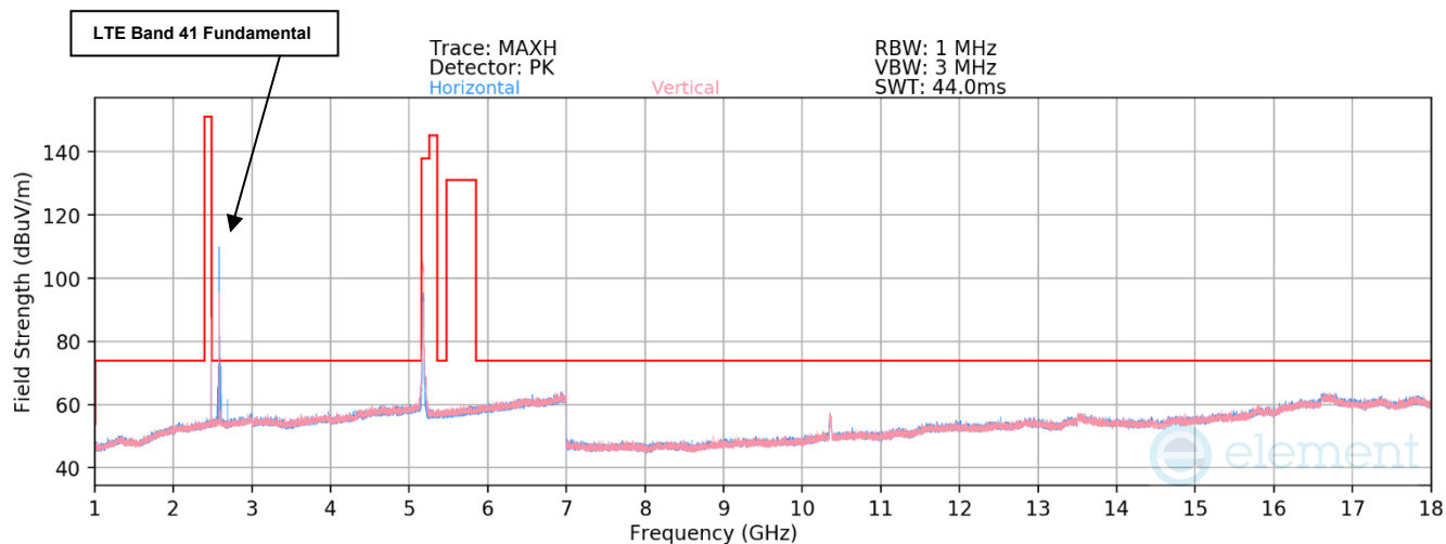
Plot 7-41. Radiated Spurious Emissions 1 - 18GHz – Simultaneous Transmission
