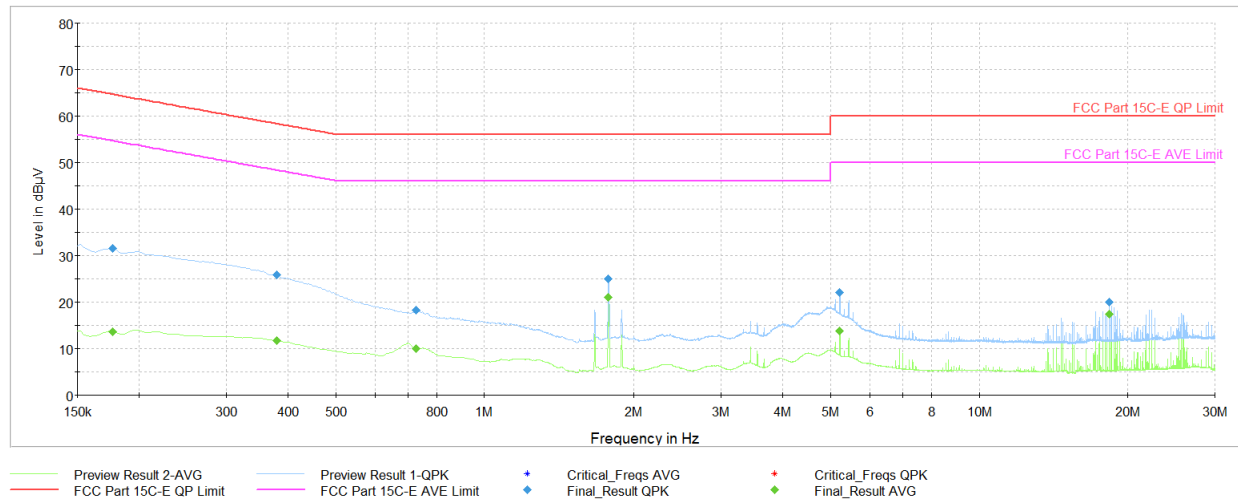
Plot 7-30. AC Line Conducted Plot (O-QPSK, 250Kbps – Ch. 24) (L1) with AC/DC Adapter & magnetic charger
