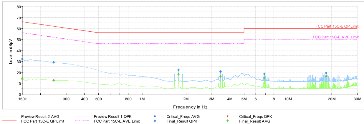
Plot 7-38. AC Line Conducted Plot with Bluetooth HDR (L1, 4Mbps ePA - Ch.38 with AC/DC adaptor via USB-C cable with magnetic charger)
