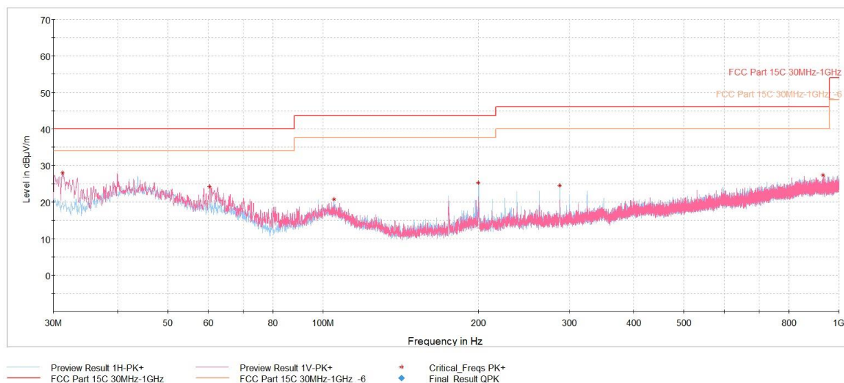
Plot 7-37. Radiated Spurious Emissions Below 1GHz (1Mbps, ePA – Ch.19, Pol. H & V, with AC/DC adaptor via USB-C cable with magnetic charger)
