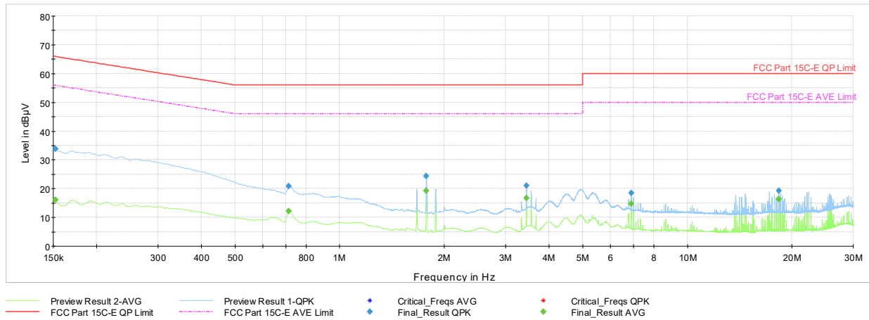
Plot 7-38. AC Line Conducted Plot with Bluetooth LE (L1, 1Mbps ePA – Ch.19 with AC/DC adaptor via USB-C cable with magnetic charger)
