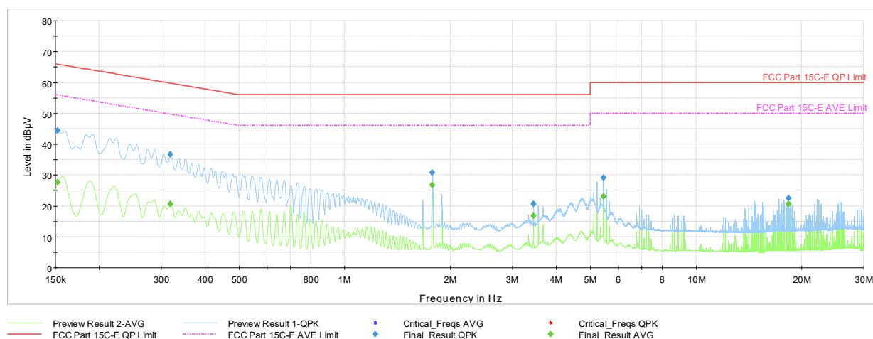
Plot 7-44. AC Line-Conducted Test Plot (N, GFSK ePA – Ch.39, with AC/DC Adapter + Magnetic Charger)
