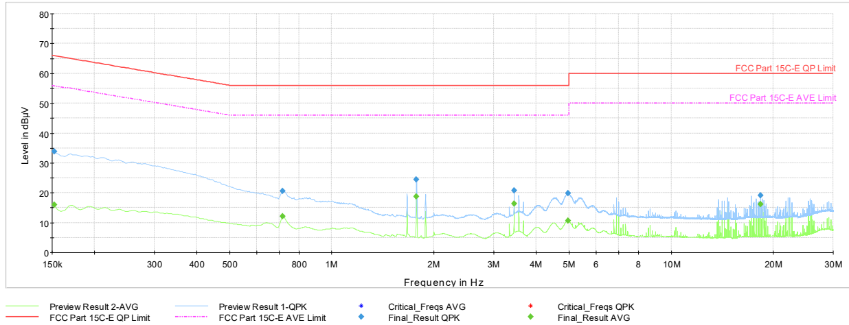
Plot 7-43. AC Line-Conducted Test Plot (L1, GFSK ePA – Ch.39, with AC/DC Adapter + Magnetic Charger)
