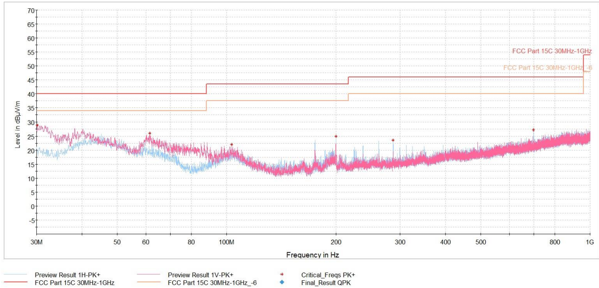
Plot 7-41. Radiated Spurious Emissions Below 1GHz (GFSK ePA – Ch.39, with AC/DC Adapter & Magnetic Charger)
