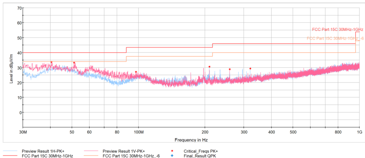
Plot 7-11. Radiated Spurious Emissions 30MHz – 1GHz (Reader A 848kbps, with AC/DC Adapter and Magnetic Charger)
