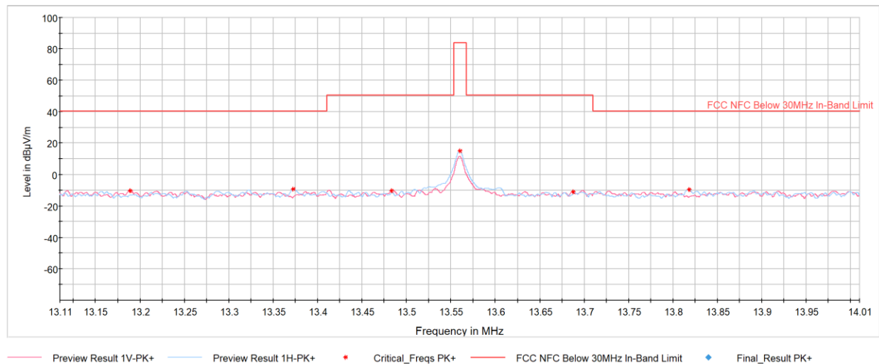
Plot 7-6. In Band Radiated Spurious Emissions (CE F 424kbps, with AC/DC Adapter and Magnetic Charger)
