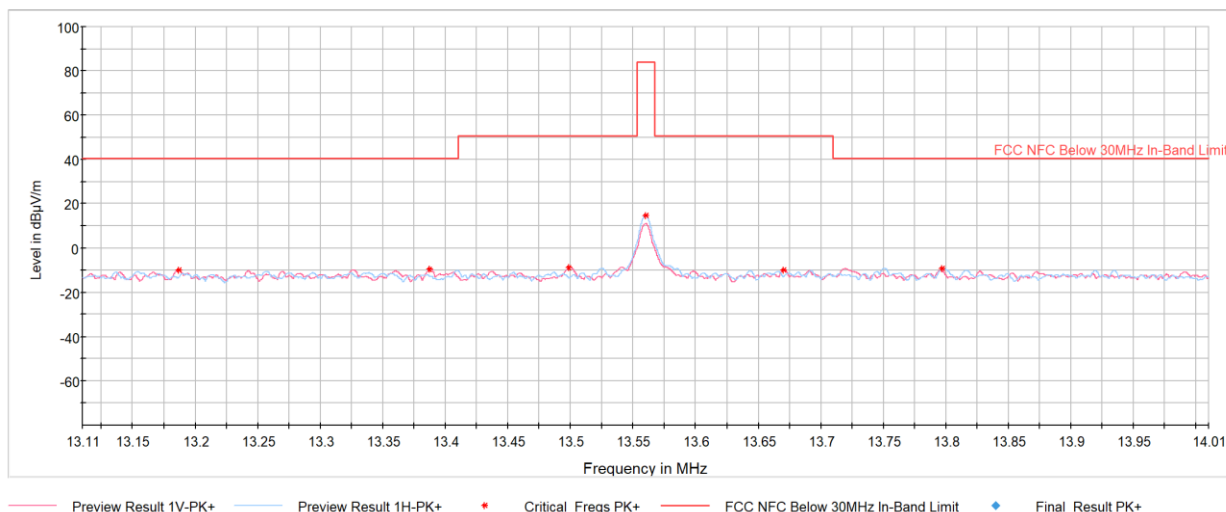
Plot 7-6. In Band Radiated Spurious Emissions (CE F 424kbps, with AC/DC Adapter and Magnetic Charger)
