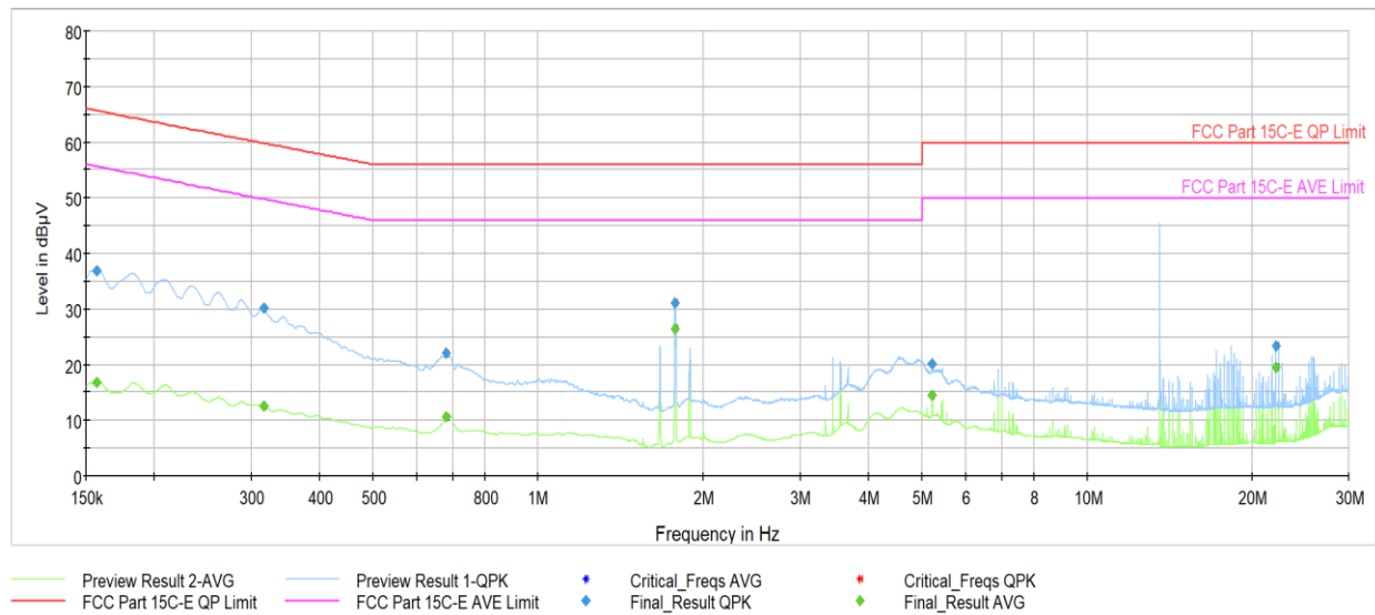
Plot 7-12. AC Line-Conducted Plot (L1, CE F 424kbps, with AC/DC Adapter and Magnetic Charger)
