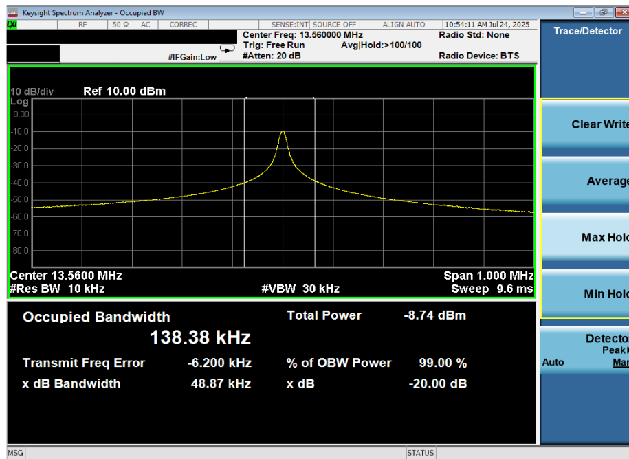
Plot 7-2. 20dB and 99% Bandwidth Plot (CE F 106kbps)
