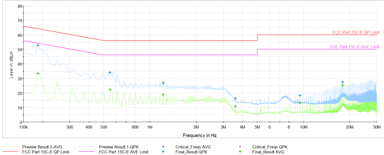
Plot 6-14. AC Line Conducted Plot (N - Mode 1, with Host Laptop via USB-C Cable)
