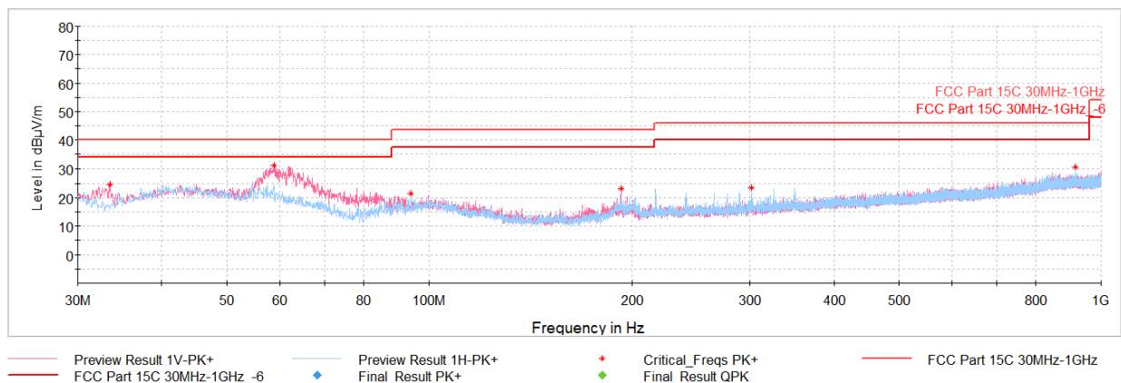
Plot 6-12. Radiated Spurious Emissions 30MHz – 1GHz (Mode 1, with Host Laptop via USB-C Cable)
