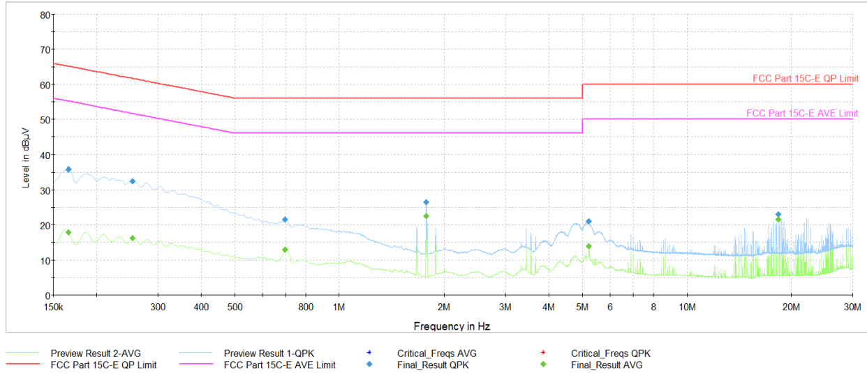
Plot 7-38. AC Line Conducted (Ch. 5, Config 9, Payload 65B N, with AC/DC Adapter + Magnetic Charger)
