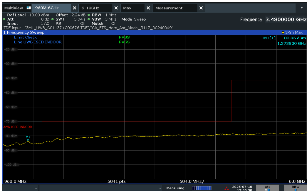
Plot 7-17. ISD Radiated Spurious Emission 960-6000MHz (Ch. 5, Config 9, Payload 65B Ant. Pol. H)
