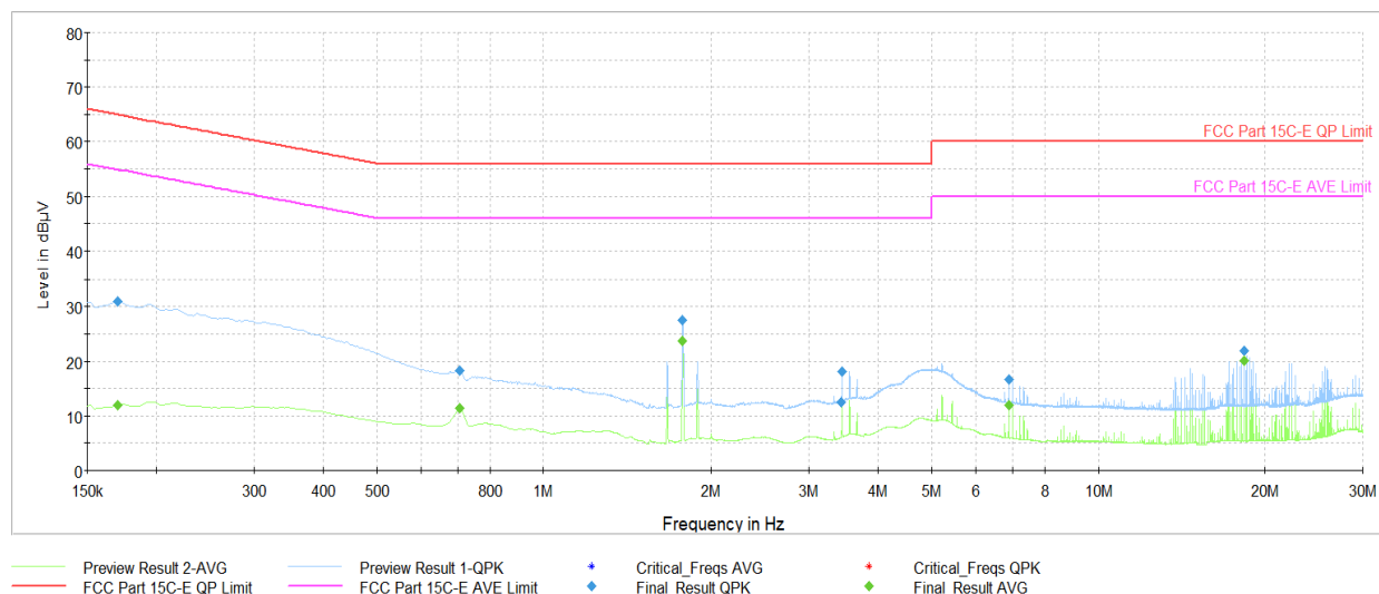
Plot 7-40. AC Line Conducted Plot (Ch. 9, Config 9, Payload 65B N, with AC/DC Adapter + Magnetic Charger)
