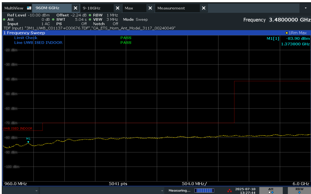
Plot 7-18. ISD Radiated Spurious Emission 960-6000MHz (Ch. 5, Config 9, Payload 65B Ant. Pol. V)
