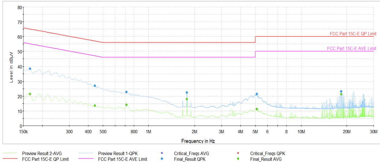
Plot 7-37. AC Line Conducted (Ch. 5, Config 9, Payload 65B L1, with AC/DC Adapter + Magnetic Charger)
