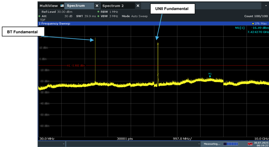
Plot 7-29. Conducted Simultaneous Tx Spurious Plot
