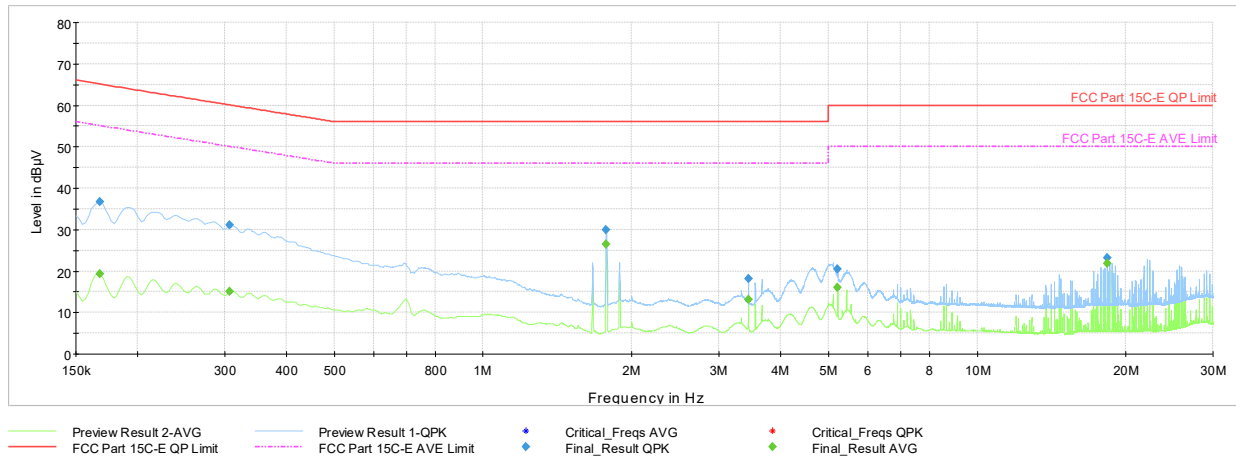
Plot 7-44. AC Line-Conducted Test Plot (N, GFSK ePA – Ch.39, with AC/DC adaptor via USB-C cable with magnetic charger)
