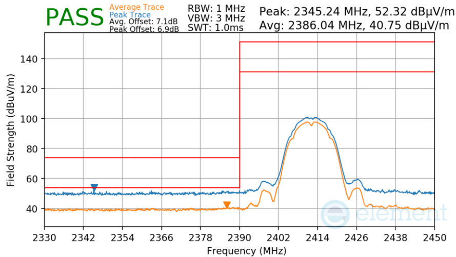
Plot 7-55. Radiated Restricted Lower Band Edge Measurement
