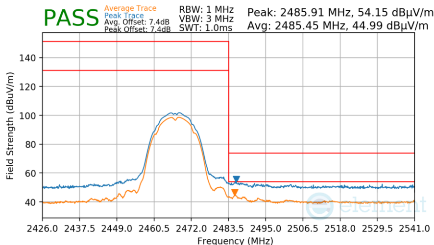
Plot 7-56. Radiated Restricted Upper Band Edge Measurement
