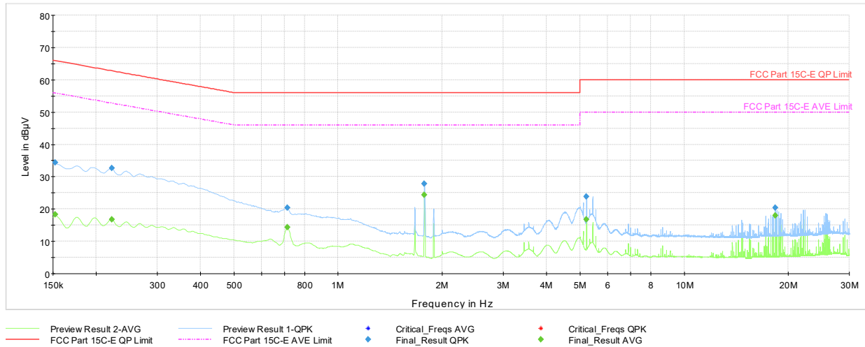
Plot 7-70. AC Line Conducted Plot 802.11b - Ch.6 (L1, with AC/DC adaptor via USB-C cable with magnetic charger)
