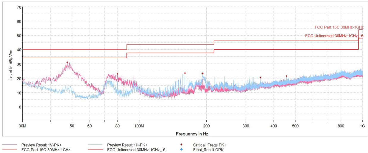
Plot 7-69. Radiated Spurious Emissions below 1GHz 11b Ch.6, with AC/DC Adapter via USB-C cable with magnetic charger
