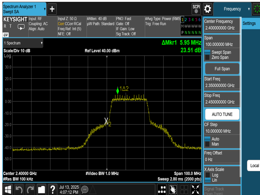
Plot 7-34. Band Edge Plot (802.11n (2.4GHz) – Ch. 1) – MCS0
