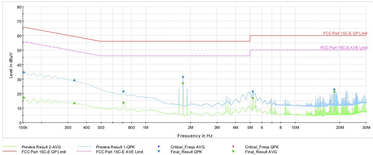
Plot 7-39. AC Line Conducted Plot with Bluetooth LE (N, 1Mbps ePA – Ch.19, with AC/DC adaptor via USB-C cable with magnetic charger)
