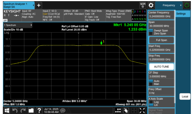
Plot 7-18. ISD PSD (20MHz BW 802.11n - Ch. 48, MCS0)
