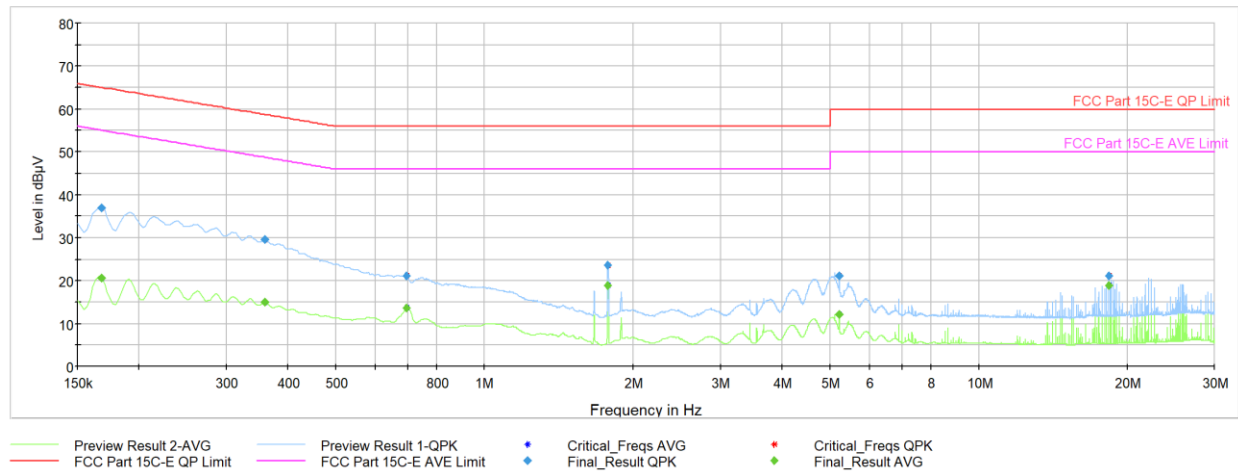
Plot 7-59. AC Line Conducted Plot with 802.11n Ch.157 (L1), with AC/DC adapter & magnetic charger
