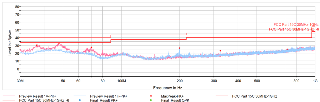
Plot 7-57. Radiated Spurious Emissions below 1GHz, 802.11n, Ch. 157 with AC/DC Adapter & magnetic charger
