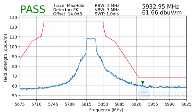
Plot 7-56. (Pk & Avg, Ch.165, 802.11n, MCS7)
