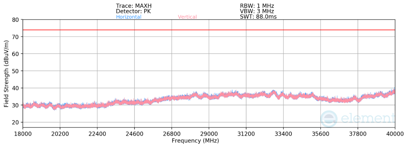
Plot 7-42. Radiated Spurious Emissions Above 18GHz Simultaneous Transmission Configuration
