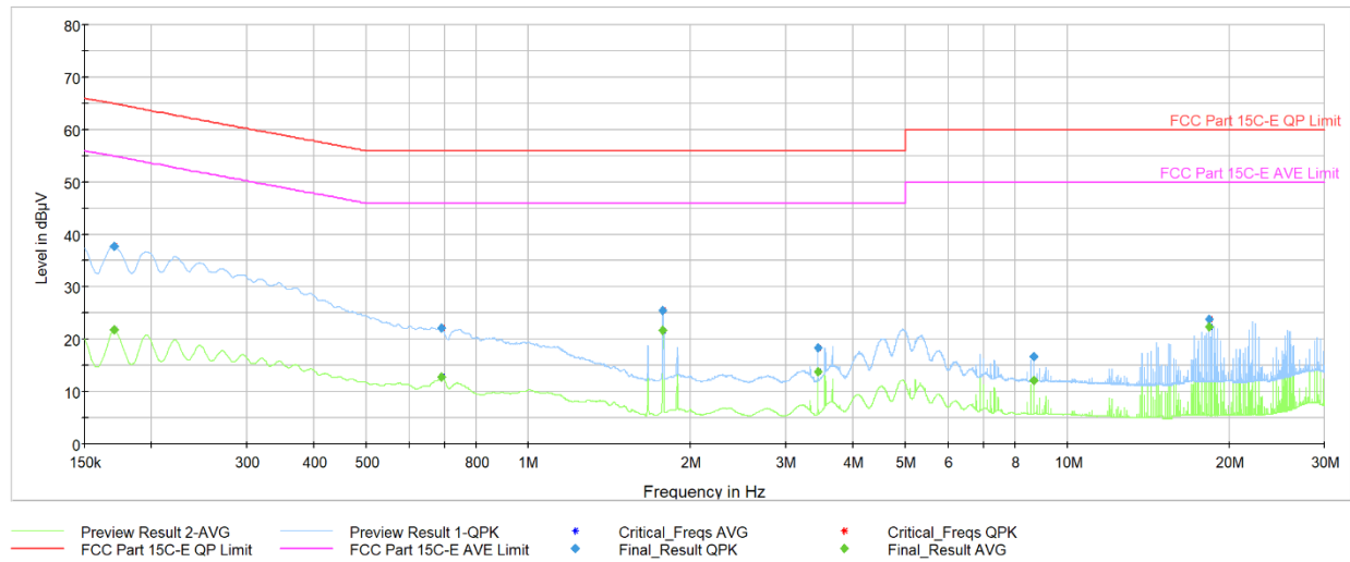
Plot 7-60. AC Line Conducted Plot with 802.11n Ch.157 (N), with AC/DC & magnetic charger
