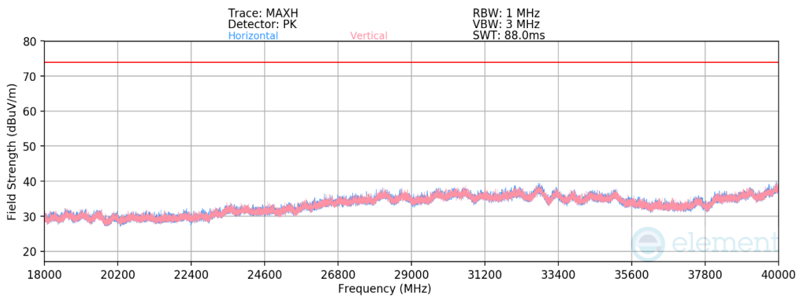
Plot 7-39. Radiated Emissions 18GHz-40GHz (802.11n – Ch. 157)
