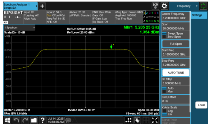
Plot 7-17. ISD PSD (20MHz BW 802.11n - Ch. 40, MCS0)
