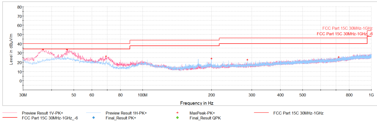
Plot 7-29. RSE 30MHz - 1GHz (O-QPSK, 250Kbps – Ch. 24), with AC/DC Adapter & magnetic charger
