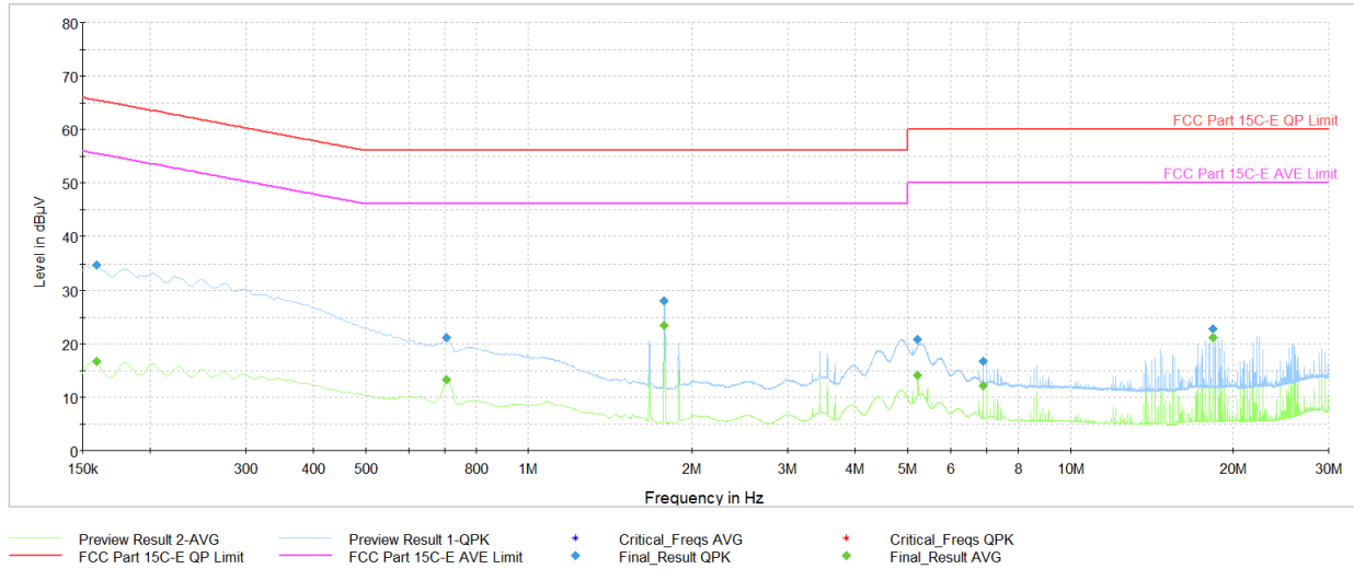
Plot 7-31. AC Line Conducted Plot (O-QPSK, 250Kbps – Ch. 24) (N) with AC/DC Adapter & magnetic charger
