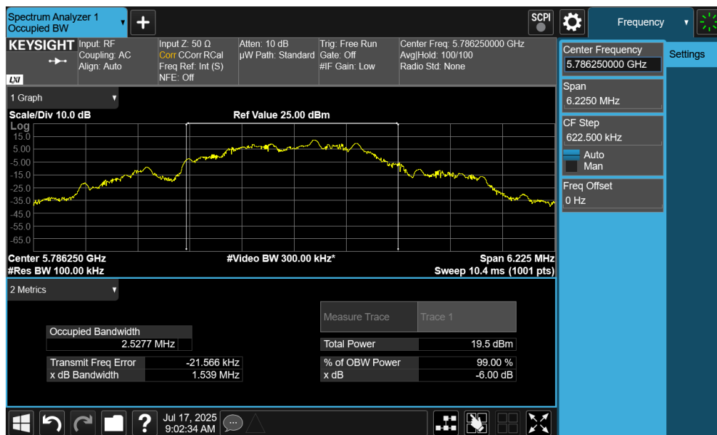
Plot 7-8. 6dB BW & 99% OBW (O-QPSK, 5786.25MHz, 1000kpbs)
