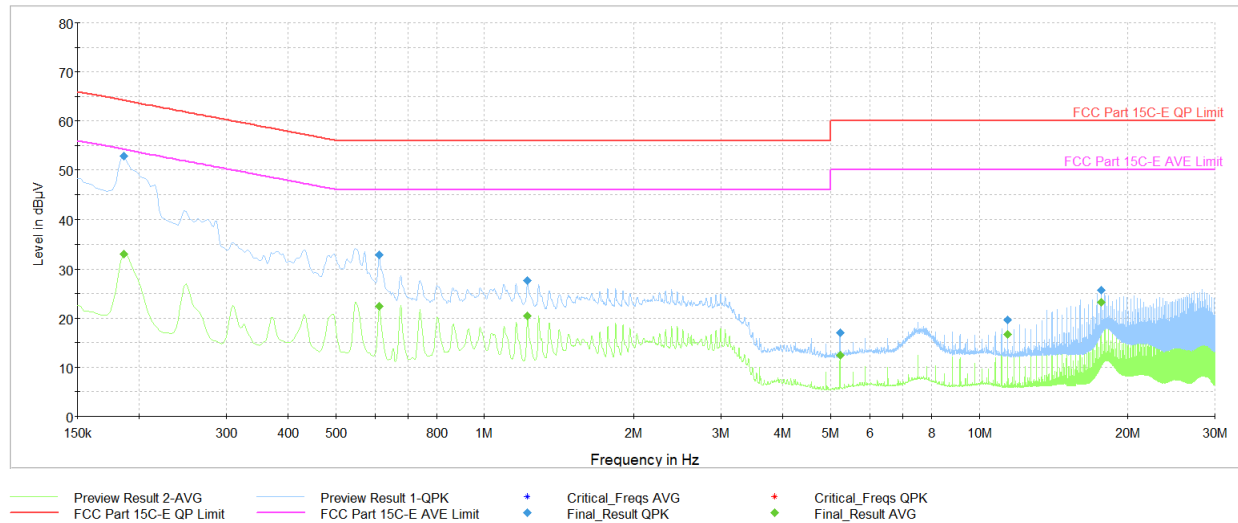
Plot 6-14. AC Line Conducted Plot (N - Mode 1, with Host Laptop via USB-C Cable)
