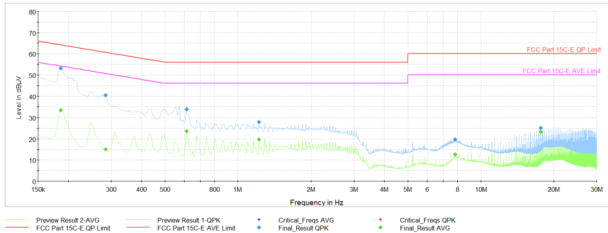
Plot 6-13. AC Line Conducted Plot (L1 - Mode 1, with Host Laptop via USB-C Cable)
