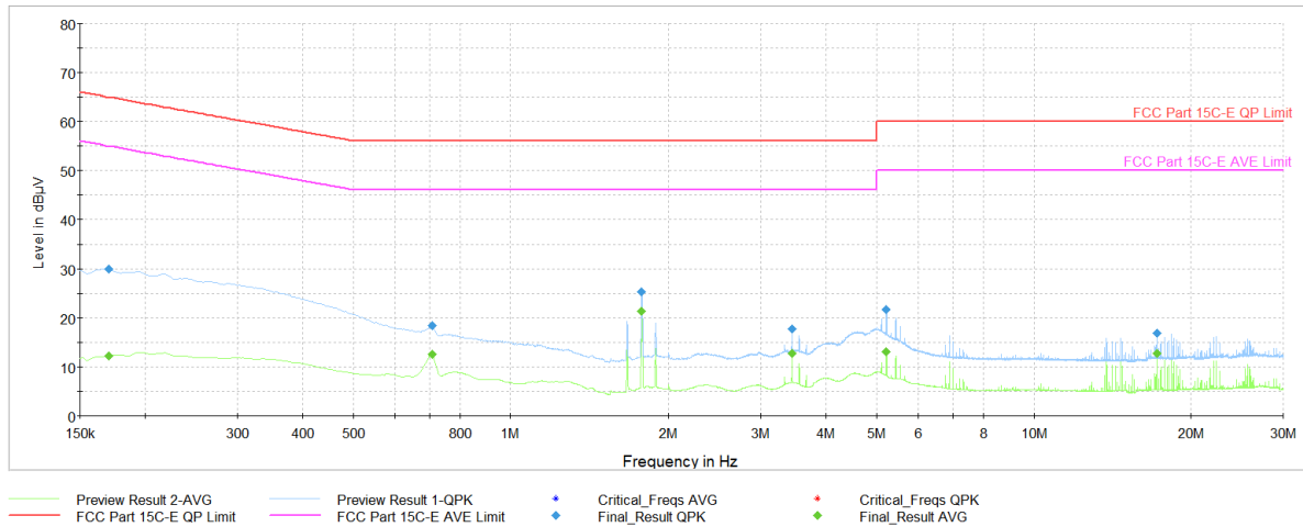
Plot 7-38. AC Line Conducted (Ch. 5, Config 16, Payload 65B N, with AC/DC Adapter + Magnetic Charger)
