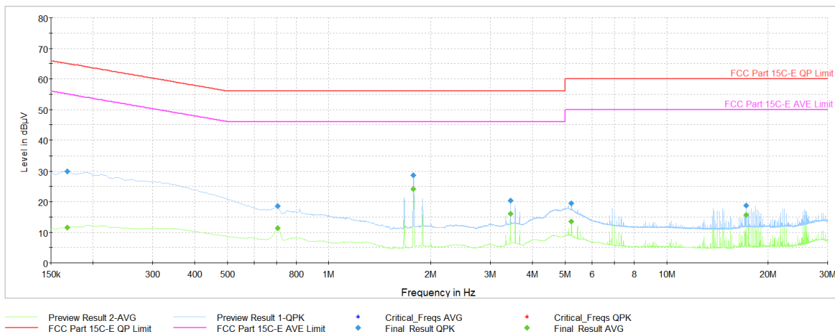
Plot 7-37. AC Line Conducted (Ch. 5, Config 16, Payload 65B L1, with AC/DC Adapter + Magnetic Charger)
