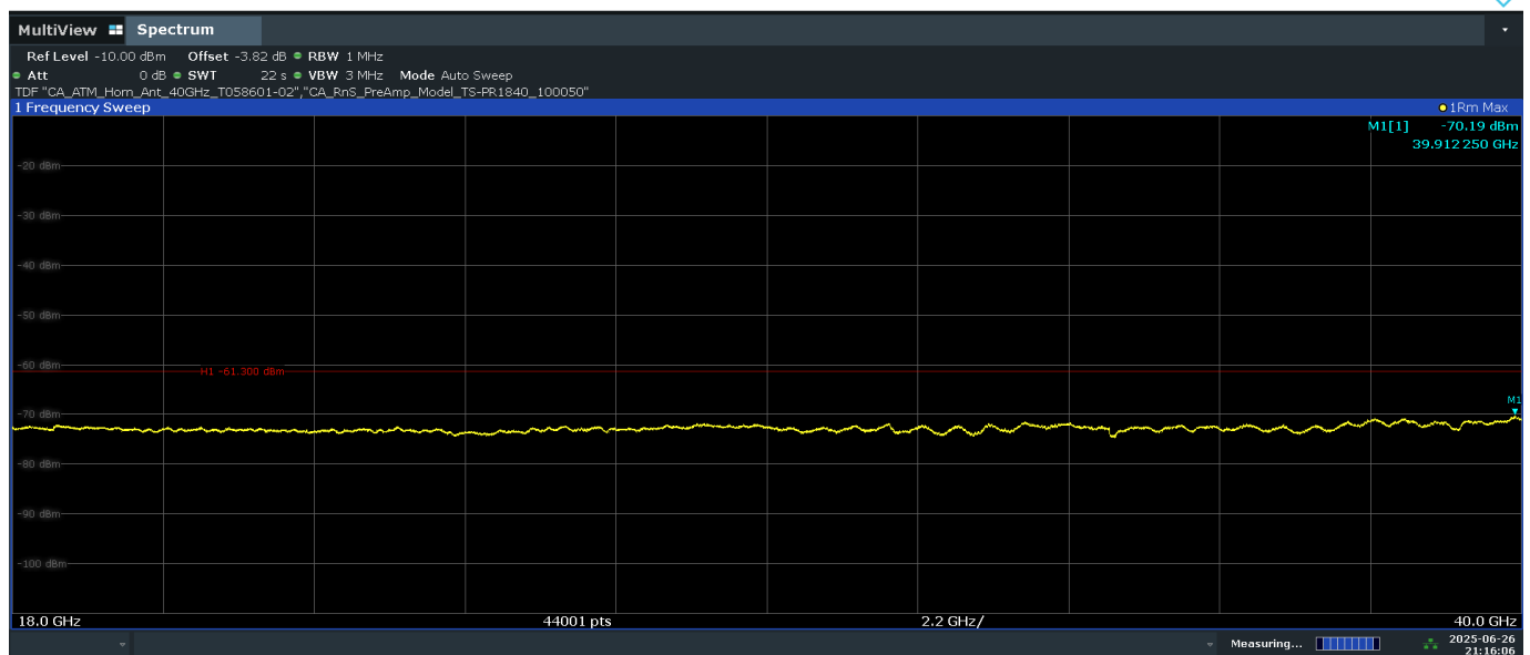
Plot 7-32. Radiated Spurious Emission 18-40GHz (Ch. 5, Config 16, Payload 65B Ant. Pol. V)
