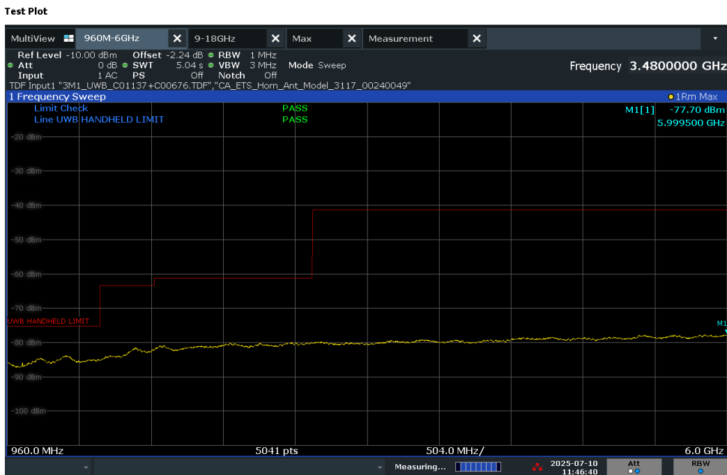
Plot 7-24. FCC Radiated Spurious Emission 960-6000MHz (Ch.9, Config 9, Payload 65B Ant. Pol. V)
