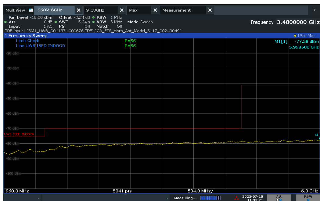
Plot 7-26. ISD Radiated Spurious Emission 960-6000MHz (Ch.9, Config 9, Payload 65B Ant. Pol. V)
