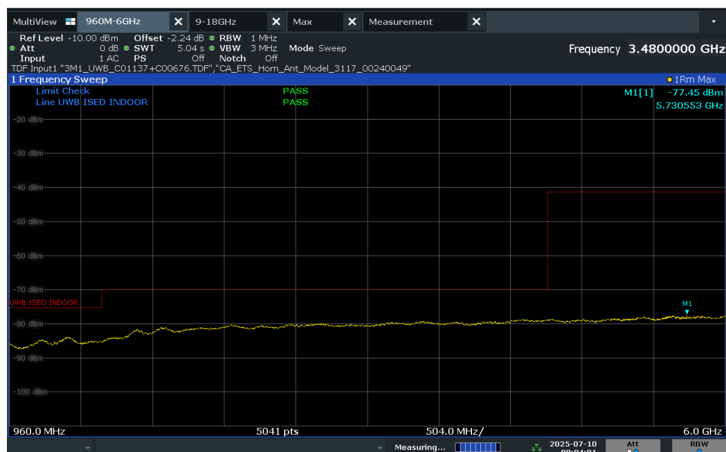
Plot 7-17. ISD Radiated Spurious Emission 960-6000MHz (Ch. 5, Config 16, Payload 65B Ant. Pol. H)
