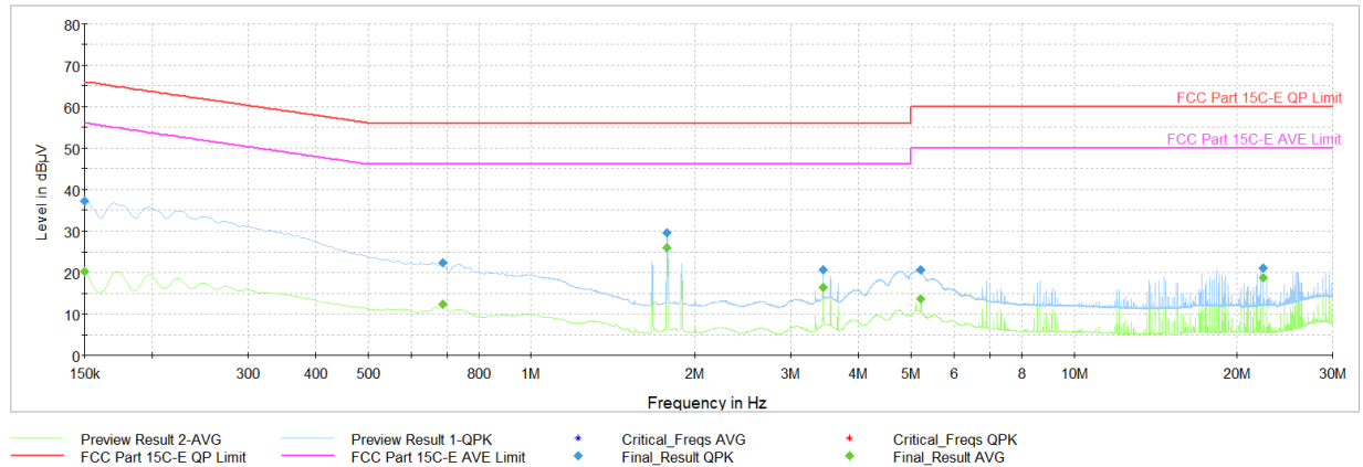
Plot 7-39. AC Line Conducted (Ch. 9, Config 9, Payload 65B L1, with AC/DC Adapter + Magnetic Charger)
