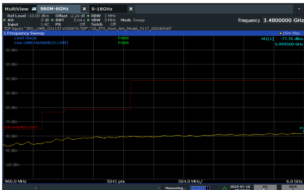
Plot 7-16. FCC Radiated Spurious Emissions 960-6000MHz (Ch. 5, Config 16, Payload 65B Ant. Pol. V)
