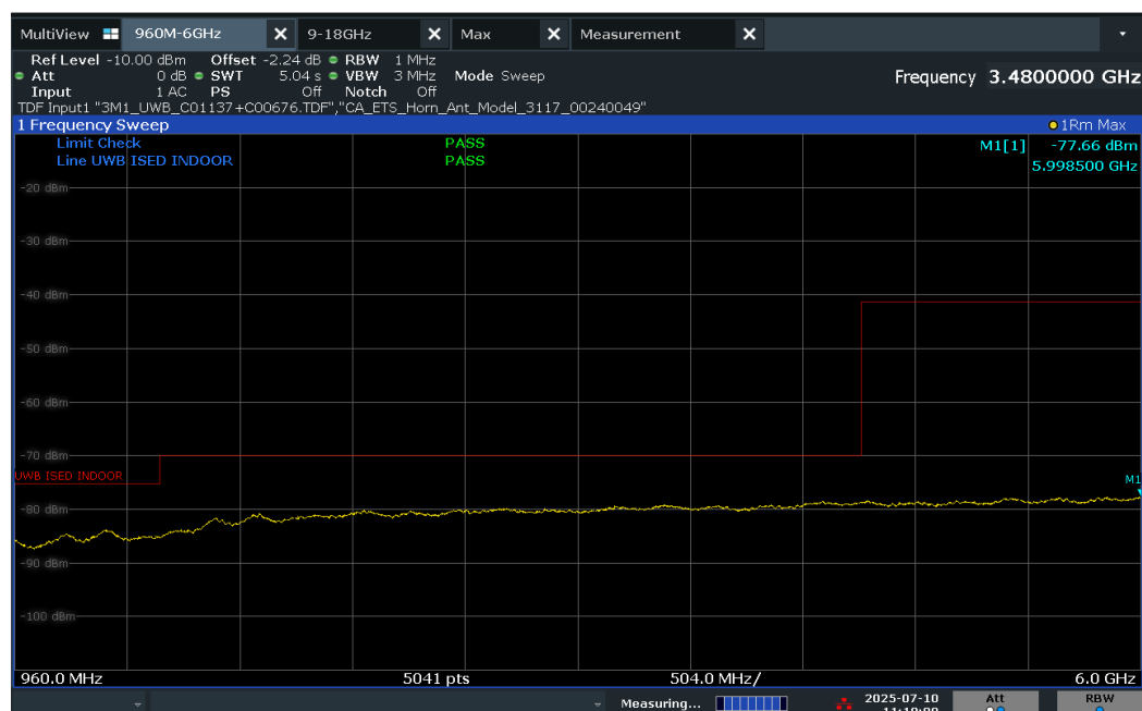
Plot 7-25. ISD Radiated Spurious Emission 960-6000MHz (Ch. 9, Config 9, Payload 65B Ant. Pol. H)
