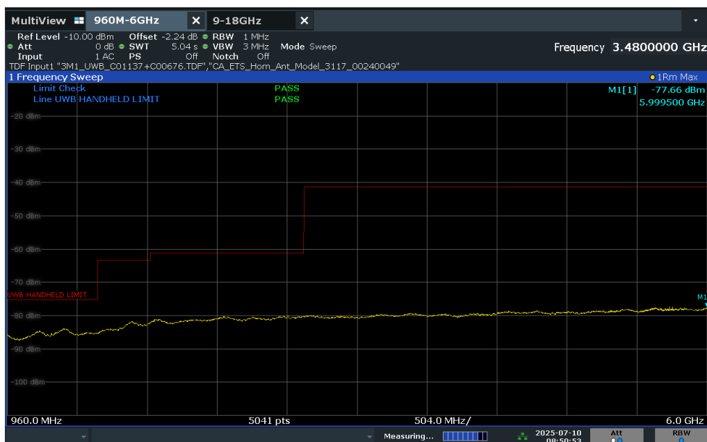
Plot 7-15. FCC Radiated Spurious Emission 960-6000MHz (Ch. 5, Config 16, Payload 65B Ant. Pol. H)
