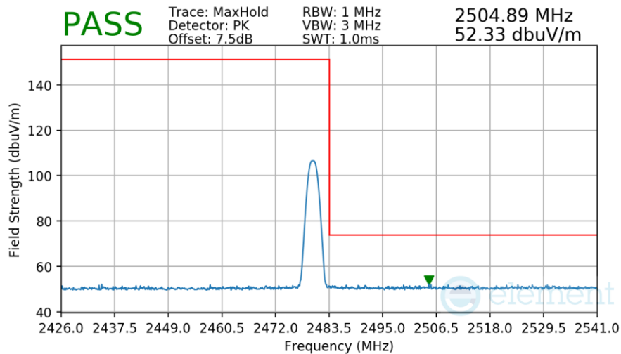
Plot 7-39. Radiated Restricted Upper Band Edge Measurement
