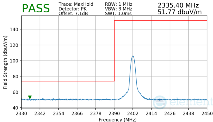
Plot 7-38. Radiated Restricted Lower Band Edge Measurement
