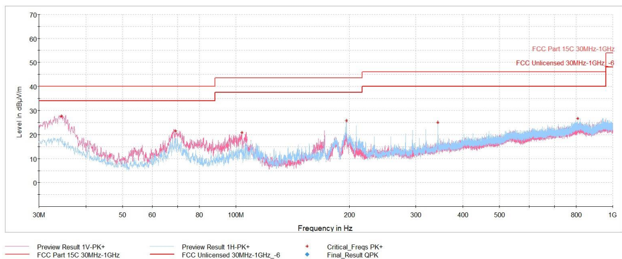
Plot 7-41. Radiated Spurious Emissions Below 1GHz (GFSK ePA – Ch.39, with AC/DC adaptor via USB-C cable with magnetic charger)
