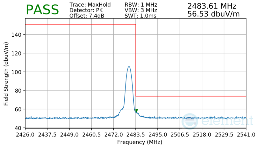
Plot 7-40. Radiated Restricted Upper Band Edge Measurement
