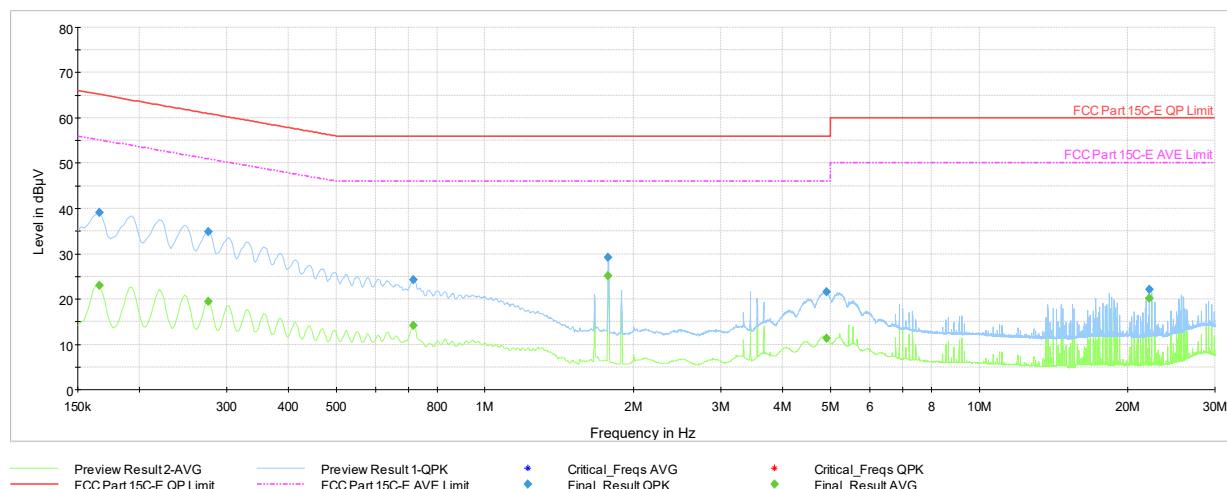
Plot 7-43. AC Line-Conducted Test Plot (L1, GFSK ePA – Ch.39, with AC/DC adaptor via USB-C cable with magnetic charger)
