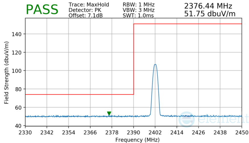
Plot 7-37. Radiated Restricted Lower Band Edge Measurement
