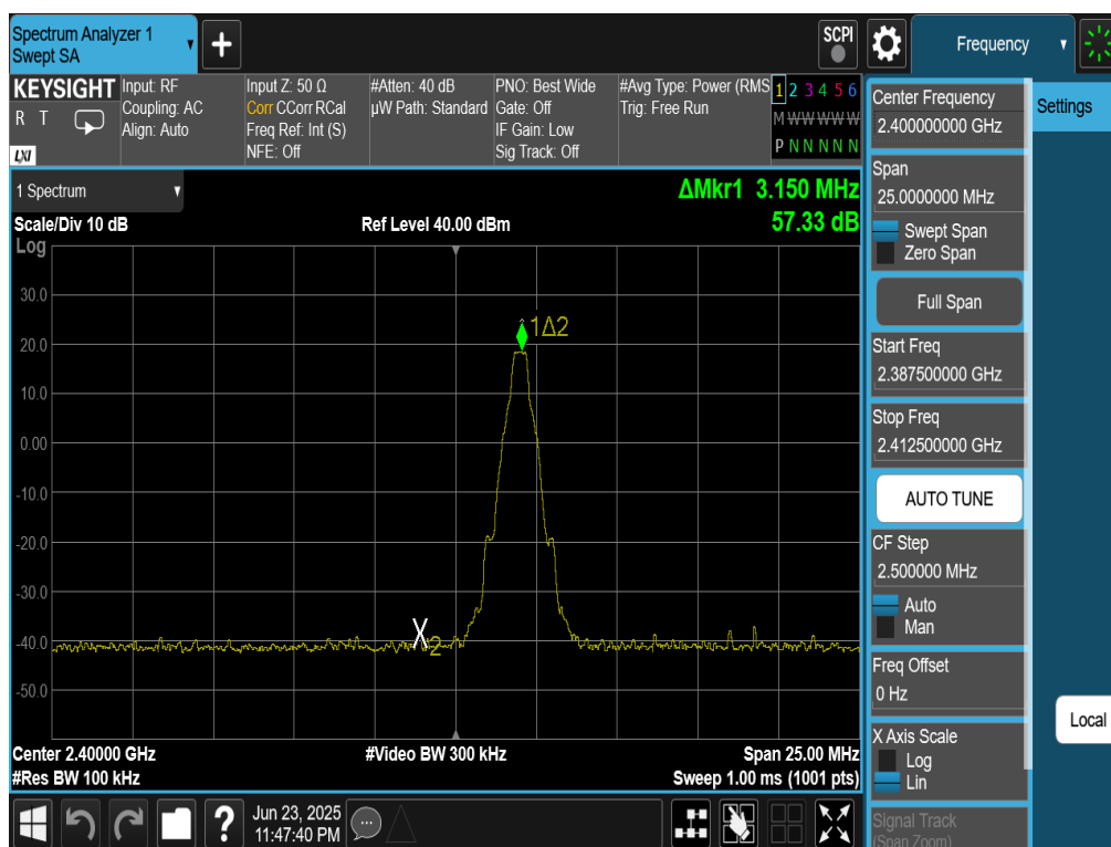
Plot 7-7. Band Edge Plot (Bluetooth with Hopping Disabled, GFSK, ePA – Ch. 0)
