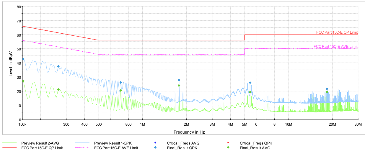
Plot 7-44. AC Line-Conducted Test Plot (N, GFSK ePA – Ch.39, with AC/DC adaptor via USB-C cable with magnetic charger)
