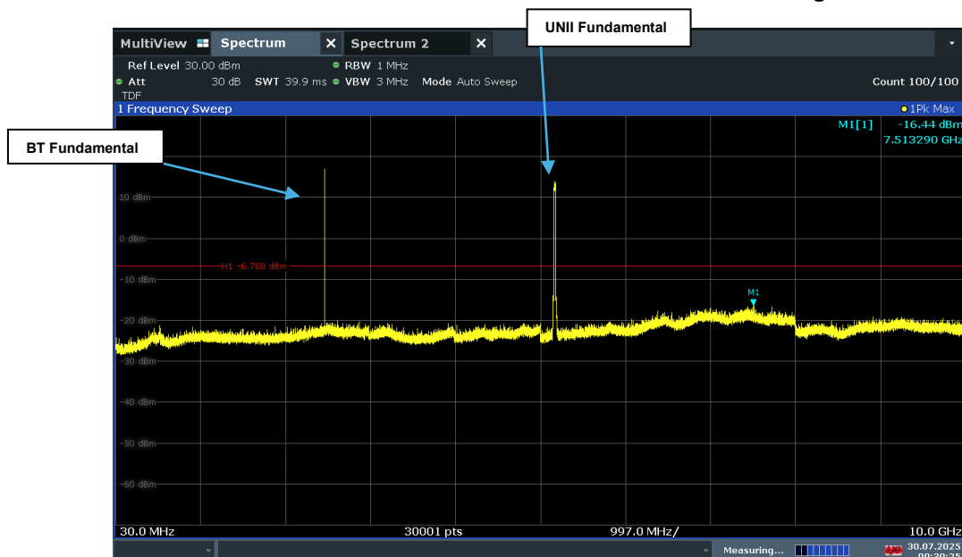
Plot 7-29. Conducted Simultaneous Tx Spurious Plot
