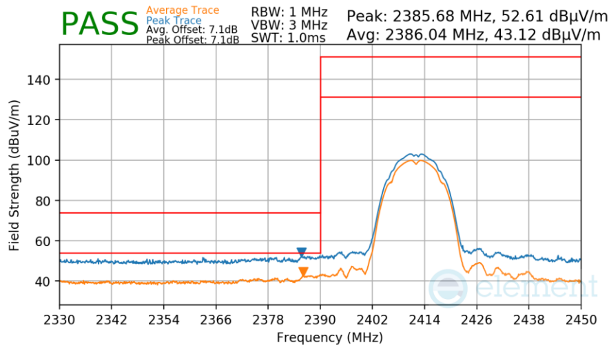
Plot 7-57. Radiated Restricted Lower Band Edge Measurement
