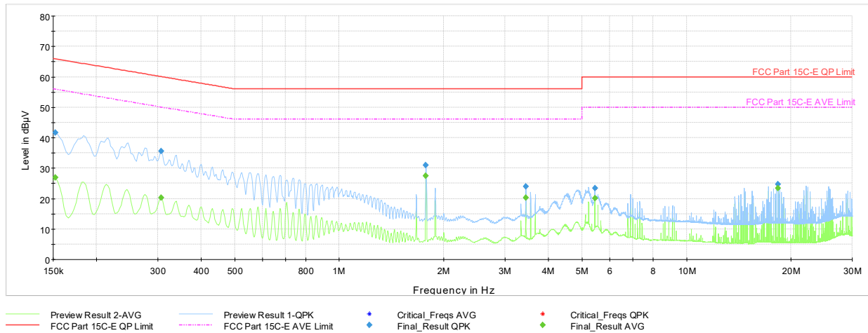
Plot 7-73. AC Line Conducted Plot 802.11b - Ch.6 (L1, with AC/DC adaptor via USB-C cable with magnetic charger)
