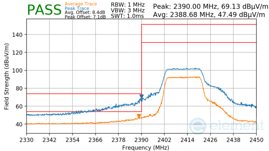
Plot 7-67. Radiated Restricted Lower Band Edge Measurement
