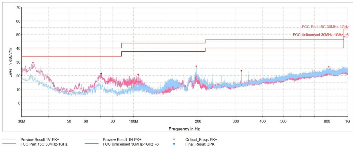
Plot 7-72. Radiated Spurious Emissions below 1GHz 11b Ch.6, with AC/DC Adapter via USB-C cable with magnetic charger
