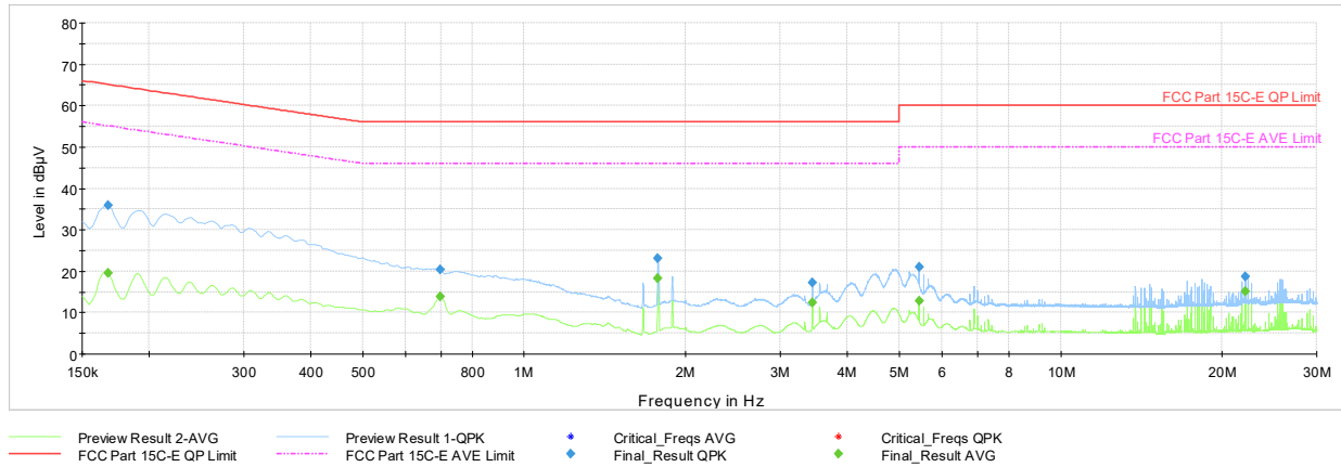
Plot 7-74. AC Line Conducted Plot 802.11b - Ch.6 (N, with AC/DC adaptor via USB-C cable with magnetic charger)
