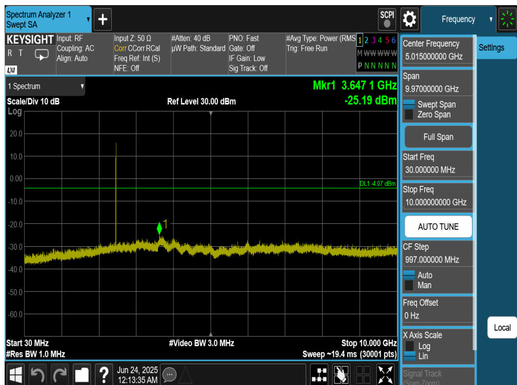
Plot 7-27. Conducted Spurious Plot (Bluetooth (HDR4), 4 Mbps, ePA – Ch. 73)
