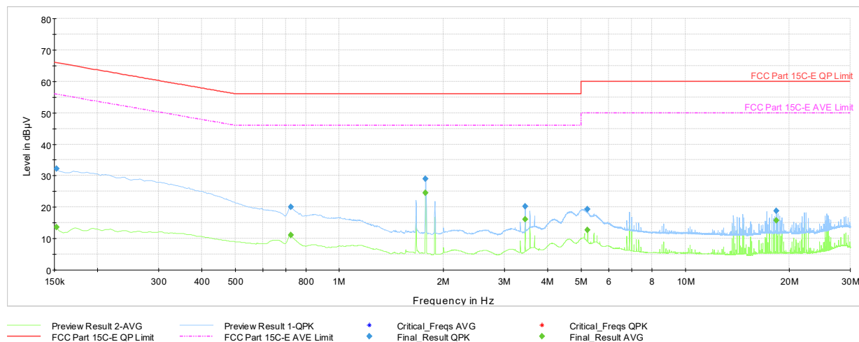
Plot 7-38. AC Line Conducted Plot with Bluetooth HDR (L1, 4Mbps ePA - Ch.38 with AC/DC adaptor via USB-C cable with magnetic charger)
