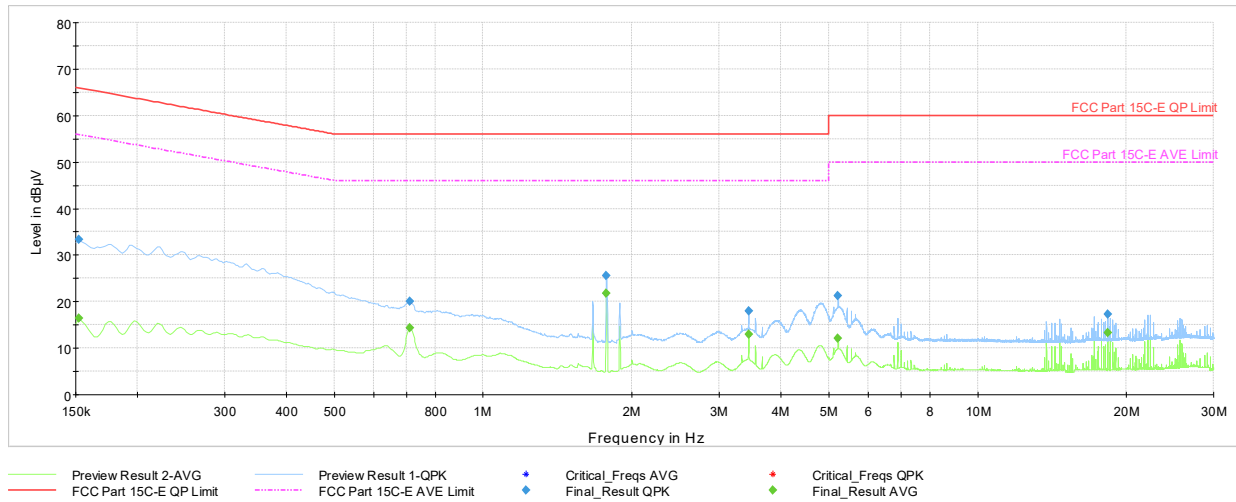
Plot 7-39. AC Line Conducted Plot with Bluetooth HDR (N, 4Mbps ePA - Ch.38 with AC/DC adaptor via USB-C cable with magnetic charger)
