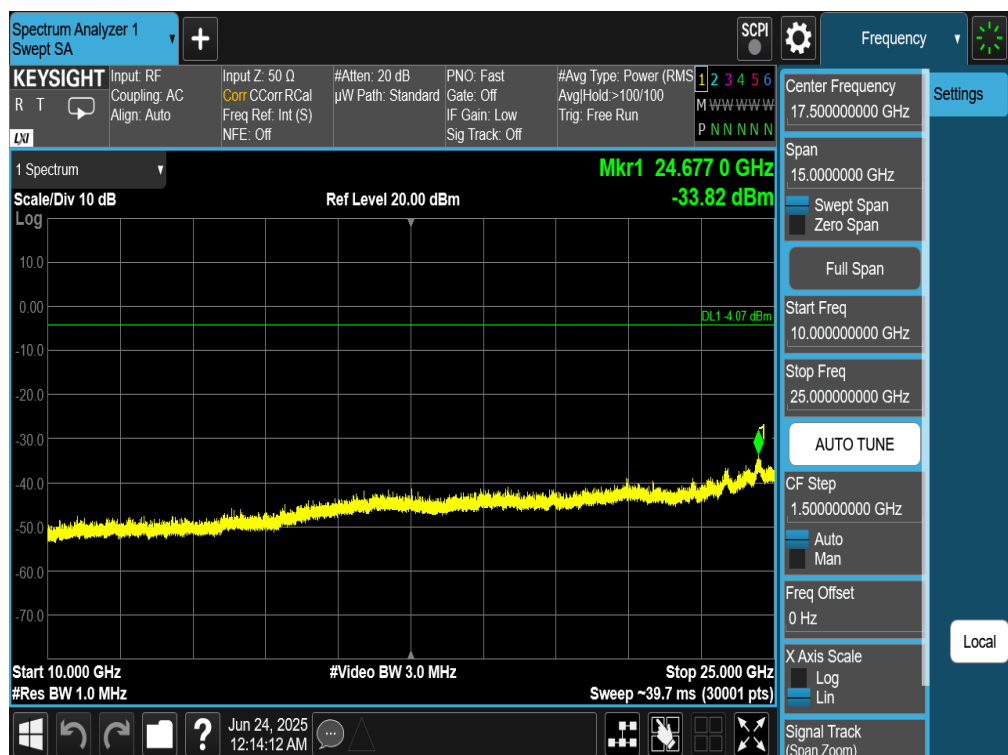
Plot 7-28. Conducted Spurious Plot (Bluetooth (HDR4), 4 Mbps, ePA – Ch. 73)
