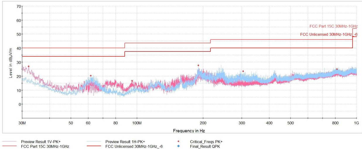
Plot 7-37. Radiated Spurious Emissions Below 1GHz (4Mbps, ePA – Ch.38 with AC/DC adaptor via USB-C cable with magnetic charger)
