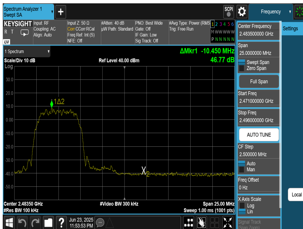
Plot 7-22. Band Edge Plot (Bluetooth (HDR8), ePA – Ch. 73)
