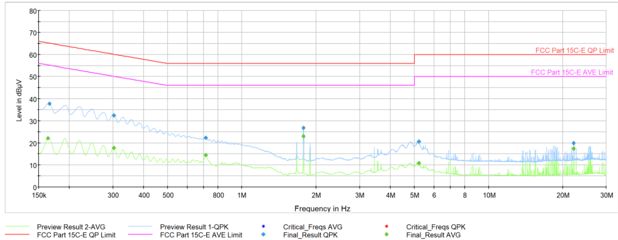
Plot 7-60. AC Line Conducted Plot with 802.11n Ch.64 (N), with AC/DC & magnetic charger
