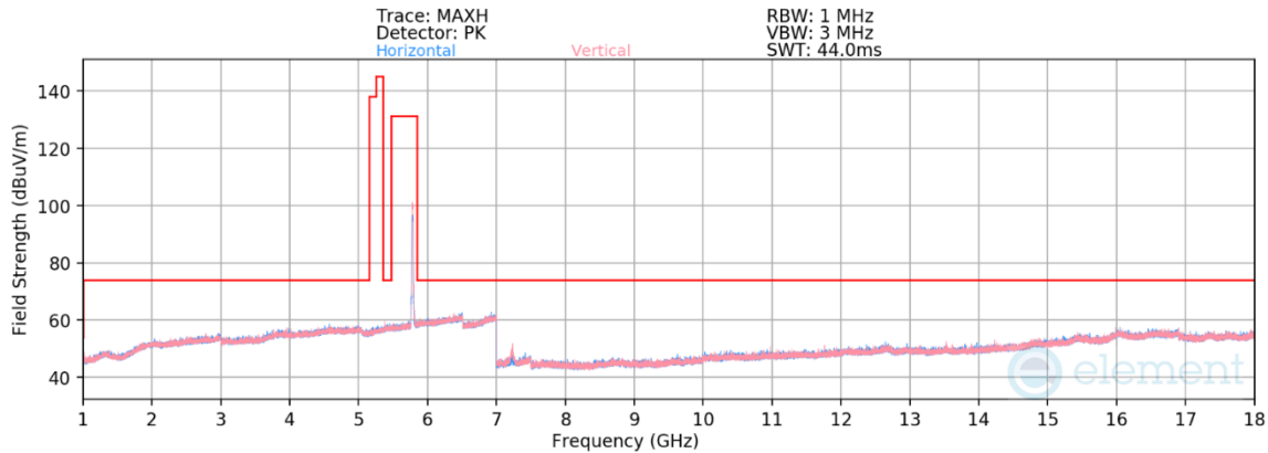
Plot 7-39. Radiated Spurious Emissions above 1GHz(802.11n – Ch. 157)
