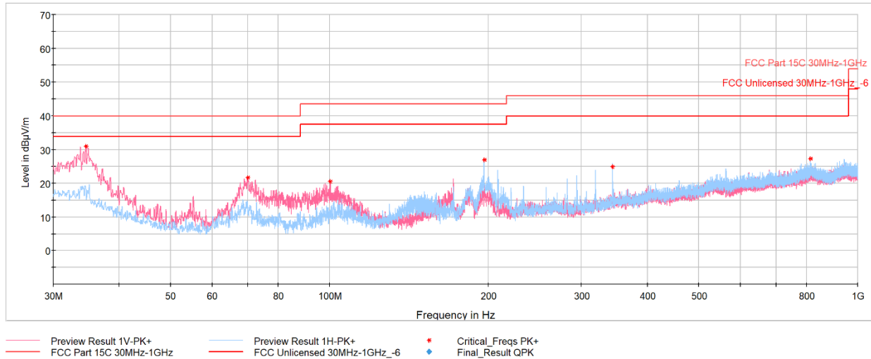
Plot 7-57. Radiated Spurious Emissions below 1GHz, 802.11n, Ch.64 with AC/DC Adapter & magnetic charger
