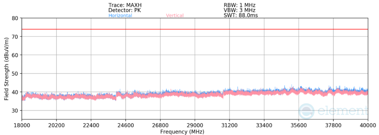
Plot 7-34. Radiated Emissions 18GHz-40GHz (802.11n – Ch. 64)
