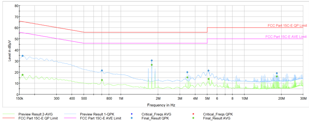
Plot 7-59. AC Line Conducted Plot with 802.11n Ch.64 (L1), with AC/DC adapter & magnetic charger
