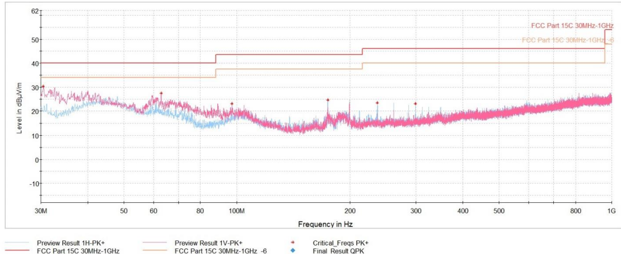
Plot 7-58. Radiated Spurious Emissions – Simultaneous Transmission 30MHz – 1GHz, with AC/DC Adapter & magnetic charger)
