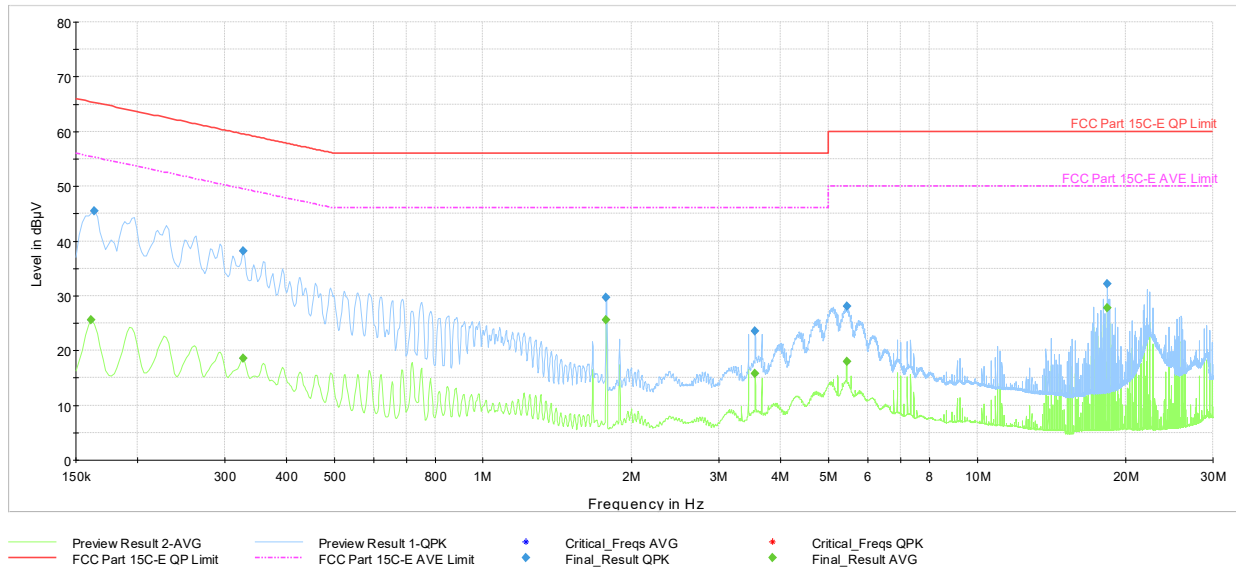
Plot 7-44. AC Line-Conducted Test Plot (N, GFSK ePA – Ch.39, with AC/DC adaptor via USB-C cable with magnetic charger)
