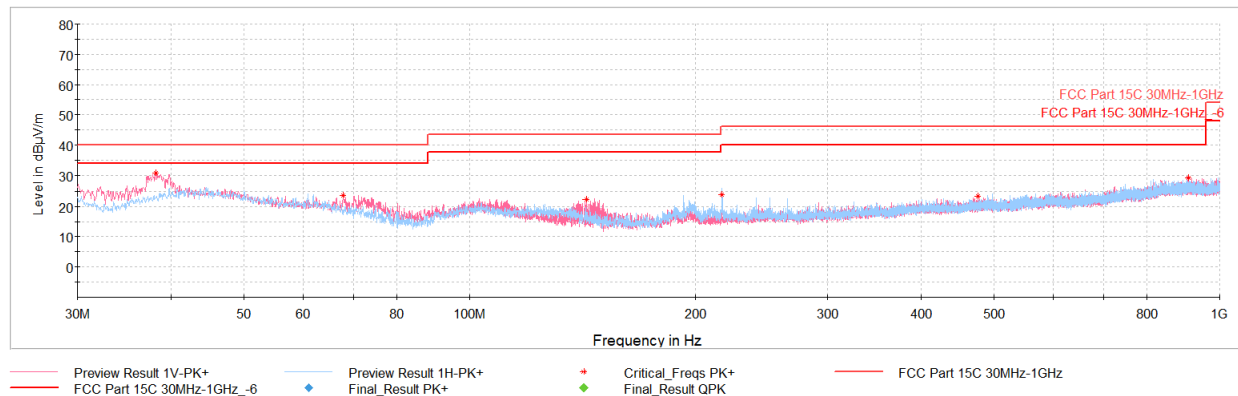
Plot 7-41. Radiated Spurious Emissions Below 1GHz (GFSK ePA – Ch.39, with AC/DC adaptor via USB-C cable with magnetic charger)
