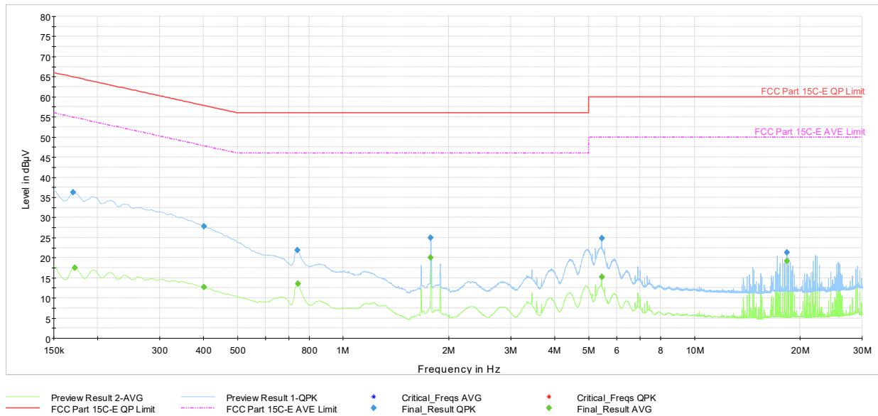
Plot 7-38. AC Line Conducted Plot with Bluetooth LE (L1, 1Mbps ePA – Ch.19 with AC/DC adaptor via USB-C cable with magnetic charger)
