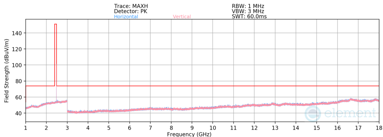
Plot 7-32. Radiated Spurious Emissions 1-18GHz (1Mbps ePA – Ch. 39)
