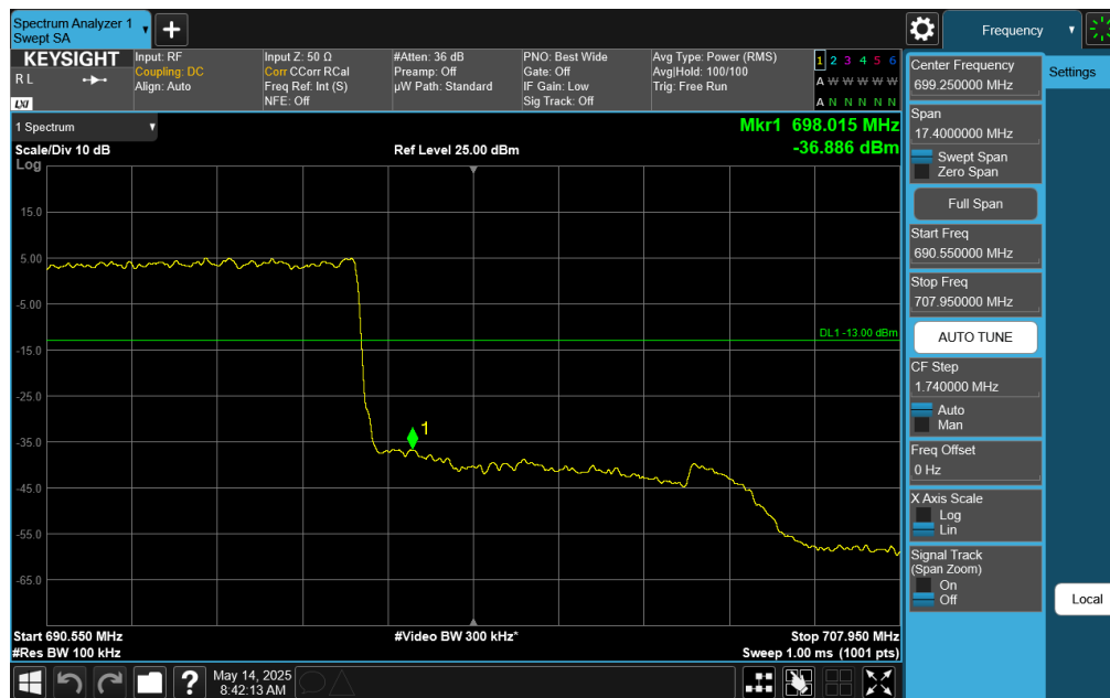
Plot 7-233. Upper Band Edge Plot (NR Band n71 – 15.0MHz DFT-s-OFDM \pi/2 BPSK - Full RB)
