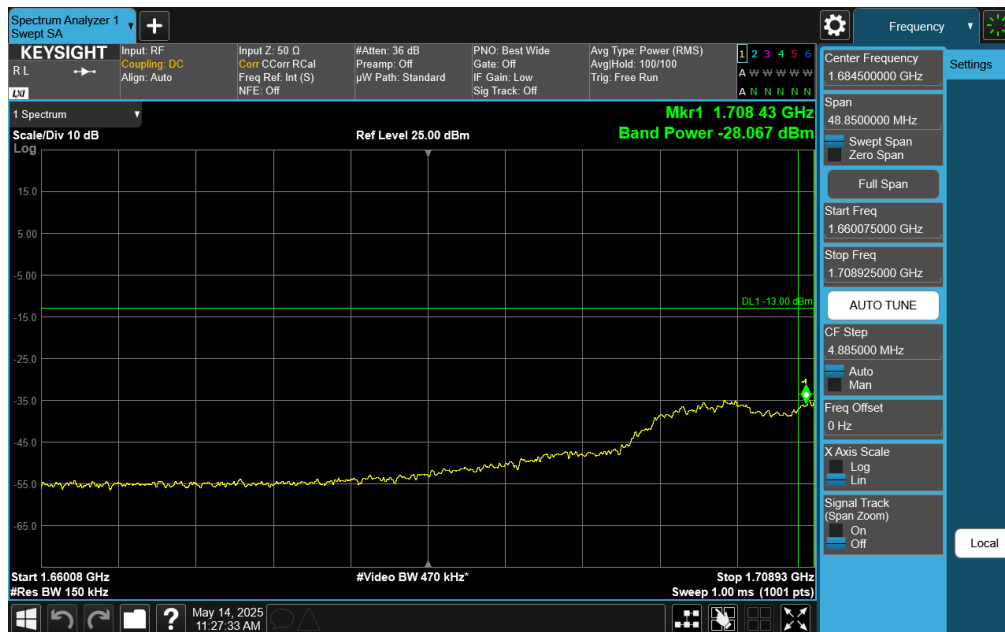
Plot 7-221. Lower Extended Band Edge Plot (NR Band n66 – 15.0MHz DFT-s-OFDM \pi/2 BPSK - Full RB)
