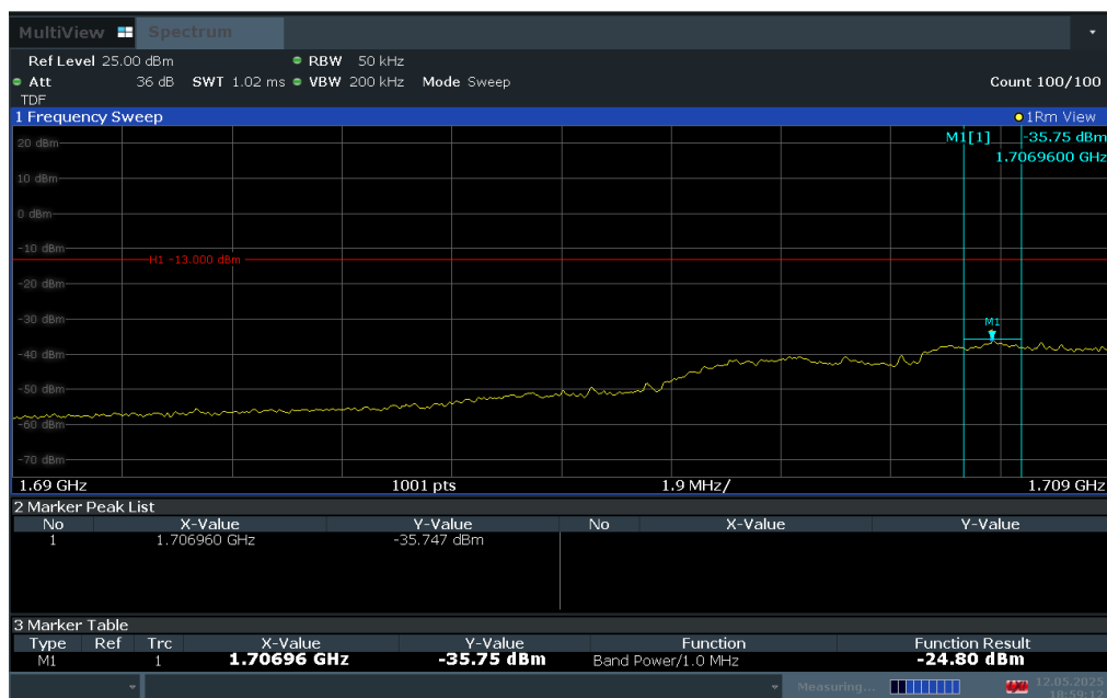
Plot 7-169. Lower Extended Band Edge Plot (LTE Band 4 - 5MHz QPSK – Full RB)
