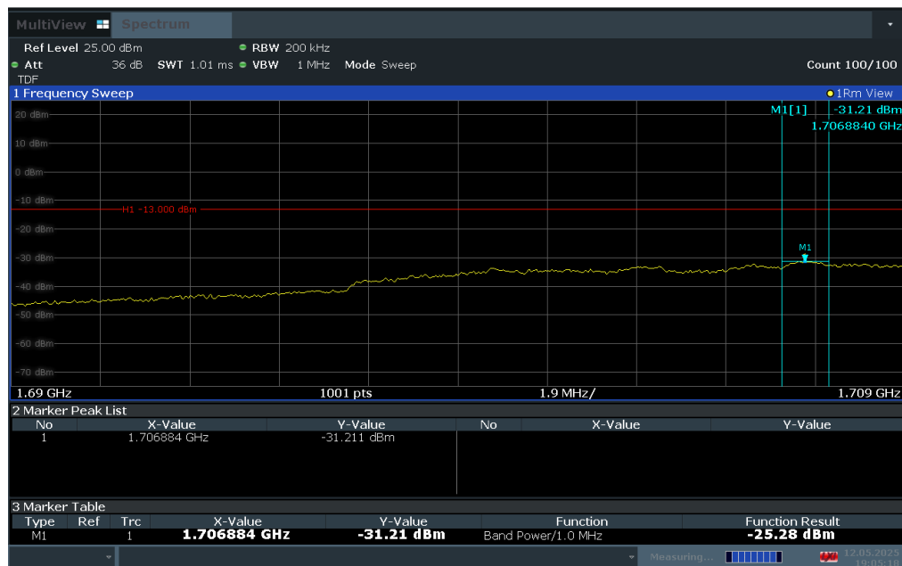
Plot 7-177. Lower Extended Band Edge Plot (LTE Band 4 - 15MHz QPSK – Full RB)
