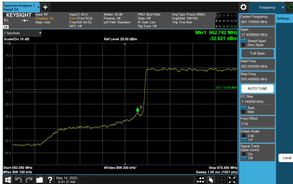
Plot 7-232. Lower Band Edge Plot (NR Band n71 – 15.0MHz DFT-s-OFDM \pi/2 BPSK - Full RB)
