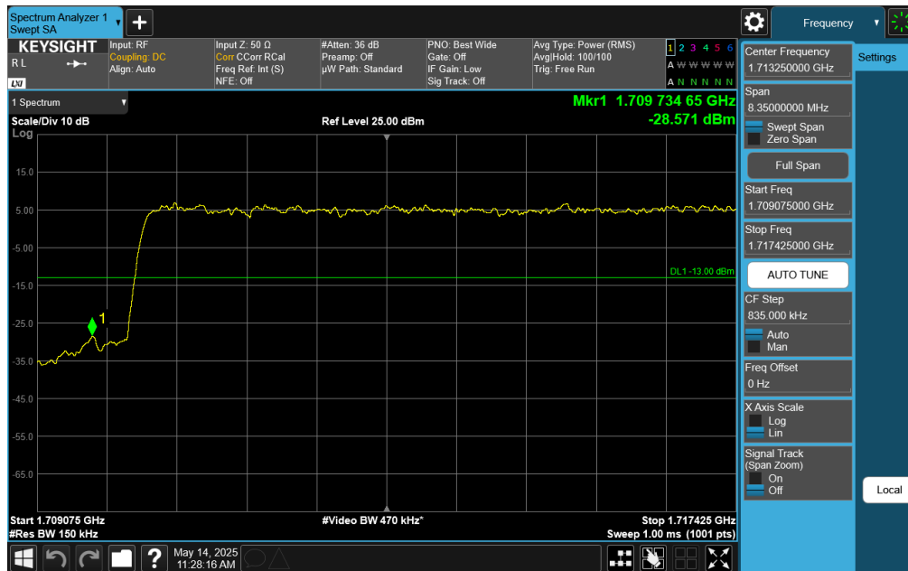
Plot 7-220. Lower Band Edge Plot (NR Band n66 – 15.0MHz DFT-s-OFDM \pi/2 BPSK - Full RB)
