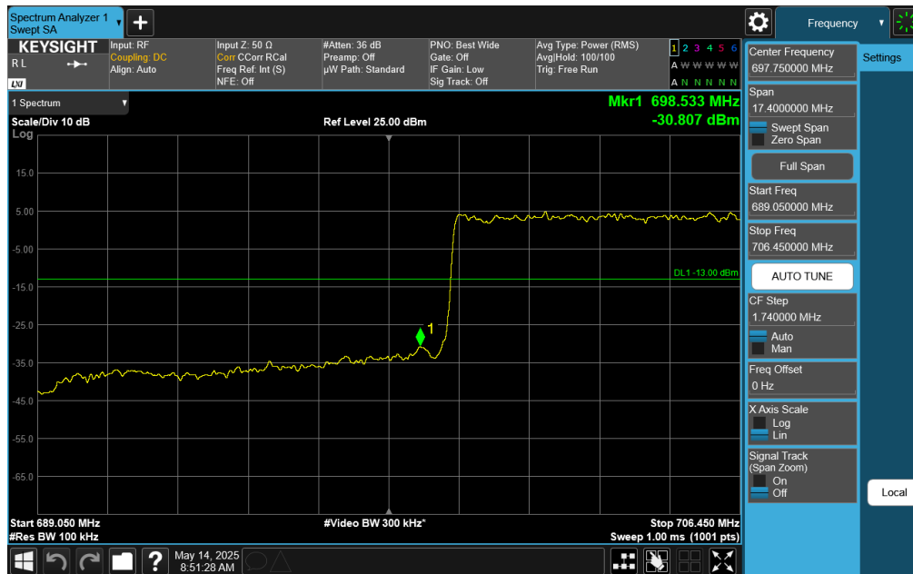
Plot 7-240. Lower Band Edge Plot (NR Band n12 – 15.0MHz DFT-s-OFDM \pi/2 QPSK - Full RB)
