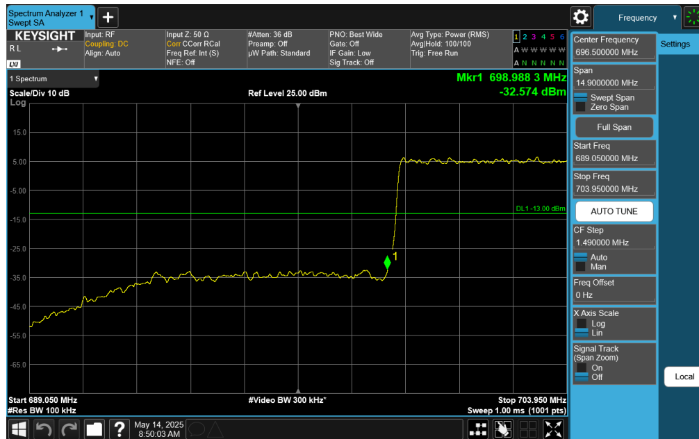
Plot 7-238. Lower Band Edge Plot (NR Band n12 – 10.0MHz DFT-s-OFDM \pi/2 QPSK - Full RB)
