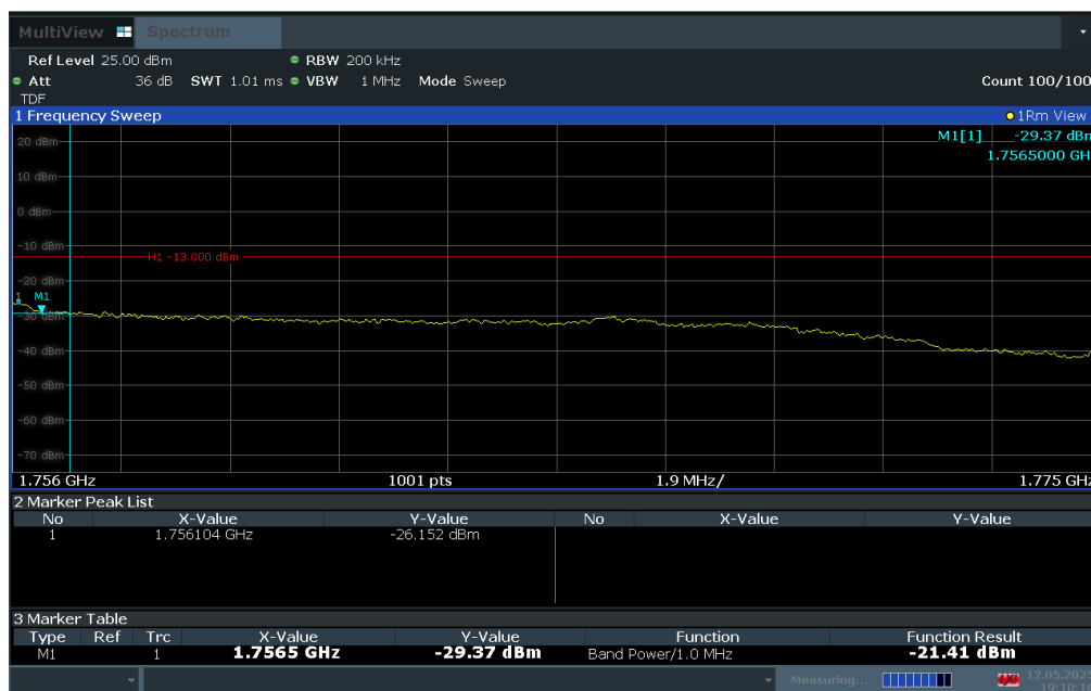
Plot 7-183. Upper Extended Band Edge Plot (LTE Band 4 - 20MHz QPSK – Full RB)
