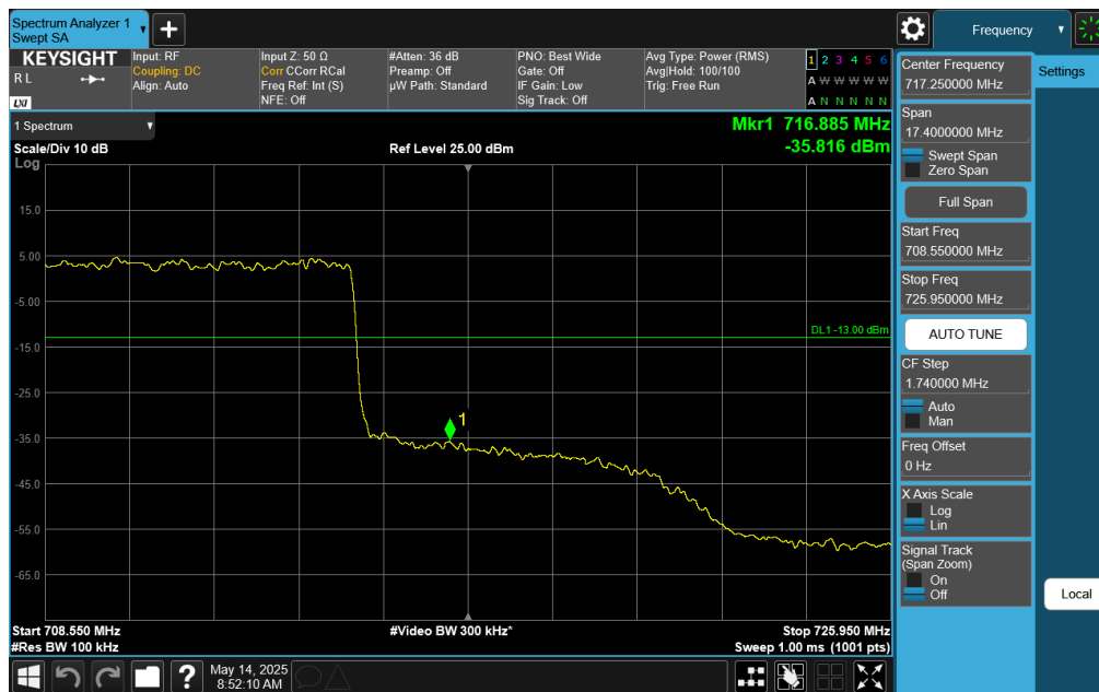
Plot 7-241. Upper Band Edge Plot (NR Band n12 – 15.0MHz DFT-s-OFDM \pi/2 QPSK - Full RB)
