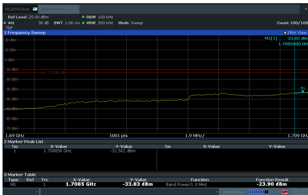
Plot 7-173. Lower Extended Band Edge Plot (LTE Band 4 - 10MHz QPSK – Full RB)
