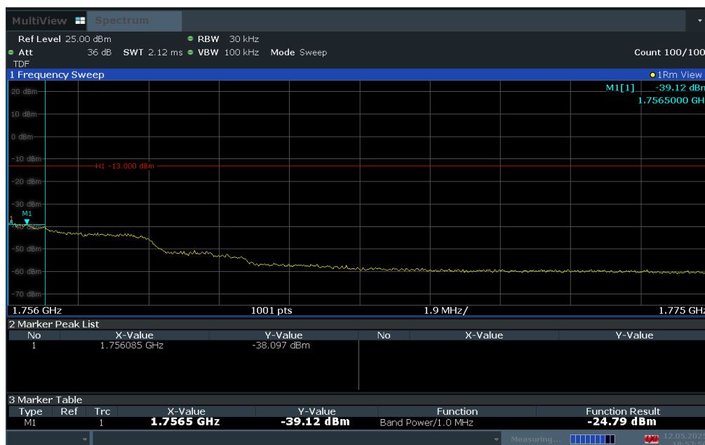
Plot 7-167. Upper Extended Band Edge Plot (LTE Band 4 - 3MHz QPSK – Full RB)
