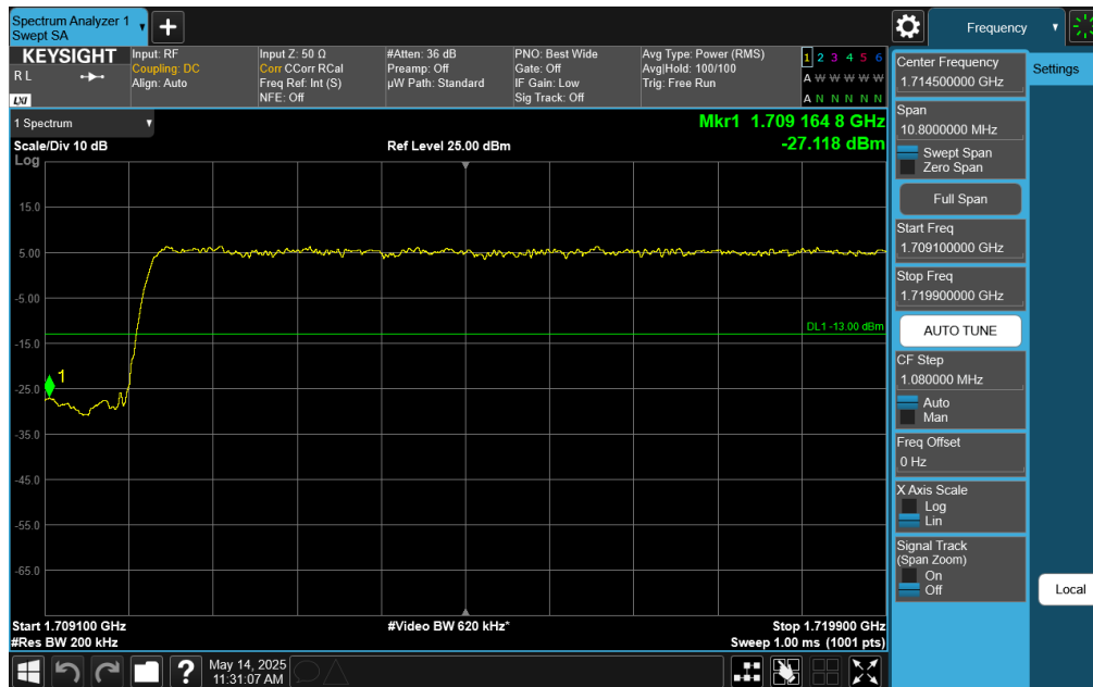
Plot 7-224. Lower Band Edge Plot (NR Band n66 – 20.0MHz DFT-s-OFDM \pi/2 BPSK - Full RB)
