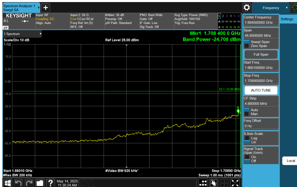
Plot 7-225. Lower Extended Band Edge Plot (NR Band n66 – 20.0MHz DFT-s-OFDM \pi/2 BPSK - Full RB)
