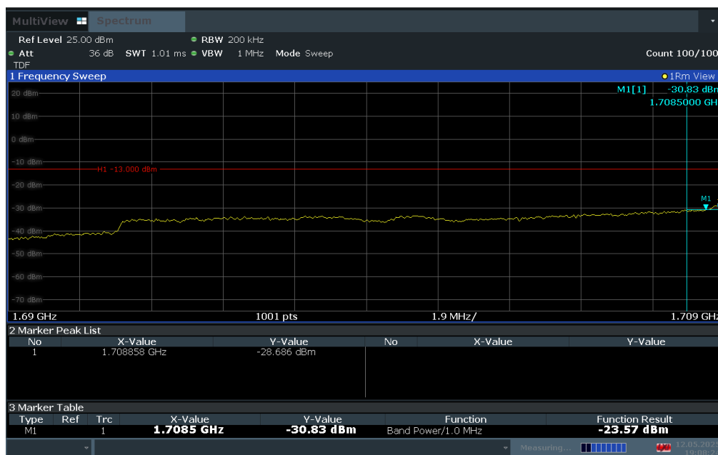
Plot 7-181. Lower Extended Band Edge Plot (LTE Band 4 - 20MHz QPSK – Full RB)
