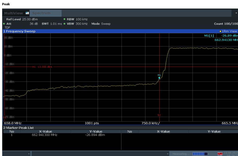
Plot 7-184. Lower Band Edge Plot (LTE Band 71 - 5MHz QPSK – Full RB)
