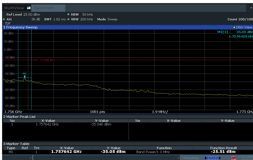
Plot 7-171. Upper Extended Band Edge Plot (LTE Band 4 - 5MHz QPSK – Full RB)
