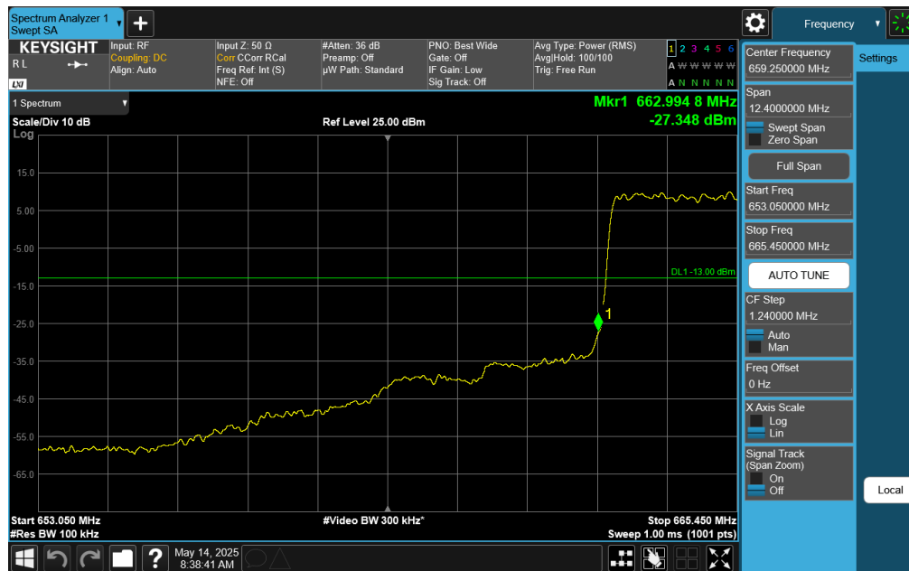
Plot 7-228. Lower Band Edge Plot (NR Band n71 – 5.0MHz DFT-s-OFDM \pi/2 BPSK - Full RB)
