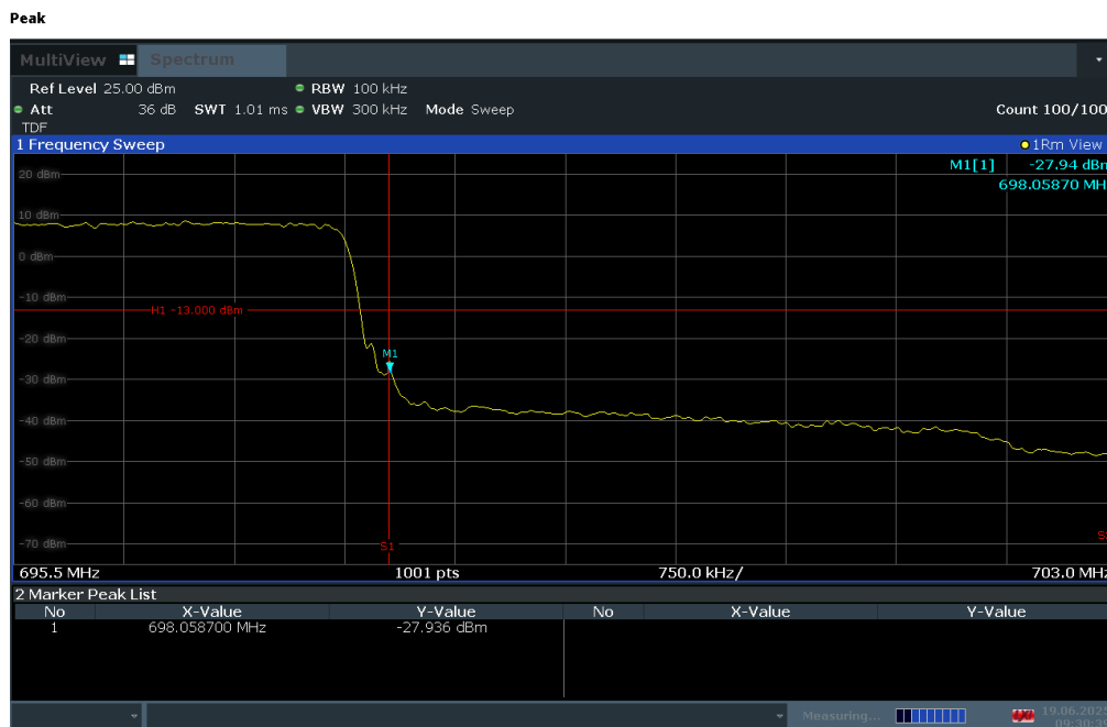
Plot 7-185. Upper Band Edge Plot (LTE Band 71 - 5MHz QPSK – Full RB)
