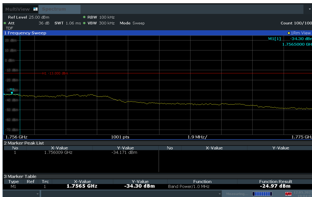
Plot 7-175. Upper Extended Band Edge Plot (LTE Band 4 - 10MHz QPSK – Full RB)
