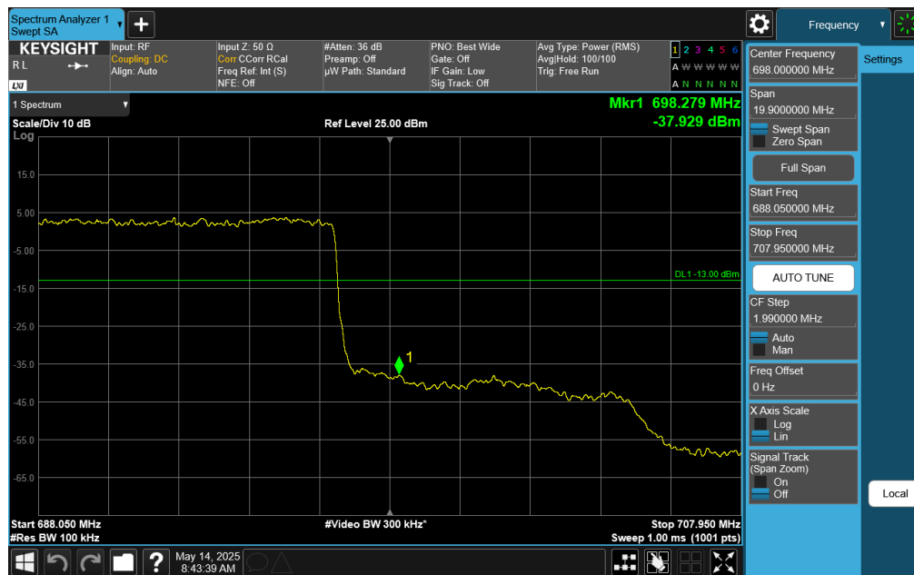
Plot 7-235. Upper Band Edge Plot (NR Band n71 – 20.0MHz DFT-s-OFDM \pi/2 BPSK - Full RB)
