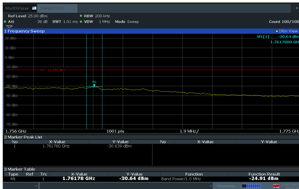
Plot 7-179. Upper Extended Band Edge Plot (LTE Band 4 - 15MHz QPSK – Full RB)
