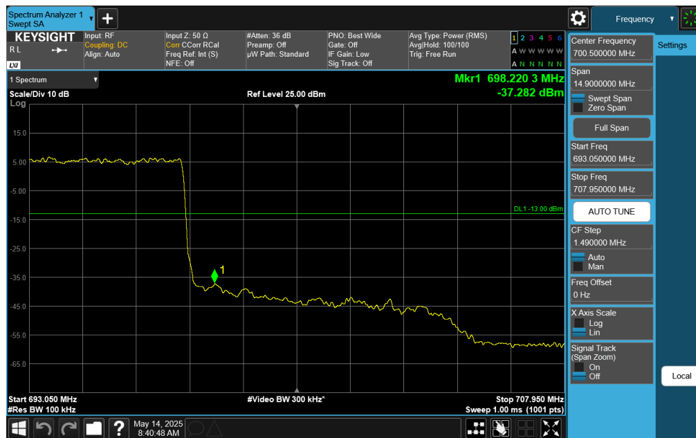
Plot 7-231. Upper Band Edge Plot (NR Band n71 – 10.0MHz DFT-s-OFDM \pi/2 BPSK - Full RB)
