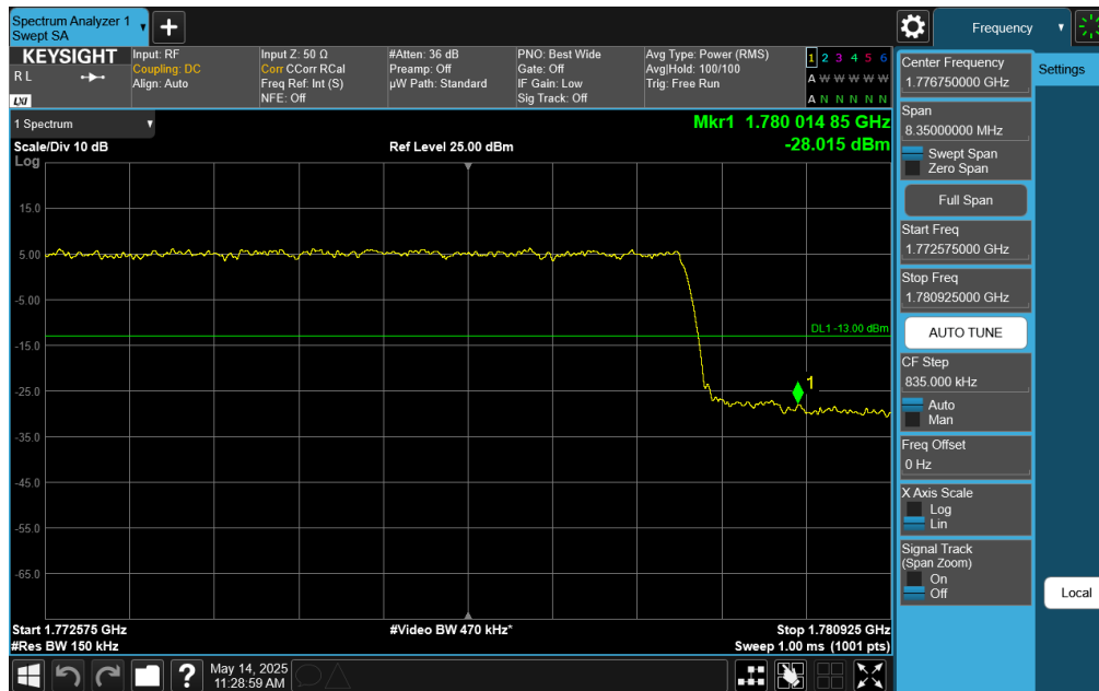
Plot 7-222. Upper Band Edge Plot (NR Band n66 – 15.0MHz DFT -OFDM \pi/2 BPSK - Full RB)
