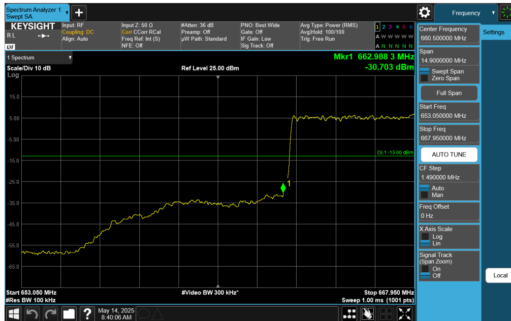
Plot 7-230. Lower Band Edge Plot (NR Band n71 – 10.0MHz DFT-s-OFDM \pi/2 BPSK - Full RB)
