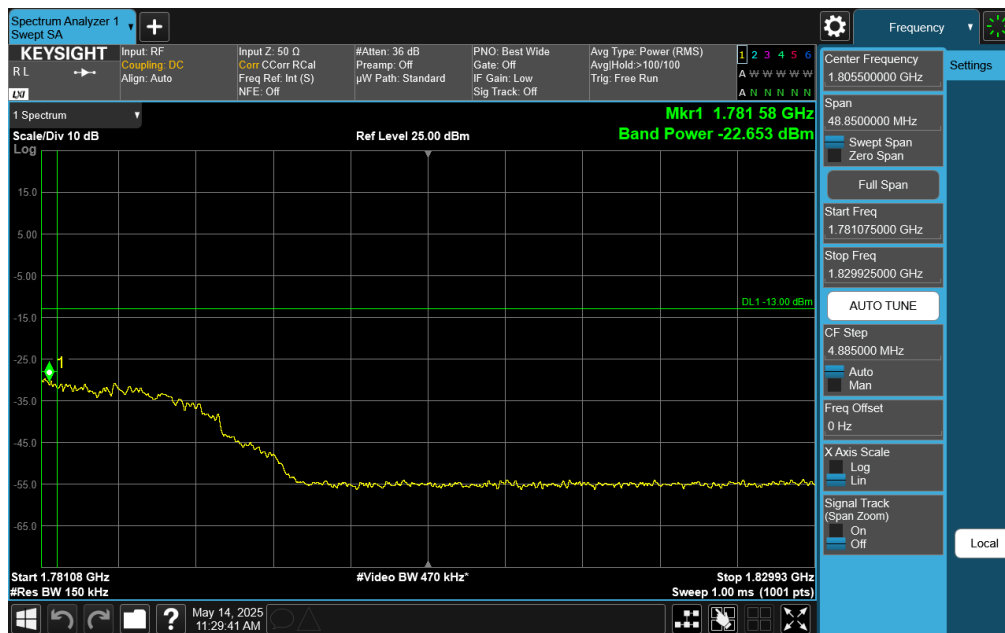
Plot 7-223. Upper Extended Band Edge Plot (NR Band n66 – 15.0MHz DFT-s-OFDM \pi/2 BPSK - Full RB)
