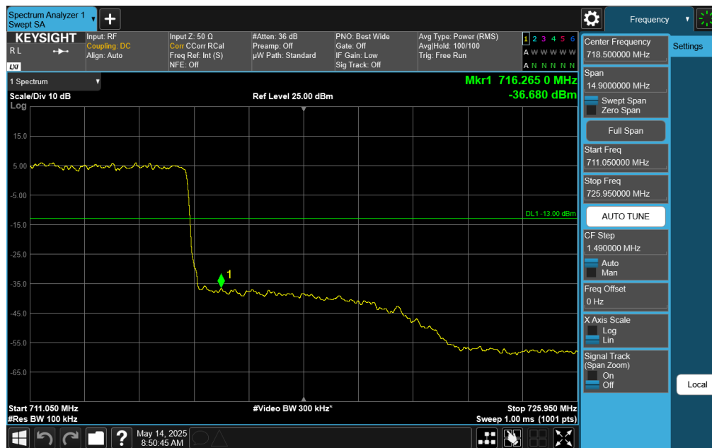
Plot 7-239. Upper Band Edge Plot (NR Band n12 – 10.0MHz DFT-s-OFDM \pi/2 QPSK - Full RB)
