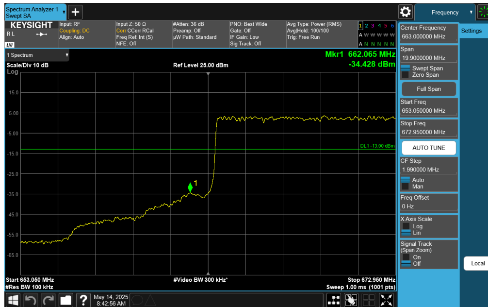
Plot 7-234. Lower Band Edge Plot (NR Band n71 – 20.0MHz DFT-s-OFDM \pi/2 BPSK - Full RB)
