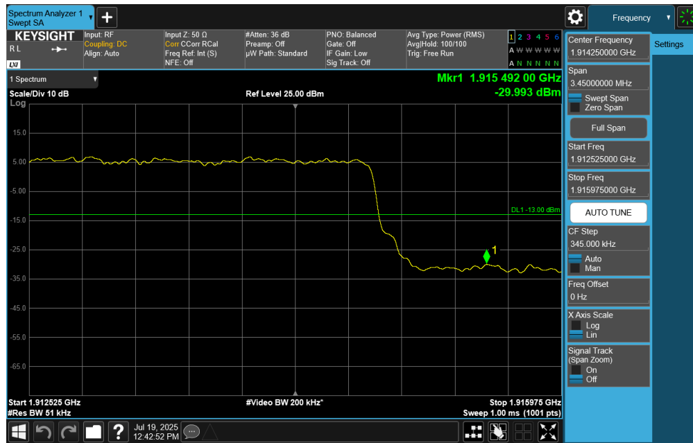
Plot 7-97. Upper Band Edge Plot (NR Band n25 – 5MHz DFT-s-OFDM \pi/2 QPSK – Full RB Configuration)
