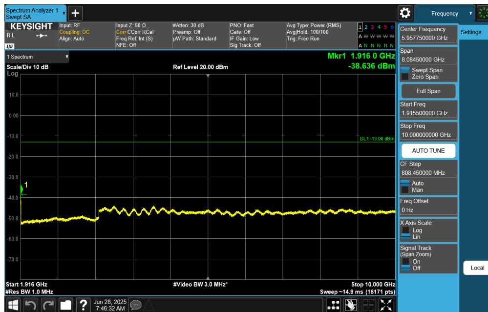
Plot 7-45. Conducted Spurious Plot (NR Band n25/n2 - 20.0MHz DFT-s-OFDM QPSK - RB Size 1, RB Offset 50 - High Channel)
