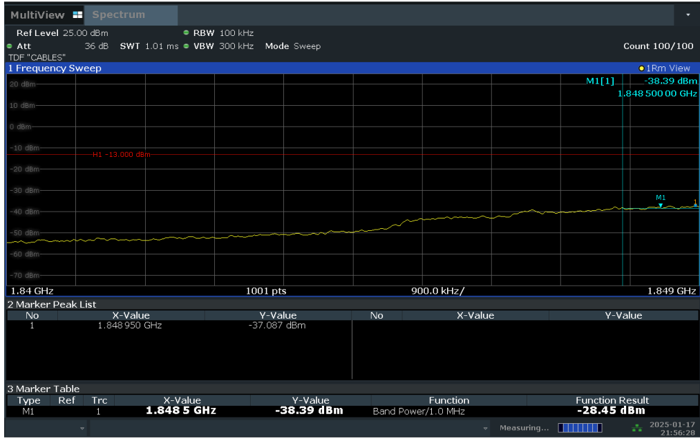
Plot 7-76. Extended Lower Band Edge Plot (LTE Band 2 – 3MHz QPSK – Full RB Configuration)
