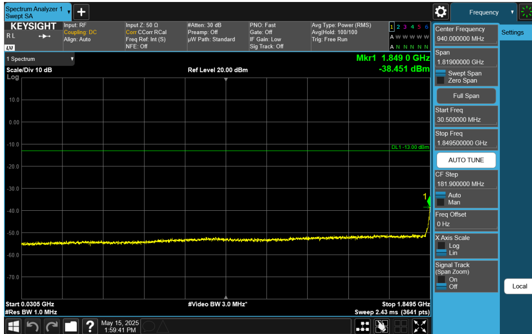
Plot 7-38. Conducted Spurious Plot (NR Band n25/n2 - 20.0MHz DFT-s-OFDM QPSK - RB Size 1, RB Offset 50 - Low Channel)
