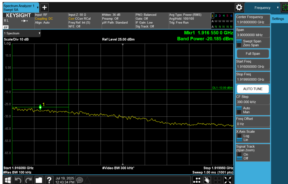
Plot 7-98. Extended Upper Band Edge Plot (NR Band n25 – 5MHz DFT-s- QPSK \pi/2 QPSK – Full RB Configuration)
