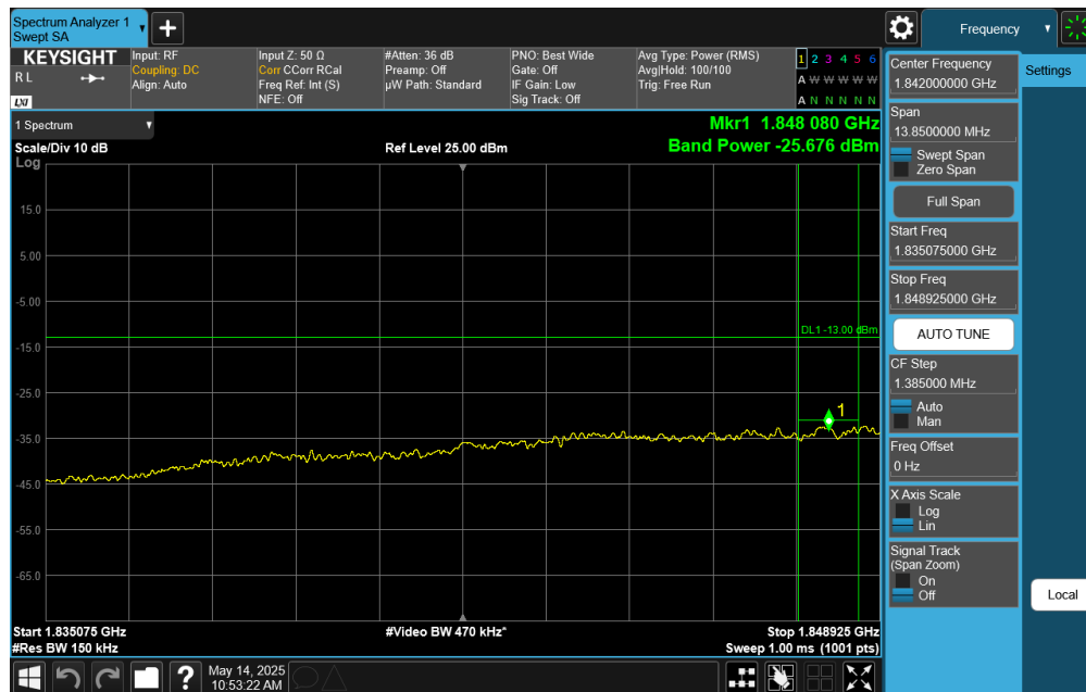
Plot 7-104. Extended Lower Band Edge Plot (NR Band n25 – 15MHz DFT-s-OFDM \pi/2 BPSK – Full RB Configuration)
