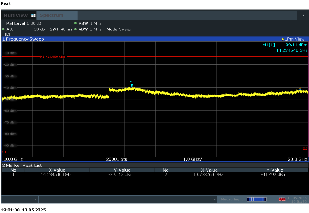
Plot 7-37. Conducted Spurious Plot (LTE Band 25/2 - 20MHz QPSK - RB Size 1, RB Offset 50 - High Channel)
