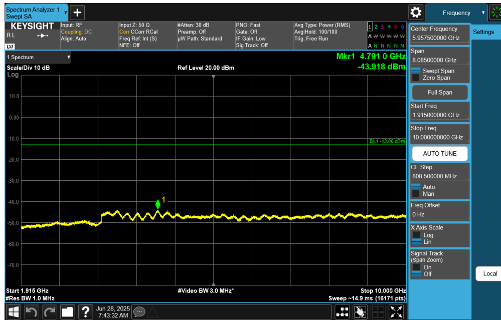
Plot 7-42. Conducted Spurious Plot (NR Band n25/n2 - 20.0MHz DFT-s-OFDM QPSK - RB Size 1, RB Offset 50 - Mid Channel)
