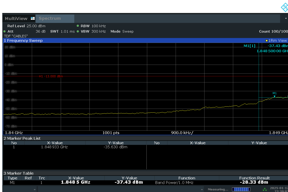
Plot 7-48. Extended Lower Band Edge Plot (LTE Band 25 – 1.4MHz QPSK – Full RB Configuration)
