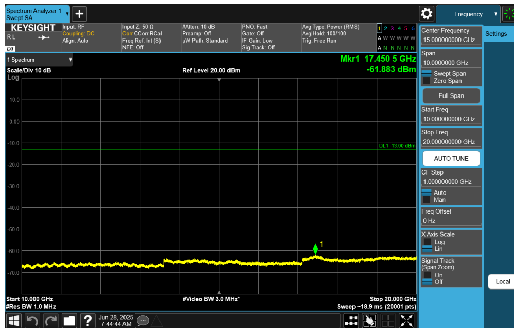
Plot 7-43. Conducted Spurious Plot (NR Band n25/n2 - 20.0MHz DFT-s-OFDM QPSK - RB Size 1, RB Offset 50 - Mid Channel)
