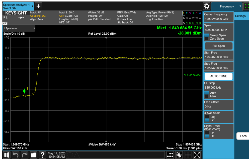
Plot 7-103. Lower Band Edge Plot (NR Band n25 – 15MHz DFT-s-OFDM \pi/2 BPSK – Full RB Configuration)
