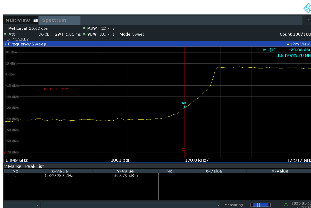
Plot 7-71. Lower Band Edge Plot (LTE Band 2 – 1.4MHz QPSK – Full RB Configuration)
