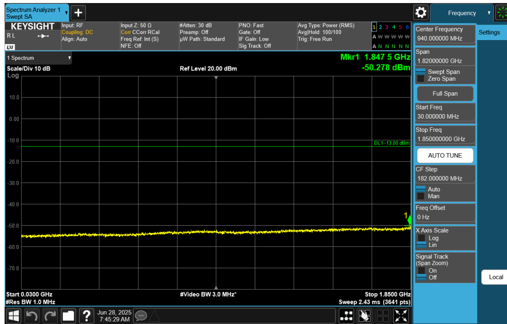
Plot 7-44. Conducted Spurious Plot (NR Band n25/n2 - 20.0MHz DFT-s-OFDM QPSK - RB Size 1, RB Offset 50 - High Channel)
