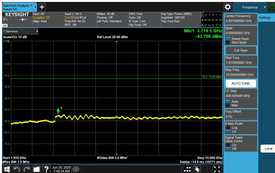
Plot 7-39. Conducted Spurious Plot (NR Band n25/n2 - 20.0MHz DFT-s-OFDM QPSK - RB Size 1, RB Offset 50 - Low Channel)
