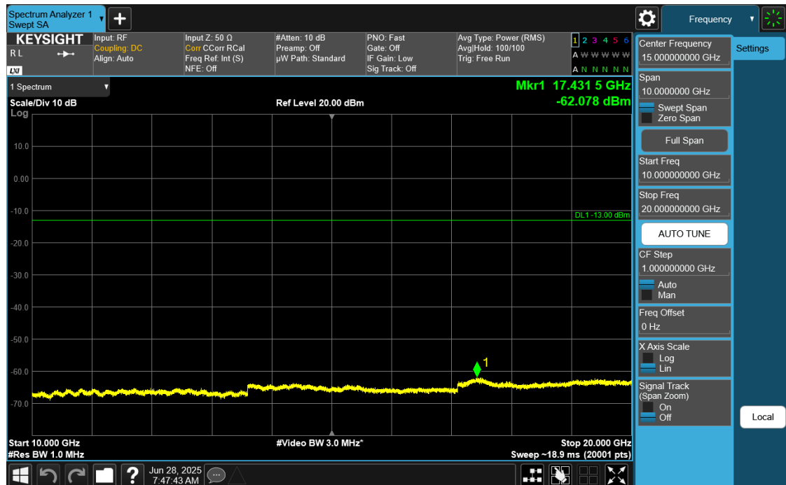
Plot 7-46. Conducted Spurious Plot (NR Band n25/n2 - 20.0MHz DFT-s-OFDM QPSK - RB Size 1, RB Offset 50 - High Channel)
