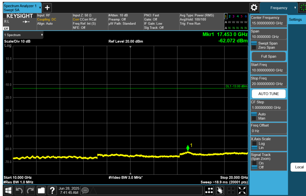
Plot 7-40. Conducted Spurious Plot (NR Band n25/n2 - 20.0MHz DFT-s-OFDM QPSK - RB Size 1, RB Offset 50 - Low Channel)
