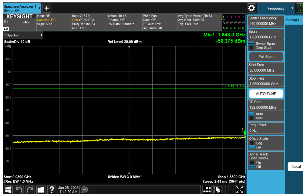
Plot 7-41. Conducted Spurious Plot (NR Band n25/n2 - 20.0MHz DFT-s-OFDM QPSK - RB Size 1, RB Offset 50 - Mid Channel)
