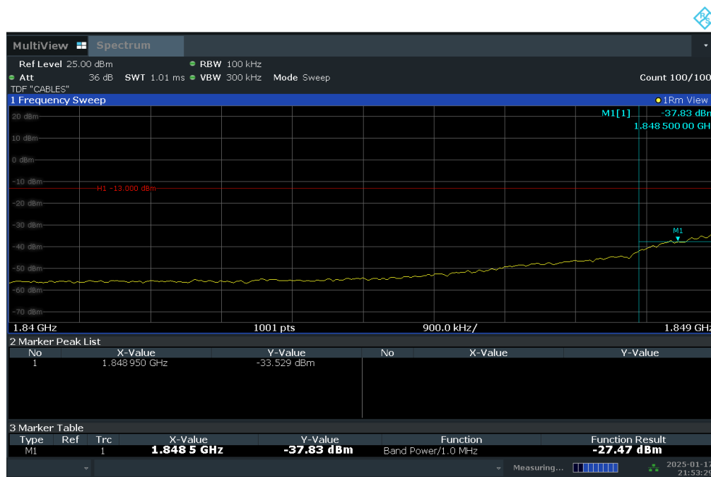
Plot 7-72. Extended Lower Band Edge Plot (LTE Band 2 – 1.4MHz QPSK – Full RB Configuration)
