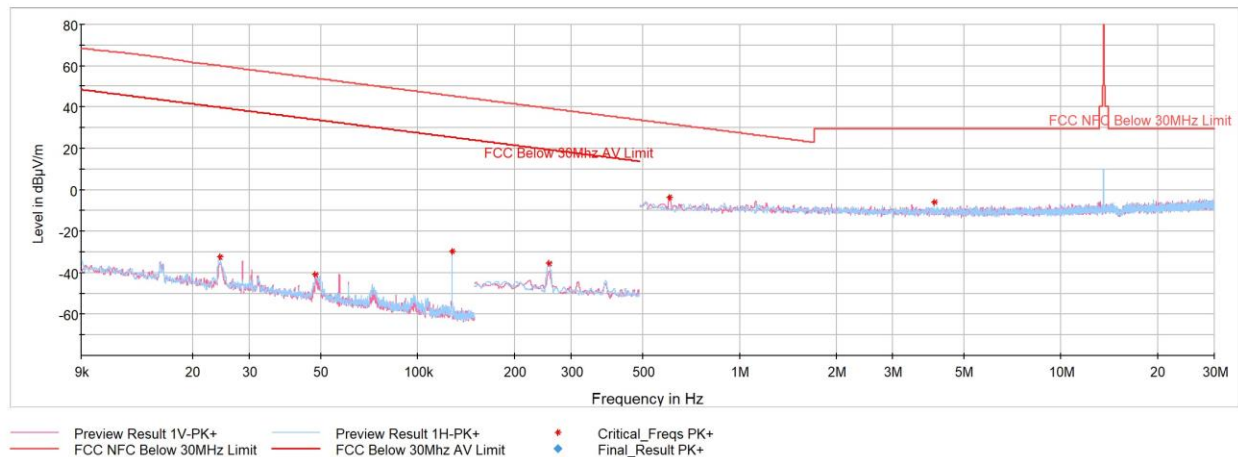
Plot 7-8. Radiated Spurious Emissions 9kHz – 30MHz (CE F 424kbps, with AC/DC Adapter and Magnetic Charger)
