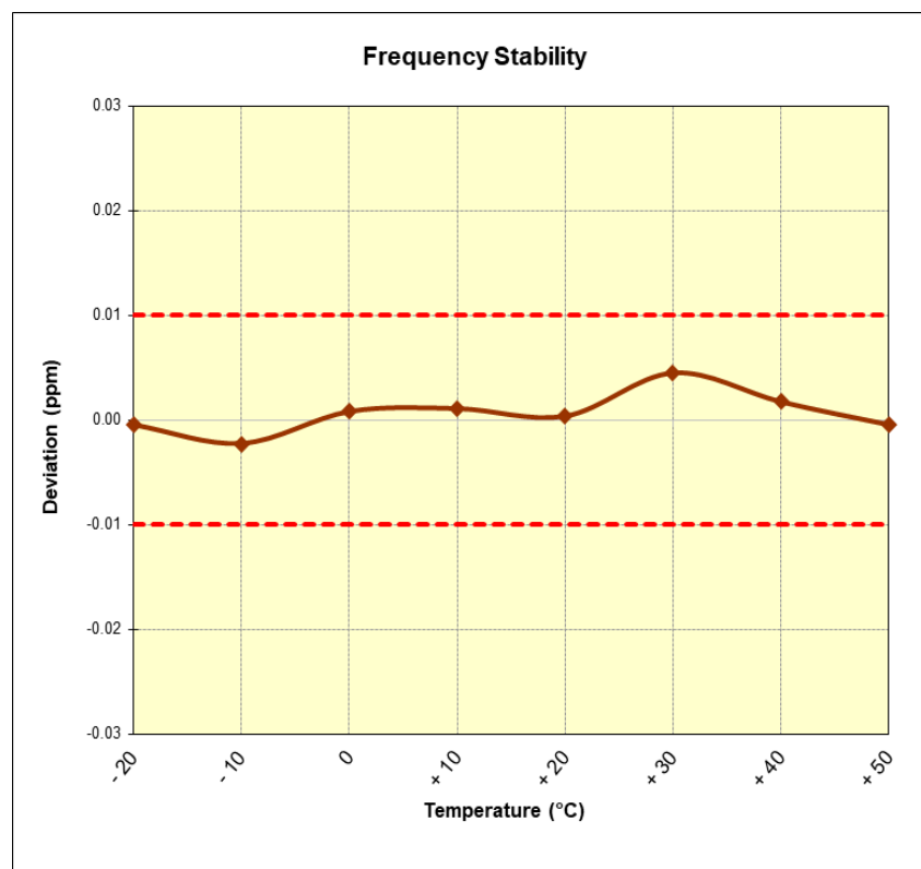
Figure 7-3. Frequency Stability Plot (CE F 424kbps)
