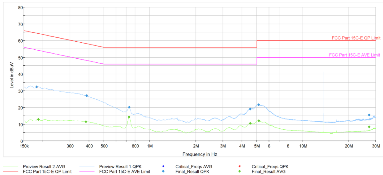
Plot 7-13. AC Line-Conducted Plot (N, CE F 424kbps, with AC/DC Adapter and Magnetic Charger)
