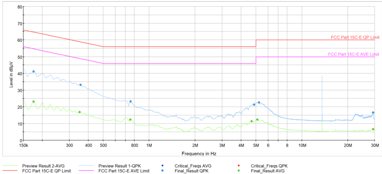
Plot 7-15. AC Line-Conducted Plot (N, Reader A 106kbps, with AC/DC Adapter and Magnetic Charger)
