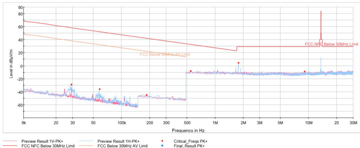
Plot 7-9. Radiated Spurious Emissions 9kHz – 30MHz (Reader A 106kbps, with AC/DC Adapter and Magnetic Charger)
