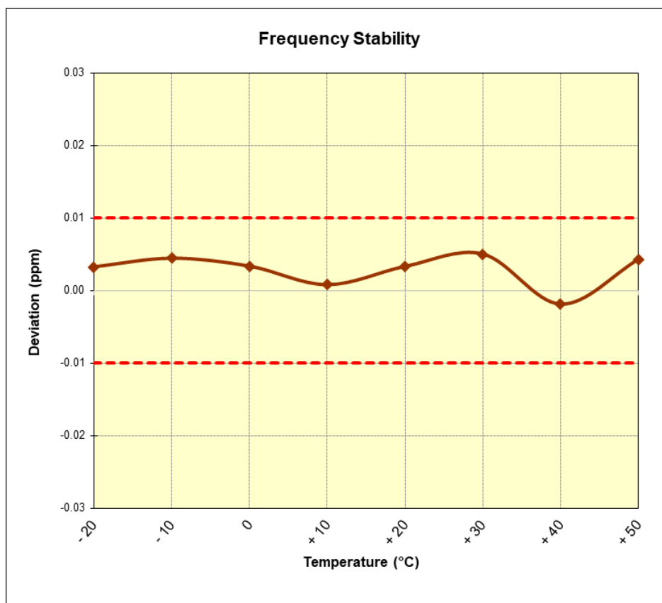
Figure 7-4. Frequency Stability Plot (Reader A 106kbps)
