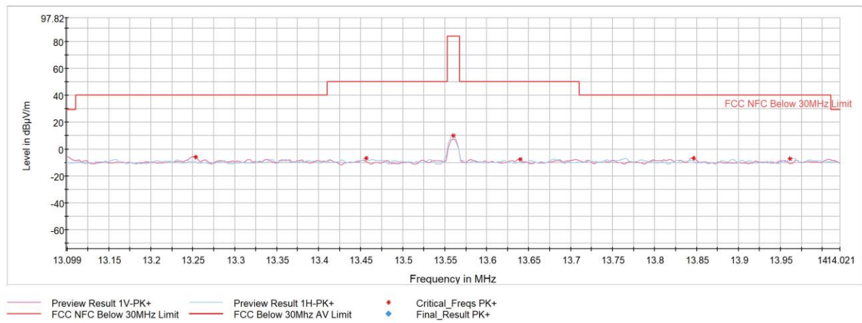
Plot 7-6. In Band Radiated Spurious Emissions (CE F 424kbps, with AC/DC Adapter and Magnetic Charger)
