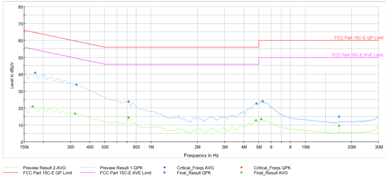
Plot 7-14. AC Line-Conducted Plot (L1, Reader A 106kbps, with AC/DC Adapter and Magnetic Charger)
