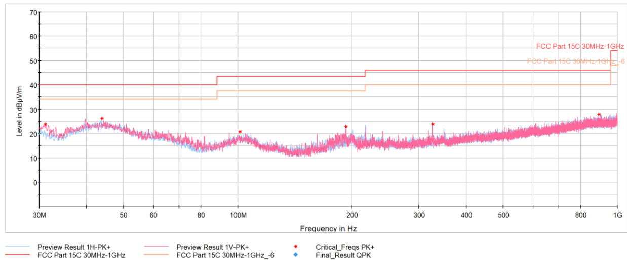
Plot 7-11. Radiated Spurious Emissions 30MHz – 1GHz (Reader A 106kbps, with AC/DC Adapter and Magnetic Charger)
