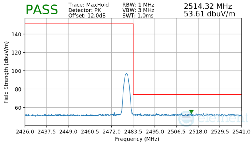
Plot 7-40. Radiated Restricted Upper Band Edge Measurement
