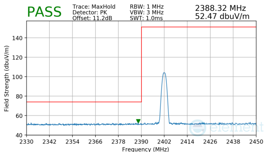
Plot 7-37. Radiated Restricted Lower Band Edge Measurement
