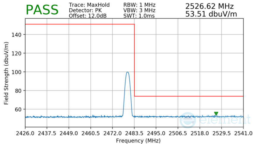
Plot 7-39. Radiated Restricted Upper Band Edge Measurement
