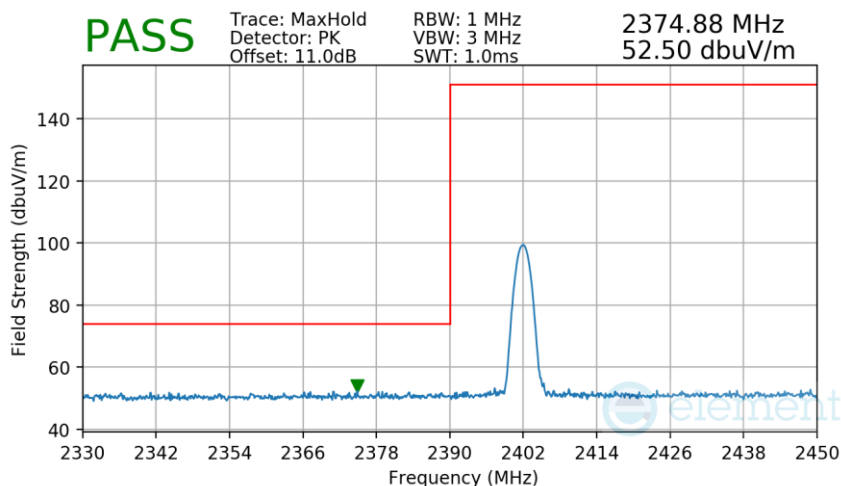
Plot 7-38. Radiated Restricted Lower Band Edge Measurement
