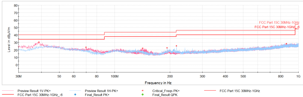
Plot 7-37. Radiated Spurious Emissions Below 1GHz (4Mbps, ePA – Ch.38 with AC/DC adaptor via USB-C cable with magnetic charger)
