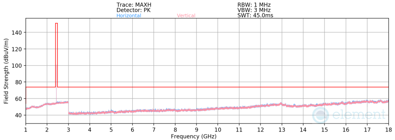
Plot 7-31. Radiated Spurious Emissions 1-18GHz (1Mbps, ePA – Ch. 19)
