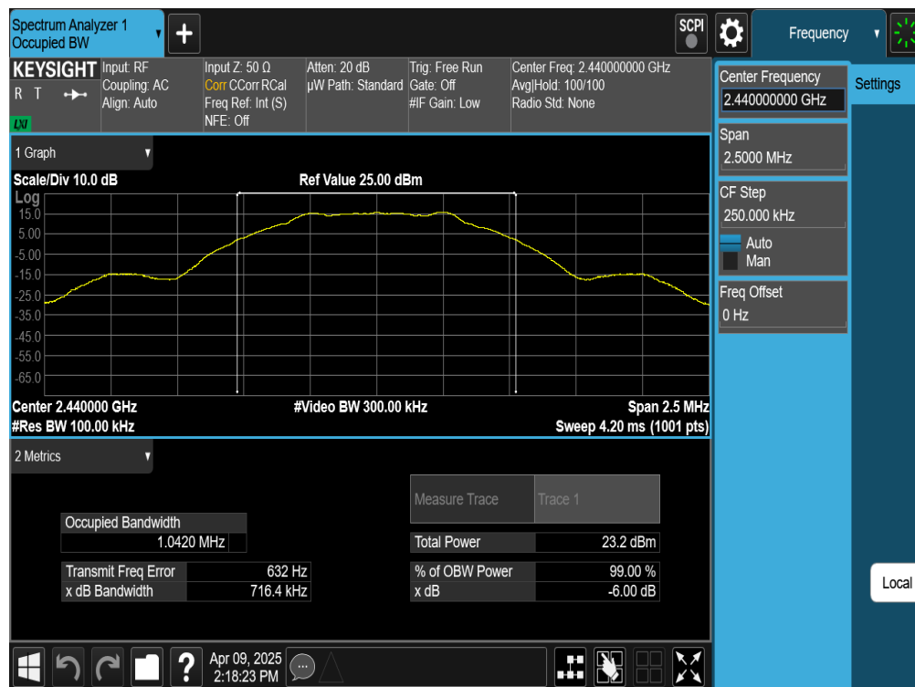
Plot 7-2. 6dB BW & 99% OBW Plot (Bluetooth (LE), 1Mbps, ePA – Ch. 19)
