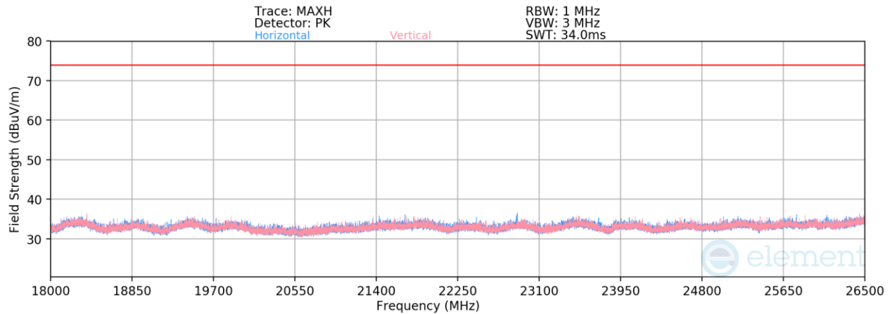
Plot 7-30. Radiated Spurious Emissions above 18GHz (1Mbps ePA – Ch. 0)
