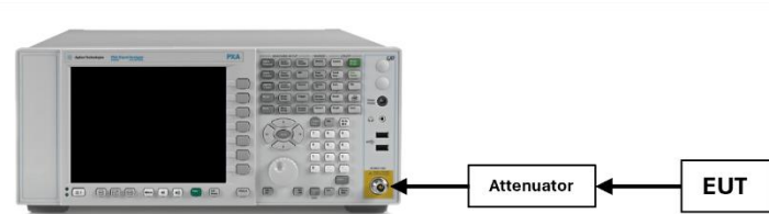
Figure 7-1. Test Instrument & Measurement Setup
