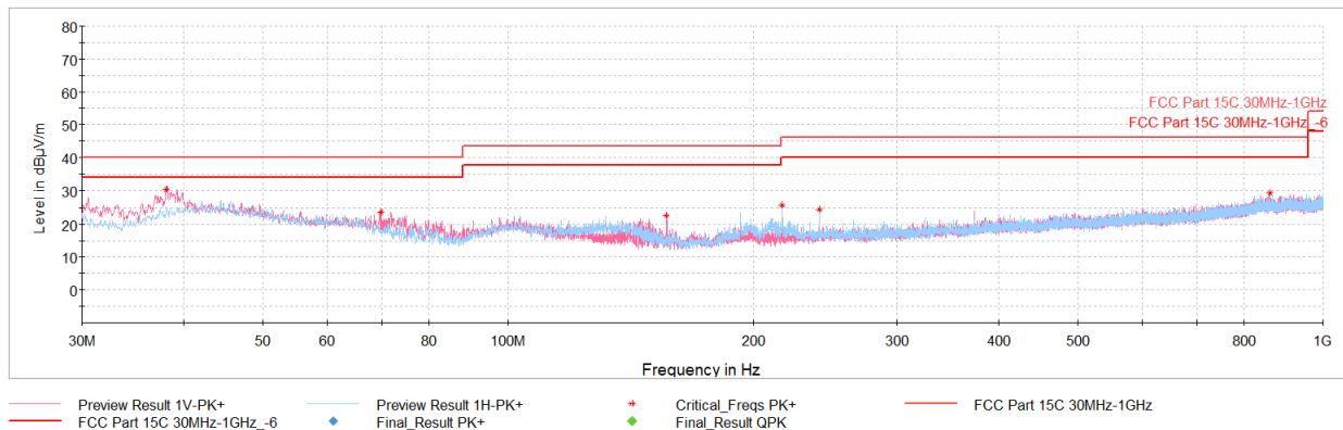
Plot 7-37. Radiated Spurious Emissions Below 1GHz (1Mbps, ePA – Ch.0, Pol. H & V, with AC/DC adaptor via USB-C cable with magnetic charger)
