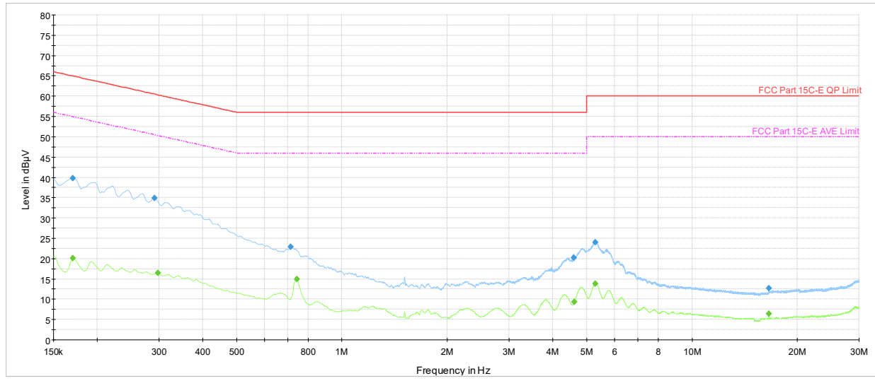
Plot 7-39. AC Line Conducted Plot with Bluetooth LE (N, 1Mbps ePA – Ch.0, with AC/DC adaptor via USB-C cable with magnetic charger)
