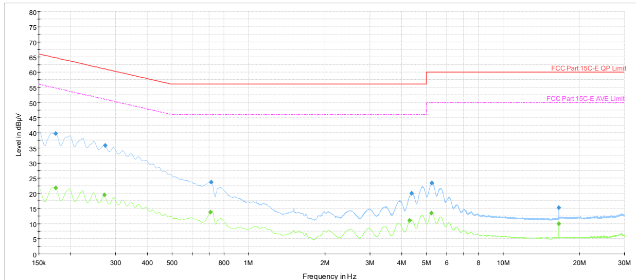
Plot 7-38. AC Line Conducted Plot with Bluetooth LE (L1, 1Mbps ePA – Ch.0 with AC/DC adaptor via USB-C cable with magnetic charger)
