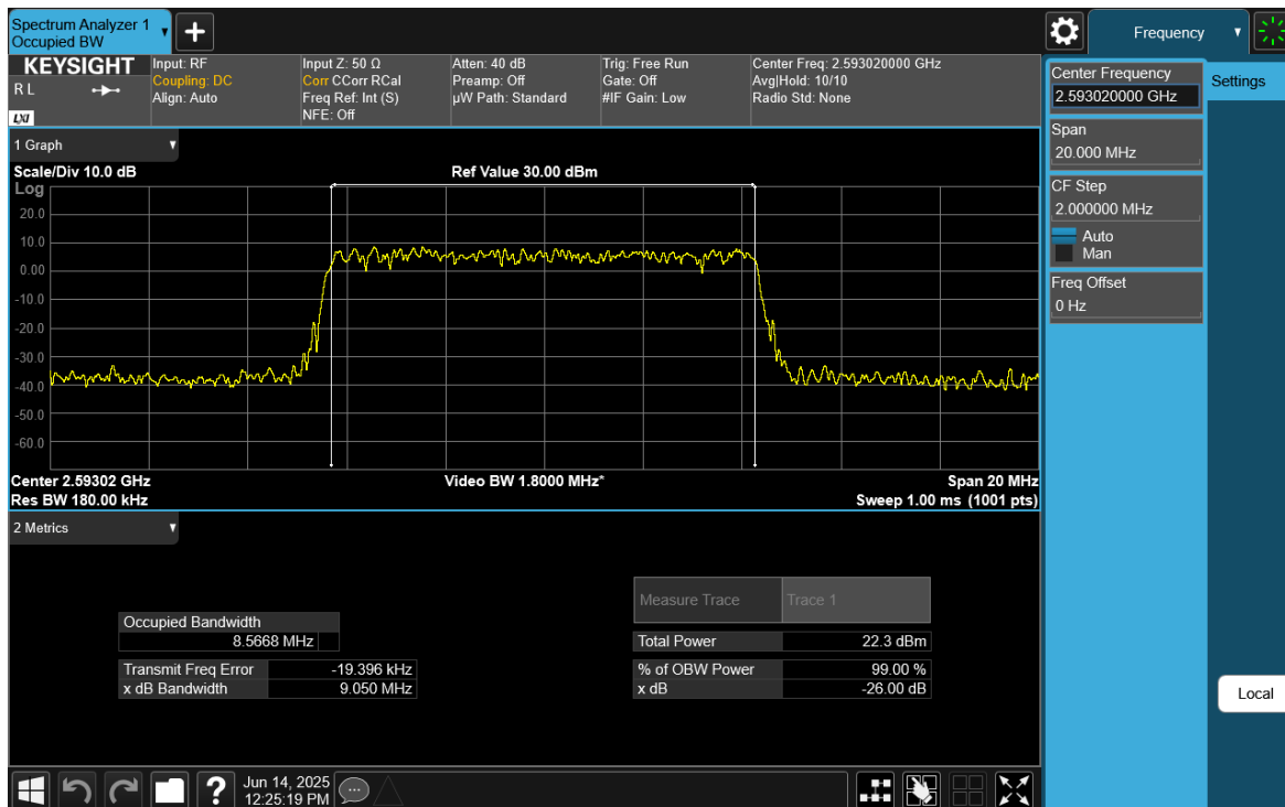
Plot 7-36. Occupied Bandwidth Plot (NR Band n41 - 10MHz DFT-s-OFDM 64-QAM - Full RB)
