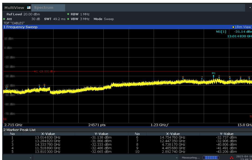
Plot 7-61. Conducted Spurious Plot (LTE Band 41 - 20MHz QPSK - RB Size 1, RB Offset 50 - High Channel)
