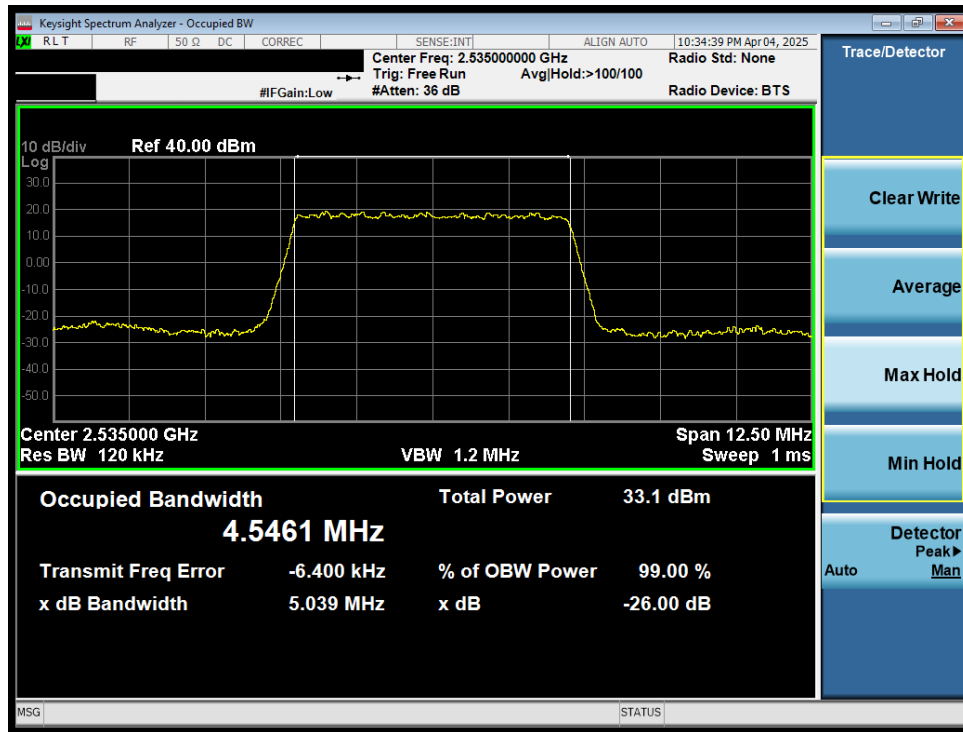
Plot 7-1. Occupied Bandwidth Plot (LTE Band 7 - 5MHz QPSK - Full RB)
