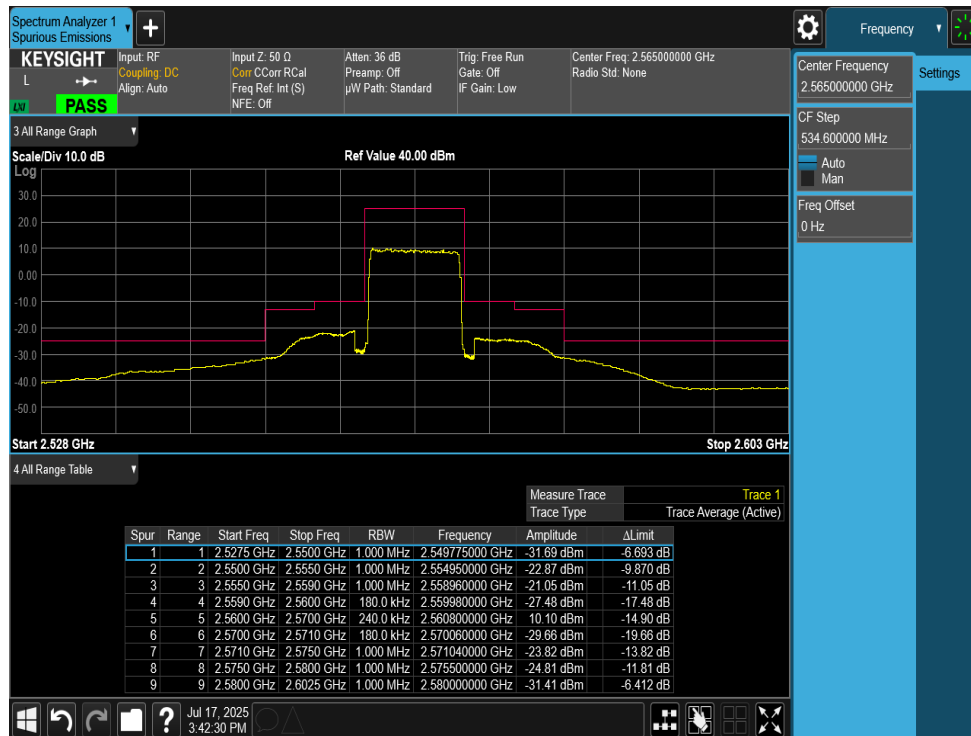
Plot 7-89. Upper Band Edge Plot (LTE Band 7 - 10MHz QPSK – Full RB)
