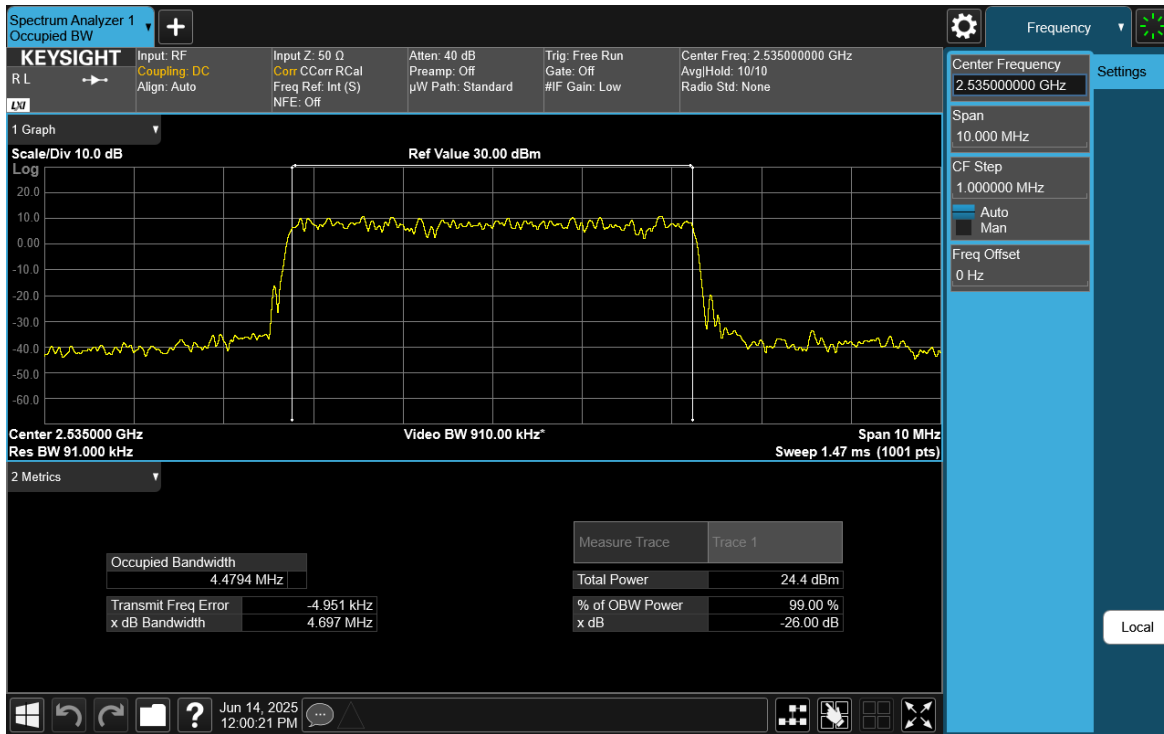
Plot 7-17. Occupied Bandwidth Plot (NR Band n7 - 5MHz DFT-s-OFDM \pi/2 BPSK - Full RB)
