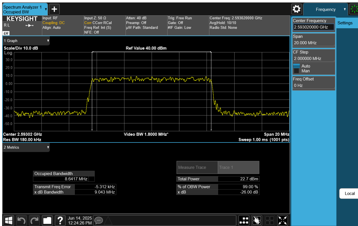
Plot 7-35. Occupied Bandwidth Plot (NR Band n41 - 10MHz DFT-s-OFDM 16-QAM - Full RB)
