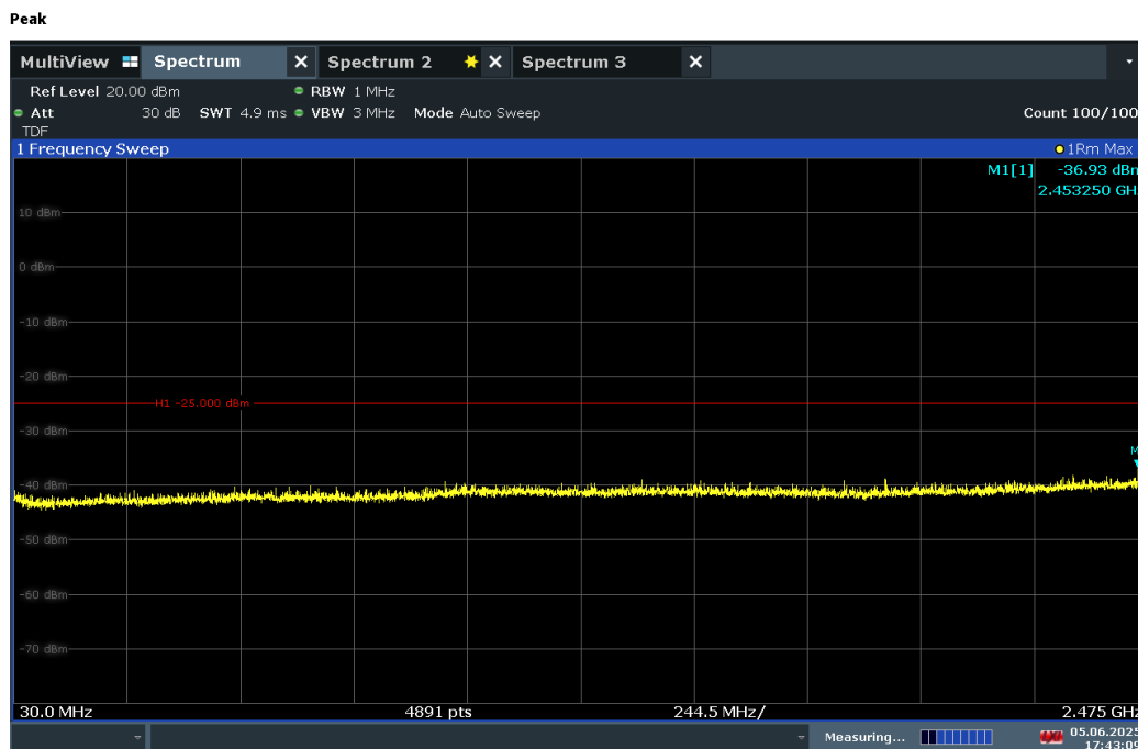
Plot 7-81. Simultaneous Tx Conducted Spurious Plot (LTE Band 41 PC3 + Bluetooth)
