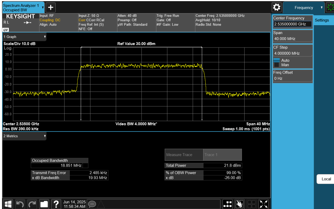
Plot 7-31. Occupied Bandwidth Plot (NR Band n7 - 20MHz CP-OFDM 16-QAM - Full RB)
