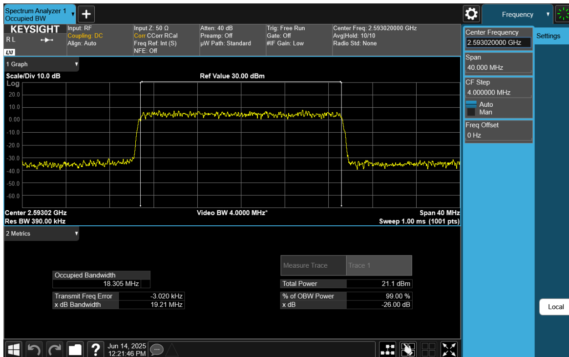
Plot 7-44. Occupied Bandwidth Plot (NR Band n41 - 20MHz CP-OFDM 64-QAM - Full RB)
