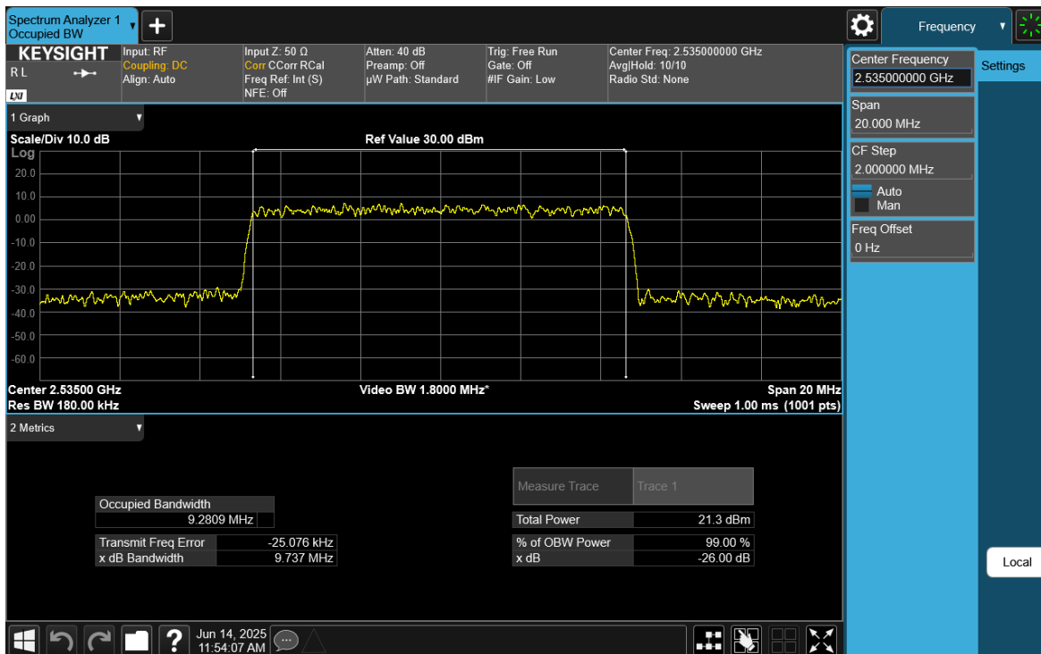
Plot 7-24. Occupied Bandwidth Plot (NR Band n7 - 10MHz CP-OFDM 64-QAM - Full RB)
