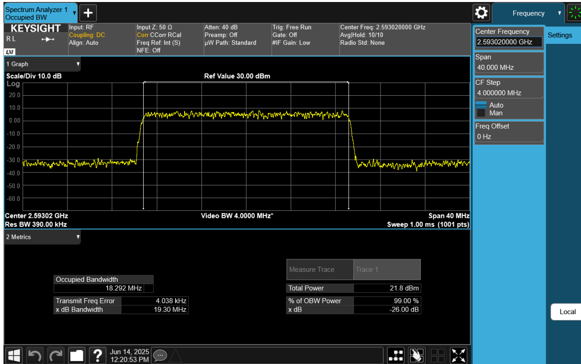
Plot 7-43. Occupied Bandwidth Plot (NR Band n41 - 20MHz CP-OFDM 16-QAM - Full RB)
