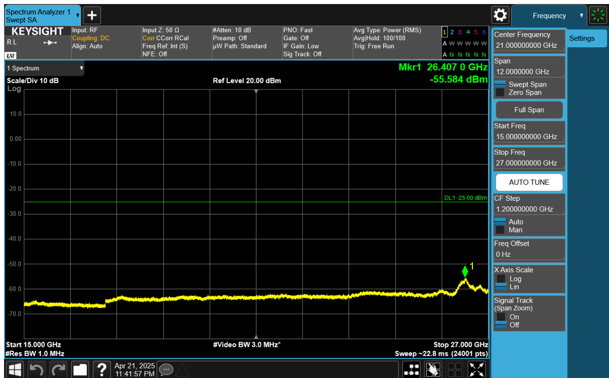
Plot 7-71. Conducted Spurious Plot (NR Band n7 - 20MHz QPSK - RB Size 1, RB Offset 50 - High Channel)
