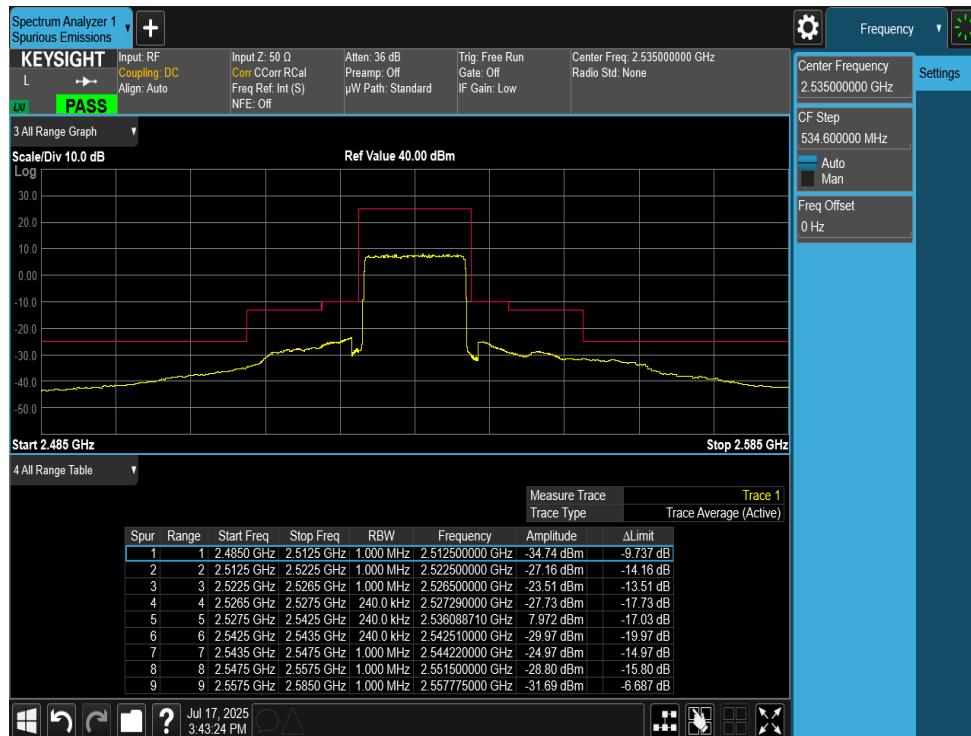
Plot 7-91. Mid Band Edge Plot (LTE Band 7 - 15MHz QPSK – Full RB)
