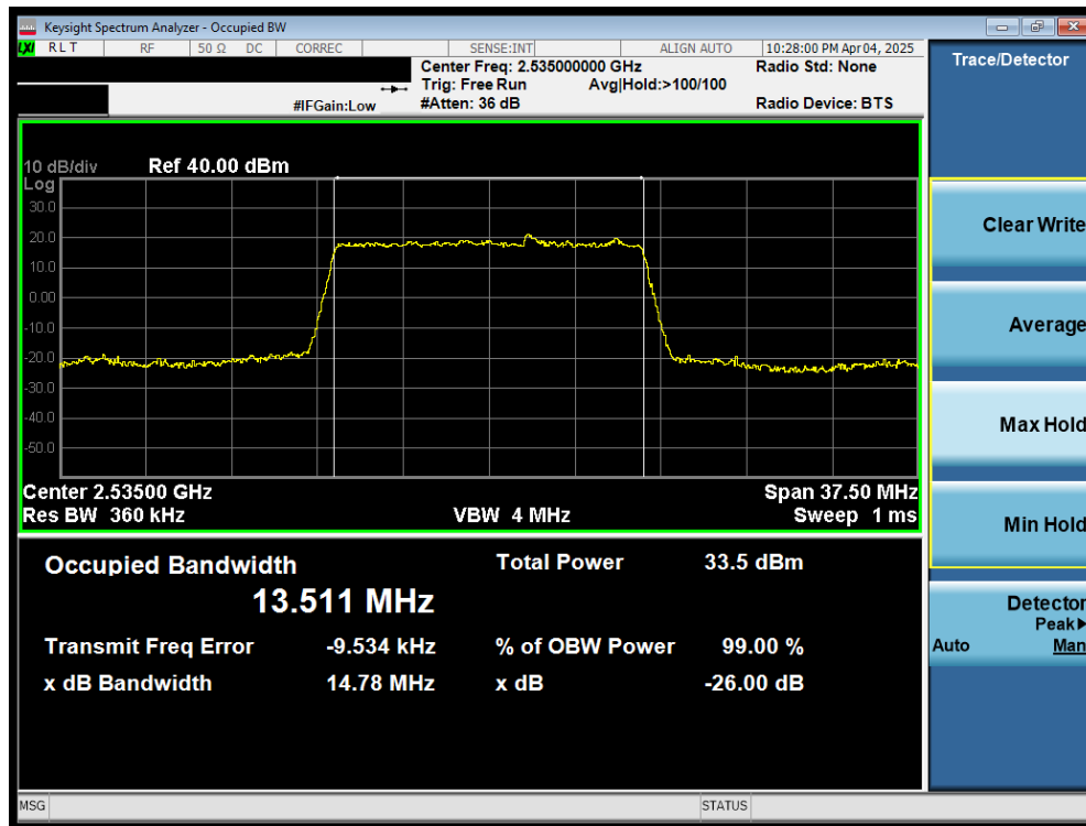
Plot 7-5. Occupied Bandwidth Plot (LTE Band 7 - 15MHz QPSK - Full RB)
