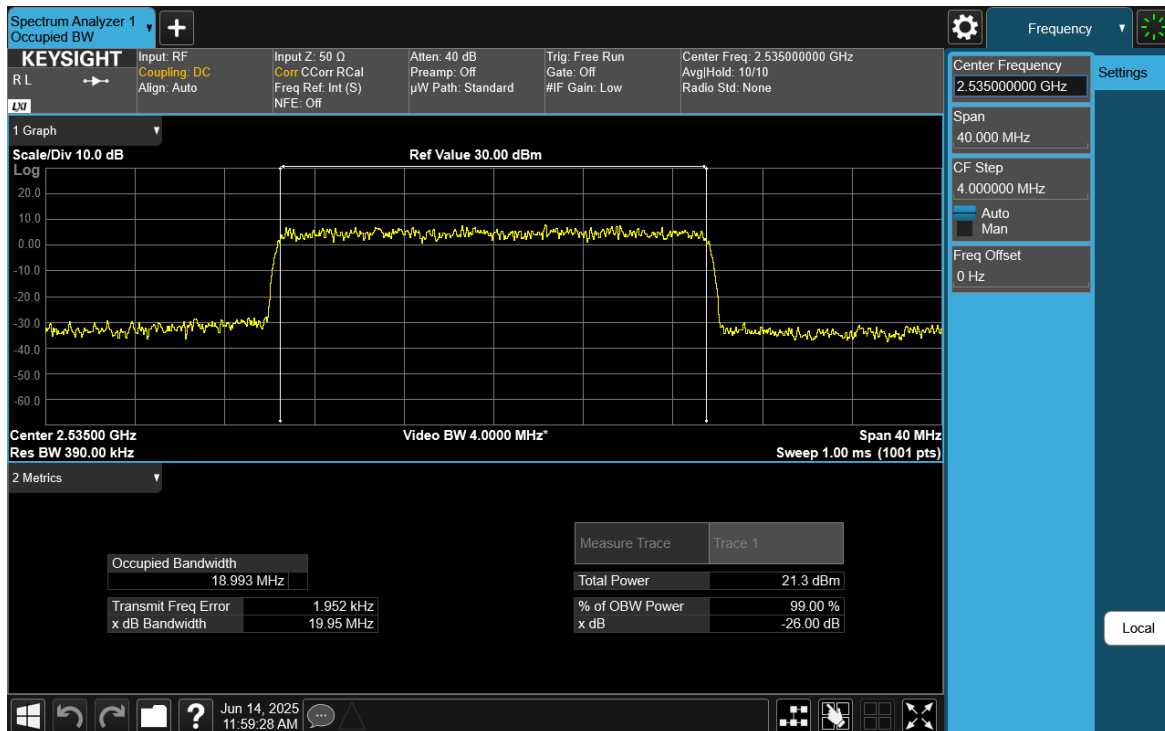
Plot 7-32. Occupied Bandwidth Plot (NR Band n7 - 20MHz CP-OFDM 64-QAM - Full RB)
