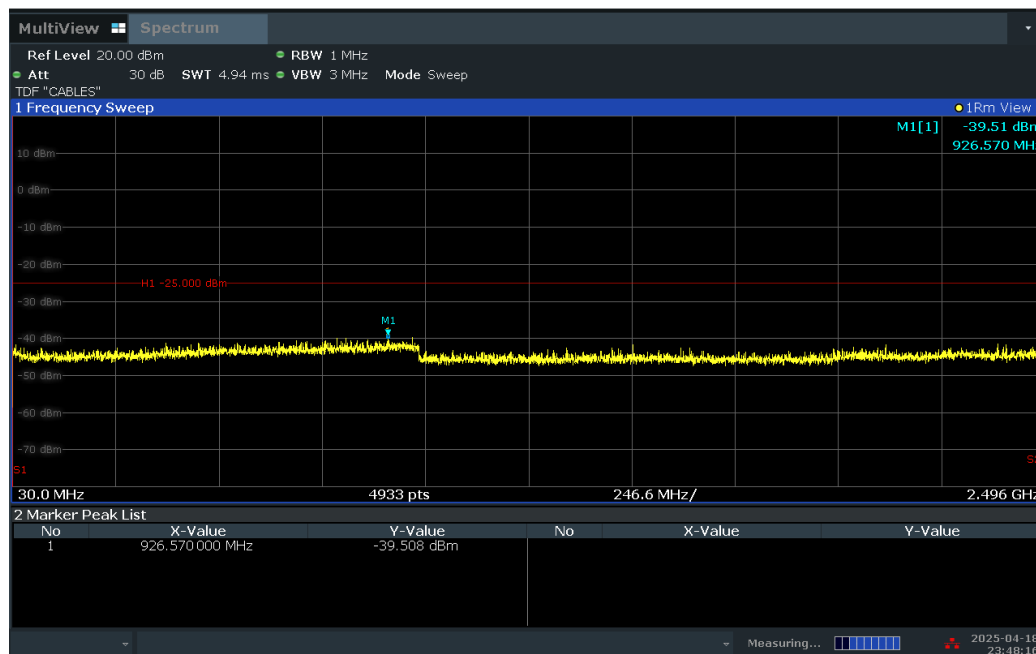
Plot 7-60. Conducted Spurious Plot (LTE Band 41 - 20MHz QPSK - RB Size 1, RB Offset 50 - High Channel)
