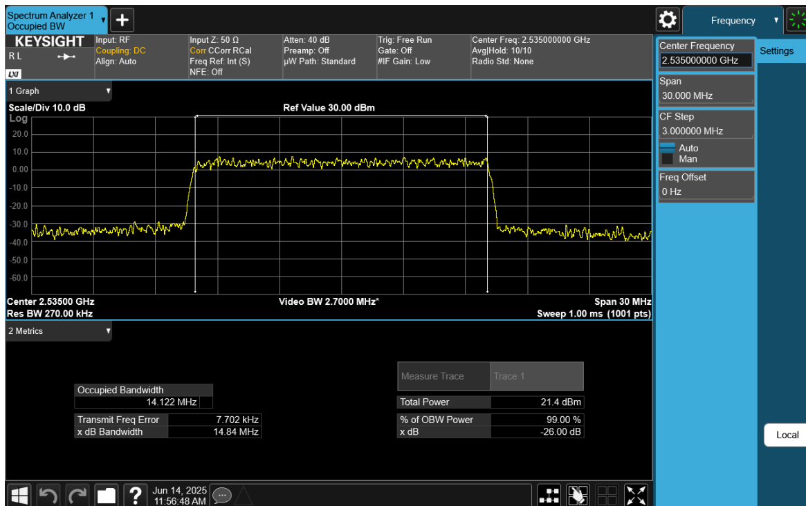
Plot 7-28. Occupied Bandwidth Plot (NR Band n7 - 15MHz CP-OFDM 64-QAM - Full RB)
