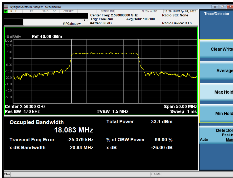
Plot 7-15. Occupied Bandwidth Plot (LTE Band 41 - 20MHz QPSK - Full RB)
