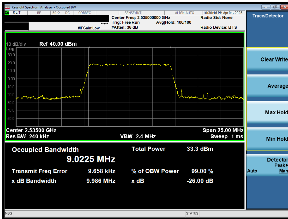
Plot 7-3. Occupied Bandwidth Plot (LTE Band 7 - 10MHz QPSK - Full RB)
