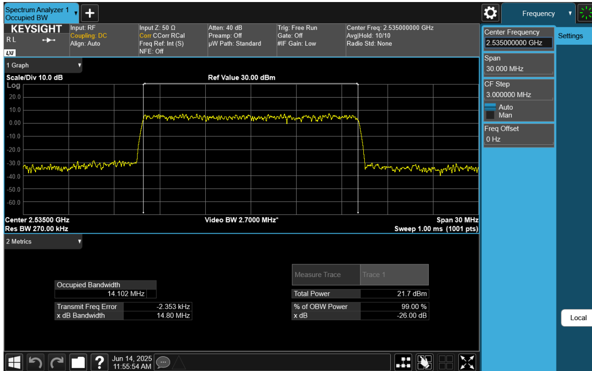
Plot 7-27. Occupied Bandwidth Plot (NR Band n7 - 15MHz CP-OFDM 16-QAM - Full RB)
