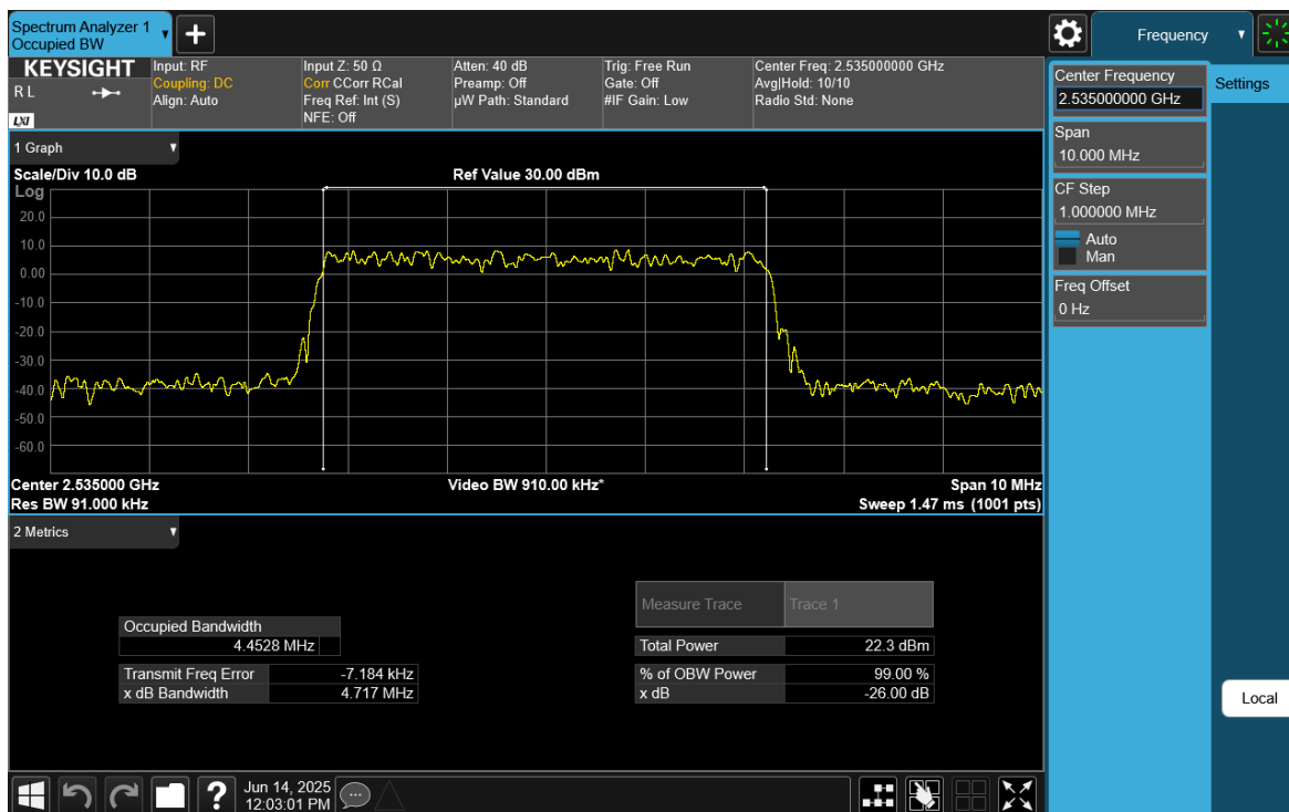
Plot 7-20. Occupied Bandwidth Plot (NR Band n7 - 5 MHz DFT-s-OFDM 64-QAM - Full RB)
