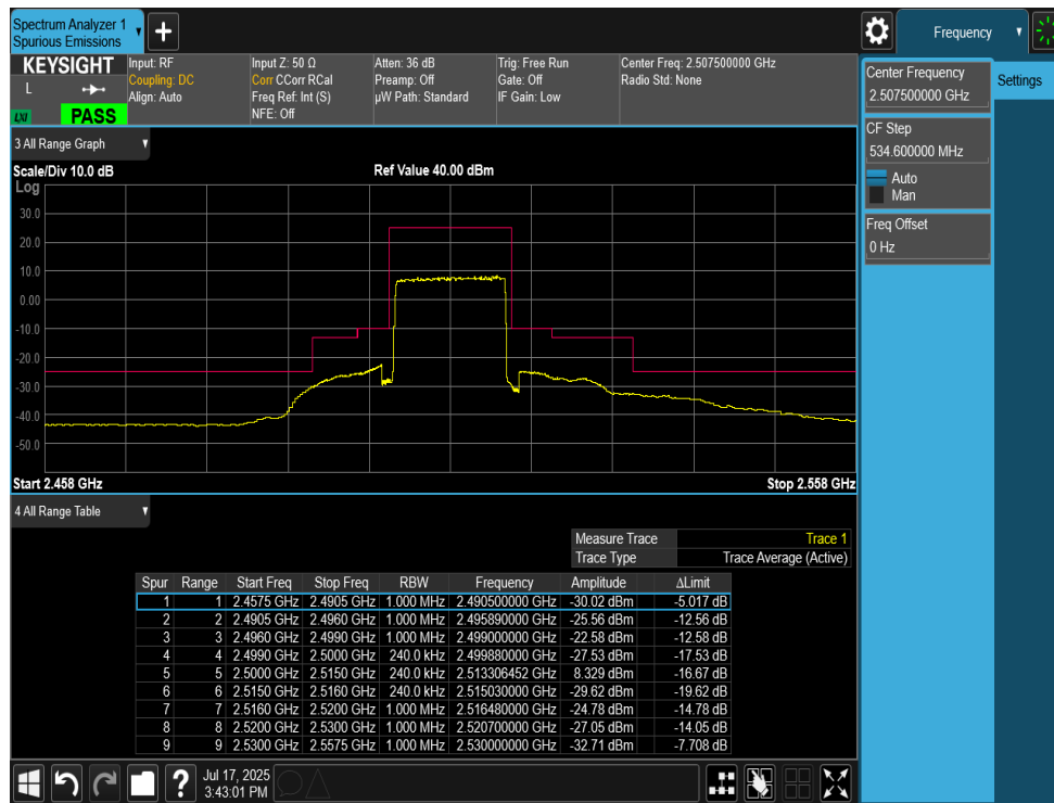
Plot 7-90. Lower Band Edge Plot (LTE Band 7 - 15MHz QPSK – Full RB)
