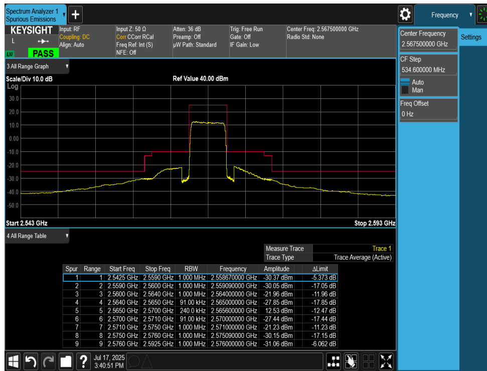
Plot 7-86. Upper Band Edge Plot (LTE Band 7 - 5MHz QPSK – Full RB)
