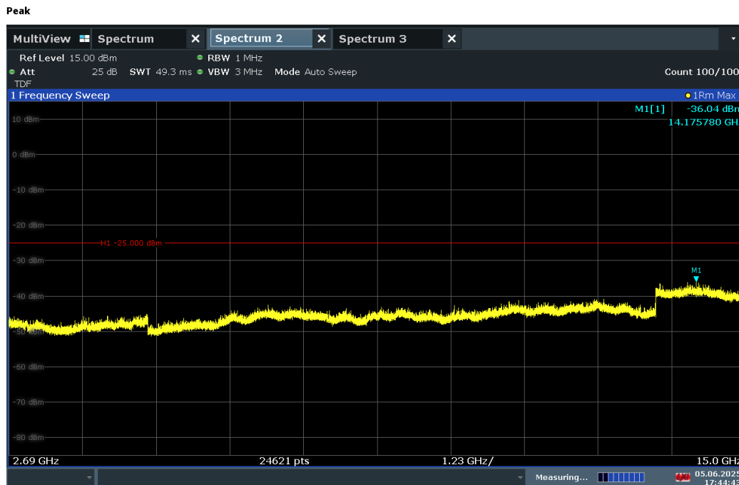
Plot 7-82. Simultaneous Tx Conducted Spurious Plot (LTE Band 41 PC3 + Bluetooth)
