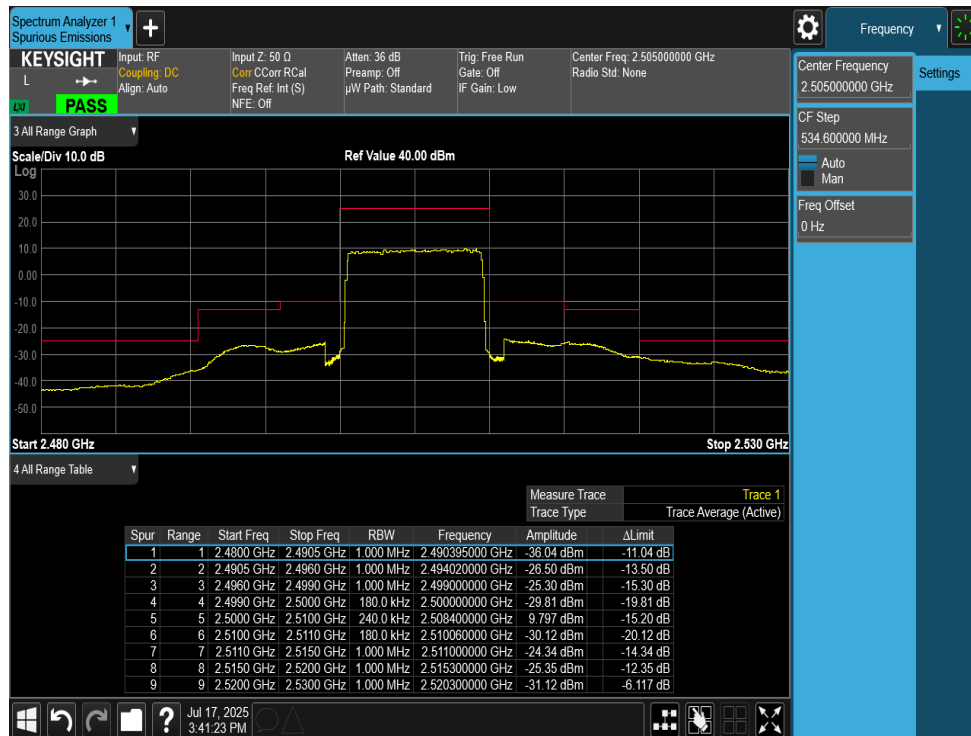
Plot 7-87. Lower Band Edge Plot (LTE Band 7 - 10MHz QPSK – Full RB)
