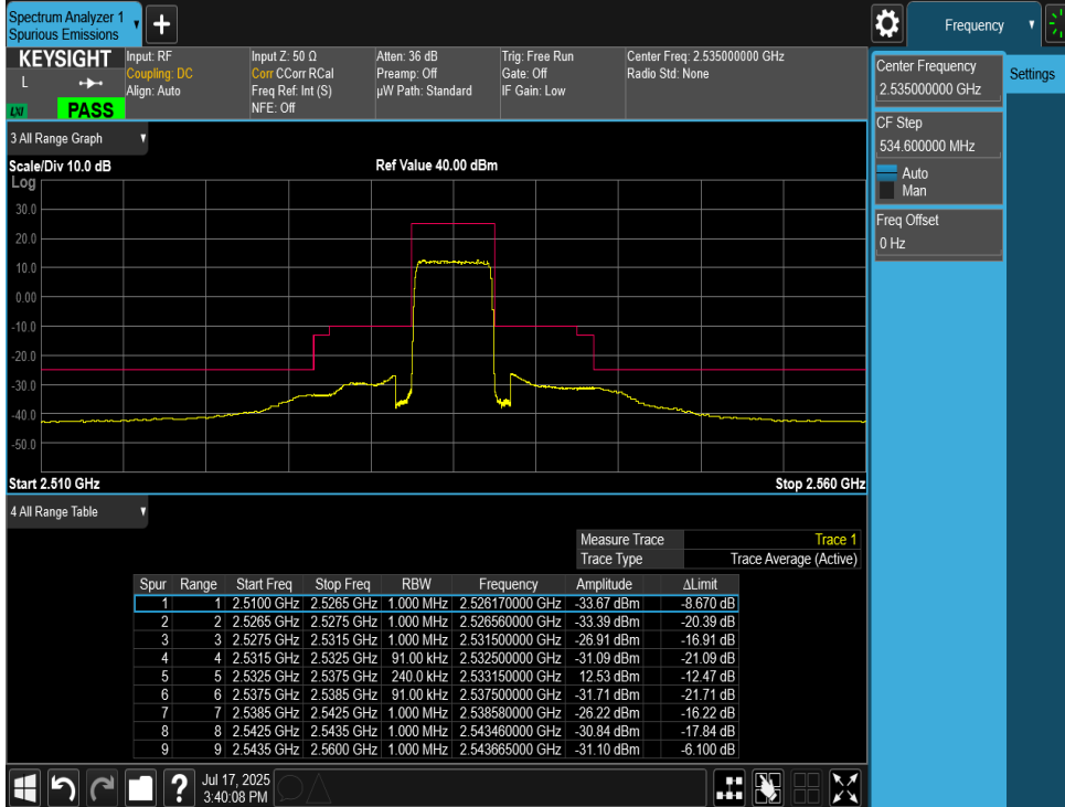
Plot 7-85. Mid Band Edge Plot (LTE Band 7 - 5MHz QPSK – Full RB)
