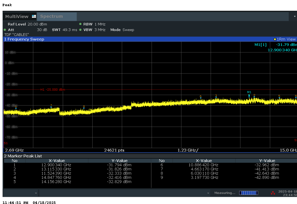
Plot 7-55. Conducted Spurious Plot (LTE Band 41 - 20MHz QPSK - RB Size 1, RB Offset 50 - Low Channel)
