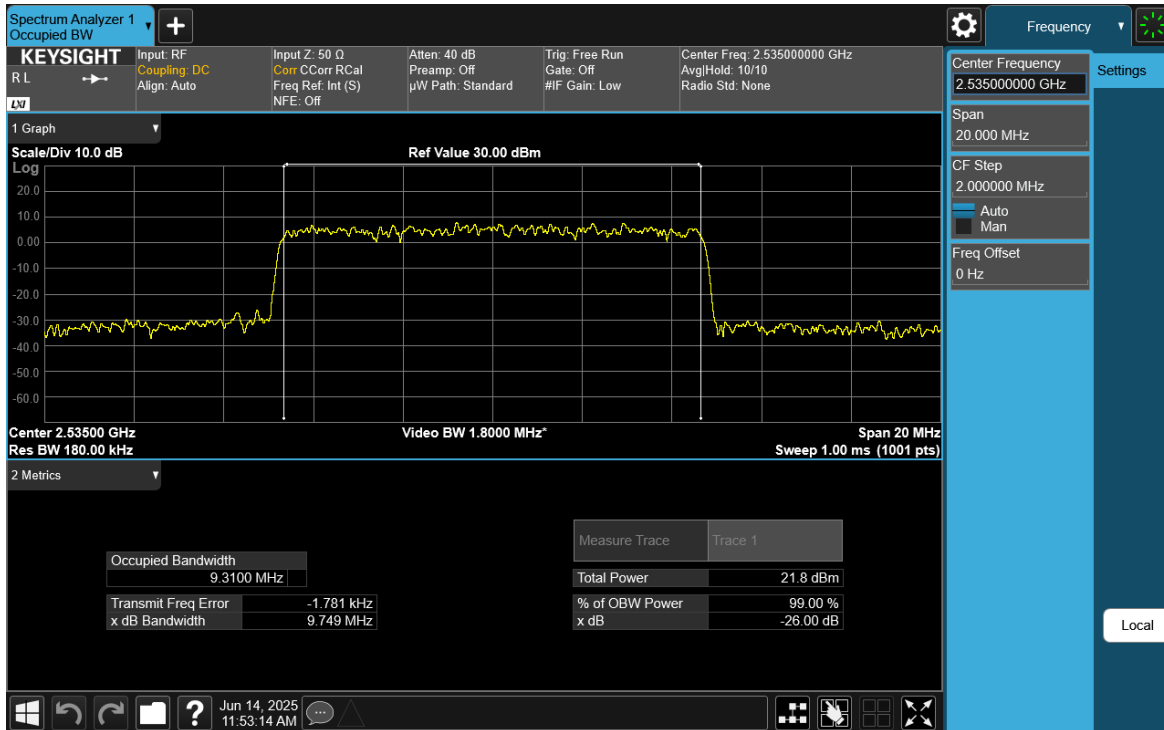
Plot 7-23. Occupied Bandwidth Plot (NR Band n7 - 10MHz CP-OFDM 16-QAM - Full RB)
