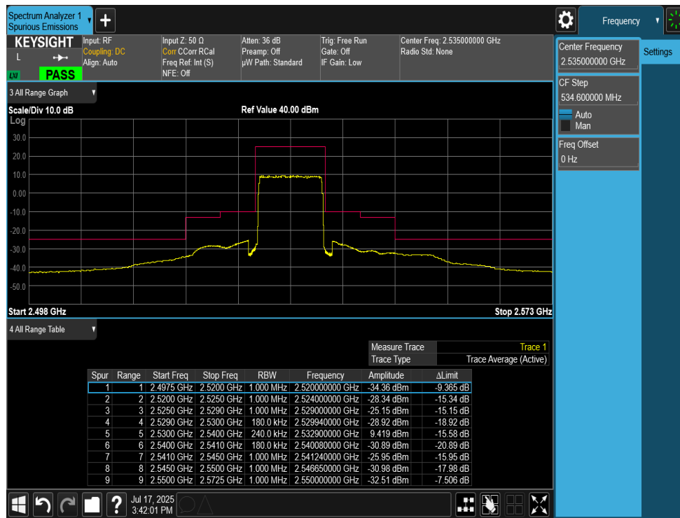
Plot 7-88. Mid Band Edge Plot (LTE Band 7 - 10MHz QPSK – Full RB)
