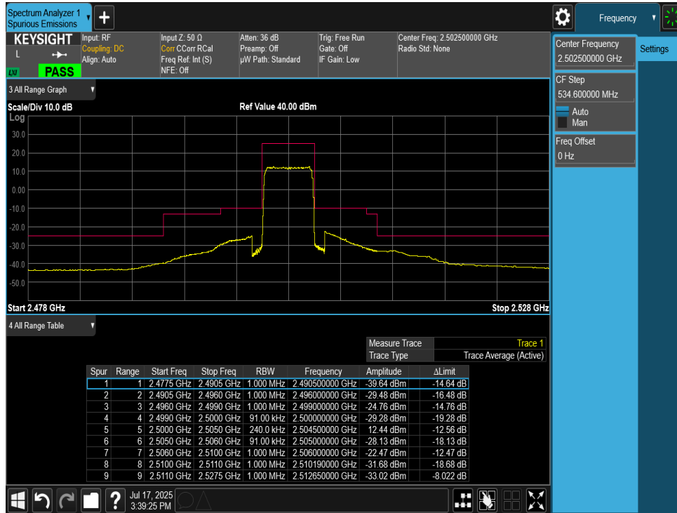
Plot 7-84. Lower Band Edge Plot (LTE Band 7 - 5MHz QPSK – Full RB)
