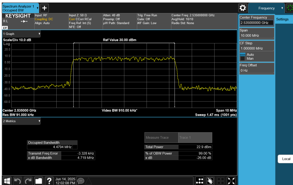
Plot 7-19. Occupied Bandwidth Plot (NR Band n7 - 5MHz DFT-s-OFDM 16-QAM - Full RB)
