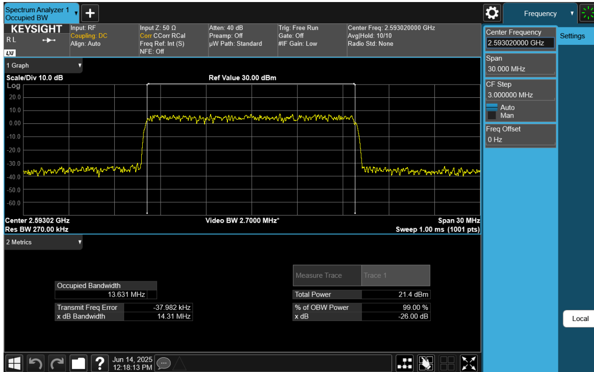
Plot 7-39. Occupied Bandwidth Plot (NR Band n41 - 15MHz CP-OFDM 16-QAM - Full RB)
