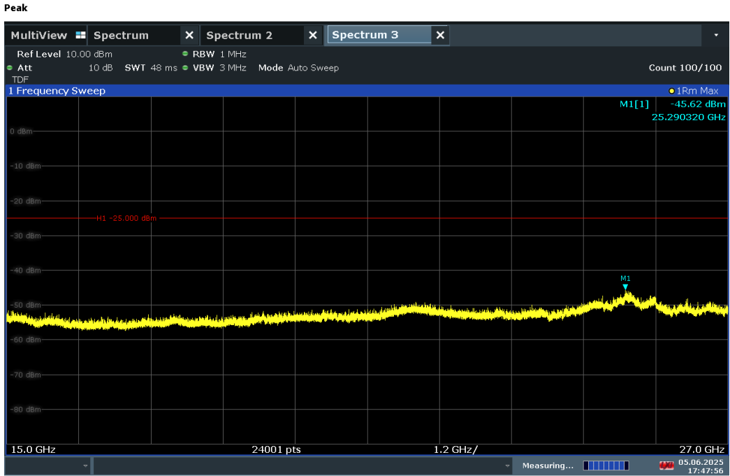
Plot 7-83. Simultaneous Tx Conducted Spurious Plot (LTE Band 41 PC3 + Bluetooth)
