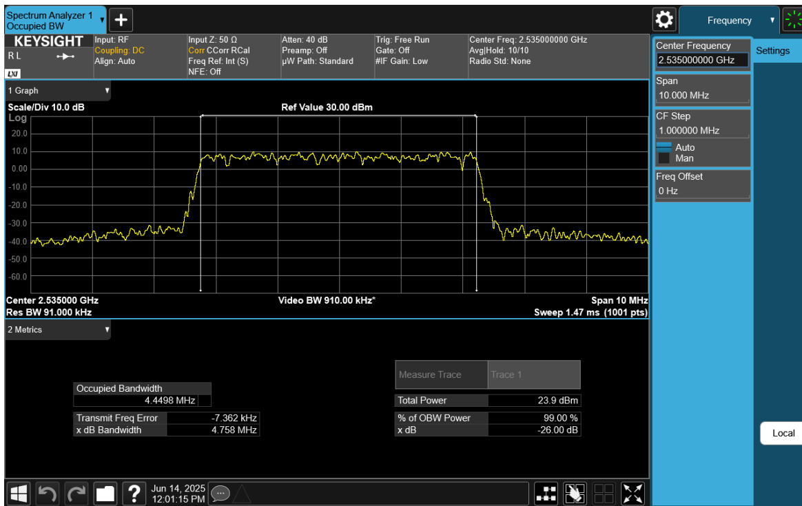
Plot 7-18. Occupied Bandwidth Plot (NR Band n7 - 5MHz DFT-s-OFDM QPSK - Full RB)
