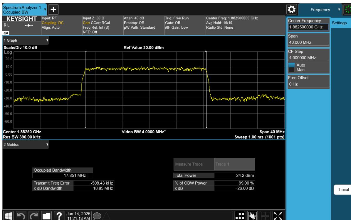
Plot 7-25. Occupied Bandwidth Plot (NR Band n25/n2 - 20MHz DFT-s-OFDM \pi/2 BPSK - Full RB)
