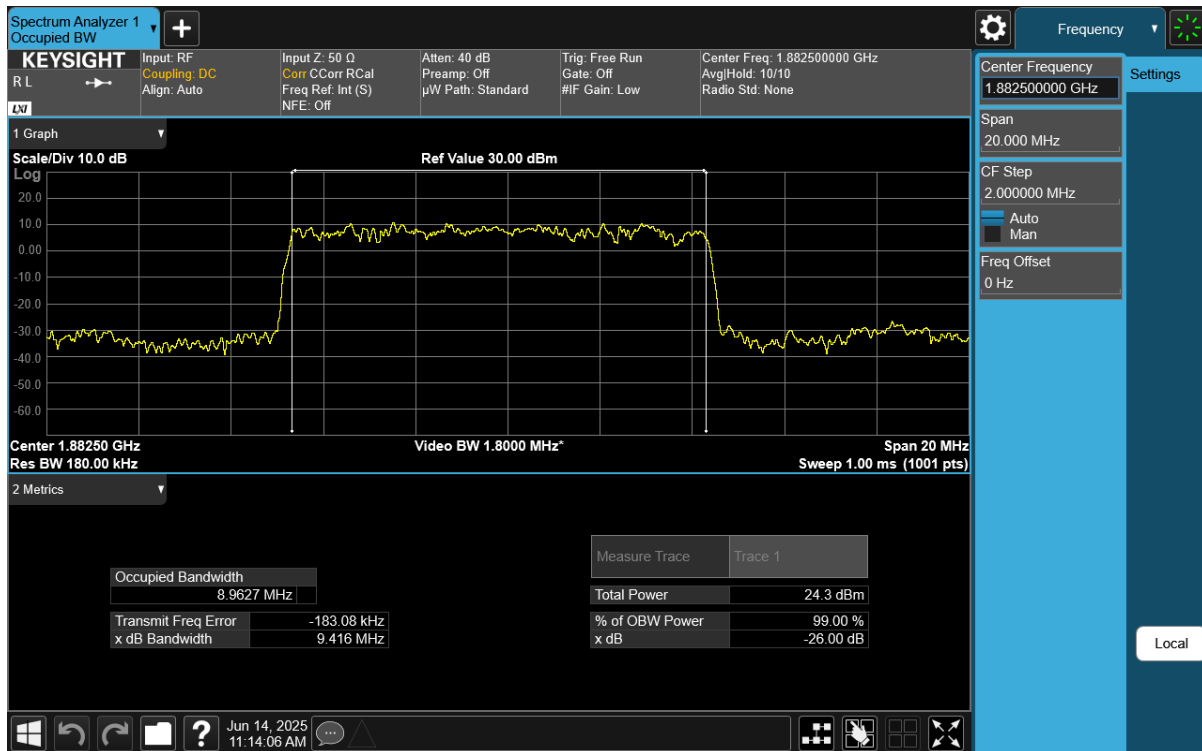
Plot 7-17. Occupied Bandwidth Plot (NR Band n25/n2 - 10MHz DFT-s-OFDM \pi/2 BPSK - Full RB)
