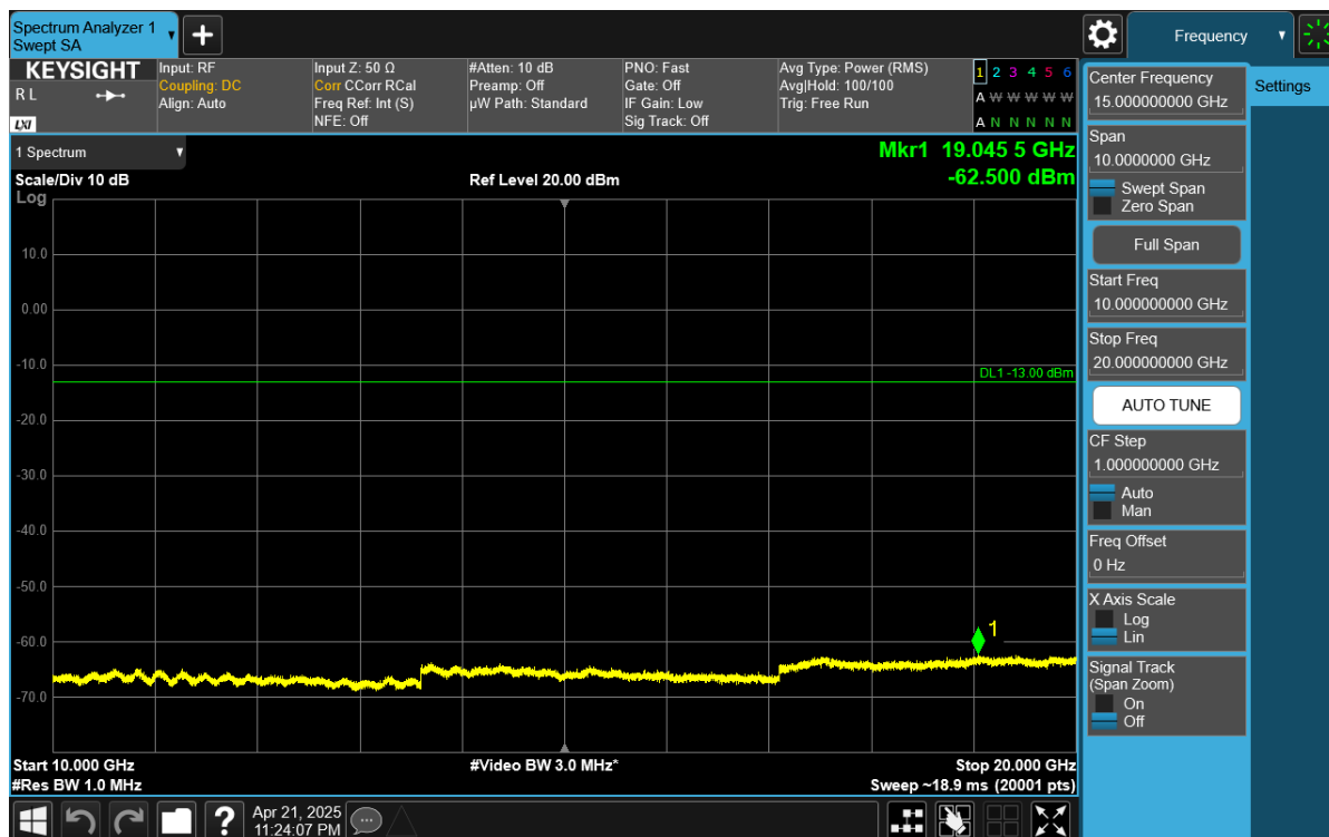
Plot 7-46. Conducted Spurious Plot (NR Band n25/n2 - 20MHz - RB Size 1, RB Offset 50 - High Channel)
