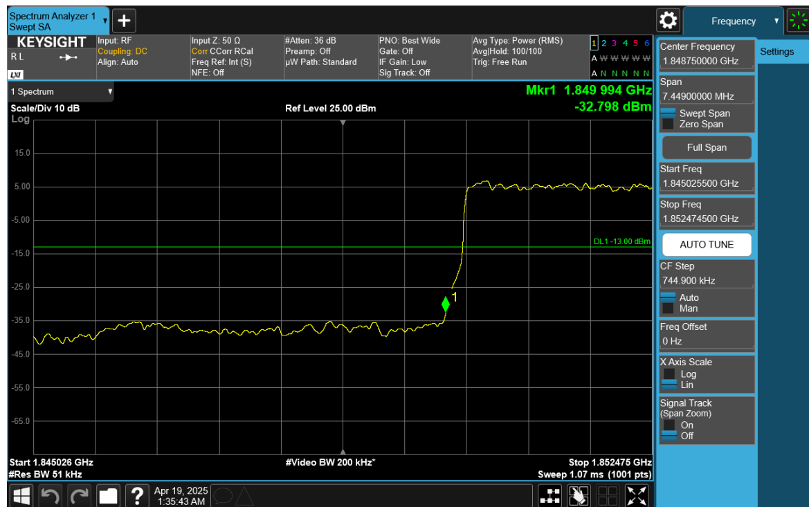
Plot 7-96. Lower Band Edge Plot (NR Band n25 – 5MHz DFT-S-OFDM \pi/2 BPSK – Full RB Configuration)
