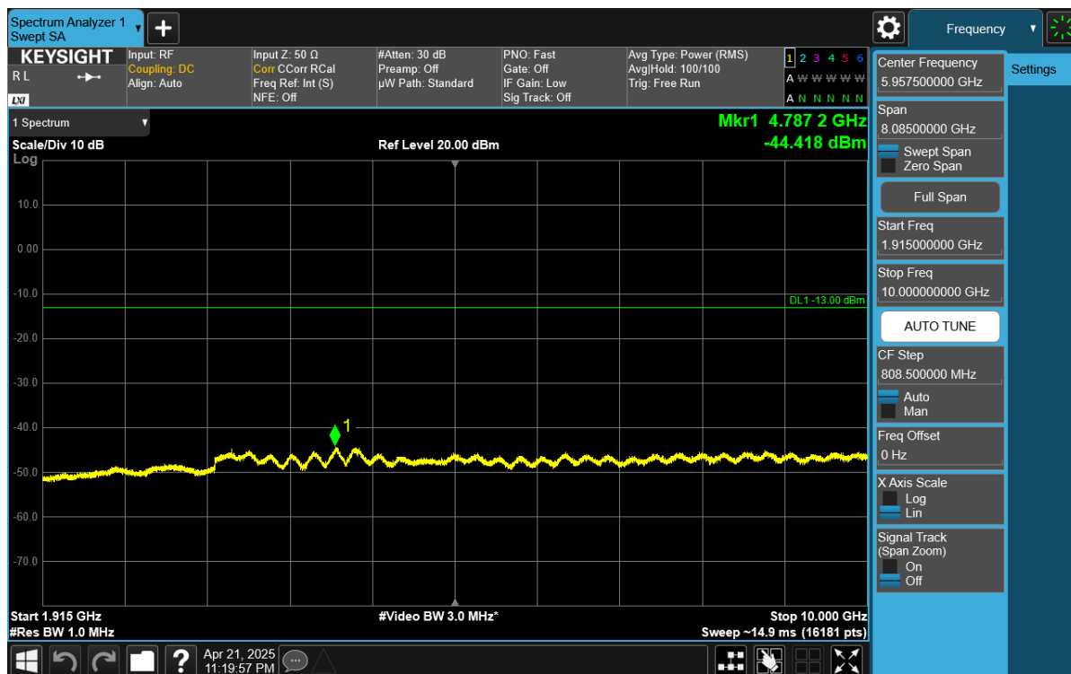
Plot 7-42. Conducted Spurious Plot (NR Band n25/n2 - 20MHz - RB Size 1, RB Offset 50 - Mid Channel)
