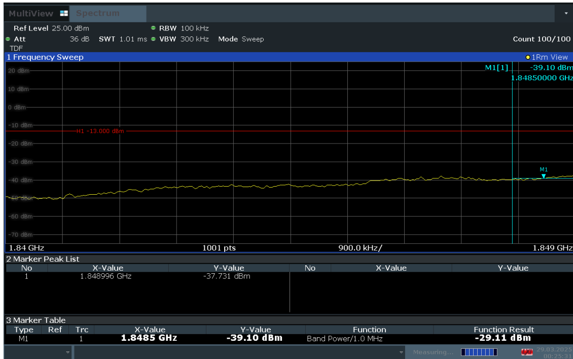
Plot 7-79. Extended Lower Band Edge Plot (LTE Band 2 – 5MHz QPSK – Full RB Configuration)
