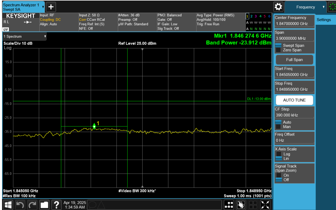
Plot 7-95. Extended Lower Band Edge Plot (NR Band n25 – 5MHz DFT-S-OFDM \pi/2 BPSK – Full RB Configuration)
