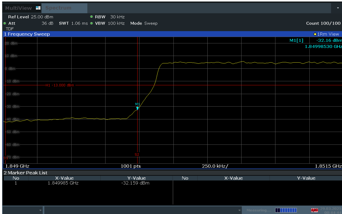
Plot 7-51. Extended Lower Band Edge Plot (LTE Band 25 – 3MHz QPSK – Full RB Configuration)
