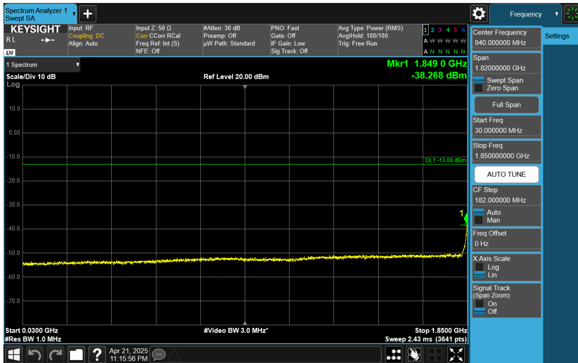
Plot 7-38. Conducted Spurious Plot (NR Band n25/n2 - 20MHz - RB Size 1, RB Offset 50 - Low Channel)
