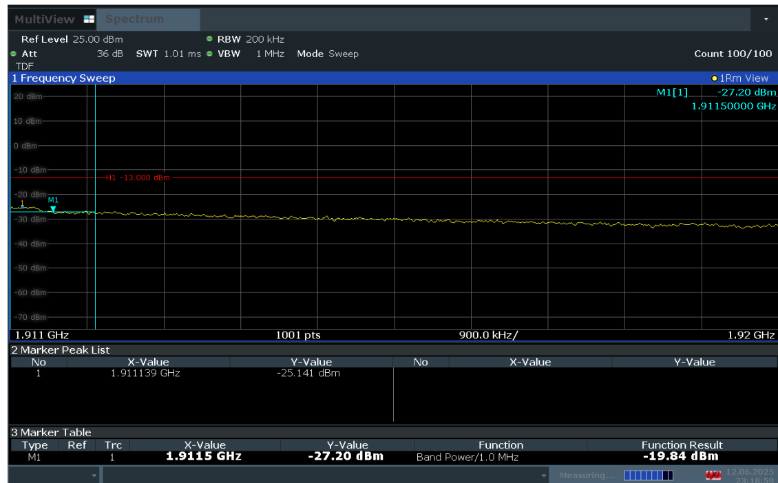
Plot 7-94. Extended Upper Band Edge Plot (LTE Band 2 – 20MHz QPSK – Full RB Configuration)
