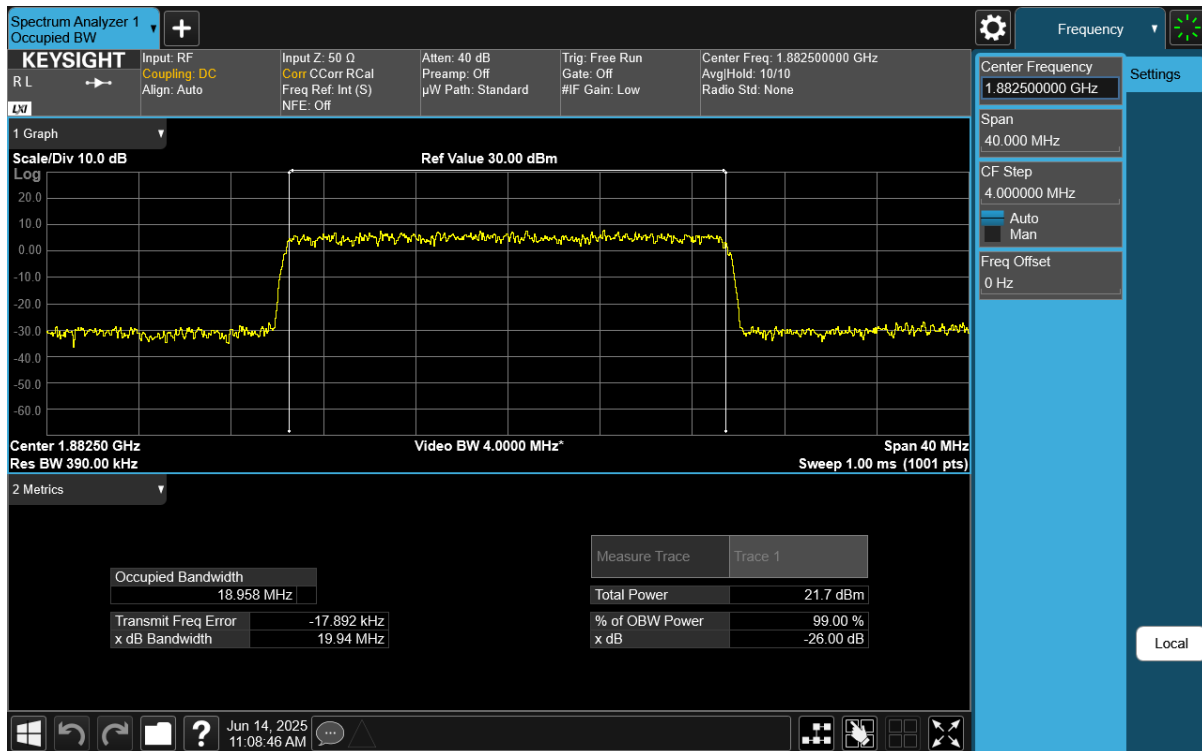
Plot 7-27. Occupied Bandwidth Plot (NR Band n25/n2 - 20MHz CP-OFDM 16QAM - Full RB)
