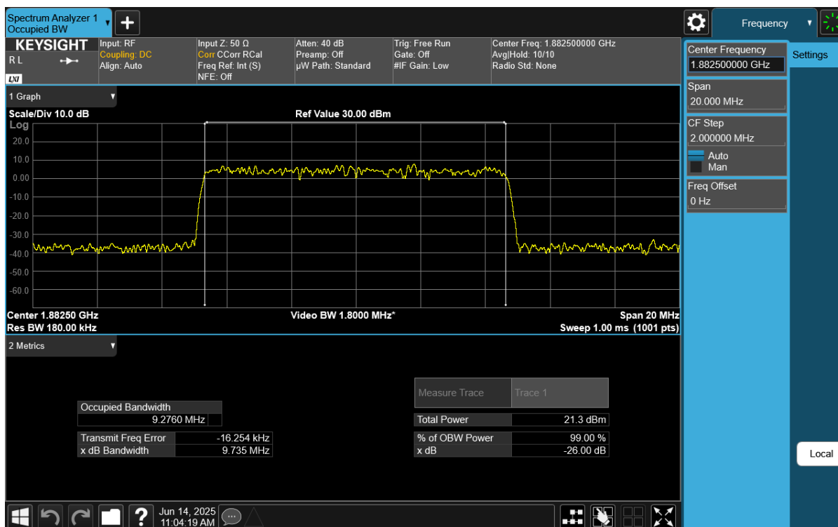
Plot 7-20. Occupied Bandwidth Plot (NR Band n25/n2 - 10MHz CP-OFDM 64QAM - Full RB)
