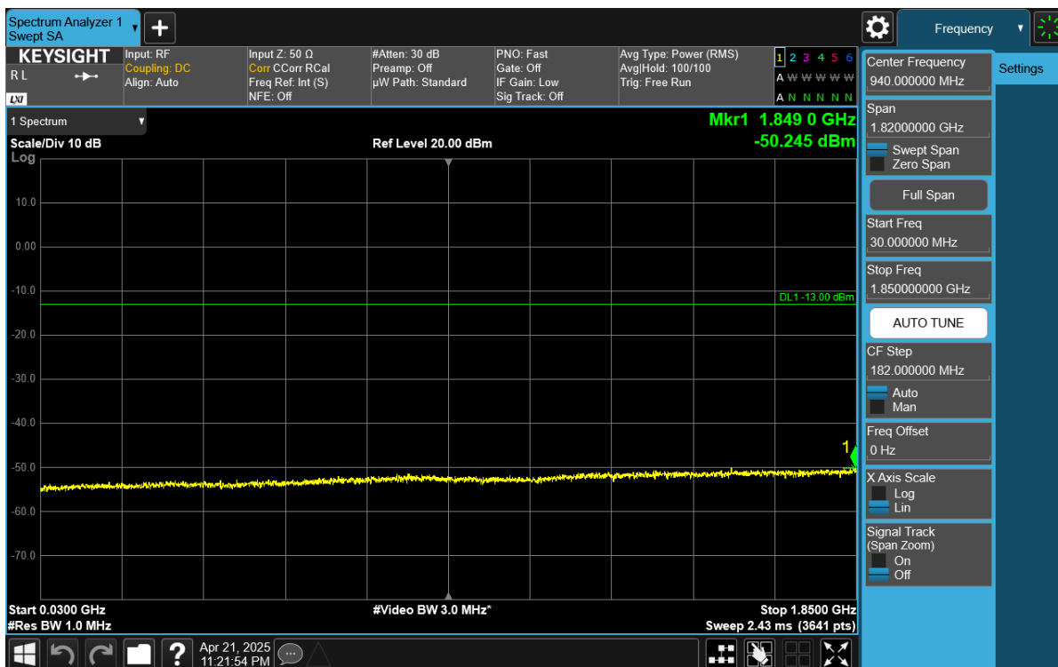
Plot 7-44. Conducted Spurious Plot (NR Band n25/n2 - 20MHz - RB Size 1, RB Offset 50 - High Channel)
