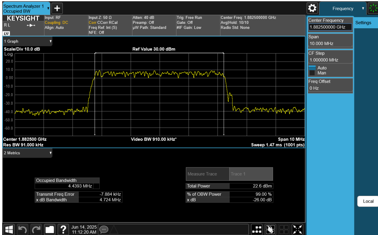
Plot 7-15. Occupied Bandwidth Plot (NR Band n25/n2 - 5MHz DFT-s-OFDM 16QAM - Full RB)
