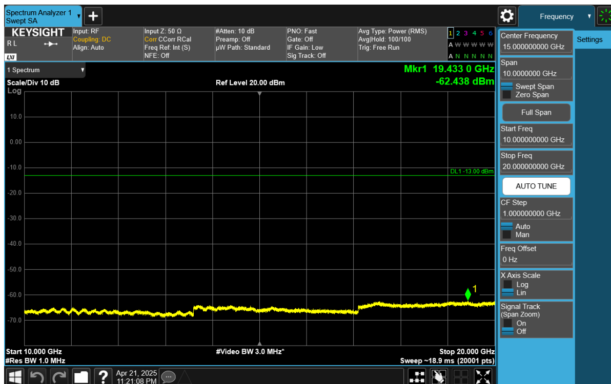
Plot 7-43. Conducted Spurious Plot (NR Band n25/n2 - 20MHz - RB Size 1, RB Offset 50 - Mid Channel)
