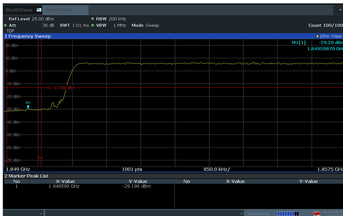
Plot 7-87. Extended Lower Band Edge Plot (LTE Band 2 – 15MHz QPSK – Full RB Configuration)
