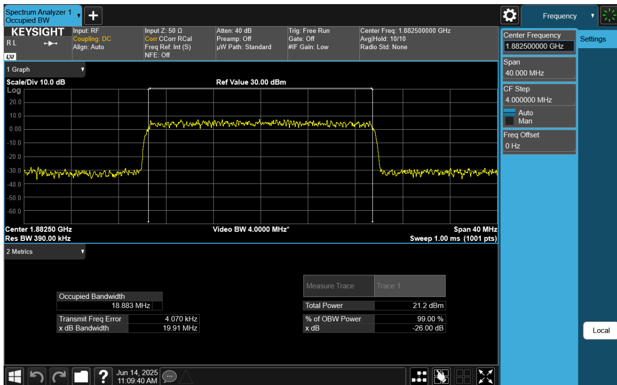
Plot 7-28. Occupied Bandwidth Plot (NR Band n25/n2 - 20MHz CP-OFDM 64QAM - Full RB)
