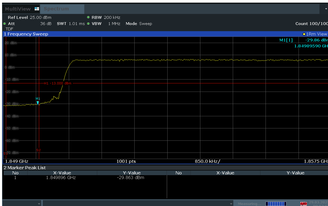
Plot 7-63. Extended Lower Band Edge Plot (LTE Band 25 – 15MHz QPSK – Full RB Configuration)
