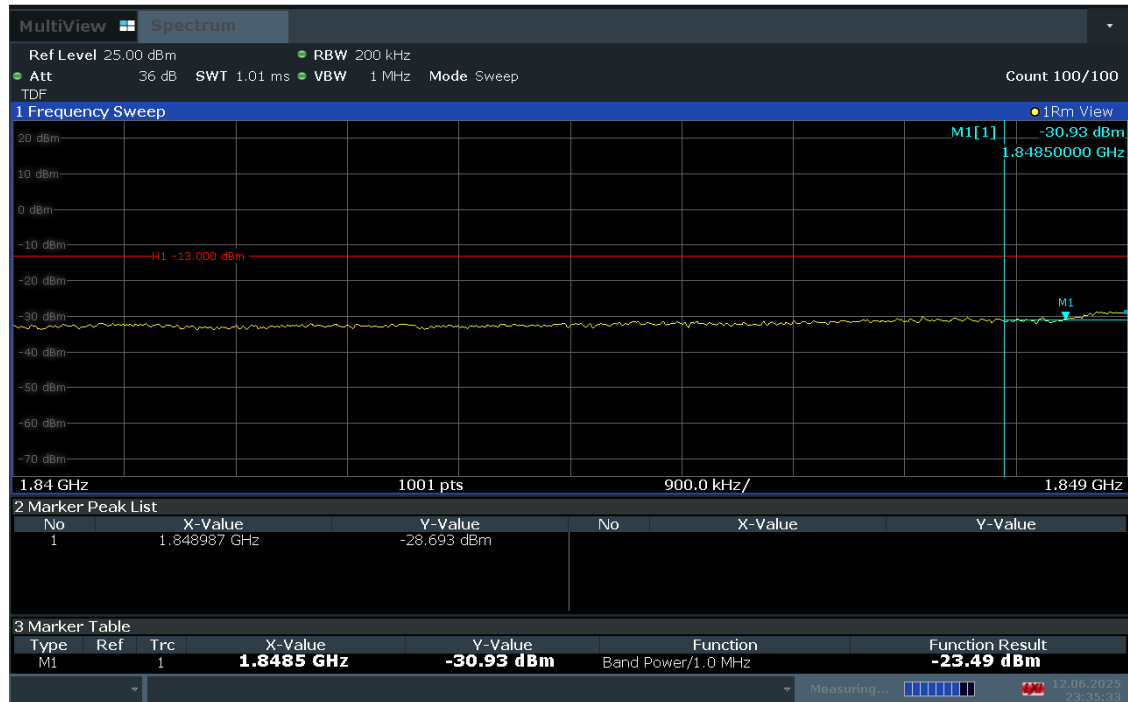
Plot 7-67. Extended Lower Band Edge Plot (LTE Band 25 – 20MHz QPSK – Full RB Configuration)
