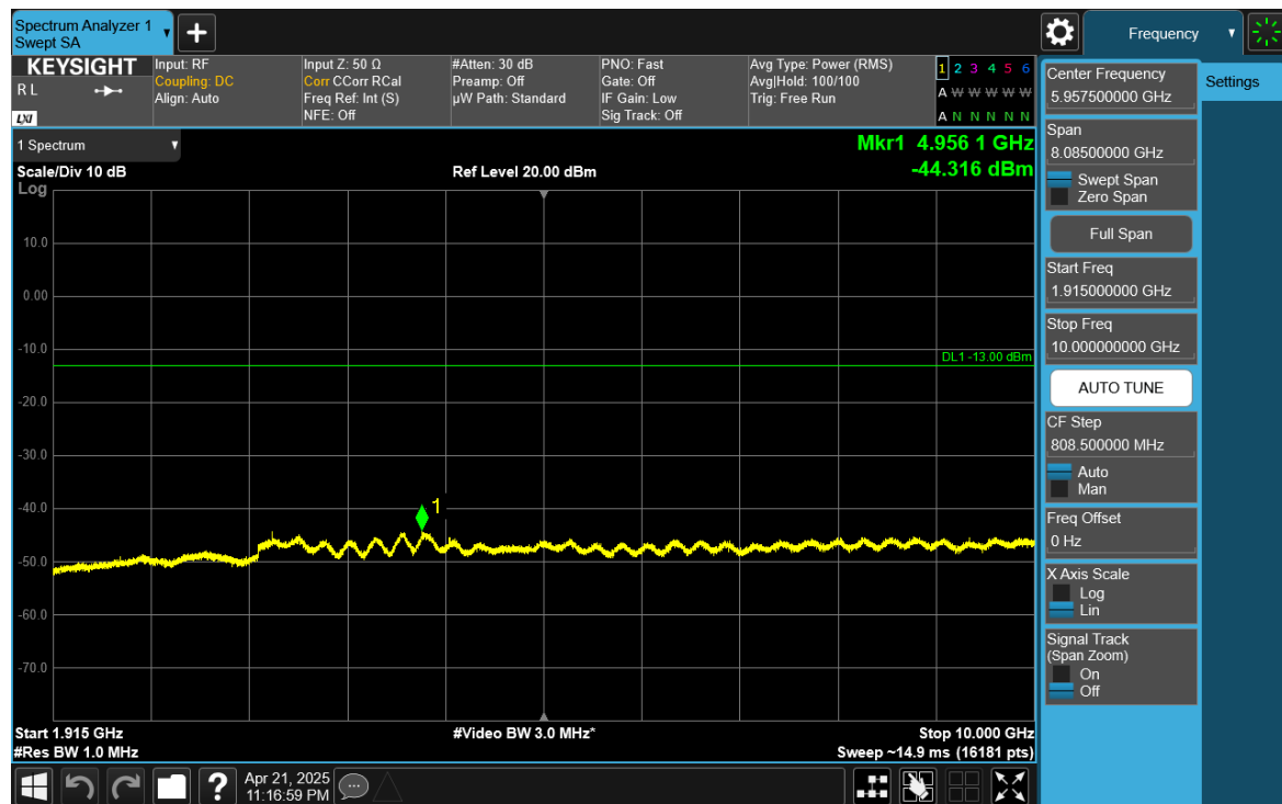
Plot 7-39. Conducted Spurious Plot (NR Band n25/n2 - 20MHz - RB Size 1, RB Offset 50 - Low Channel)
