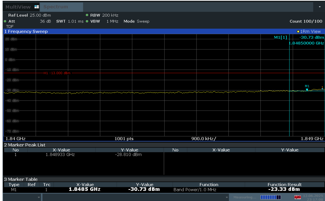
Plot 7-91. Extended Lower Band Edge Plot (LTE Band 2 – 20MHz QPSK – Full RB Configuration)
