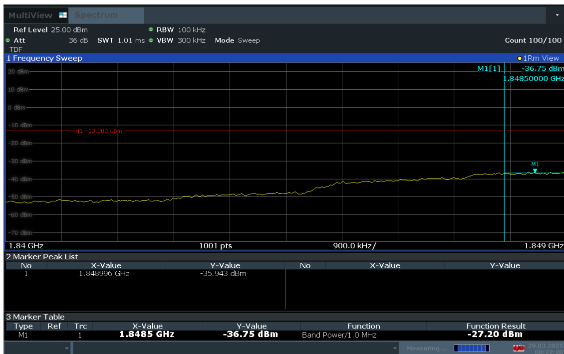
Plot 7-75. Extended Lower Band Edge Plot (LTE Band 2 – 3MHz QPSK – Full RB Configuration)
