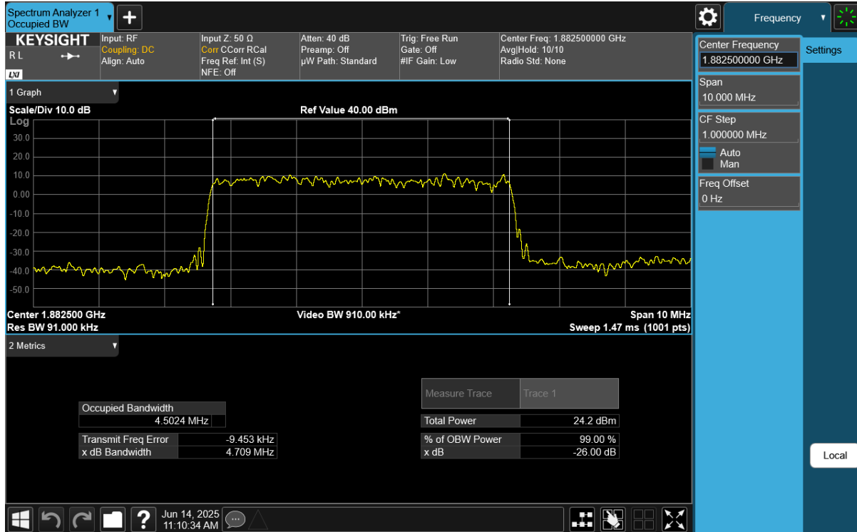
Plot 7-13. Occupied Bandwidth Plot (NR Band n25/n2 - 5MHz DFT-s-OFDM \pi/2 BPSK - Full RB)
