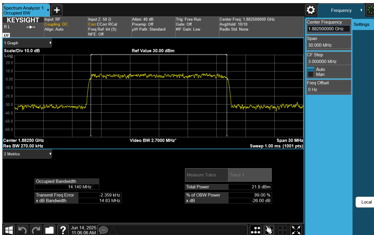
Plot 7-23. Occupied Bandwidth Plot (NR Band n25/n2 - 15MHz CP-OFDM 16QAM - Full RB)
