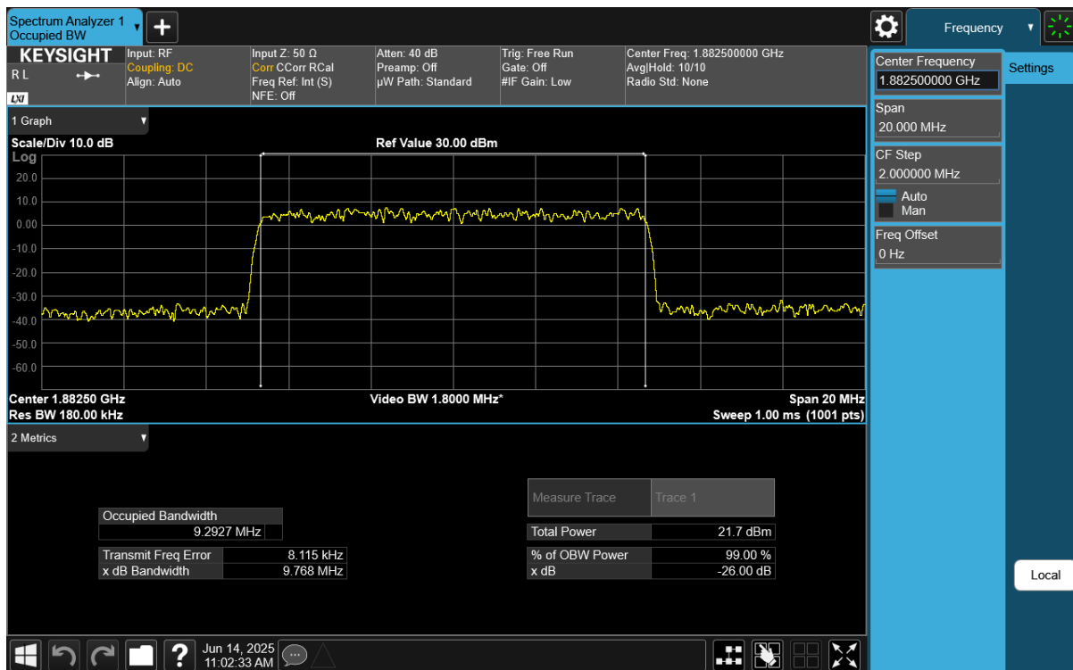
Plot 7-18. Occupied Bandwidth Plot (NR Band n25/n2 - 10MHz CP-OFDM QPSK - Full RB)
