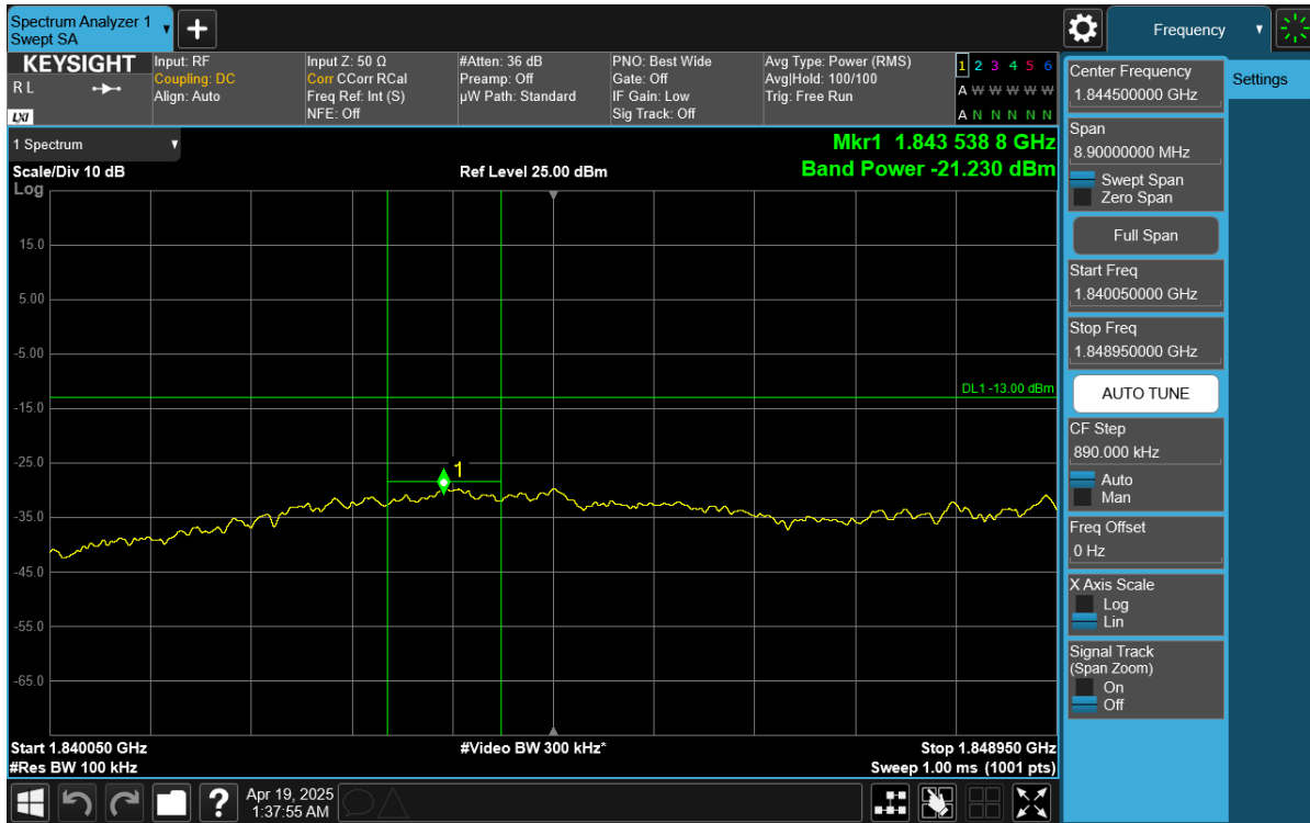
Plot 7-99. Extended Lower Band Edge Plot (NR Band n25 – 10MHz DFT-S-OFDM \pi/2 BPSK – Full RB Configuration)
