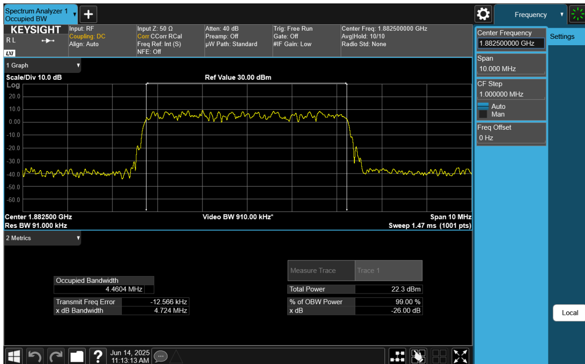
Plot 7-16. Occupied Bandwidth Plot (NR Band n25/n2 - 5MHz DFT-s-OFDM 64QAM - Full RB)
