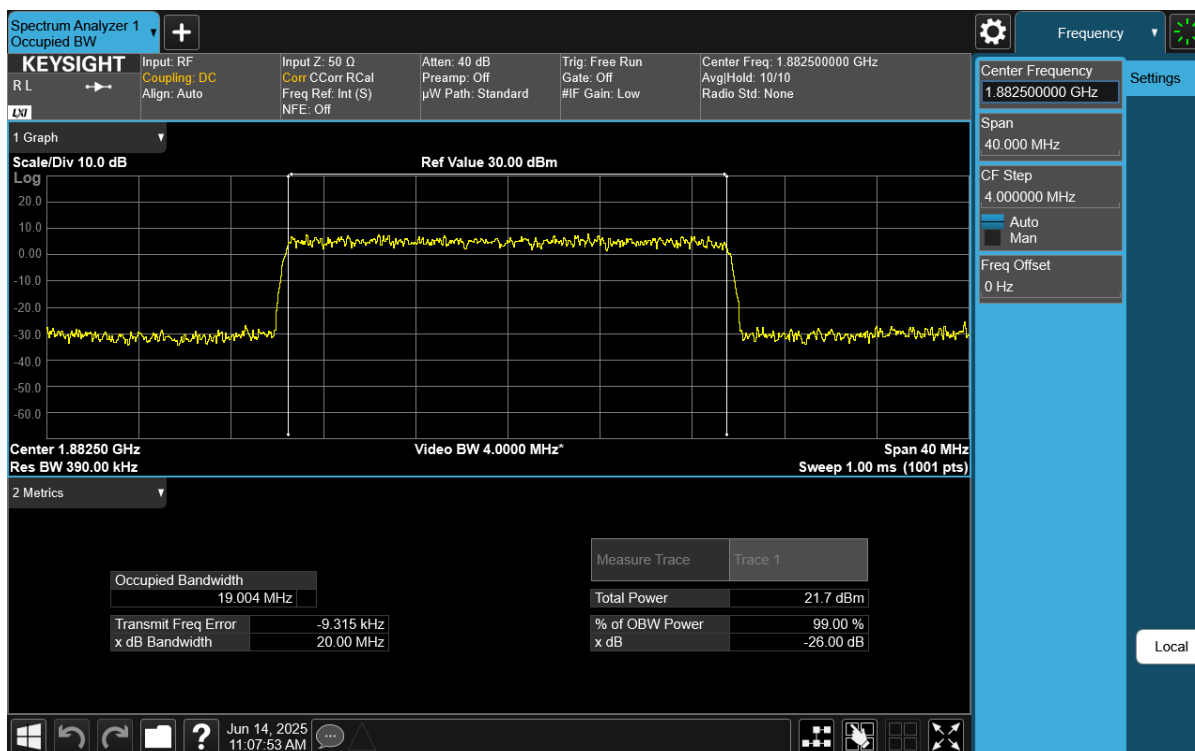
Plot 7-26. Occupied Bandwidth Plot (NR Band n25/n2 - 20MHz CP-OFDM QPSK - Full RB)
