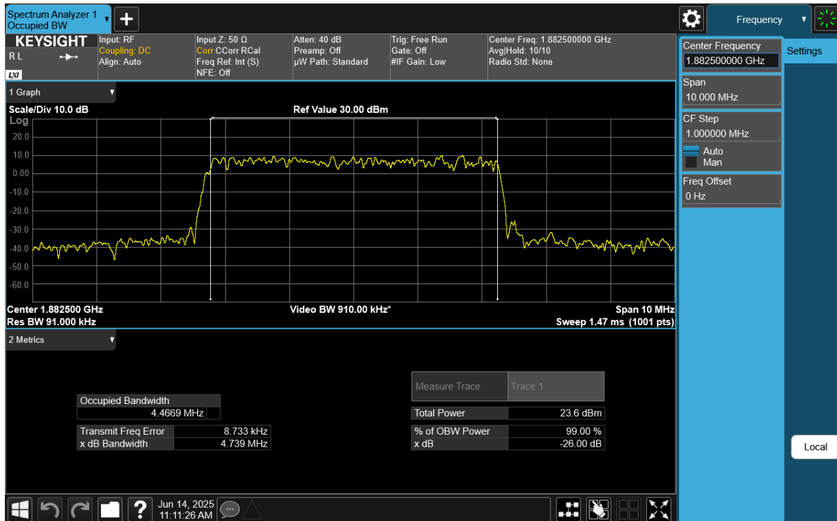
Plot 7-14. Occupied Bandwidth Plot (NR Band n25/n2 - 5MHz DFT-s-OFDM QPSK - Full RB)
