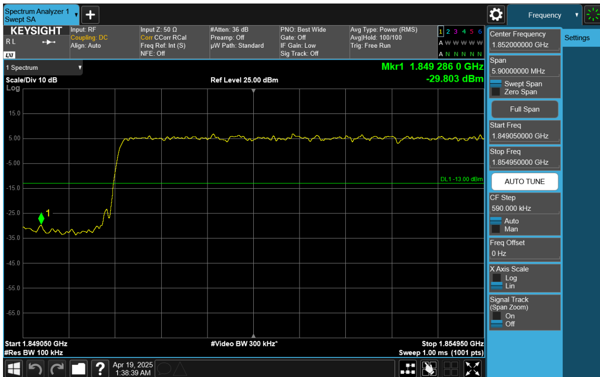
Plot 7-100. Lower Band Edge Plot (NR Band n25 – 10MHz DFT-S-OFDM \pi/2 BPSK – Full RB Configuration)
