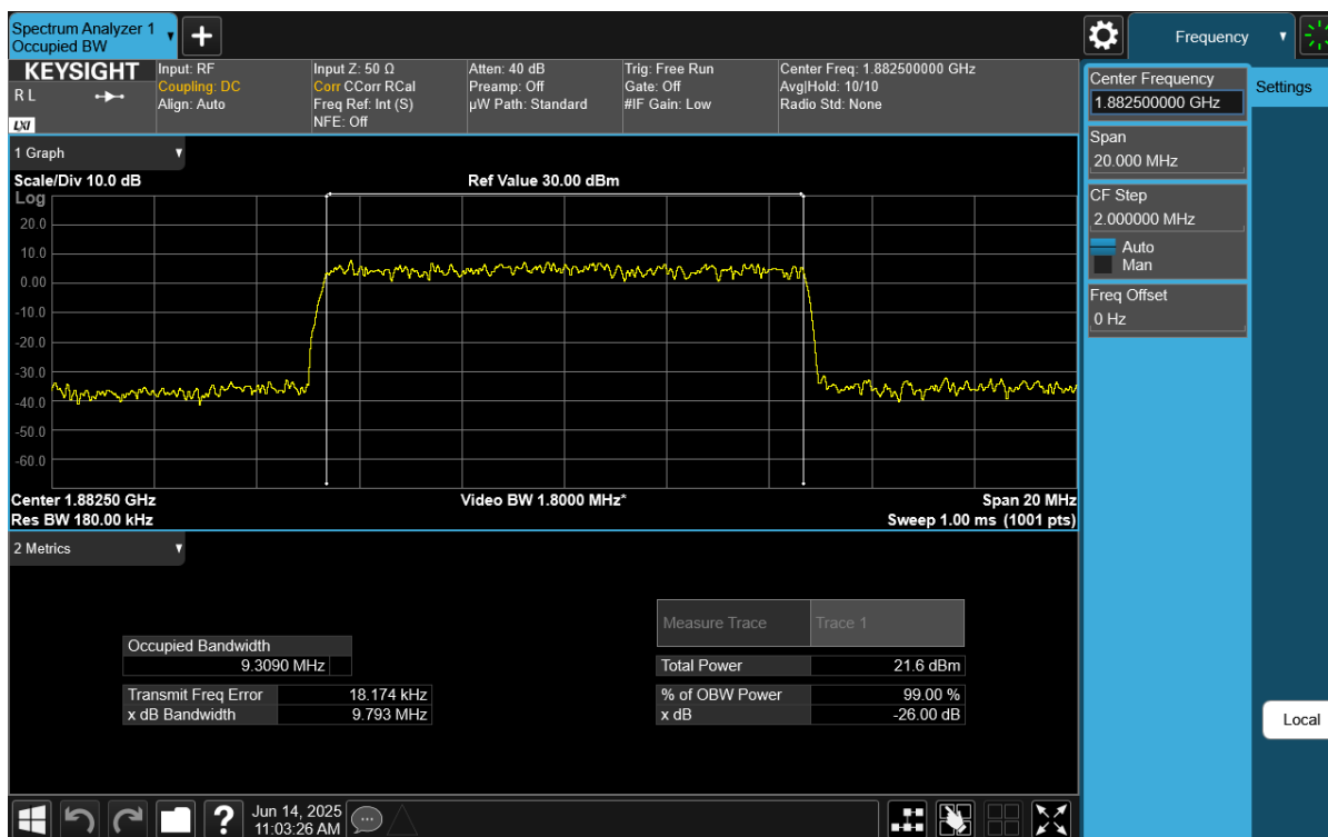
Plot 7-19. Occupied Bandwidth Plot (NR Band n25/n2 - 10MHz CP-OFDM 16QAM - Full RB)
