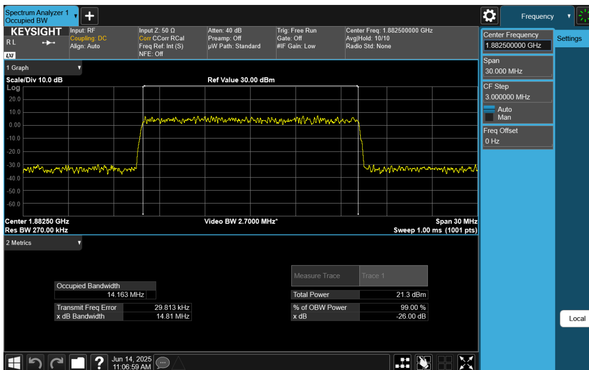
Plot 7-24. Occupied Bandwidth Plot (NR Band n25/n2 - 15MHz CP-OFDM 64QAM - Full RB)
