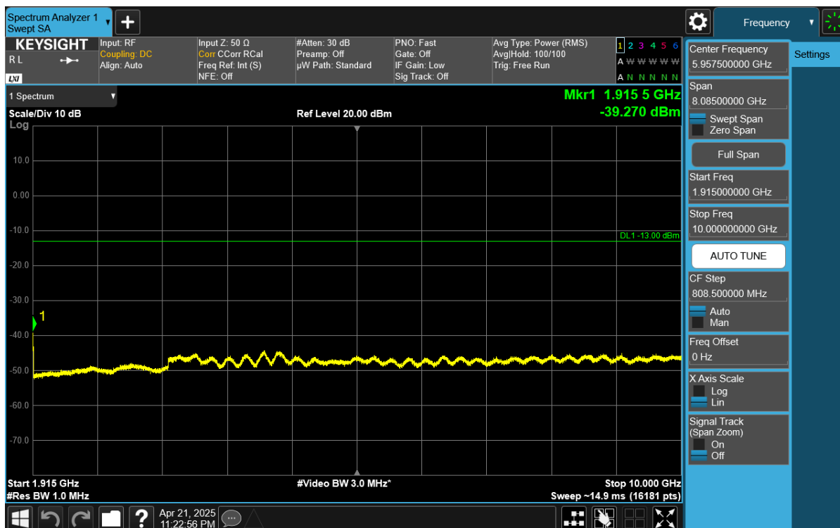
Plot 7-45. Conducted Spurious Plot (NR Band n25/n2 - 20MHz - RB Size 1, RB Offset 50 - High Channel)
