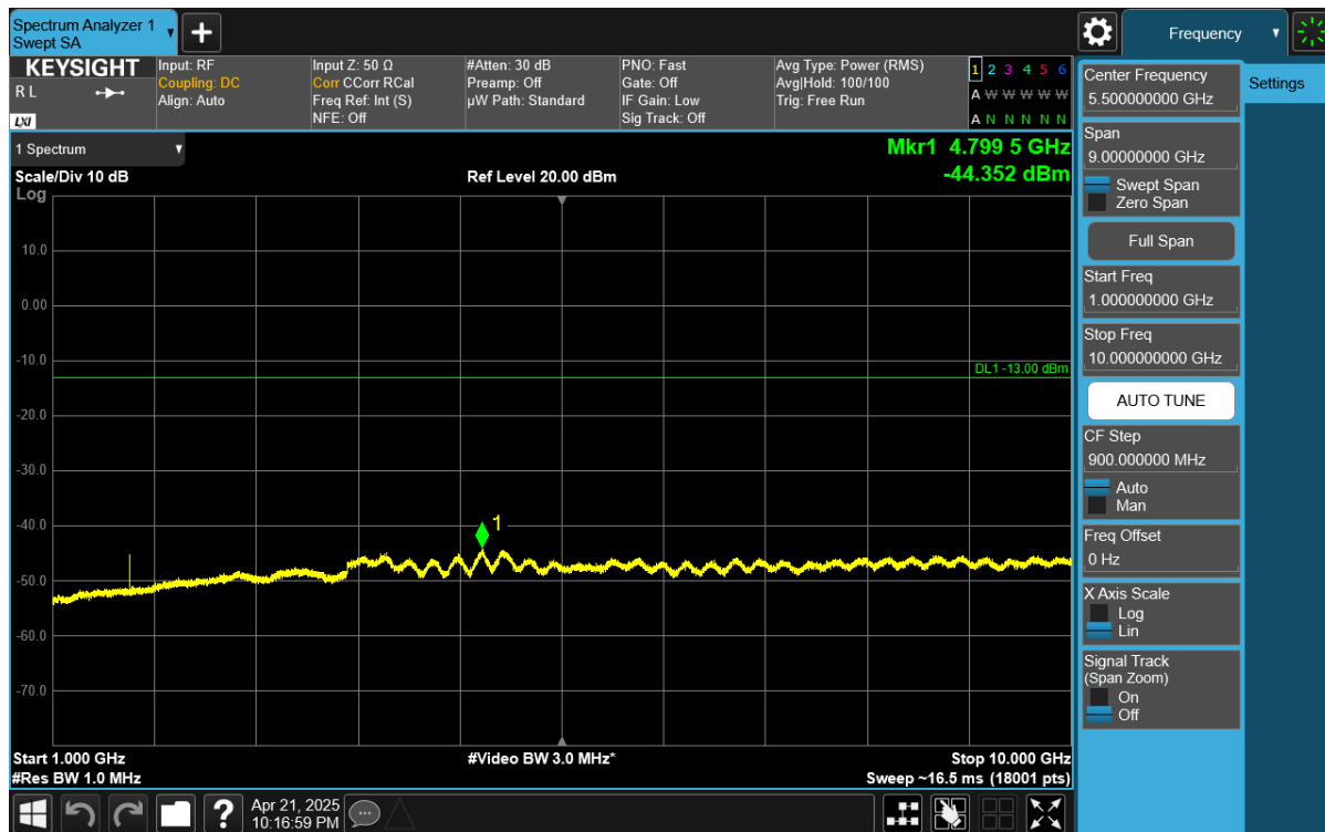
Plot 7-42. Conducted Spurious Plot (NR Band n26/n5 - 20MHz DFT-s-OFDM QPSK - RB Size 1, RB Offset 50 - High Channel)
