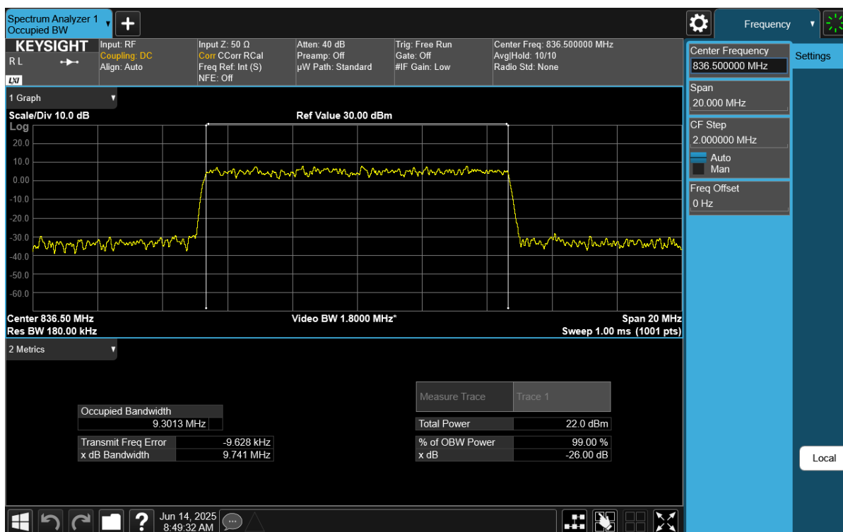
Plot 7-16. Occupied Bandwidth Plot (NR Band n26/n5 - 10MHz CP-OFDM 64-QAM - Full RB Configuration)
