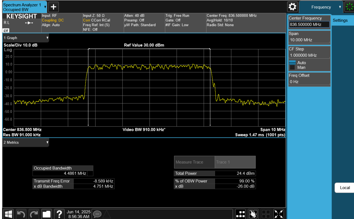
Plot 7-10. Occupied Bandwidth Plot (NR Band n26/n5 - 5MHz DFT-s-OFDM QPSK - Full RB Configuration)
