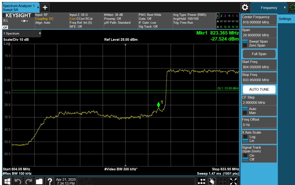
Plot 7-73. Lower BE Plot (NR Band n5 DFT-s-OFDM \pi/2 BPSK – 20MHz - Full RB)
