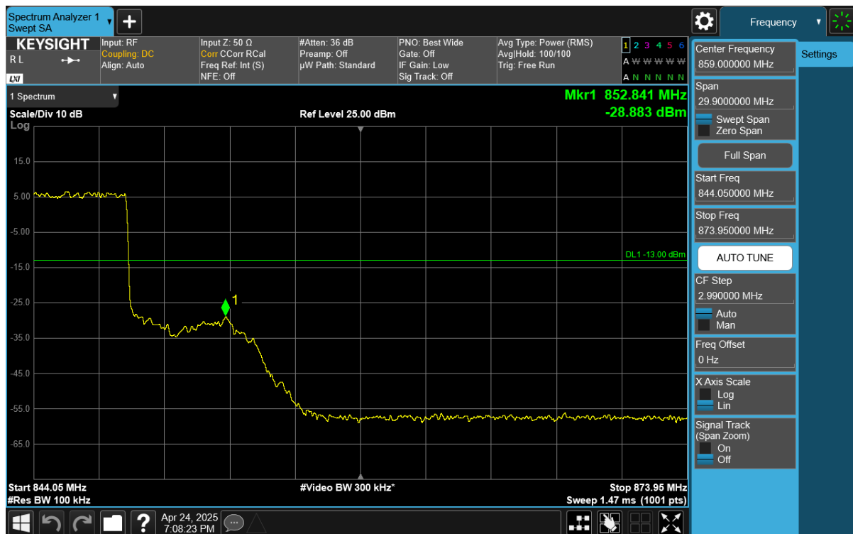
Plot 7-62. Upper BE Plot (NR Band n26 DFT-s-OFDM \pi/2 BPSK – 10MHz - Full RB)
