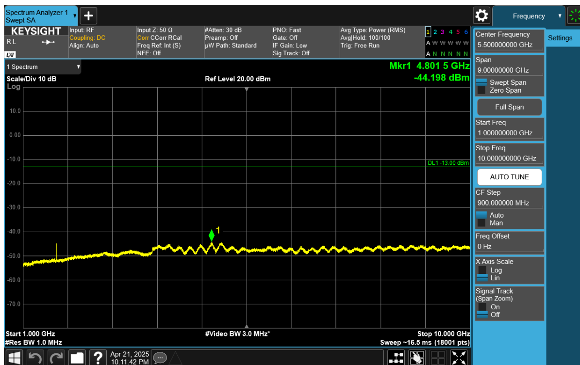
Plot 7-36. Conducted Spurious Plot (NR Band n26/n5 - 20MHz DFT-s-OFDM QPSK - RB Size 1, RB Offset 50 - Low Channel)
