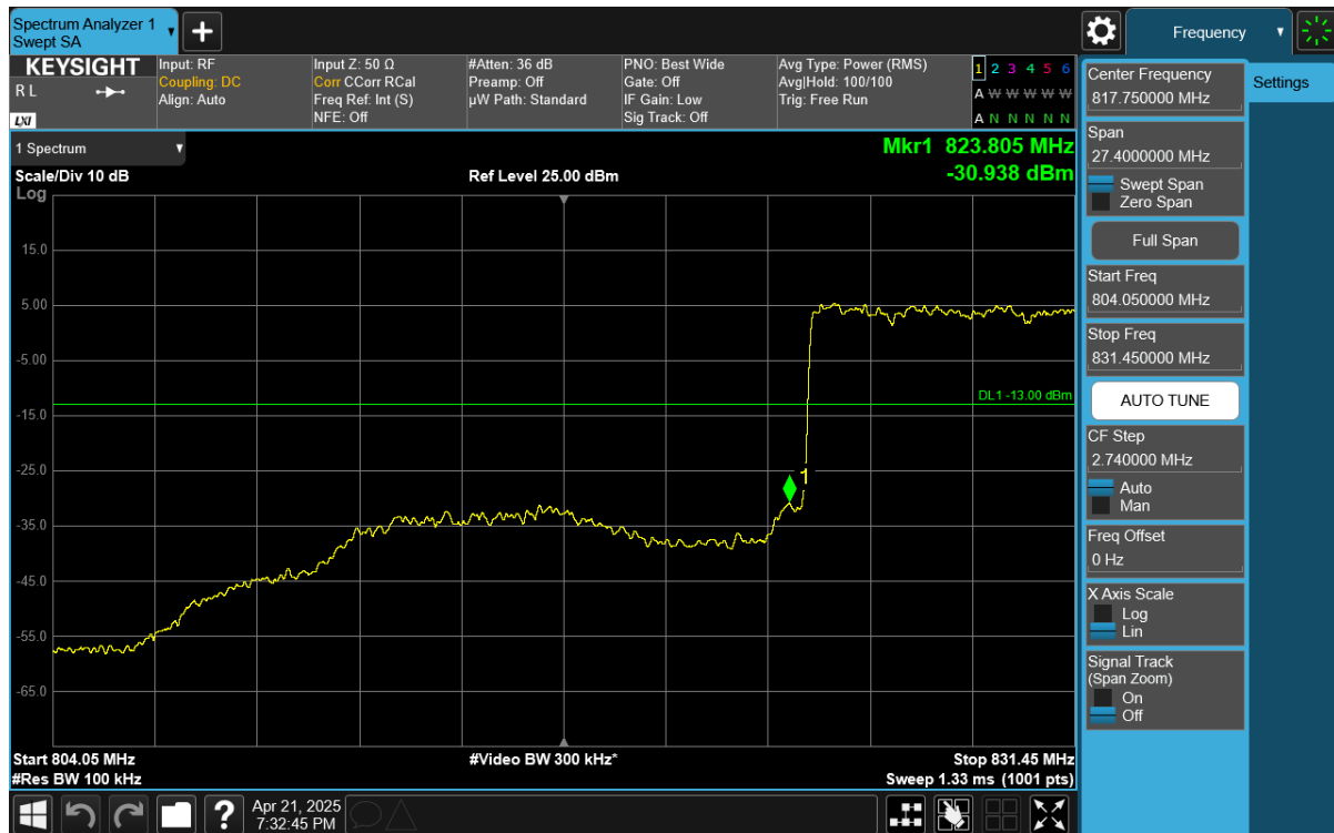
Plot 7-71. Lower BE Plot (NR Band n5 DFT-s-OFDM \pi/2 BPSK – 15MHz - Full RB)
