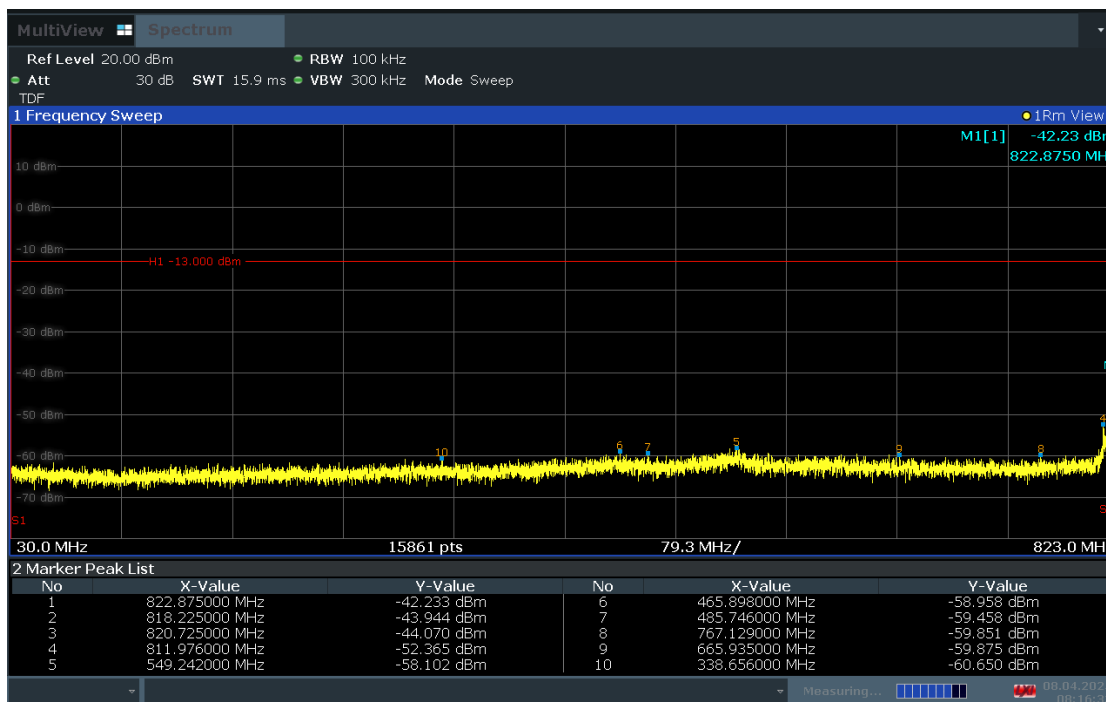
Plot 7-25. Conducted Spurious Plot (LTE Band 26/5 - 10MHz QPSK - RB Size 1, RB Offset 25 - Low Channel)
