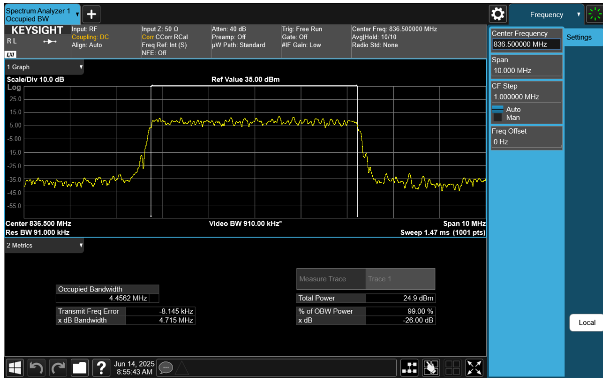
Plot 7-9. Occupied Bandwidth Plot (NR Band n26/n5 - 5MHz n5 DFT-s-OFDM \pi/2 BPSK - Full RB Configuration)
