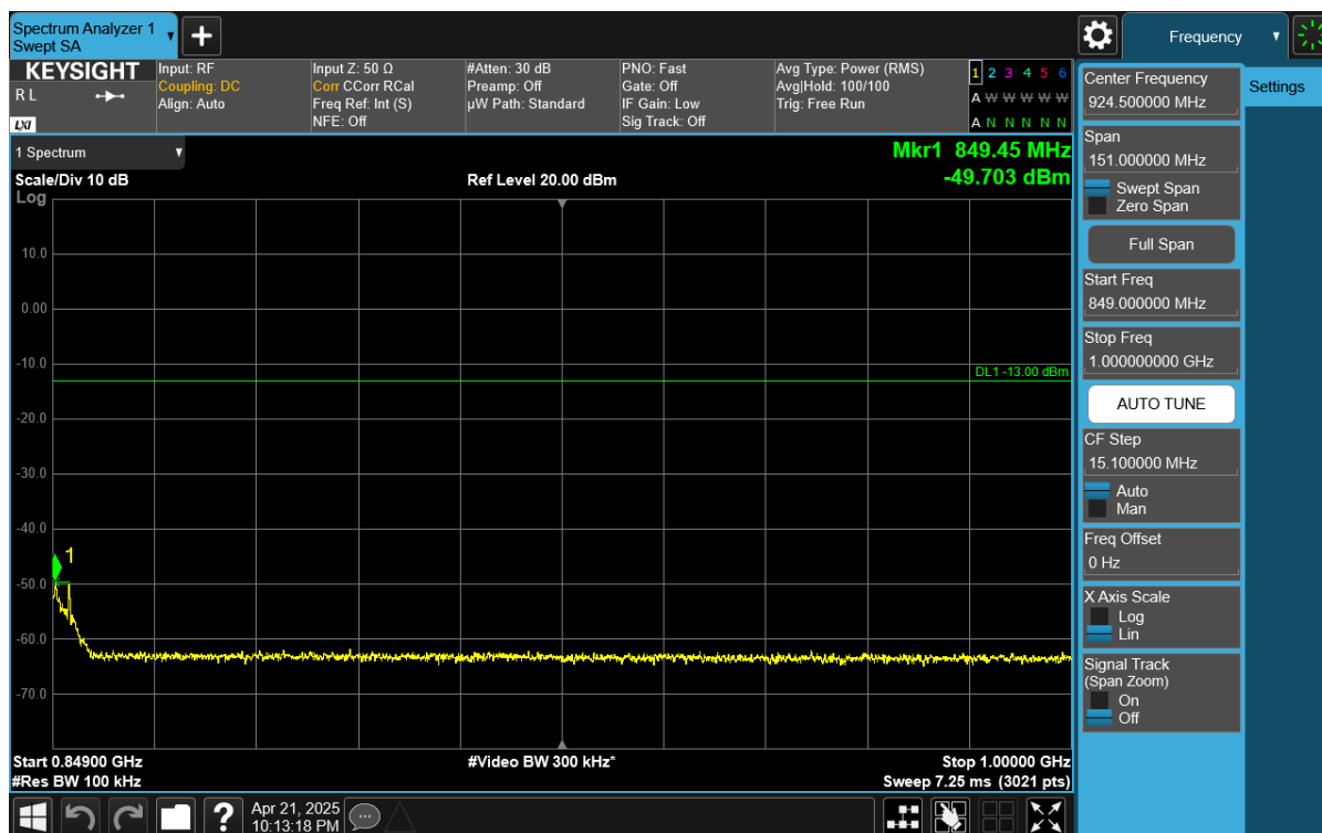
Plot 7-38. Conducted Spurious Plot (NR Band n26/n5 - 20MHz DFT-s-OFDM QPSK - RB Size 1, RB Offset 50 - Mid Channel)
