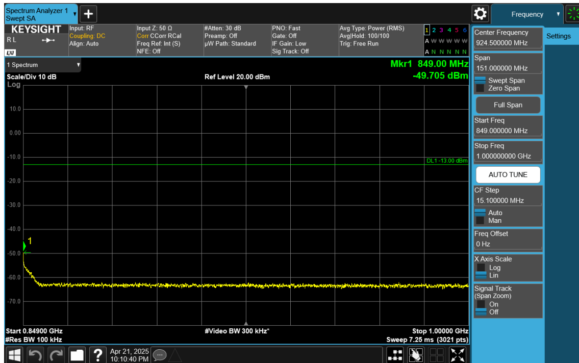
Plot 7-35. Conducted Spurious Plot (NR Band n26/n5 - 20MHz DFT-s-OFDM QPSK - RB Size 1, RB Offset 50 - Low Channel)
