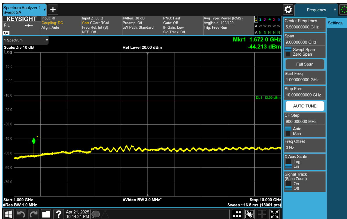
Plot 7-39. Conducted Spurious Plot (NR Band n26/n5 - 20MHz DFT-s-OFDM QPSK - RB Size 1, RB Offset 50 - Mid Channel)
