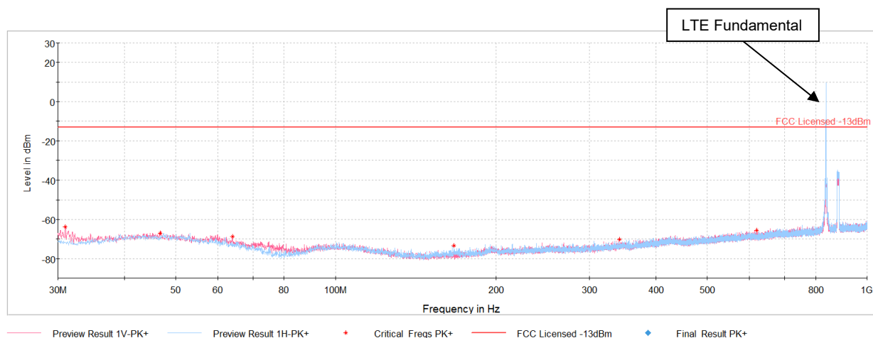
Plot 7-75. Antenna BCM Radiated Spurious Plot below 1GHz (LTE Band 26/5)
