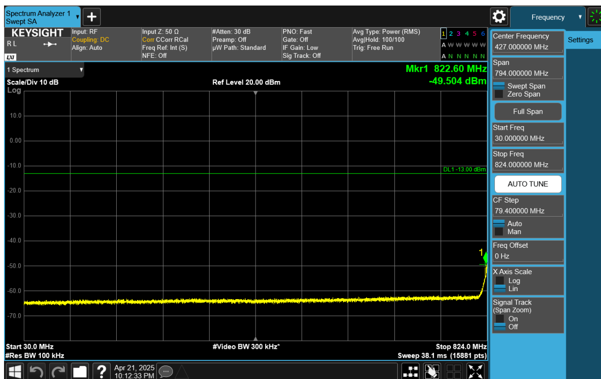
Plot 7-37. Conducted Spurious Plot (NR Band n26/n5 - 20MHz DFT-s-OFDM QPSK - RB Size 1, RB Offset 50 - Mid Channel)
