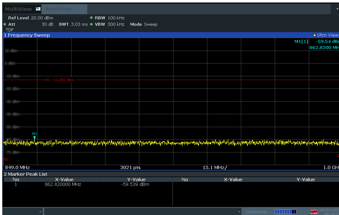
Plot 7-26. Conducted Spurious Plot (LTE Band 26/5 - 10MHz QPSK - RB Size 1, RB Offset 25 - Low Channel)
