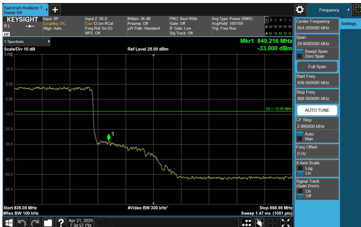
Plot 7-74. Upper BE Plot (NR Band n5 DFT-s-OFDM \pi/2 BPSK – 20MHz - Full RB)
