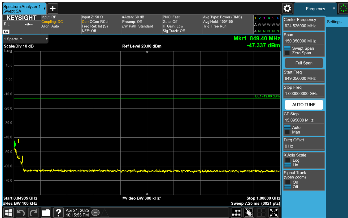
Plot 7-41. Conducted Spurious Plot (NR Band n26/n5 - 20MHz DFT-s-OFDM QPSK - RB Size 1, RB Offset 50 - High Channel)
