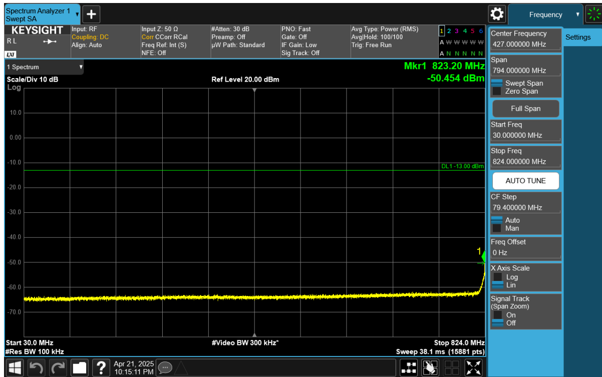
Plot 7-40. Conducted Spurious Plot (NR Band n26/n5 - 20MHz DFT-s-OFDM QPSK - RB Size 1, RB Offset 50 - High Channel)
