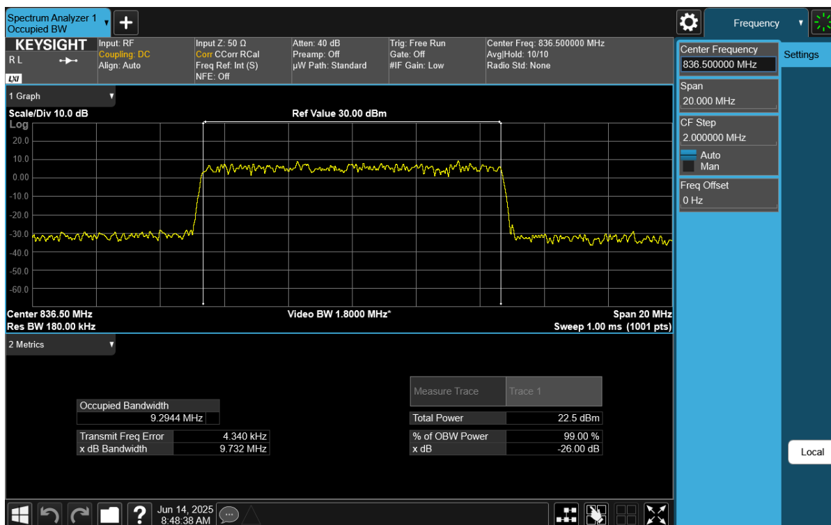
Plot 7-15. Occupied Bandwidth Plot (NR Band n26/n5 - 10MHz CP-OFDM 16-QAM - Full RB Configuration)
