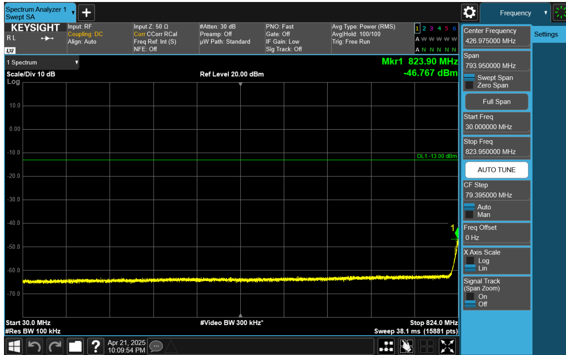
Plot 7-34. Conducted Spurious Plot (NR Band n26/n5 - 20MHz DFT-s-OFDM QPSK - RB Size 1, RB Offset 50 - Low Channel)
