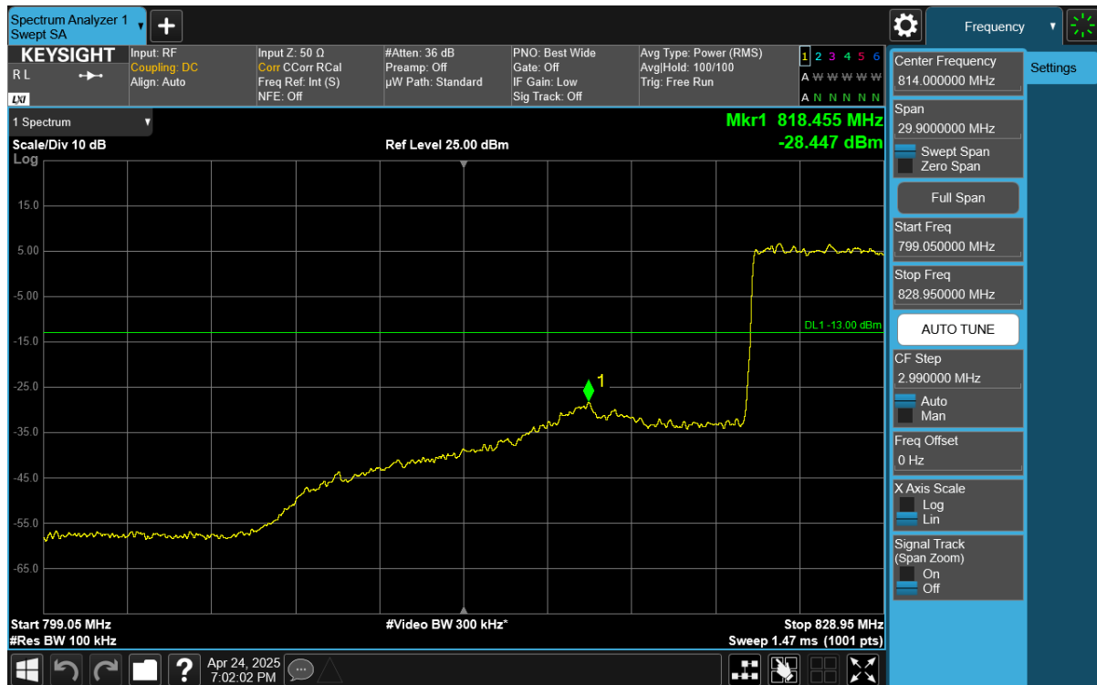
Plot 7-61. Lower BE Plot (NR Band n26 DFT-s-OFDM QPSK – 10MHz - Full RB)
