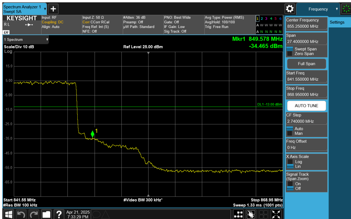
Plot 7-72. Upper BE Plot (NR Band n5 DFT-s-OFDM \pi/2 BPSK – 15MHz - Full RB)
