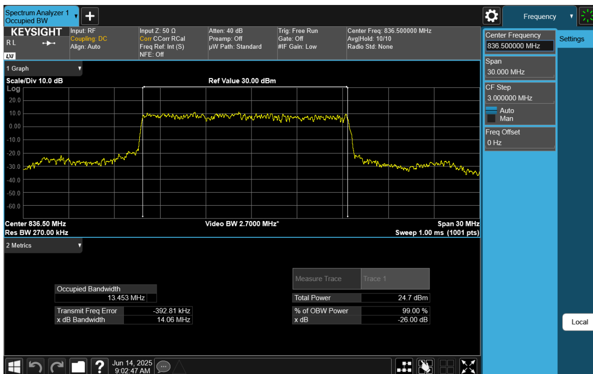
Plot 7-17. Occupied Bandwidth Plot (NR Band n26/n5 - 15MHz DFT-s-OFDM \pi/2 BPSK - Full RB Configuration)
