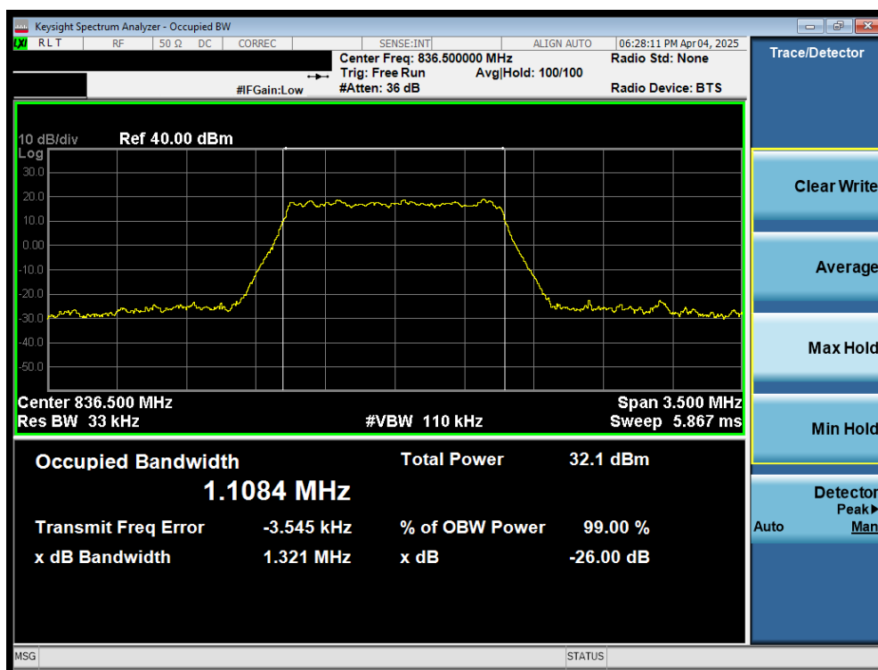
Plot 7-2. Occupied Bandwidth Plot (LTE Band 26/5 - 1.4MHz 16-QAM - Full RB Configuration)
