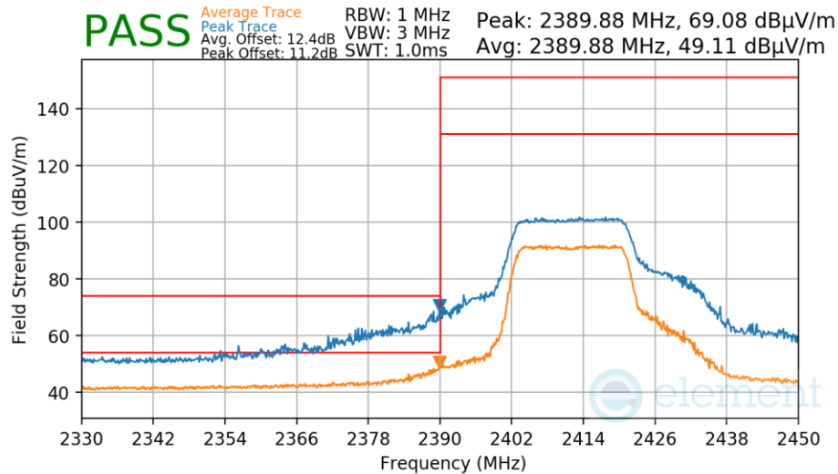
Plot 7-68. Radiated Restricted Lower Band Edge Measurement
