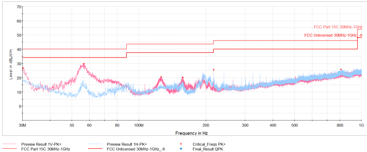
Plot 7-74. Radiated Spurious Emissions below 1GHz 11b Ch.6, with AC/DC adaptor via USB-C cable with magnetic charger
