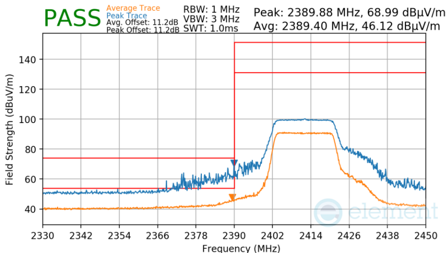
Plot 7-61. Radiated Restricted Lower Band Edge Measurement
