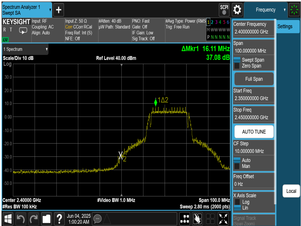
Plot 7-30. Band Edge Plot (802.11g– Ch. 3) – 6Mbps
