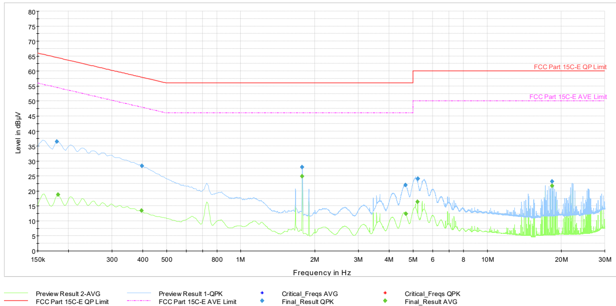
Plot 7-39. AC Line Conducted Plot with Bluetooth HDR (N, 4Mbps ePA - Ch.38 with AC/DC adaptor via USB-C cable with magnetic charger)
