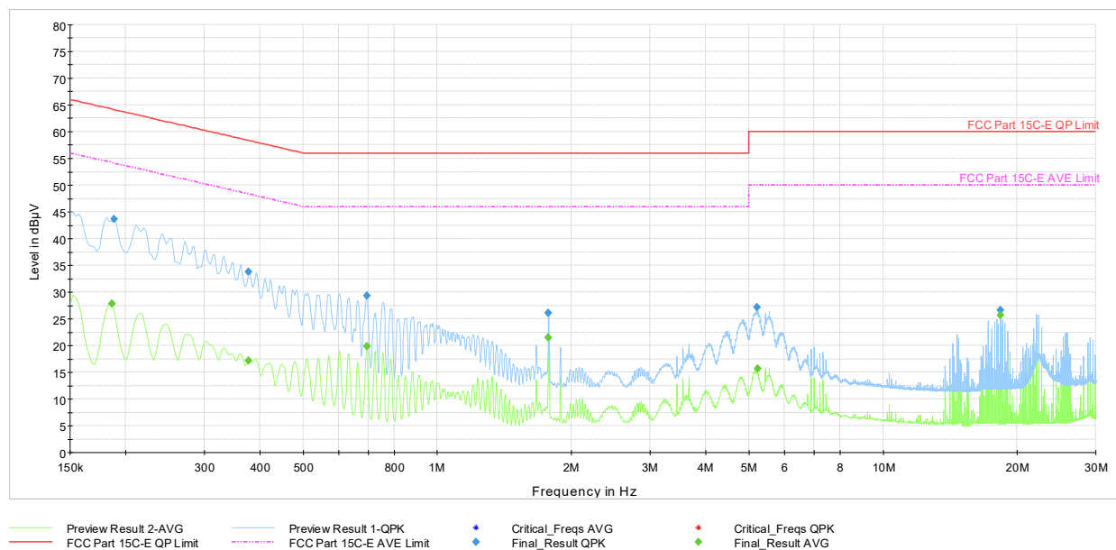
Plot 7-38. AC Line Conducted Plot with Bluetooth HDR (L1, 4Mbps ePA - Ch.38 with AC/DC adaptor via USB-C cable with magnetic charger)
