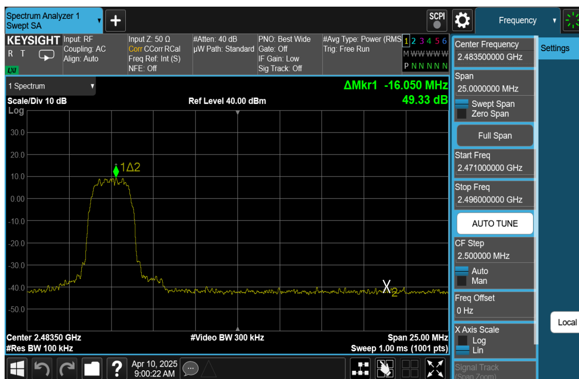
Plot 7-20. Band Edge Plot (Bluetooth (HDR4), ePA – Ch. 73)
