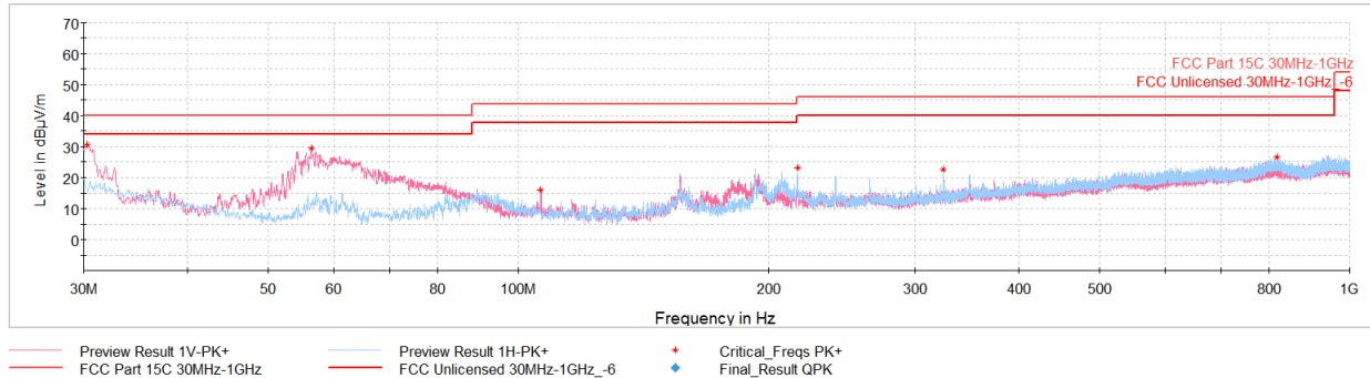
Plot 7-37. Radiated Spurious Emissions Below 1GHz (4Mbps, ePA – Ch.38 with AC/DC adaptor via USB-C cable with magnetic charger)
