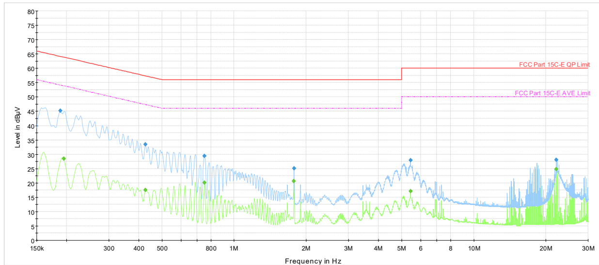
Plot 7-38. AC Line Conducted Plot with Bluetooth LE (L1, 1Mbps ePA – Ch.19 with AC/DC adaptor via USB-C cable with magnetic charger)
