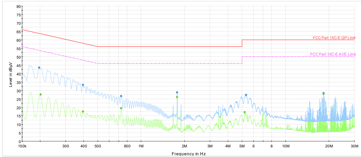
Plot 7-39. AC Line Conducted Plot with Bluetooth LE (N, 1Mbps ePA – Ch.19, with AC/DC adaptor via USB-C cable with magnetic charger)
