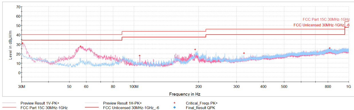
Plot 7-37. Radiated Spurious Emissions Below 1GHz (1Mbps, ePA – Ch.19, Pol. H & V, with AC/DC adaptor via USB-C cable with magnetic charger)
