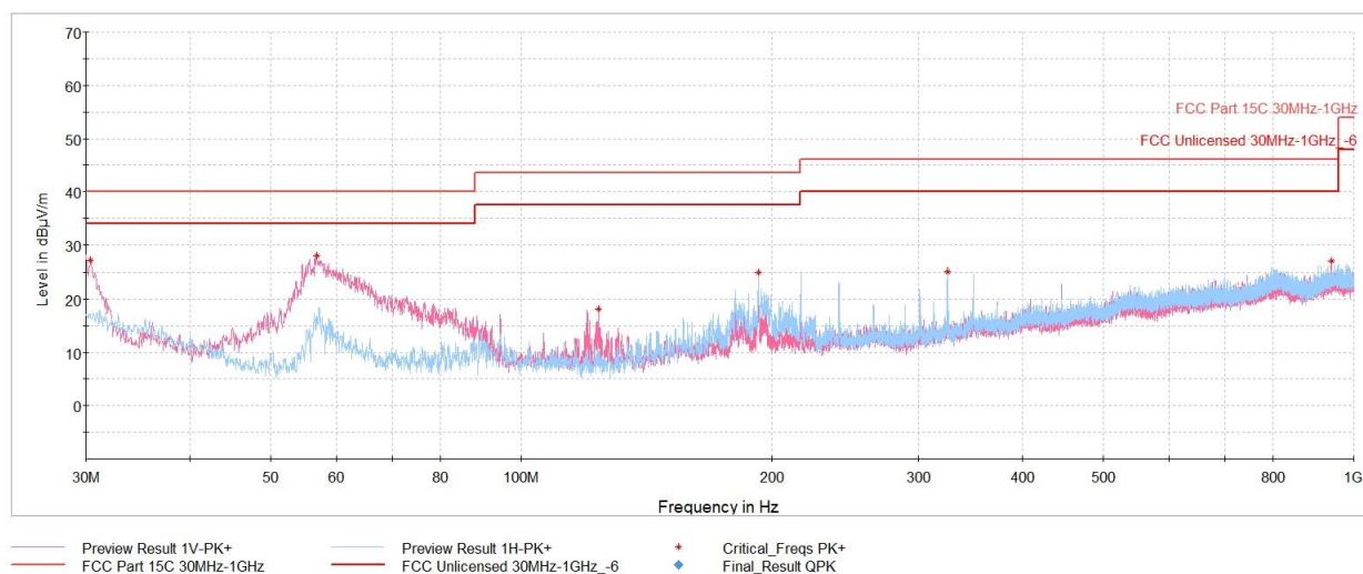
Plot 7-74. Radiated Spurious Emissions below 1GHz 11b Ch.6, with AC/DC Adapter via USB-C cable with magnetic charger
