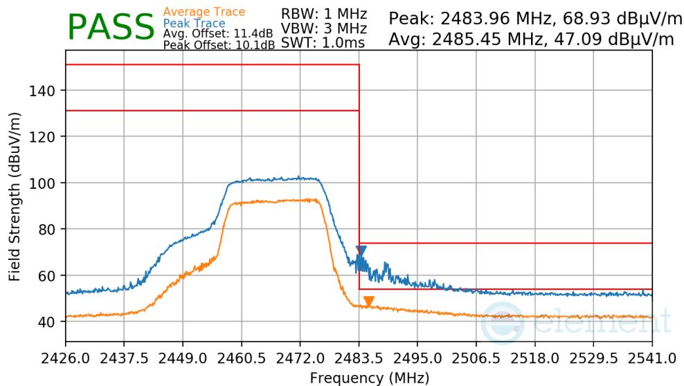
Plot 7-72. Radiated Restricted Upper Band Edge Measurement
