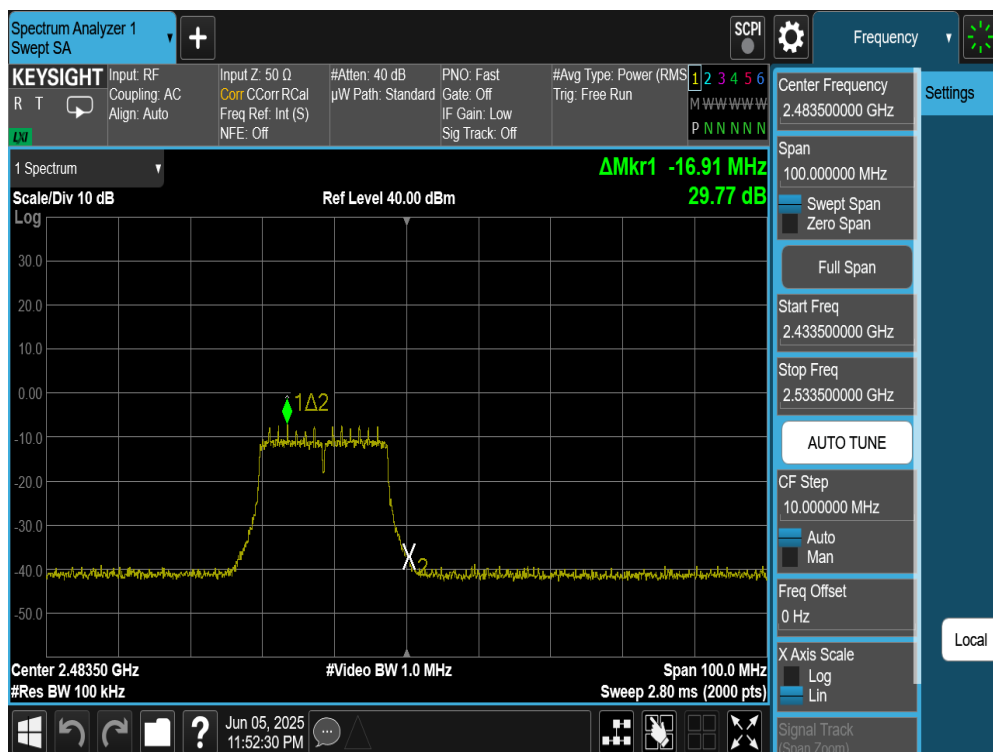
Plot 7-41. Band Edge Plot (802.11n (2.4GHz) – Ch. 13) – MCS0
