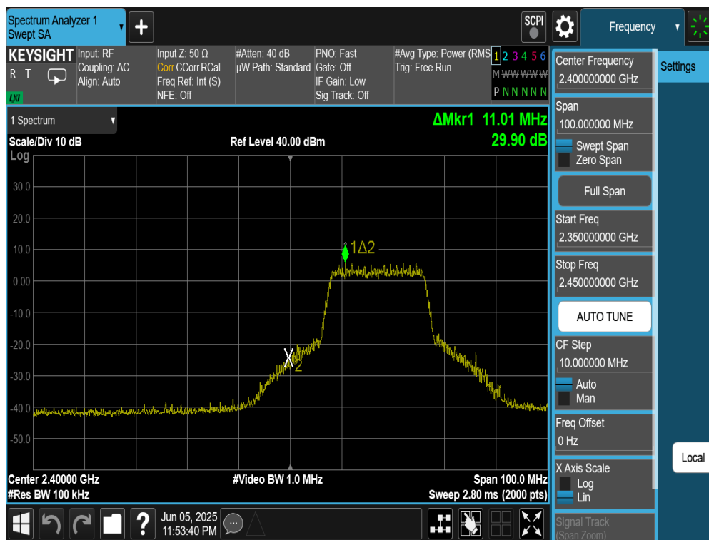
Plot 7-43. Band Edge Plot (802.11n (2.4GHz) – Ch. 2) – MCS7
