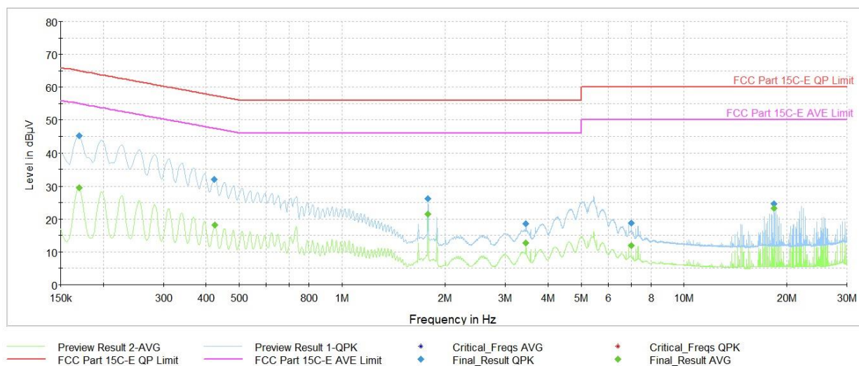
Plot 7-75. AC Line Conducted Plot 802.11b - Ch.6 (L1, with AC/DC adaptor via USB-C cable with magnetic charger)
