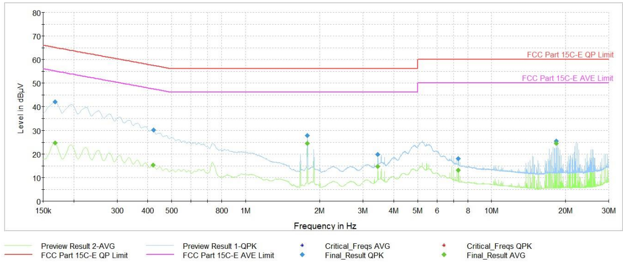
Plot 7-76. AC Line Conducted Plot 802.11b - Ch.6 (N, with AC/DC adaptor via USB-C cable with magnetic charger)
