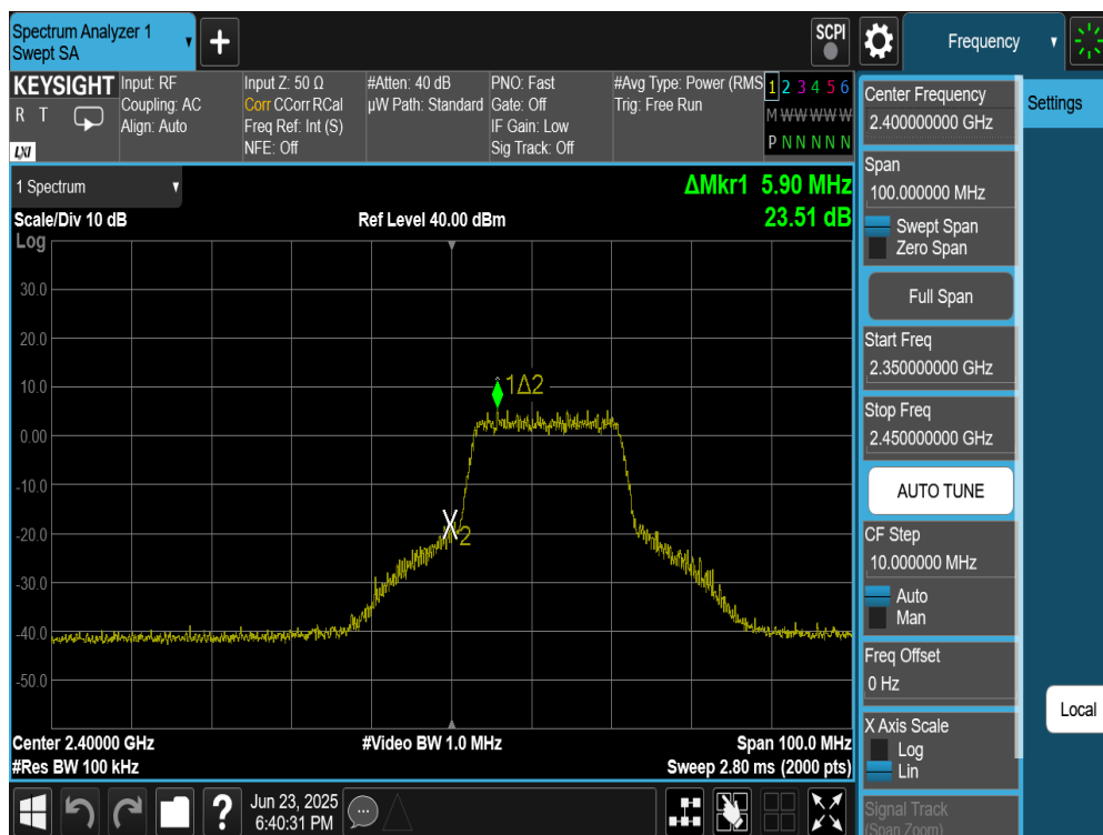
Plot 7-42. Band Edge Plot (802.11n (2.4GHz) – Ch. 1) – MCS7
