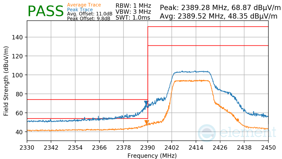
Plot 7-68. Radiated Restricted Lower Band Edge Measurement
