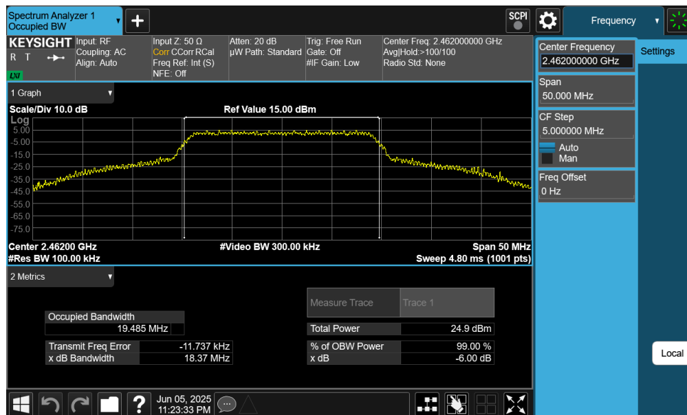
Plot 7-12. 6dB Bandwidth & 99% OBW Plot (802.11n (2.4GHz) – Ch. 11) – MCS7
