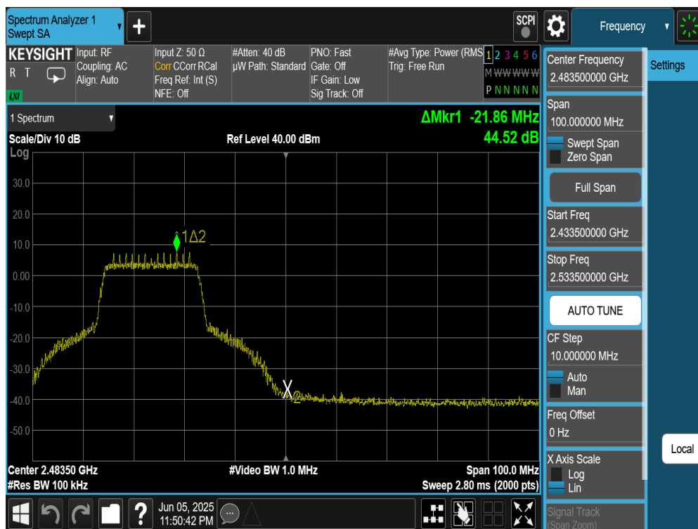
Plot 7-38. Band Edge Plot (802.11n (2.4GHz) – Ch. 10) – MCS0
