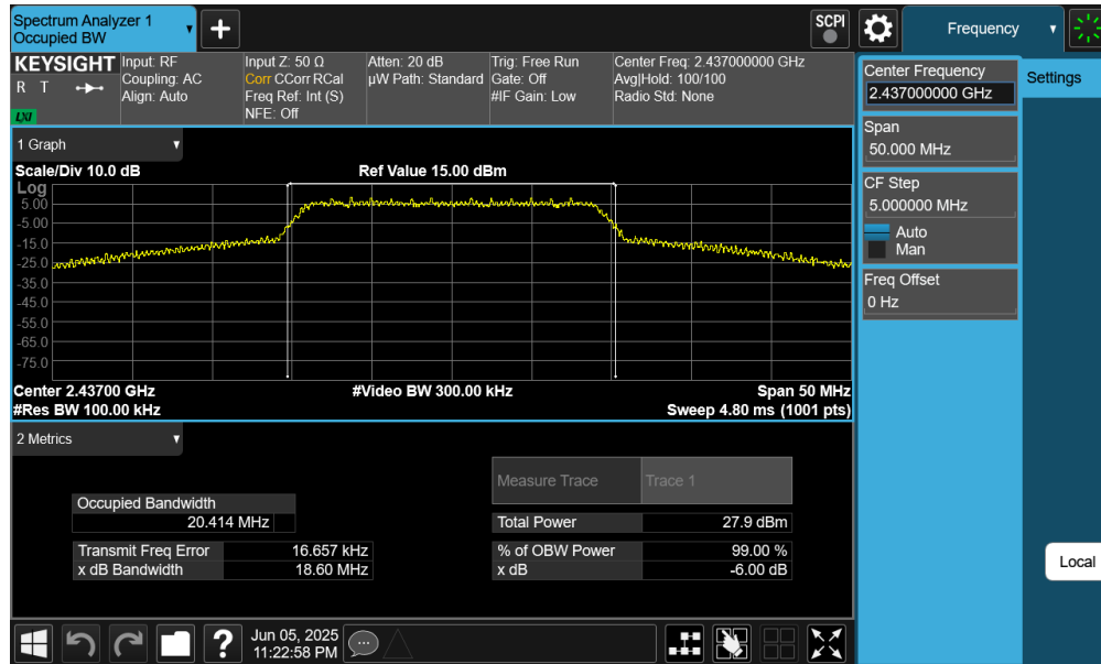
Plot 7-11. 6dB Bandwidth & 99% OBW Plot (802.11n (2.4GHz) – Ch. 6) – MCS7
