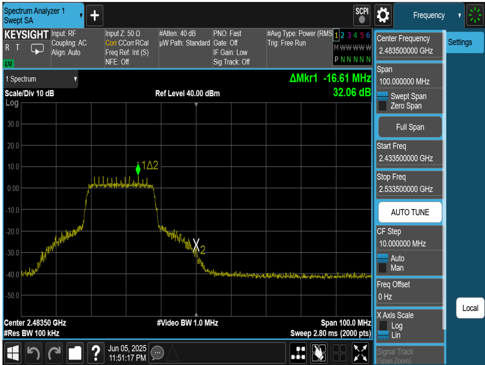
Plot 7-39. Band Edge Plot (802.11n (2.4GHz) – Ch. 11) – MCS0
