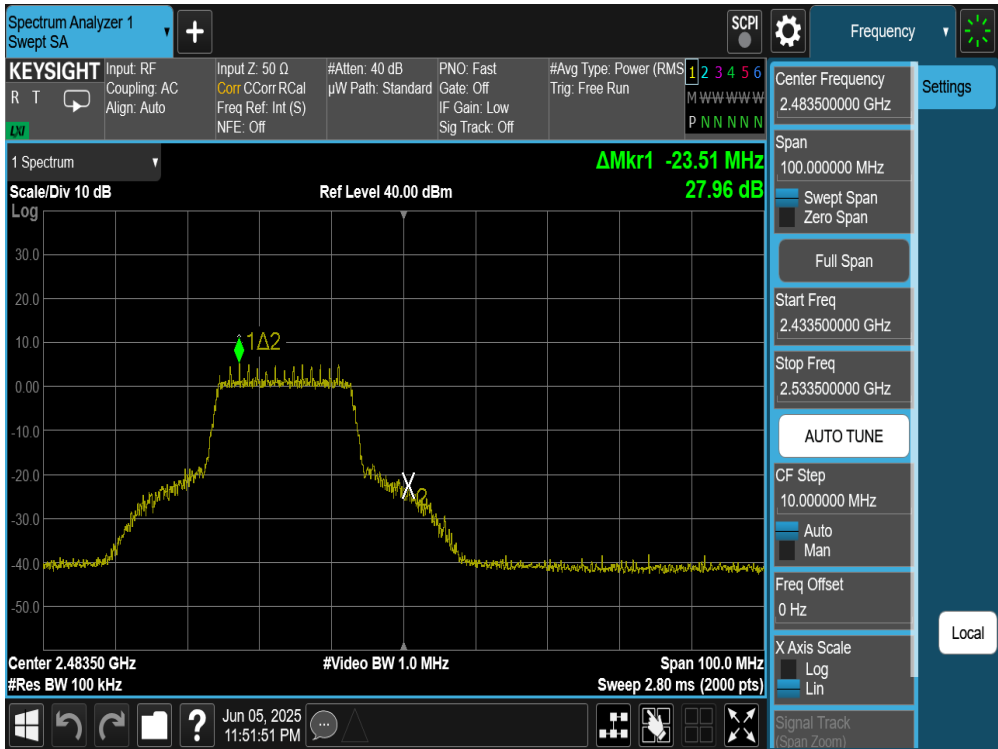
Plot 7-40. Band Edge Plot (802.11n (2.4GHz) – Ch. 12) – MCS0
