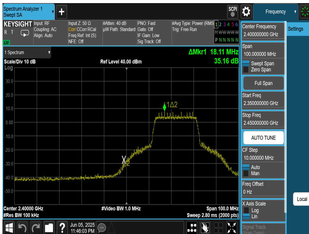
Plot 7-37. Band Edge Plot (802.11n (2.4GHz) – Ch. 3) – MCS0
