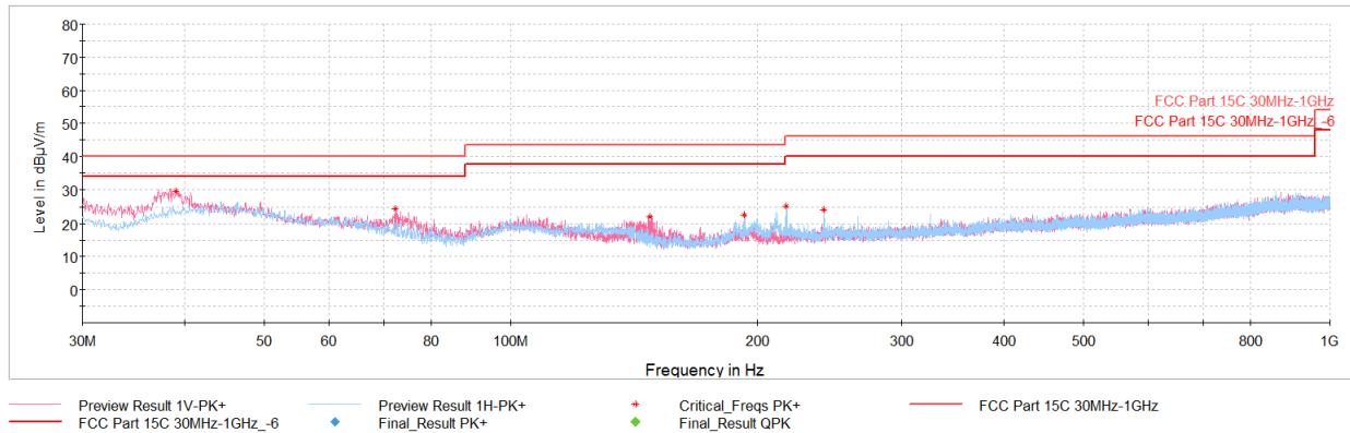
Plot 7-37. Radiated Spurious Emissions Below 1GHz (4Mbps, ePA – Ch.38 with AC/DC adaptor via USC-C cable with magnetic charger)
