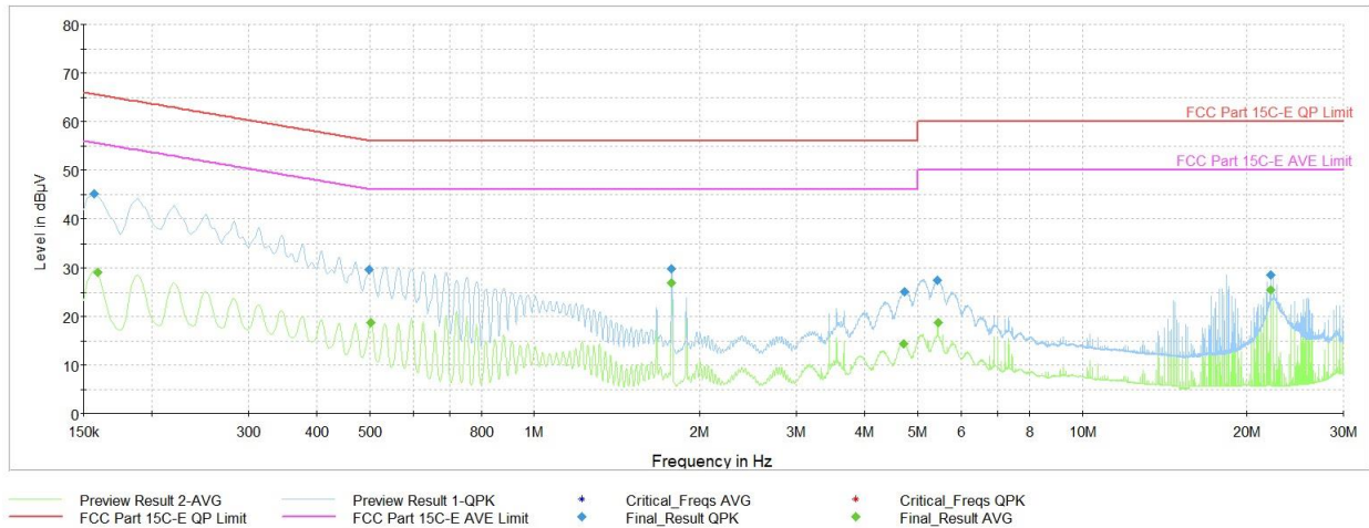
Plot 7-39. AC Line Conducted Plot with Bluetooth HDR (N, 4Mbps ePA - Ch.38 with AC/DC adaptor via USB-C cable with magnetic charger)
