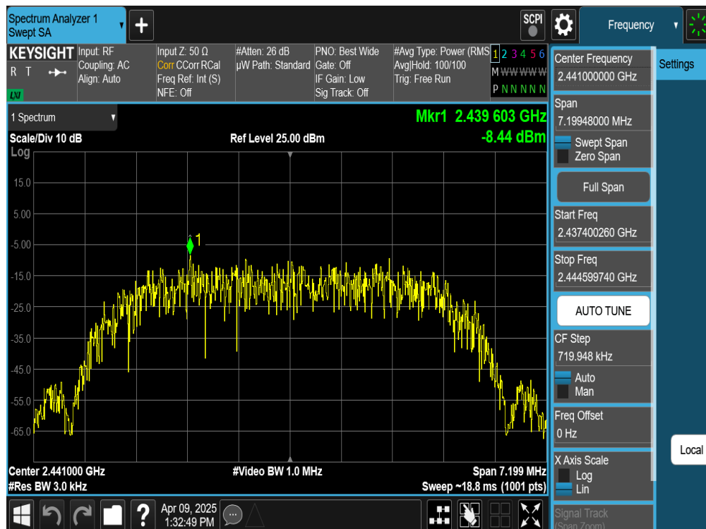
Plot 17-17. Power Spectral Density Plot (Bluetooth (HDR8), 8Mbps, iPA – Ch. 38)
