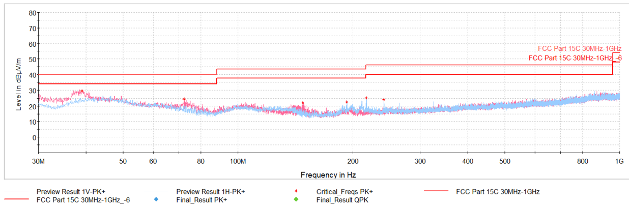
Plot 7-37. Radiated Spurious Emissions Below 1GHz (1Mbps, ePA – Ch.19, Pol. H & V, with AC/DC adaptor via USB-C cable with magnetic charger)
