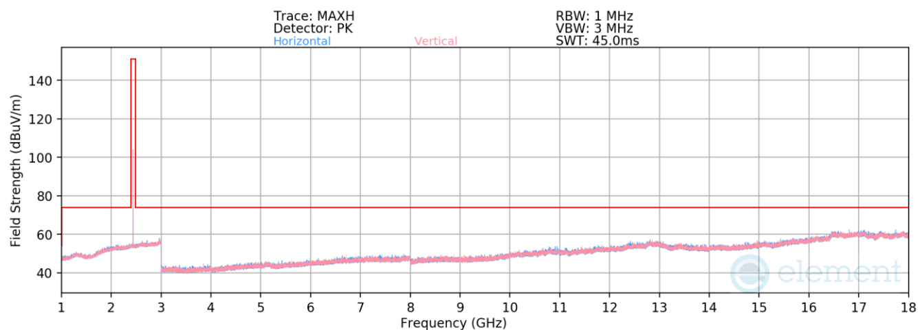
Plot 7-31. Radiated Spurious Emissions 1-18GHz (1Mbps, ePA – Ch. 19)
