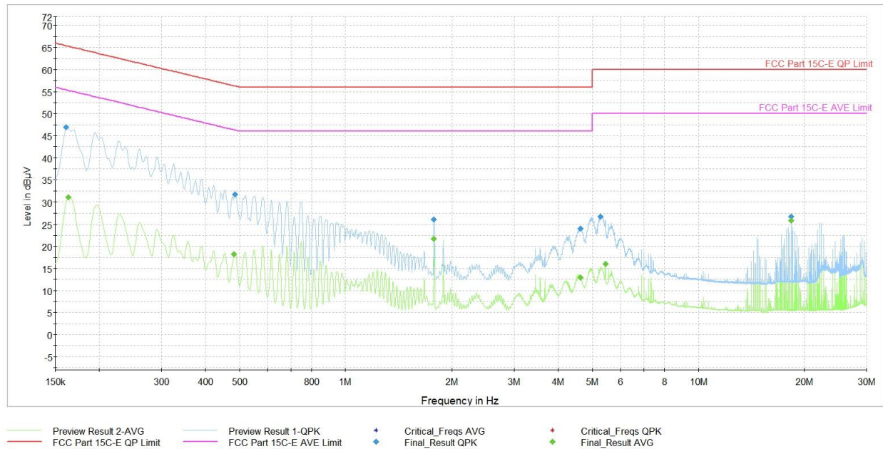
Plot 7-38. AC Line Conducted Plot with Bluetooth LE (L1, 1Mbps ePA – Ch.19 with AC/DC adaptor via USB-C cable with magnetic charger)
