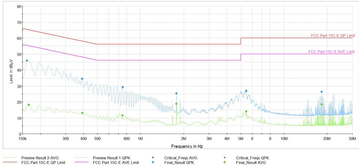
Plot 7-38. AC Line-Conducted Test Plot (L1, GFSK ePA – Ch.39, with AC/DC adaptor via USB-C cable with magnetic charger)
