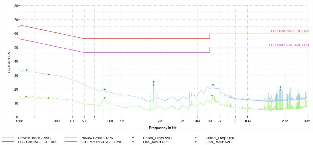
Plot 7-39. AC Line-Conducted Test Plot (N, GFSK ePA – Ch.39, with AC/DC adaptor via USB-C cable with magnetic charger)
