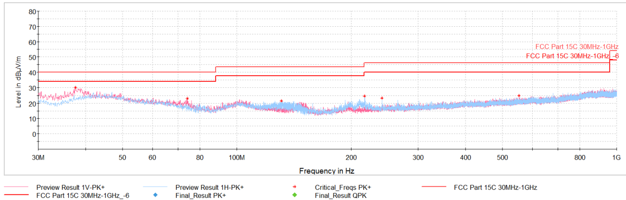
Plot 7-37. Radiated Spurious Emissions Below 1GHz (GFSK ePA – Ch.39, with AC/DC adaptor via USB-C cable with magnetic charger)
