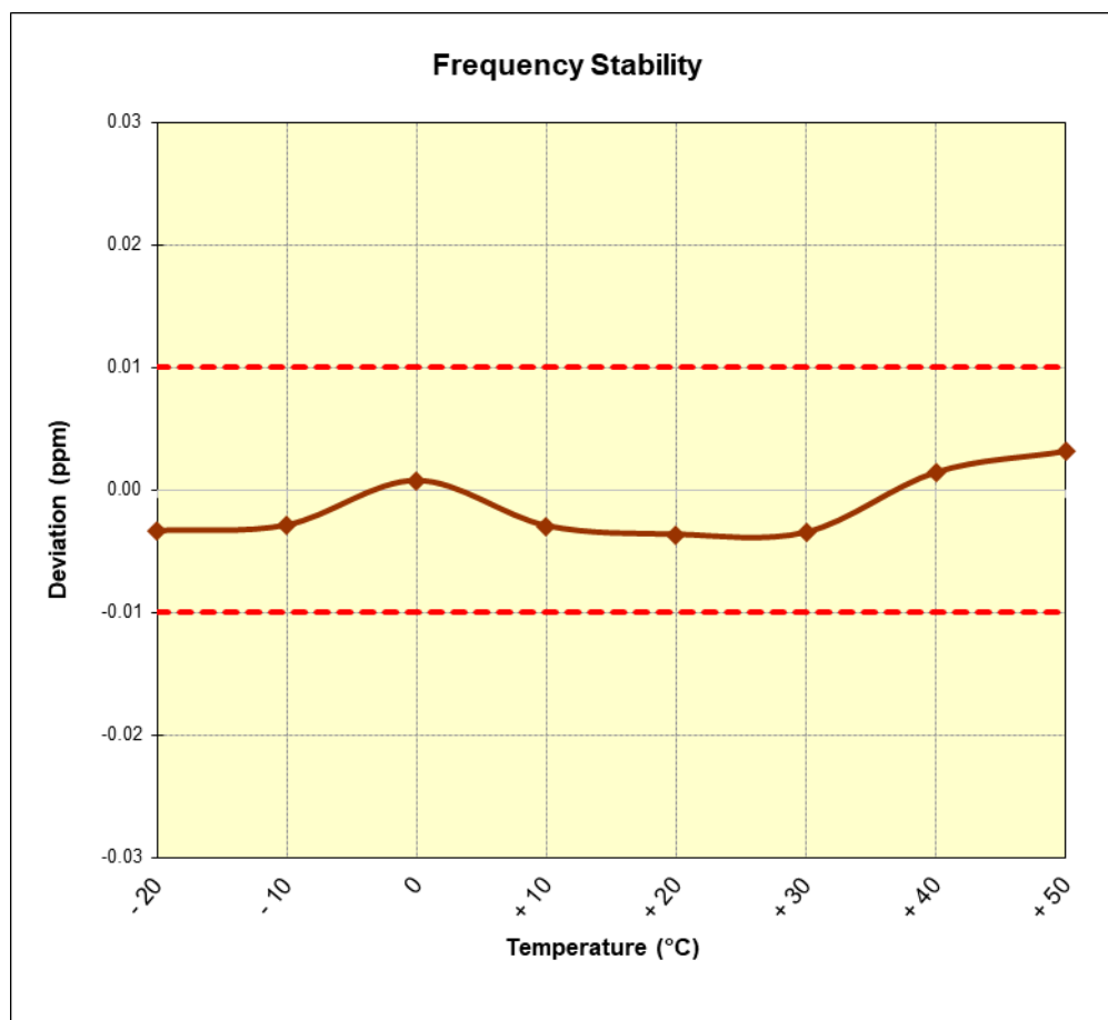
Figure 7-4. Frequency Stability Plot (Reader Type A 848K)
