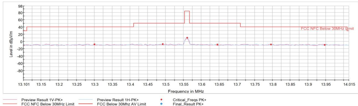
Plot 7-6. In Band Radiated Spurious Emissions (CE F 424kbps, with AC/DC Adapter and Magnetic Charger)
