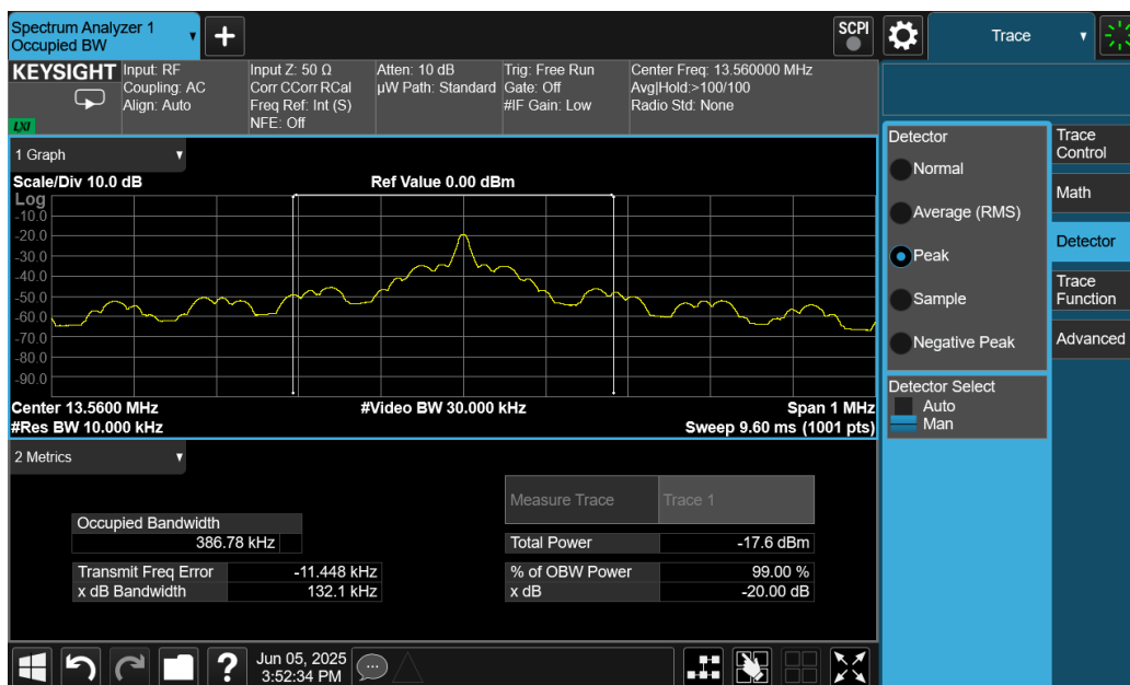
Plot 7-5. 20dB and 99% Bandwidth Plot (Reader 10% ASK 1 out of 125)
