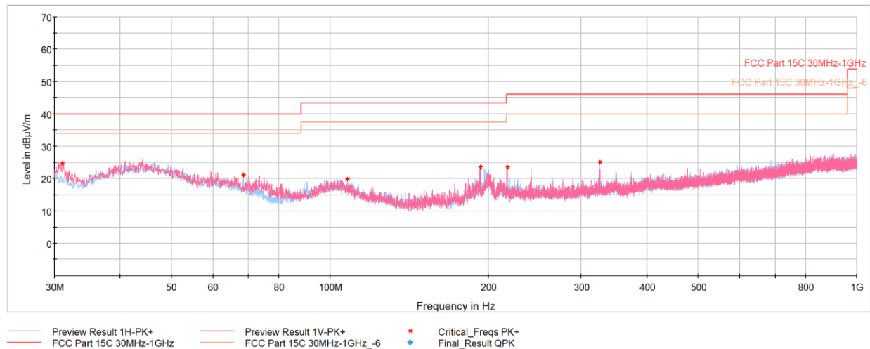
Plot 7-10. Radiated Spurious Emissions 30MHz – 1GHz (CE F 424kbps, with AC/DC Adapter and Magnetic Charger)
