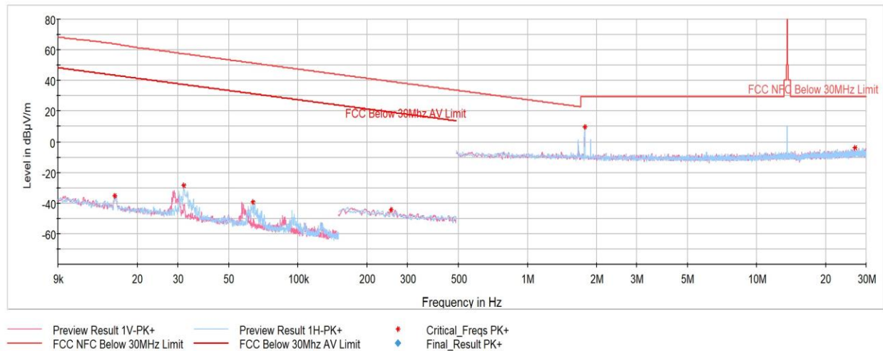
Plot 7-8. Radiated Spurious Emissions 9kHz – 30MHz (CE F 424kbps, with AC/DC Adapter and Magnetic Charger)
