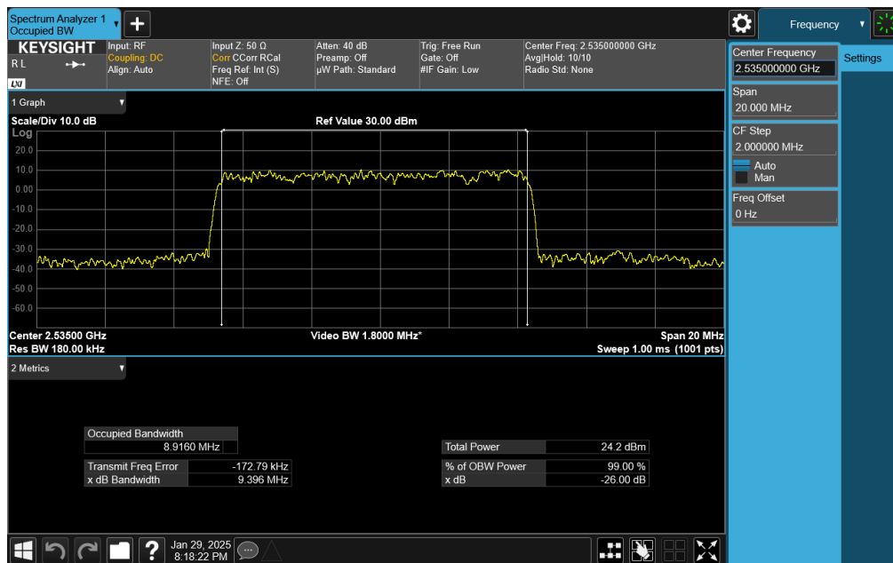
Plot 7-24. Occupied Bandwidth Plot (NR Band n7 - CP-OFDM 10MHz 64-QAM - Full RB)
