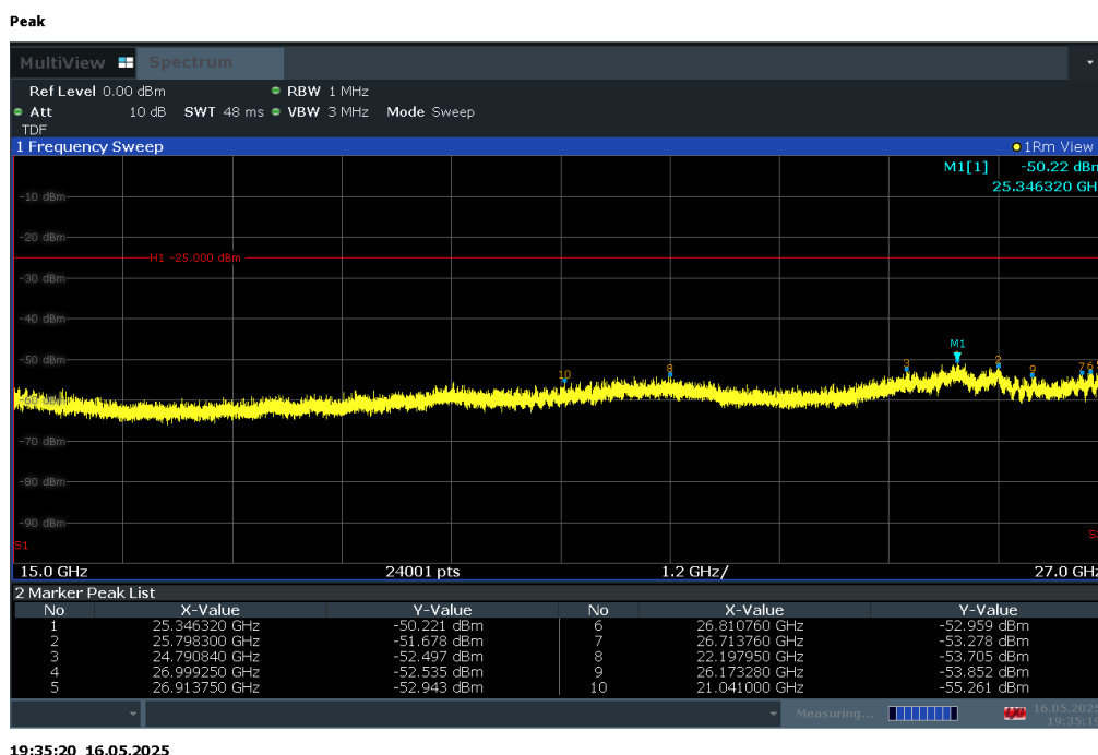
Plot 7-59. Conducted Spurious Plot (LTE Band 41 - 20MHz QPSK - RB Size 1, RB Offset 50 - Mid Channel)
