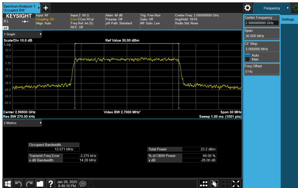
Plot 7-40. Occupied Bandwidth Plot (NR Band n41 - CP-OFDM 15MHz 64-QAM - Full RB)
