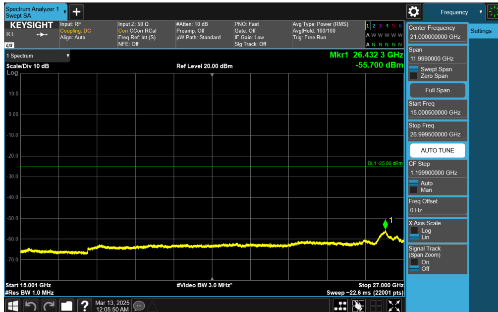
Plot 7-68. Conducted Spurious Plot (NR Band n7 - 20MHz DFT-s-OFDM QPSK - RB Size 1, RB Offset 50 - Mid Channel)
