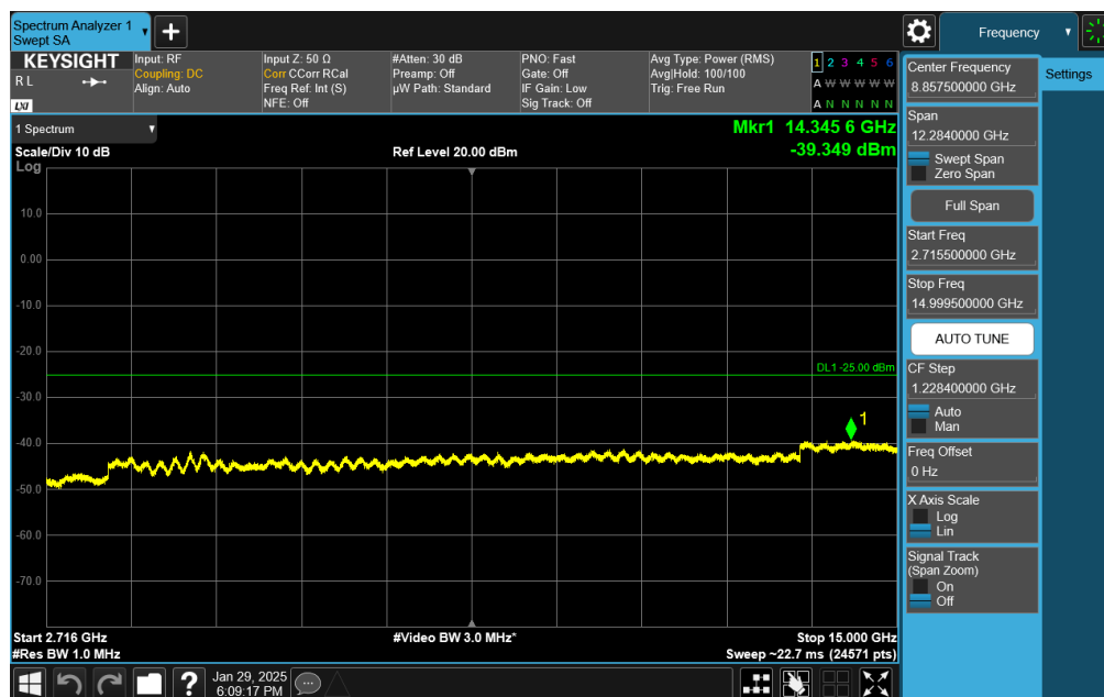
Plot 7-79. Conducted Spurious Plot (NR Band n41 - 20MHz DFT-s-OFDM QPSK - RB Size 1, RB Offset 50 - High Channel)
