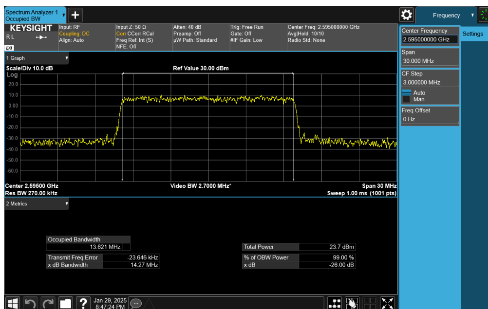
Plot 7-38. Occupied Bandwidth Plot (NR Band n41 - CP-OFDM 15MHz QPSK - Full RB)
