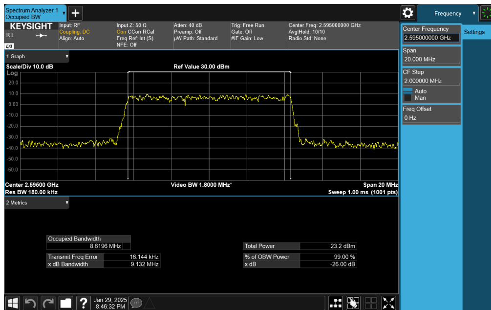
Plot 7-36. Occupied Bandwidth Plot (NR Band n41 - CP-OFDM 10MHz 64-QAM - Full RB)
