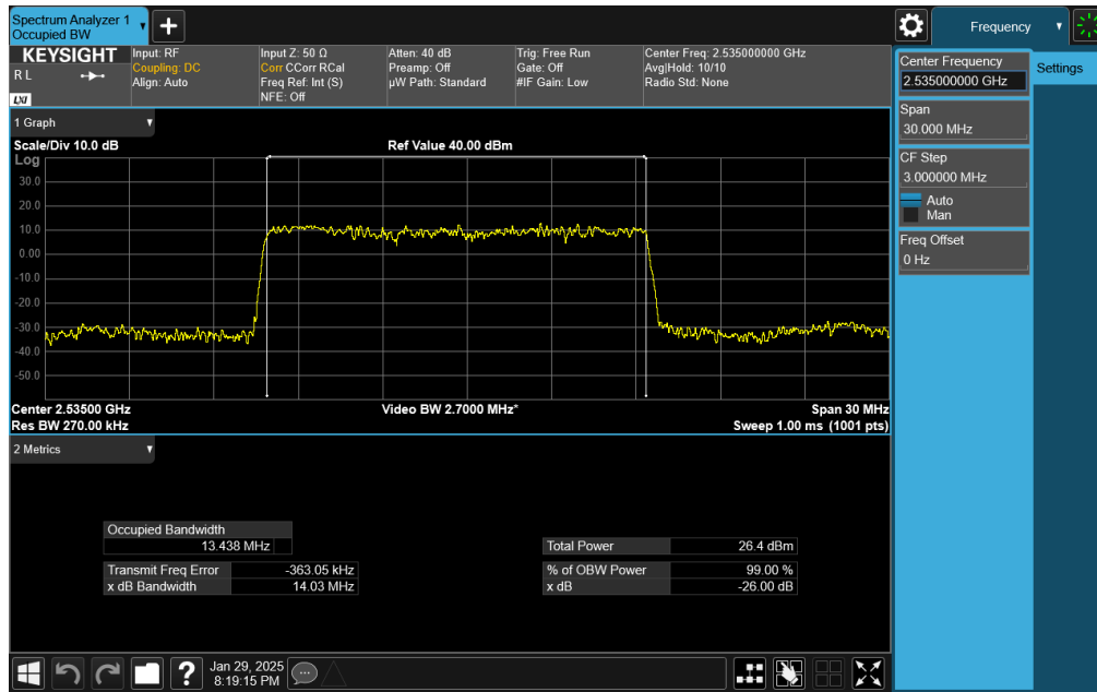
Plot 7-25. Occupied Bandwidth Plot (NR Band n7 - 15MHz DFT-s-OFDM \pi/2 BPSK - Full RB)
