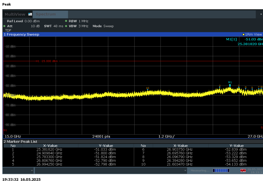
Plot 7-56. Conducted Spurious Plot (LTE Band 41 - 20MHz QPSK - RB Size 1, RB Offset 50 - Low Channel)
