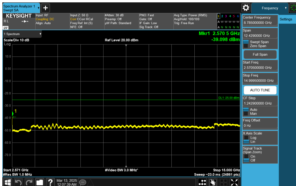
Plot 7-70. Conducted Spurious Plot (NR Band n7 - 20MHz DFT-s-OFDM QPSK - RB Size 1, RB Offset 50 - High Channel)
