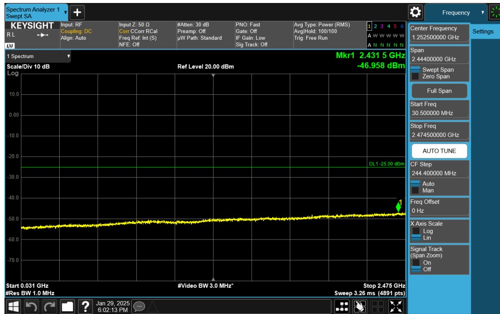
Plot 7-72. Conducted Spurious Plot (NR Band n41 - 20MHz DFT-s-OFDM QPSK - RB Size 1, RB Offset 50 - Low Channel)
