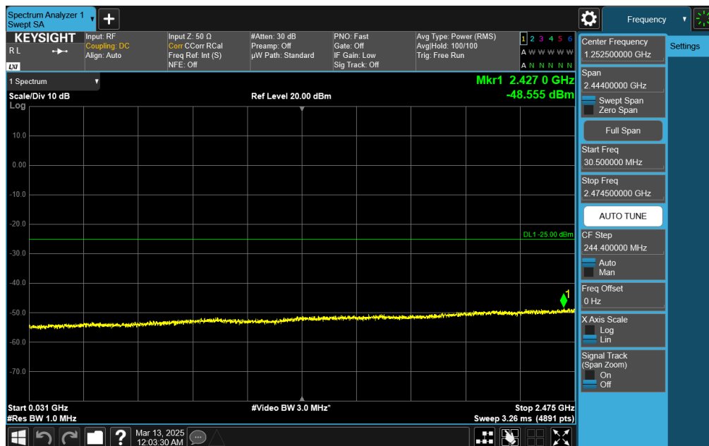
Plot 7-66. Conducted Spurious Plot (NR Band n7 - 20MHz DFT-s-OFDM QPSK - RB Size 1, RB Offset 50 - Mid Channel)
