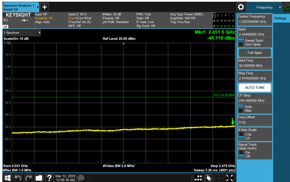
Plot 7-69. Conducted Spurious Plot (NR Band n7 - 20MHz DFT-s-OFDM QPSK - RB Size 1, RB Offset 50 - High Channel)
