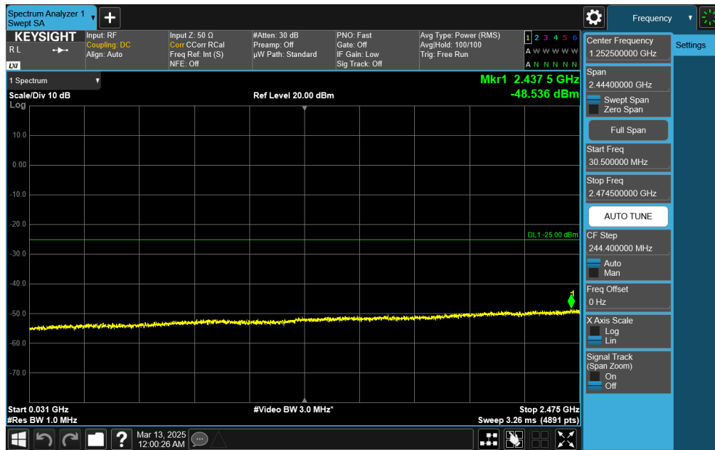
Plot 7-63. Conducted Spurious Plot (NR Band n7 - 20MHz DFT-s-OFDM QPSK - RB Size 1, RB Offset 50 - Low Channel)
