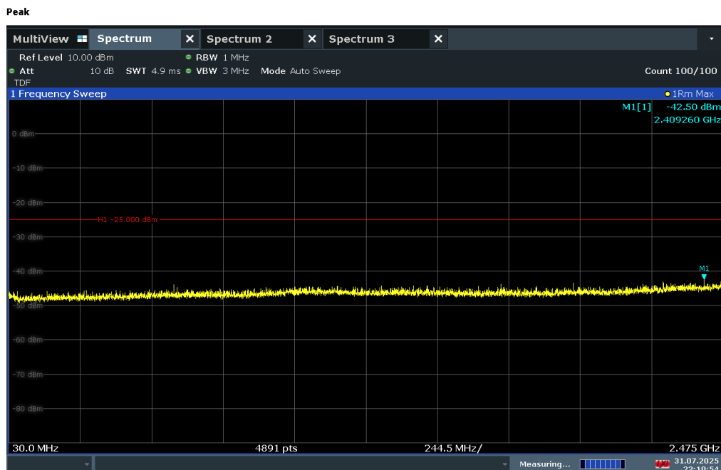
Plot 7-81. Simultaneous Tx Conducted Spurious Plot (NR Band n41 + BT + UNII)
