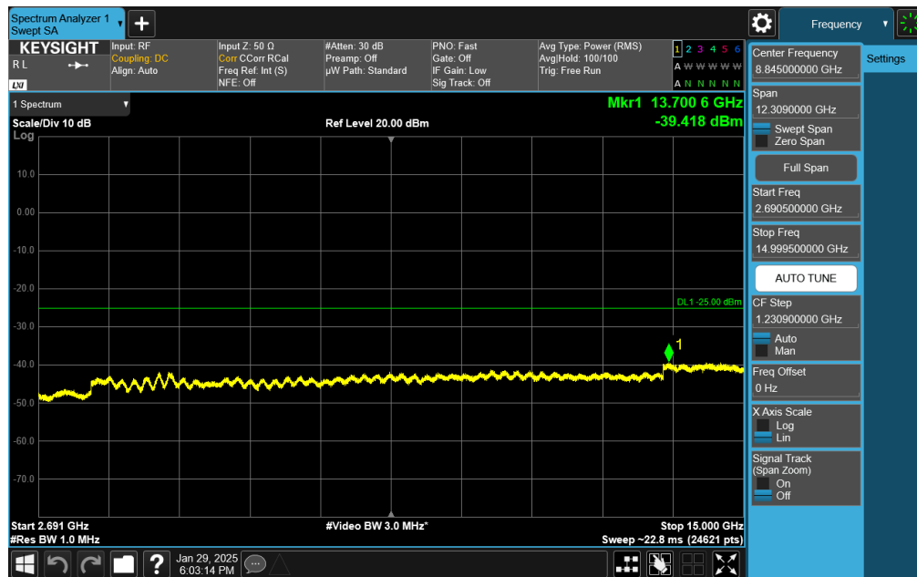
Plot 7-73. Conducted Spurious Plot (NR Band n41 - 20MHz DFT-s-OFDM QPSK - RB Size 1, RB Offset 50 - Low Channel)
