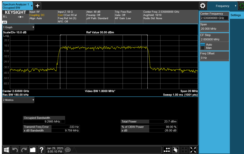
Plot 7-23. Occupied Bandwidth Plot (NR Band n7 - CP-OFDM 10MHz 16-QAM - Full RB)
