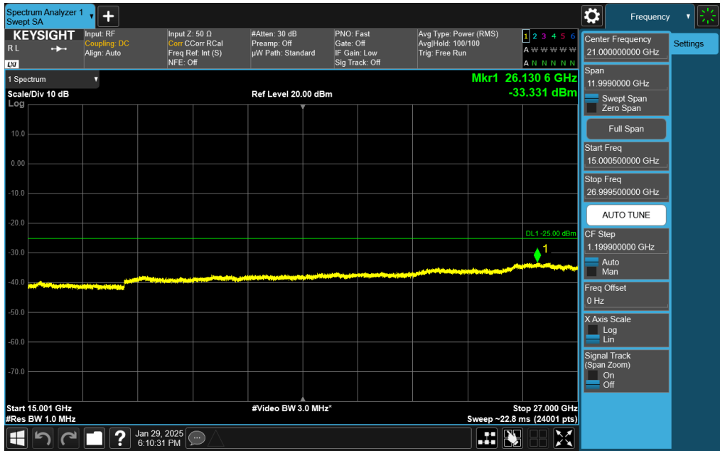
Plot 7-80. Conducted Spurious Plot (NR Band n41 - 20MHz DFT-s-OFDM QPSK - RB Size 1, RB Offset 50 - High Channel)
