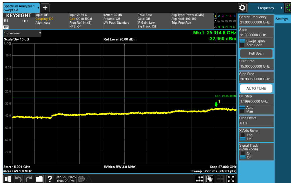
Plot 7-74. Conducted Spurious Plot (NR Band n41 - 20MHz DFT-s-OFDM QPSK - RB Size 1, RB Offset 50 - Low Channel)
