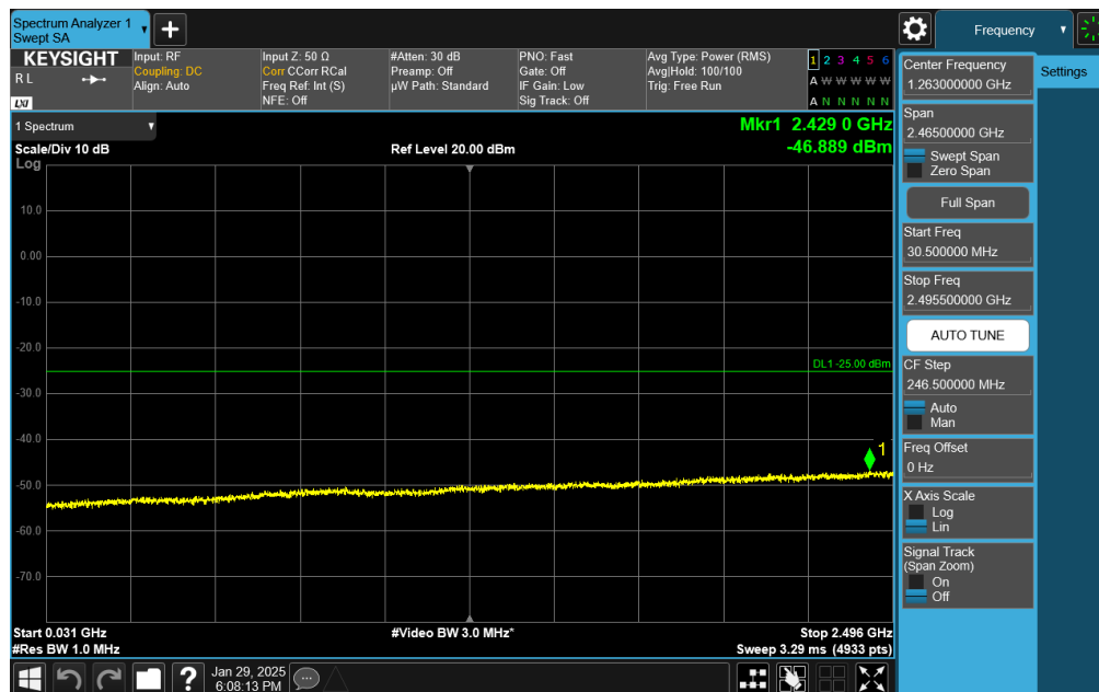
Plot 7-78. Conducted Spurious Plot (NR Band n41 - 20MHz DFT-s-OFDM QPSK - RB Size 1, RB Offset 50 - High Channel)
