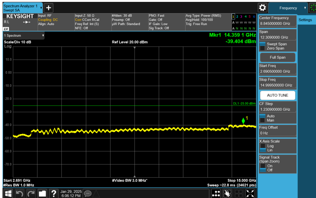
Plot 7-76. Conducted Spurious Plot (NR Band n41 - 20MHz DFT-s-OFDM QPSK - RB Size 1, RB Offset 50 - Mid Channel)
