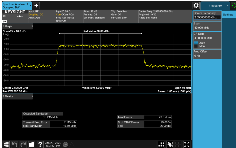
Plot 7-43. Occupied Bandwidth Plot (NR Band n41 - CP-OFDM 20MHz 16-QAM - Full RB)
