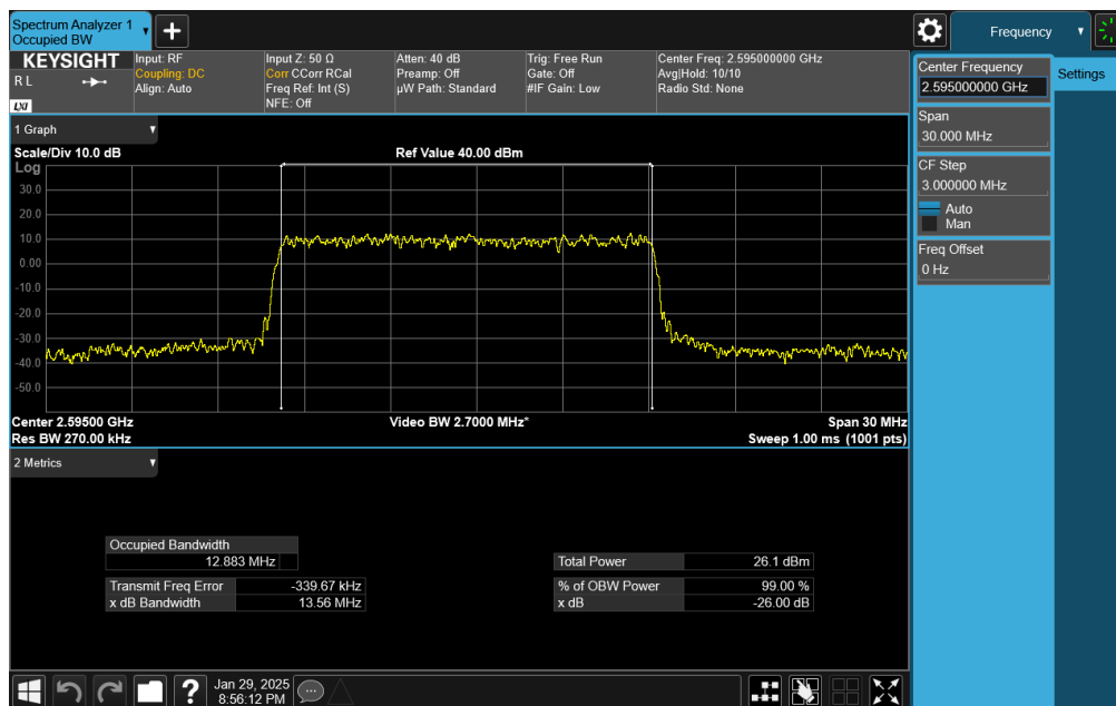
Plot 7-37. Occupied Bandwidth Plot (NR Band n41 - 15MHz DFT-s-OFDM \pi/2 BPSK - Full RB)
