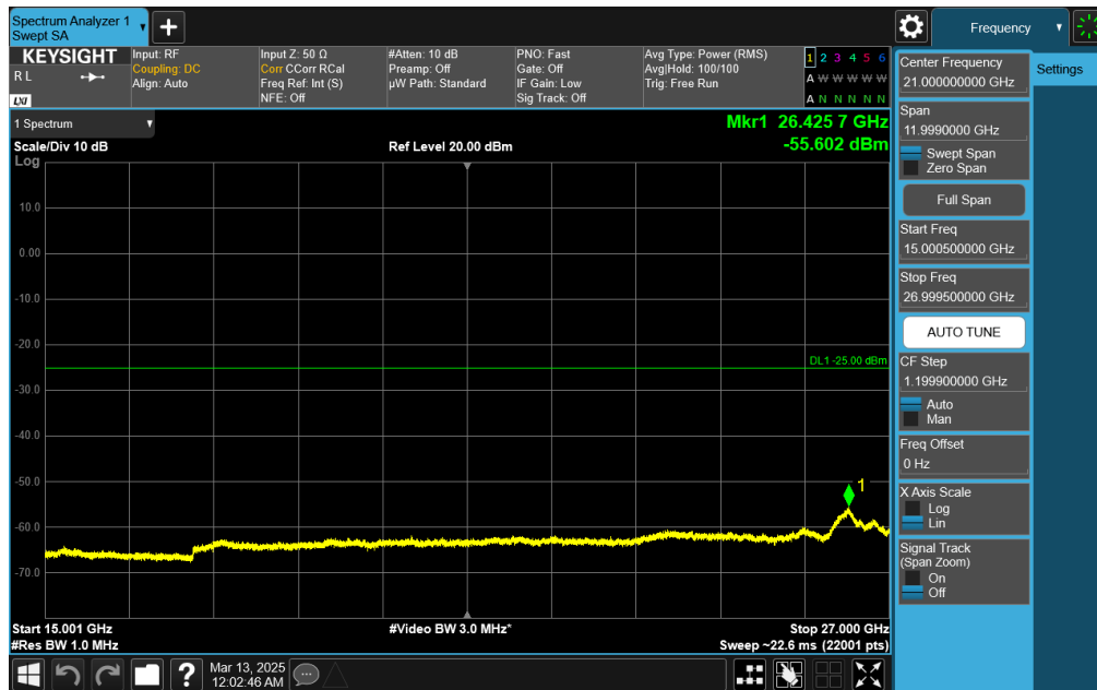
Plot 7-65. Conducted Spurious Plot (NR Band n7 - 20MHz DFT-s-OFDM QPSK - RB Size 1, RB Offset 50 - Low Channel)
