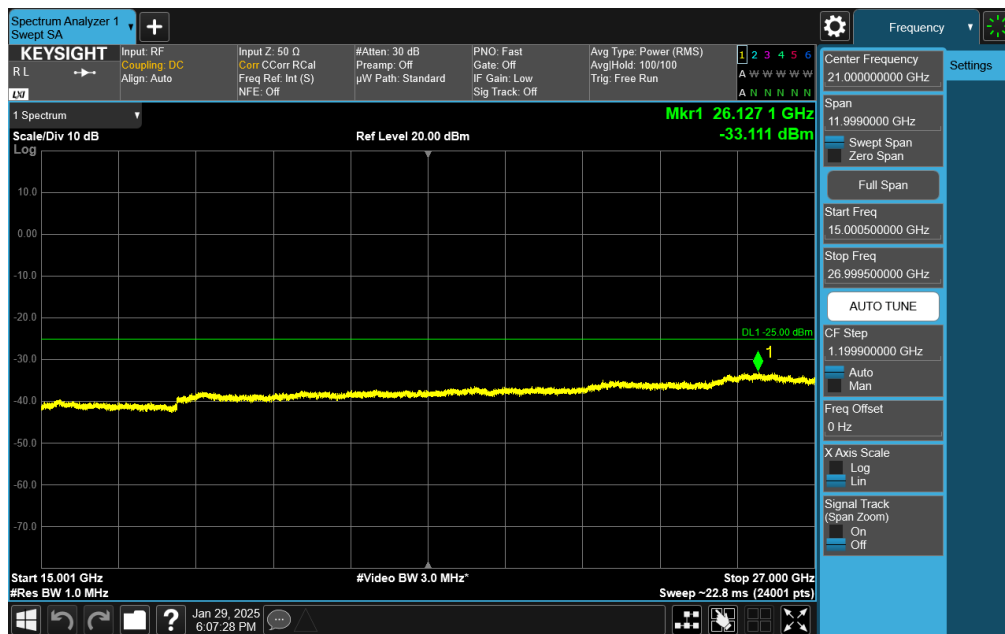
Plot 7-77. Conducted Spurious Plot (NR Band n41 - 20MHz DFT-s-OFDM QPSK - RB Size 1, RB Offset 50 - Mid Channel)
