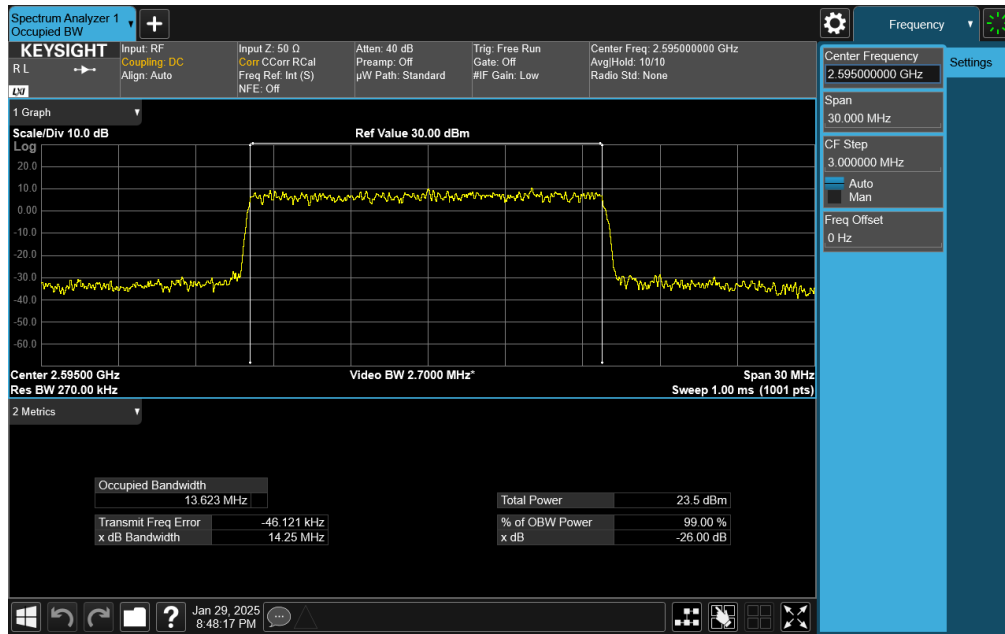
Plot 7-39. Occupied Bandwidth Plot (NR Band n41 - CP-OFDM 15MHz 16-QAM - Full RB)
