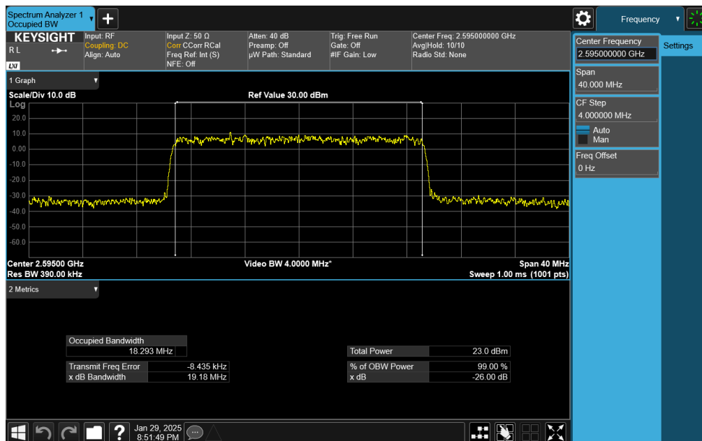
Plot 7-44. Occupied Bandwidth Plot (NR Band n41 - CP-OFDM 20MHz 64-QAM - Full RB)
