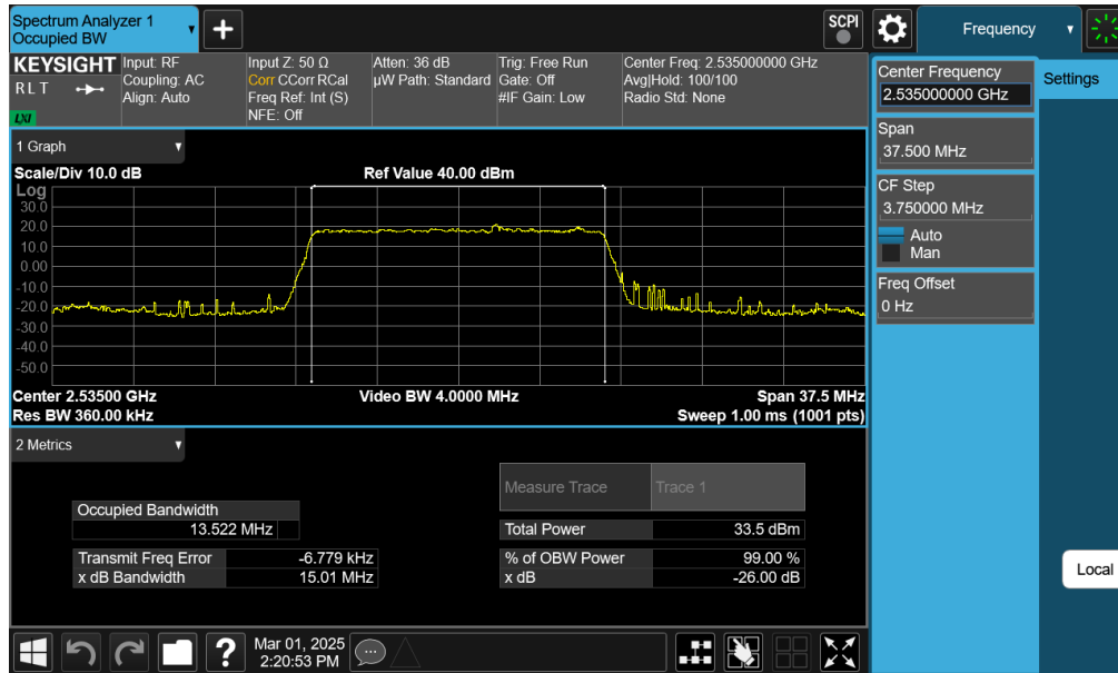
Plot 7-5. Occupied Bandwidth Plot (LTE Band 7 - 15MHz QPSK - Full RB)
