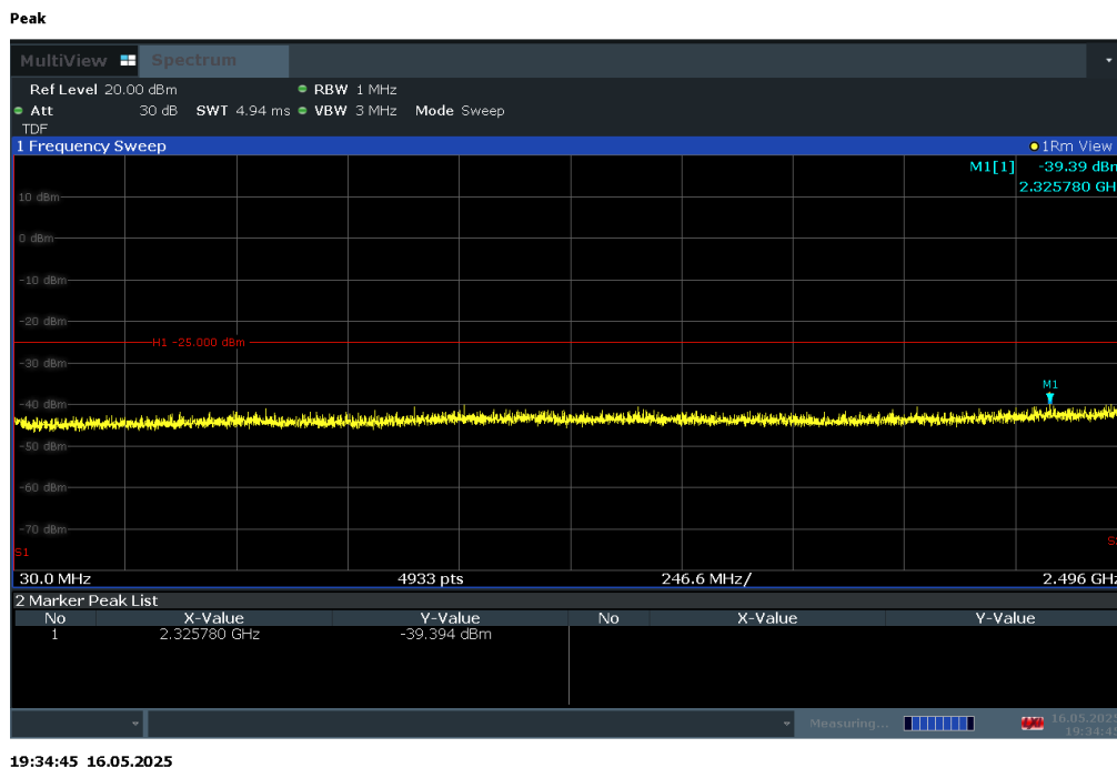
Plot 7-57. Conducted Spurious Plot (LTE Band 41 - 20MHz QPSK - RB Size 1, RB Offset 50 - Mid Channel)
