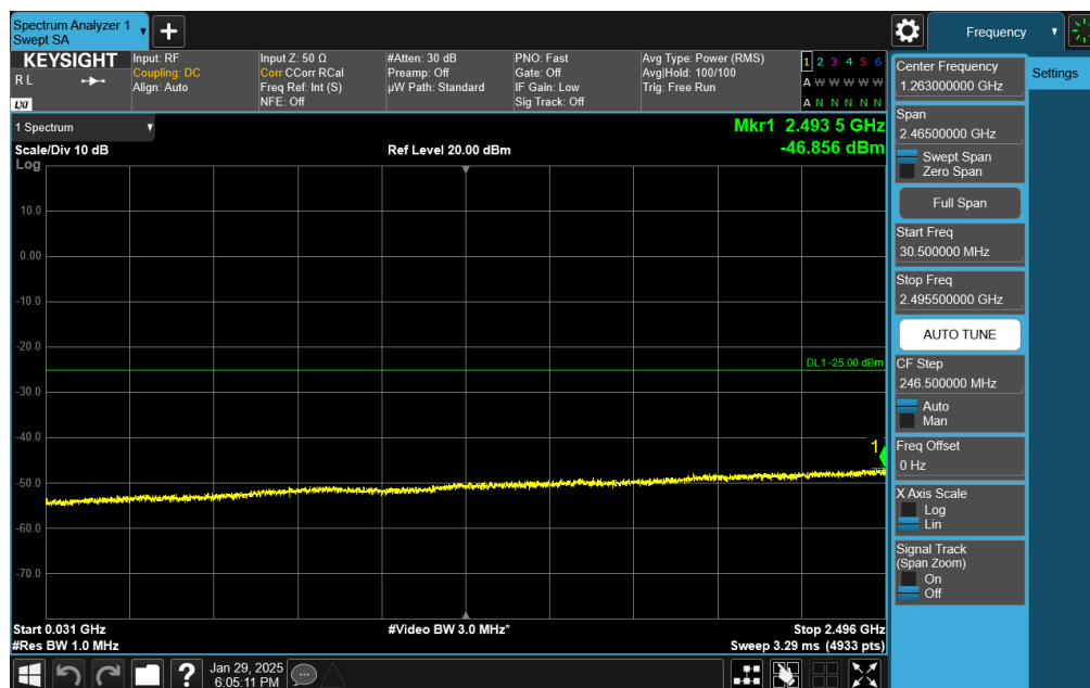
Plot 7-75. Conducted Spurious Plot (NR Band n41 - 20MHz DFT-s-OFDM QPSK - RB Size 1, RB Offset 50 - Mid Channel)
