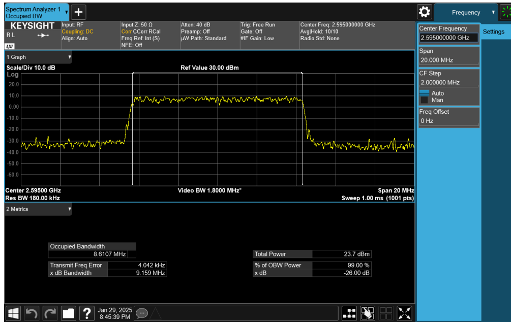
Plot 7-35. Occupied Bandwidth Plot (NR Band n41 - CP-OFDM 10MHz 16-QAM - Full RB)
