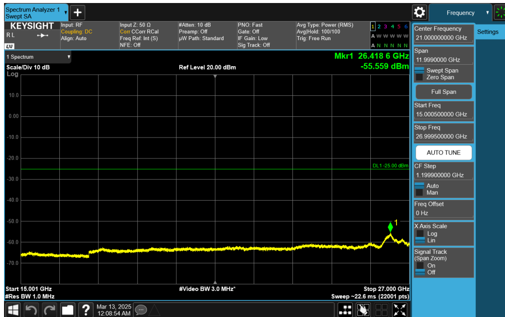
Plot 7-71. Conducted Spurious Plot (NR Band n7 - 20MHz DFT-s-OFDM QPSK - RB Size 1, RB Offset 50 - High Channel)
