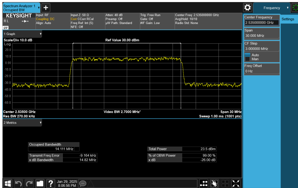
Plot 7-26. Occupied Bandwidth Plot (NR Band n7 - CP-OFDM 15MHz QPSK - Full RB)
