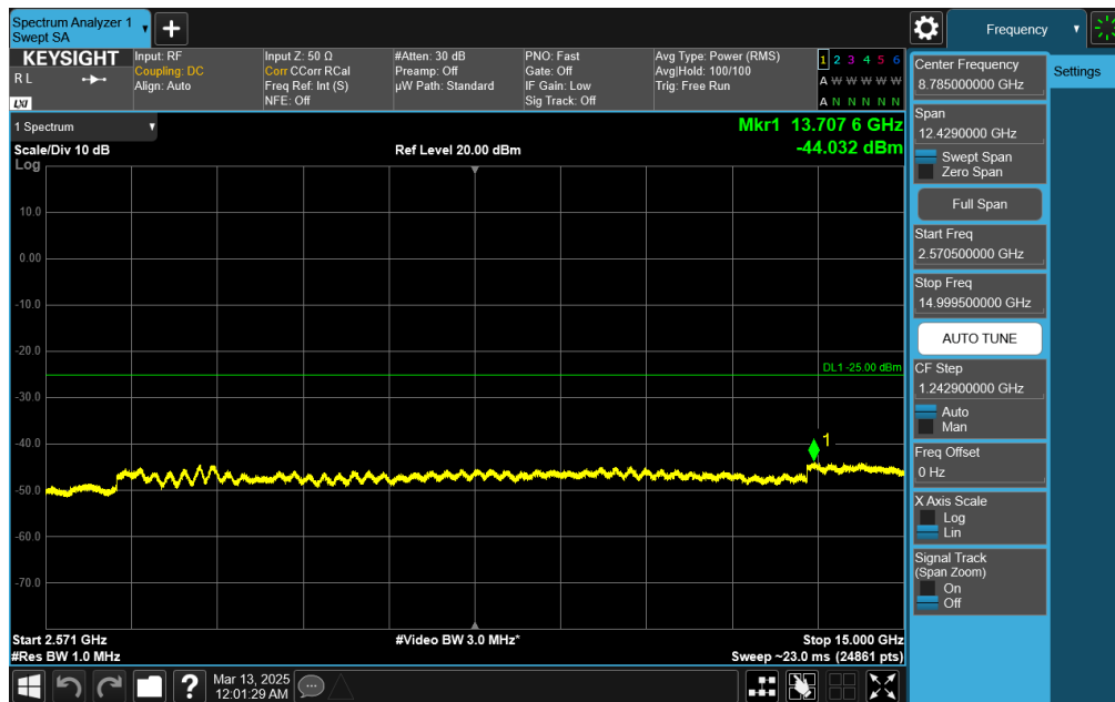
Plot 7-64. Conducted Spurious Plot (NR Band n7 - 20MHz DFT-s-OFDM QPSK - RB Size 1, RB Offset 50 - Low Channel)
