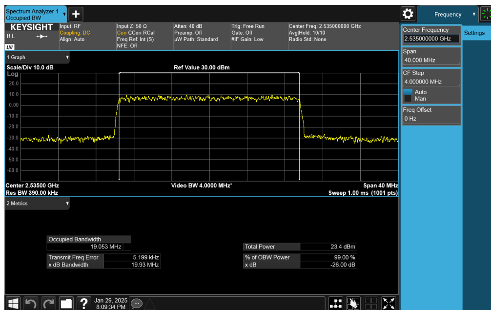
Plot 7-30. Occupied Bandwidth Plot (NR Band n7 - CP-OFDM 20MHz QPSK - Full RB)
