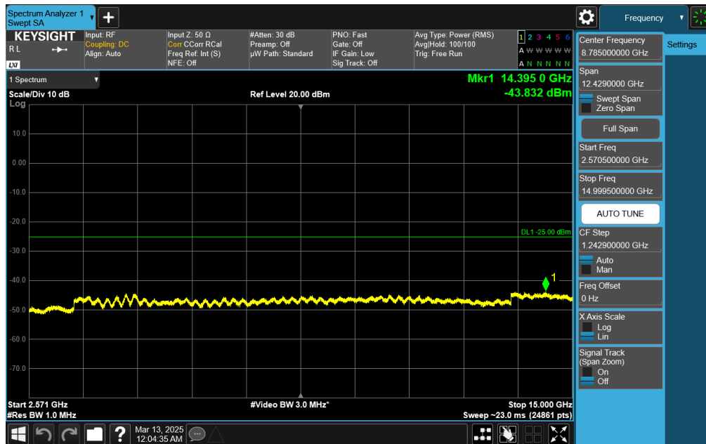
Plot 7-67. Conducted Spurious Plot (NR Band n7 - 20MHz DFT-s-OFDM QPSK - RB Size 1, RB Offset 50 - Mid Channel)
